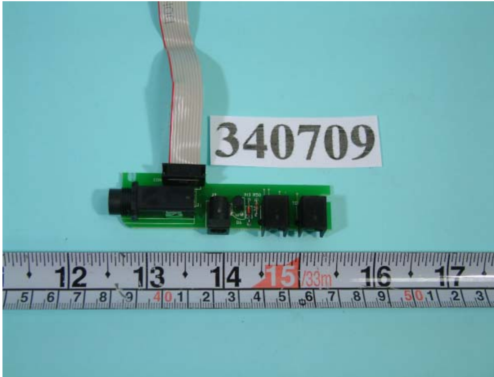
Front side of daughter board
