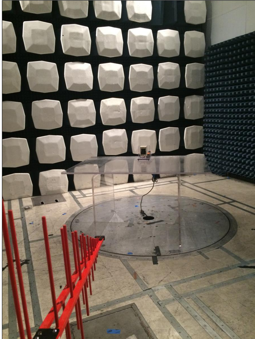
Photograph 2. Radiated Spurious Emissions, Test Setup, Below 1 GHz
