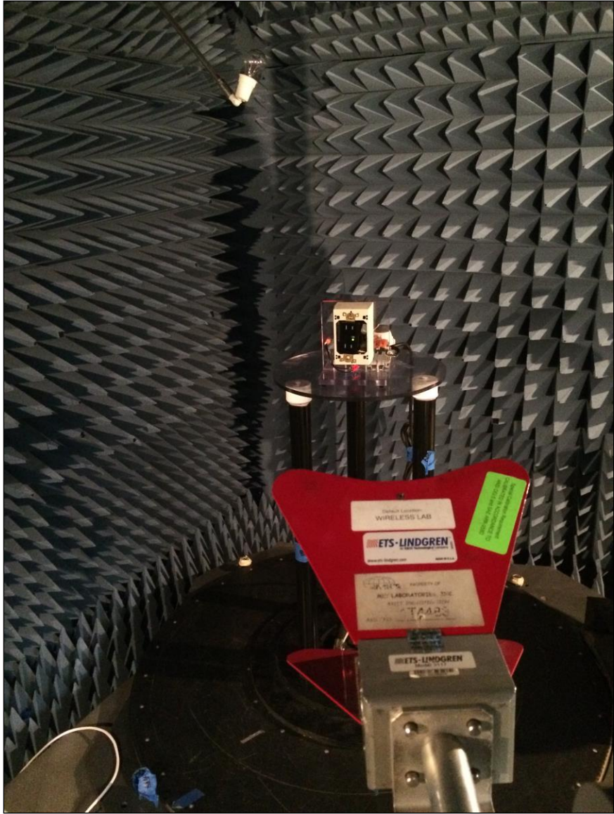
Photograph 3. Radiated Spurious Emissions, Test Setup, Above 1 GHz
