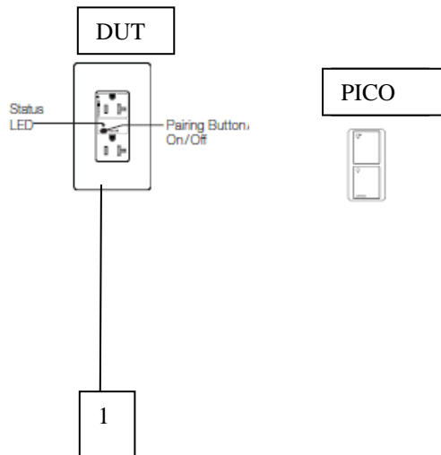
Figure 1. Block Diagram of Test Configuration
