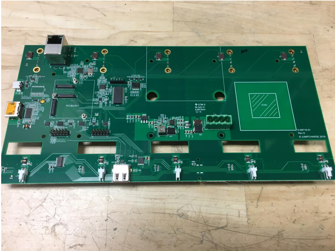
Figure 4 – Internal Photo of Base PCB Assembly (Top)
