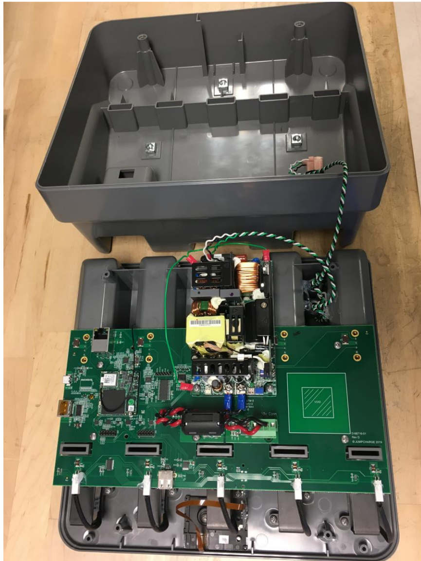
Figure 1 – Internal Photo of Open Assembly
