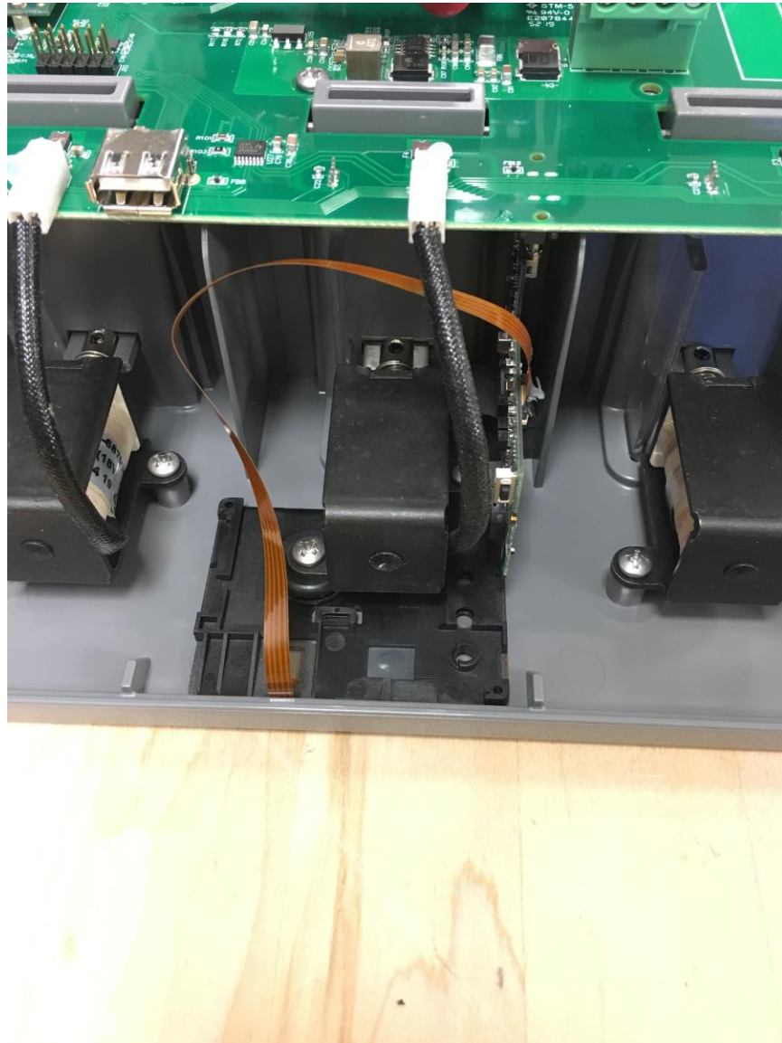
Figure 3 – Internal Photo of NFC Module Installation
