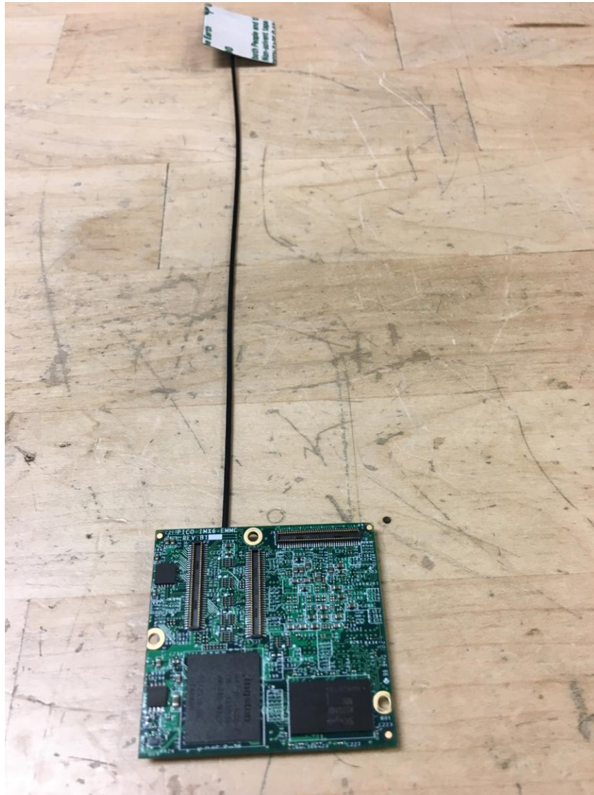
Figure 9 – Internal Photo of Processor Assembly with WIFI/BLE Module (Bottom)
