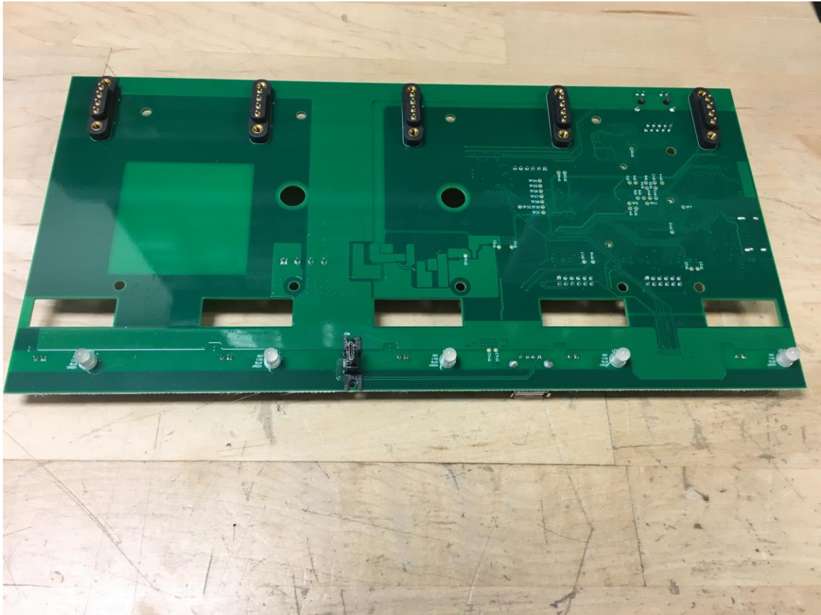
Figure 5 – Internal Photo of Base PCB Assembly (Bottom)
