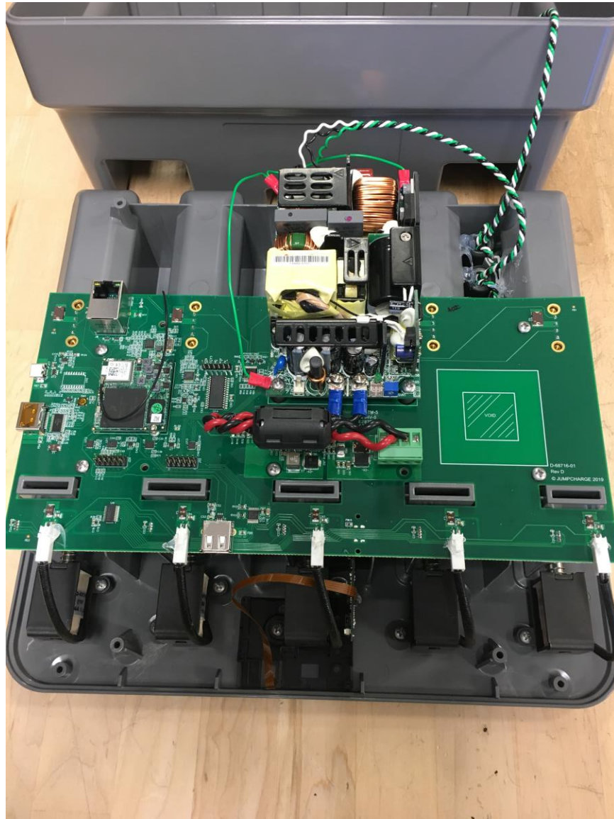
Figure 2 – Internal Photo of Base Electrical Assembly
