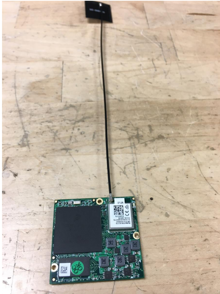
Figure 8 – Internal Photo of Processor Assembly with WIFI/BLE Module (Top)
