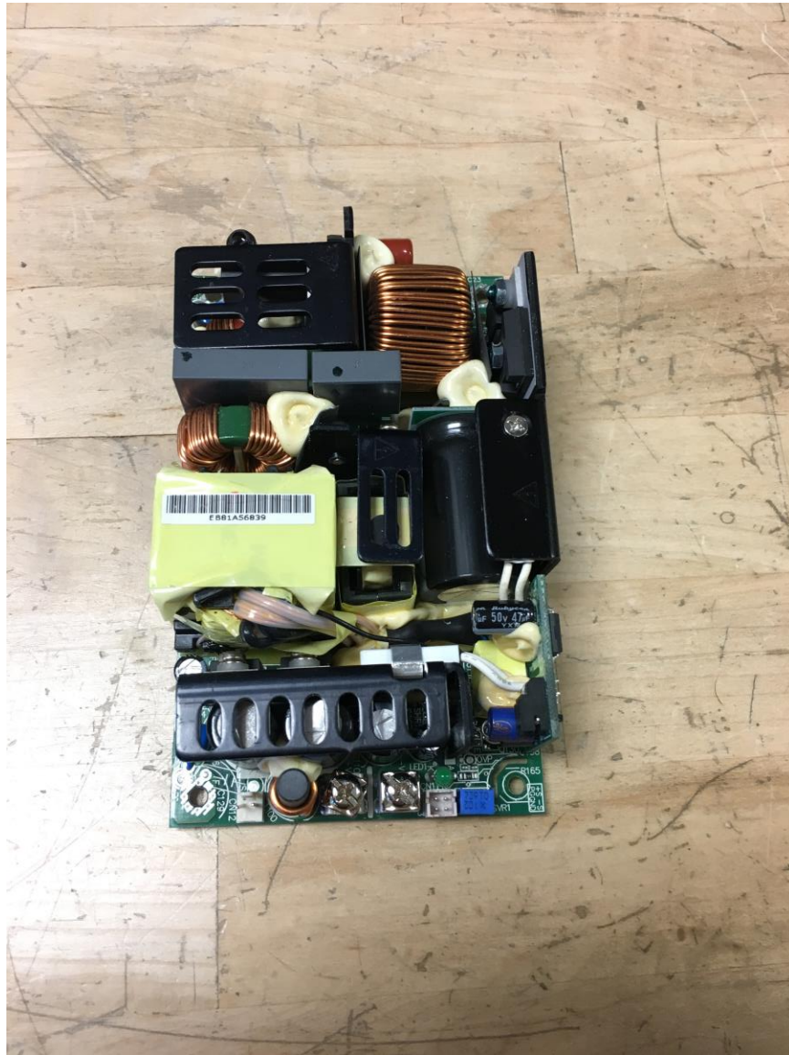
Figure 6 – Internal Photo of Power Supply Assembly (Top)
