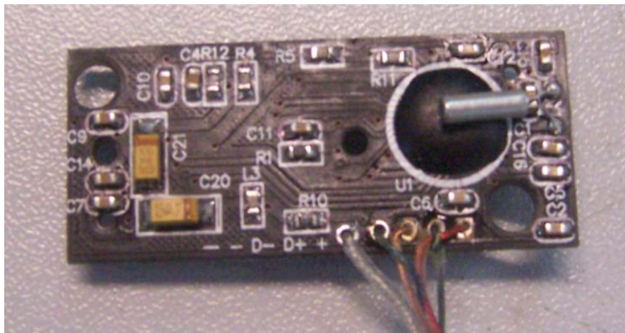
Photo 3- Back View of PCBA
