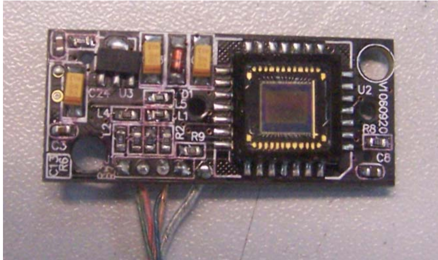
Photo 2- Front View of PCBA
