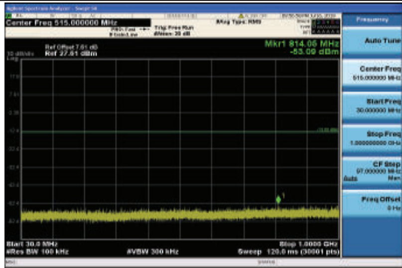
Band25-5MHz-16QAM-26065-1RB#0-30~1000MHz
