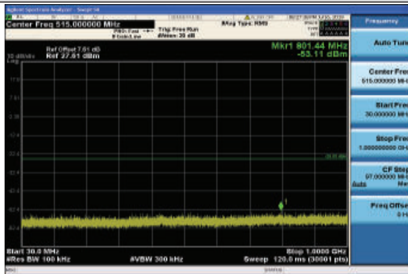
Band41-5MHz-16QAM-41215-1RB#0-30~1000MHz
