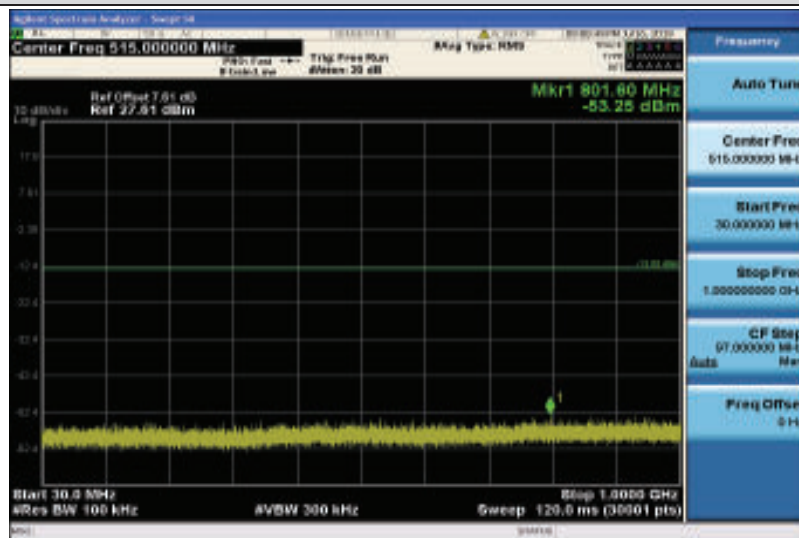
Band25-3MHz-16QAM-26365-1RB#0-30~1000MHz
