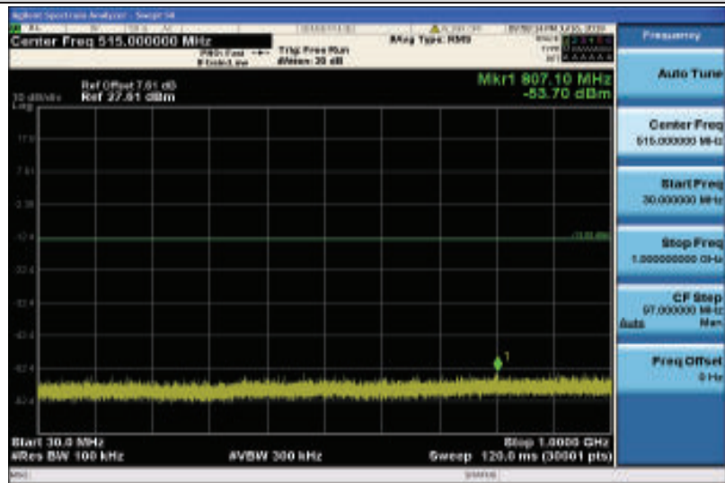
Band25-5MHz-16QAM-26365-1RB#0-30~1000MHz
