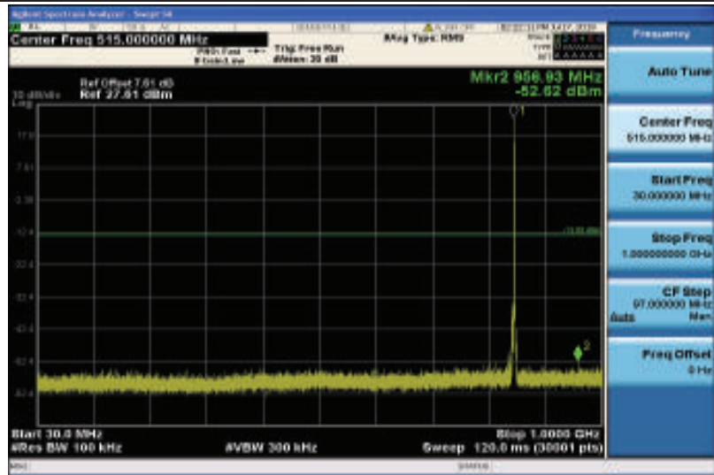
Band26-1.4MHz-QPSK-27033-1RB#0-30~1000MHz
