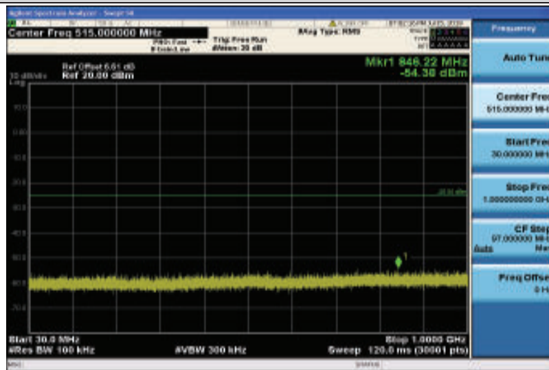
Band38-15MHz-QPSK-38175-1RB#0-Range1:30~1000MHz
