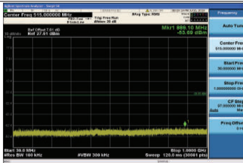
Band41-5MHz-QPSK-40620-1RB#0-30~1000MHz
