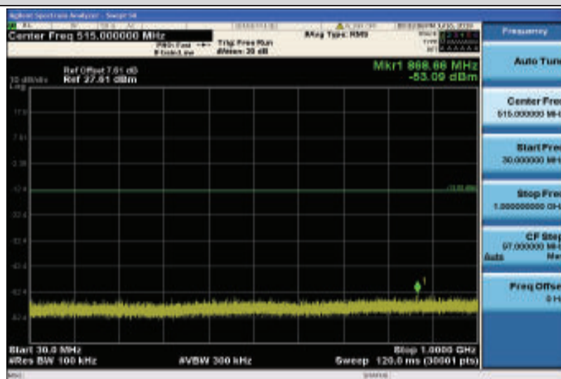
Band25-10MHz-16QAM-26365-1RB#0-30~1000MHz
