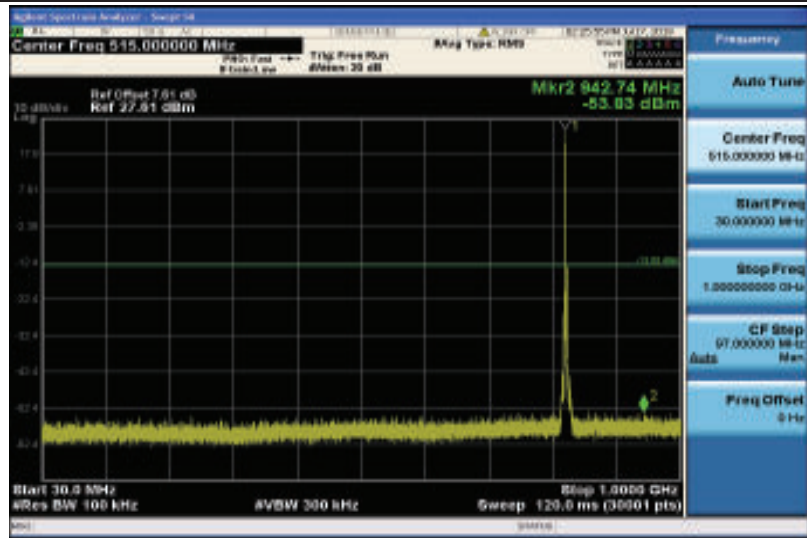
Band26-3MHz-16QAM-26805-1RB#0-30~1000MHz
