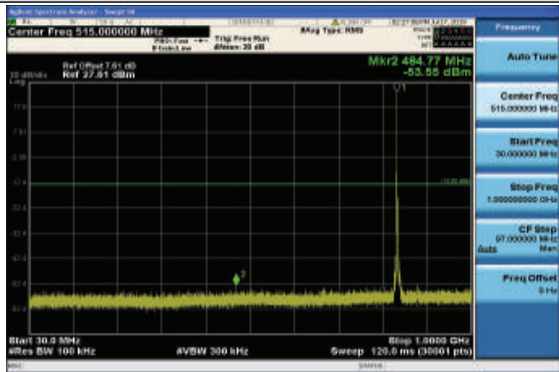
Band26-3MHz-16QAM-26915-1RB#0-30~1000MHz
