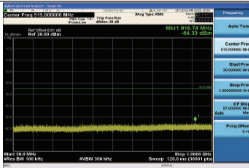
Band38-20MHz-16QAM-38150-1RB#0-Range1:30~1000MHz
