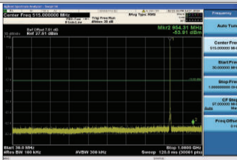
Band26-1.4MHz-16QAM-26915-1RB#0-30~1000MHz
