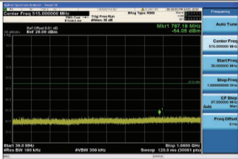
Band38-5MHz-16QAM-38000-1RB#0-Range1:30~1000MHz
