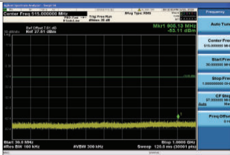
Band25-3MHz-16QAM-26675-1RB#0-30~1000MHz
