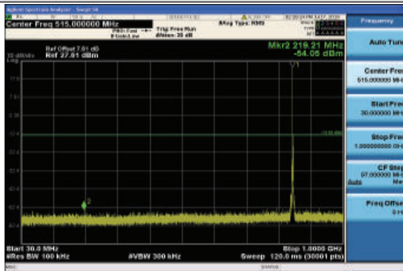
Band26-3MHz-16QAM-27025-1RB#0-30~1000MHz
