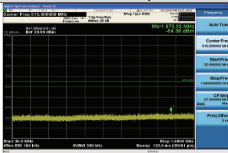
Band7-5MHz-16QAM-21100-1RB#0-Range1:30~1000MHz
