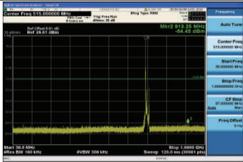
Band12-10MHz-16QAM-23060-1RB#0-Range1:30~1000MHz
