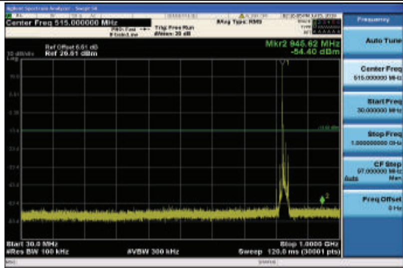
Band5-10MHz-16QAM-20450-1RB#0-Range1:30~1000MHz
