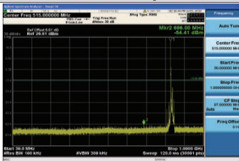
Band5-10MHz-QPSK-20525-1RB#0-Range1:30~1000MHz
