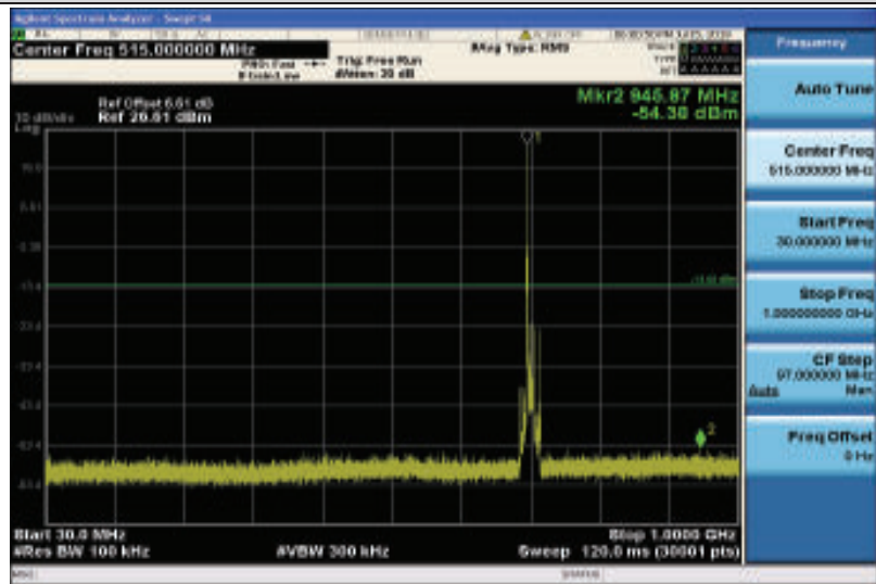
Band12-10MHz-16QAM-23095-1RB#0-Range1:30~1000MHz
