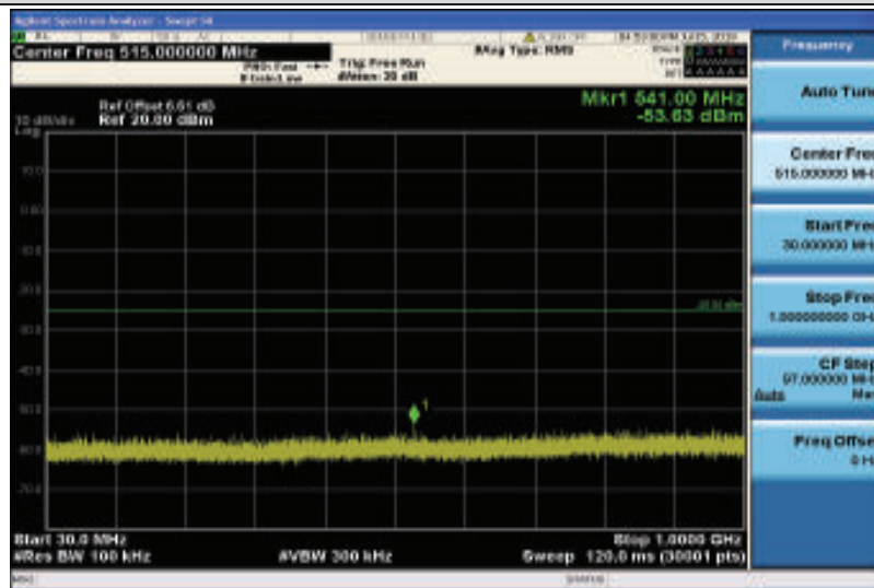
Band7-20MHz-QPSK-21350-1RB#0-Range1:30~1000MHz
