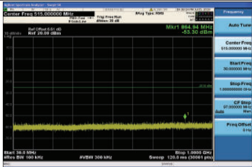
Band7-10MHz-QPSK-21400-1RB#0-Range1:30~1000MHz
