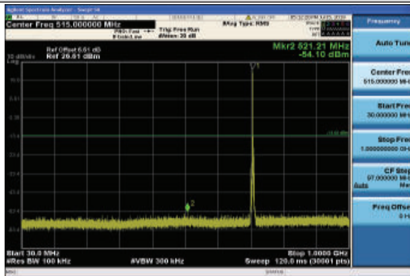
Band12-3MHz-QPSK-23165-1RB#0-Range1:30~1000MHz
