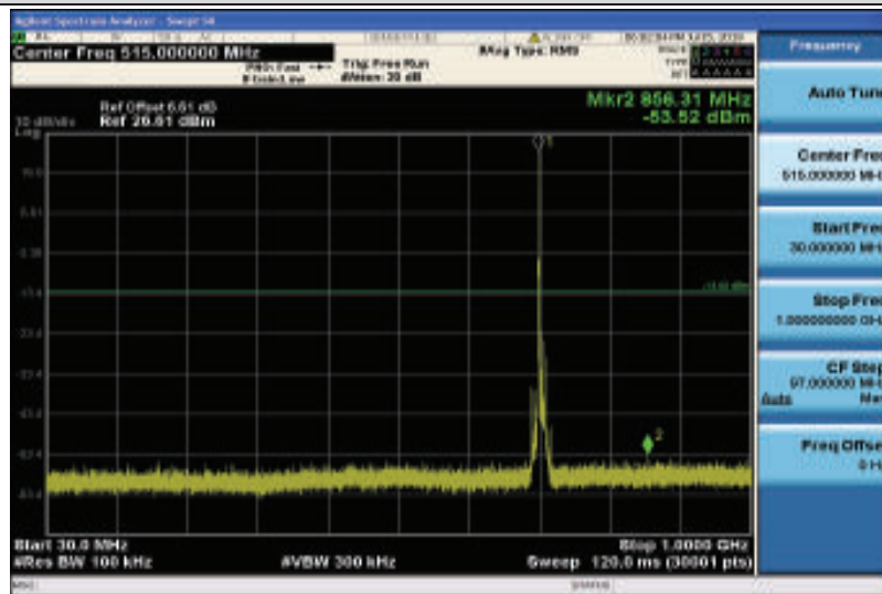
Band12-10MHz-16QAM-23130-1RB#0-Range1:30~1000MHz
