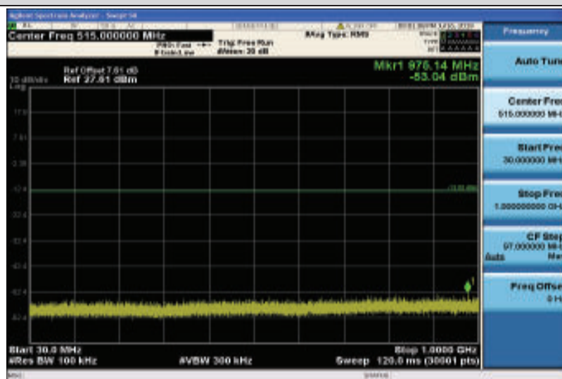
Band25-1.4MHz-16QAM-26365-1RB#0-30~1000MHz
