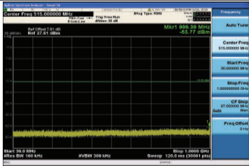
Band25-1.4MHz-QPSK-26047-1RB#0-30~1000MHz
