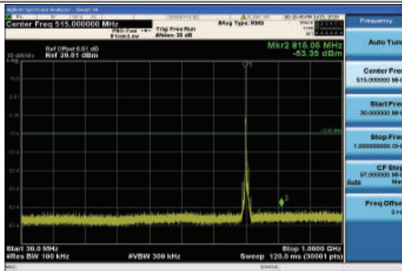
Band17-10MHz-16QAM-23800-1RB#0-Range1:30~1000MHz
