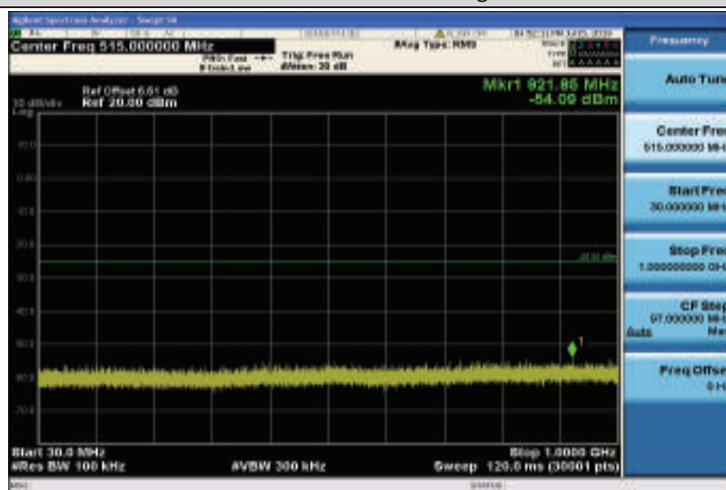
Band7-20MHz-16QAM-21100-1RB#0-Range1:30~1000MHz
