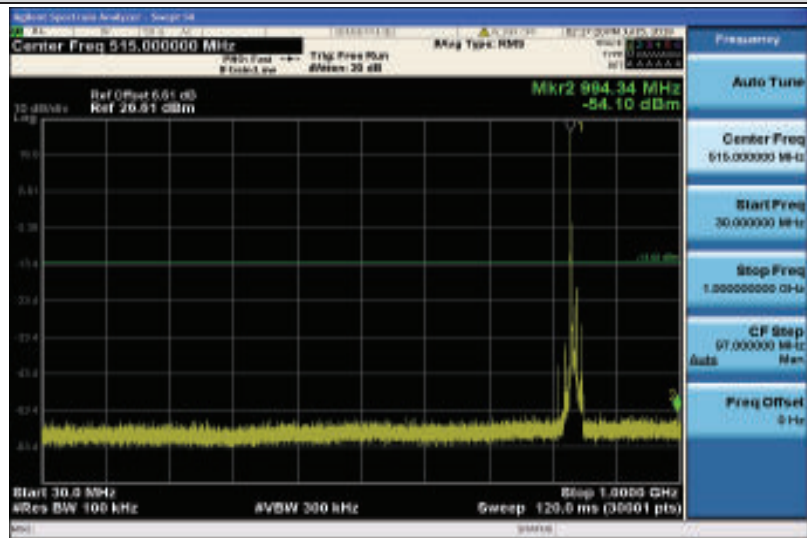
Band5-10MHz-16QAM-20525-1RB#0-Range1:30~1000MHz
