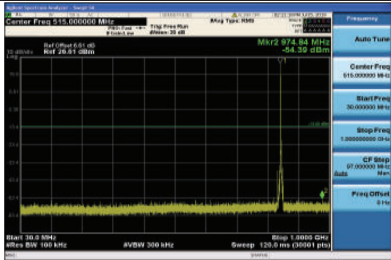
Band5-5MHz-16QAM-20625-1RB#0-Range1:30~1000MHz
