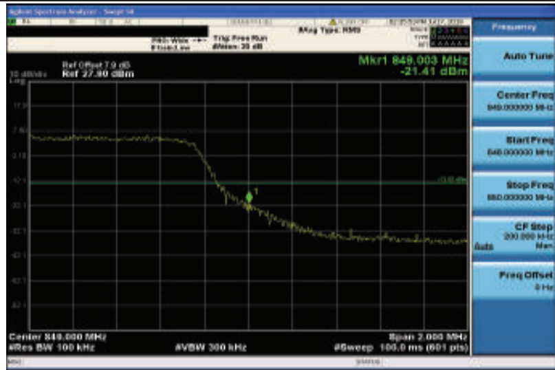
Band26-5MHz-16QAM-27015-25RB#0
