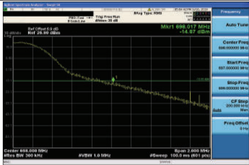
Band71-15MHz-16QAM-133397-1RB#74
