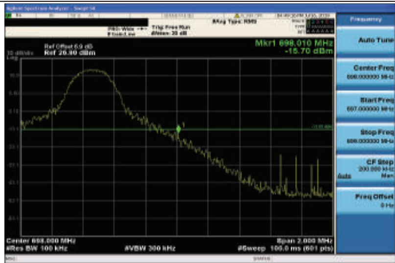
Band71-5MHz-QPSK-133447-1RB#24
