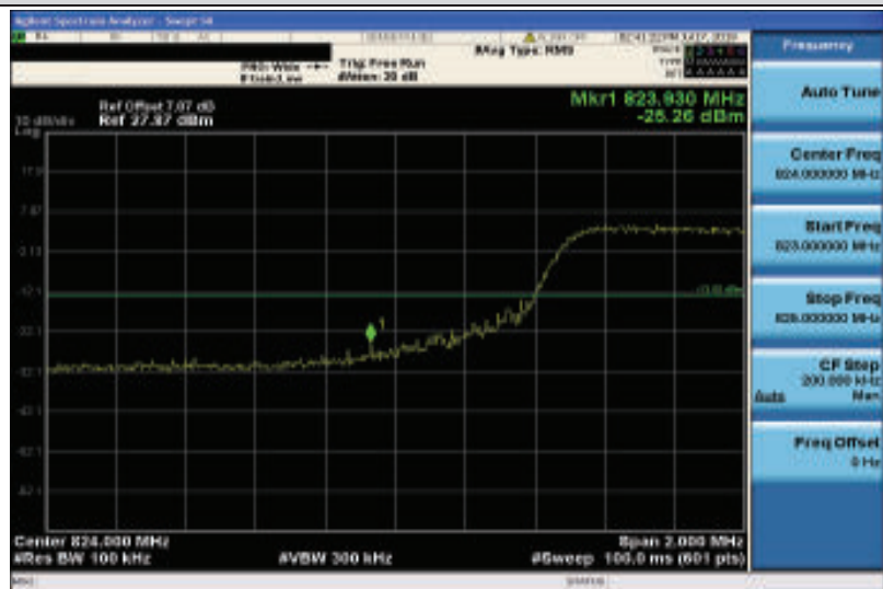
Band26-10MHz-QPSK-26840-50RB#0
