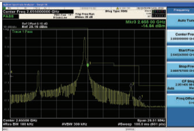
Band41-10MHz-QPSK-41190-1RB#49
