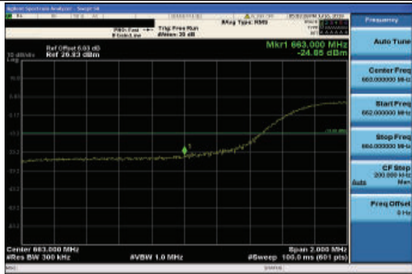
Band71-15MHz-16QAM-133197-75RB#0
