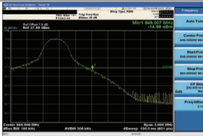
Band26-5MHz-QPSK-27015-1RB#24
