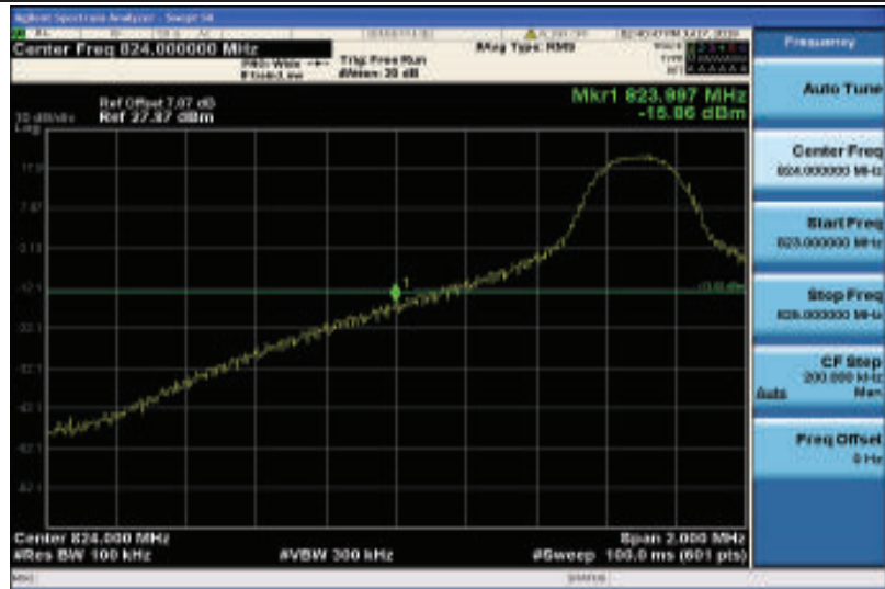
Band26-10MHz-QPSK-26840-1RB#0
