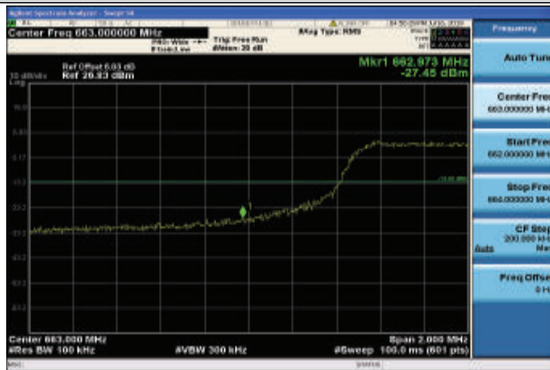
Band71-10MHz-16QAM-133172-50RB#0
