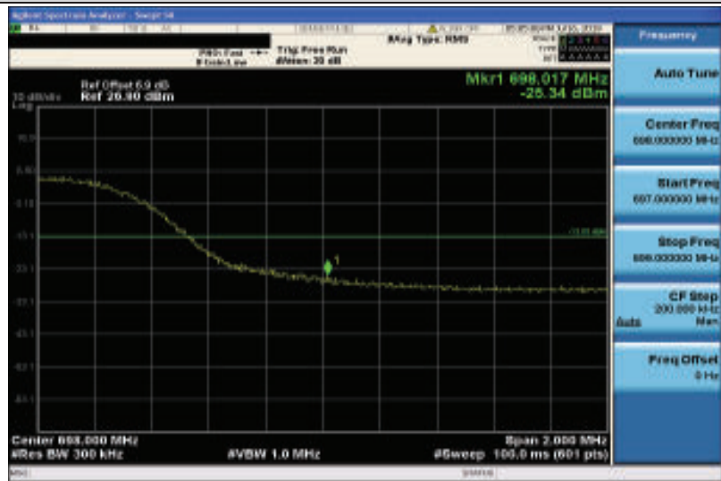
Band71-15MHz-16QAM-133397-75RB#0
