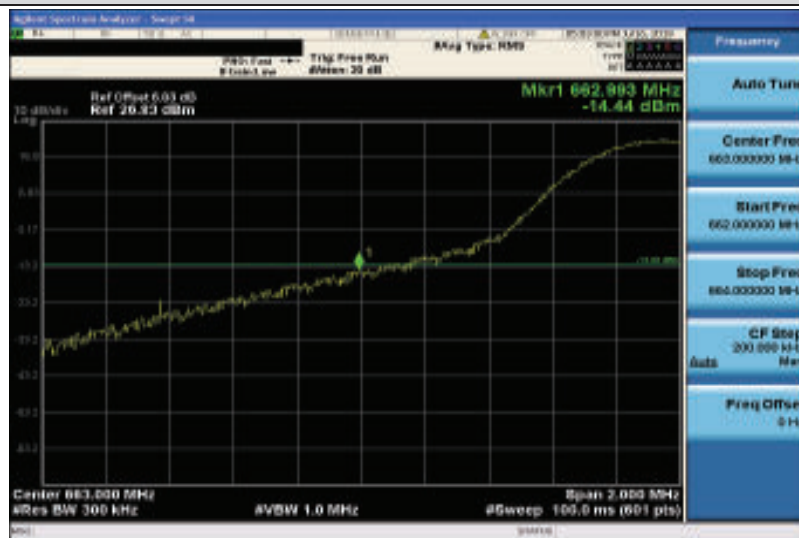
Band71-15MHz-16QAM-133197-1RB#0
