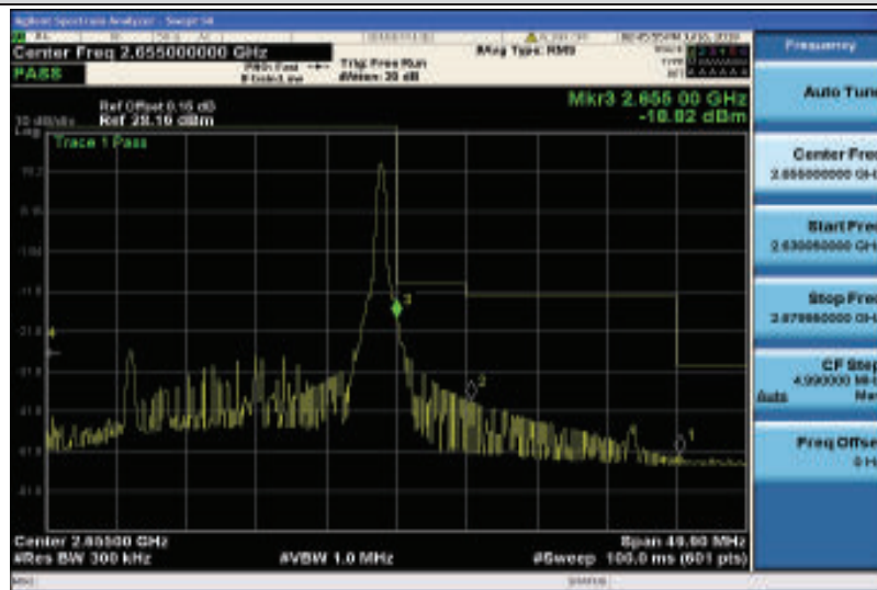
Band41-20MHz-16QAM-41140-1RB#99
