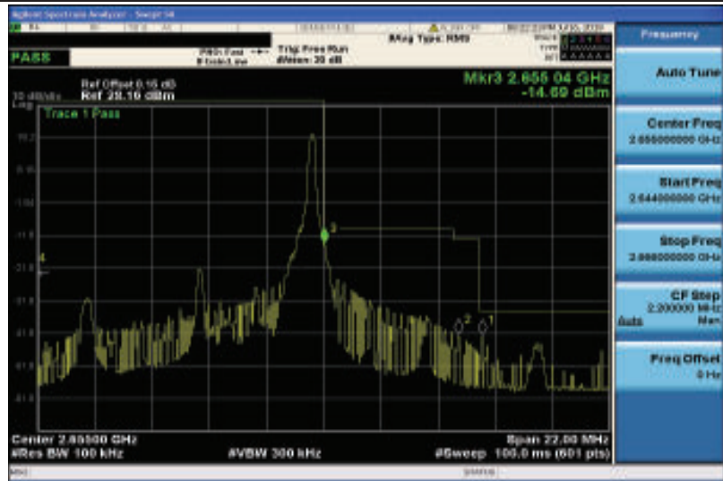
Band41-5MHz-16QAM-41215-1RB#24
