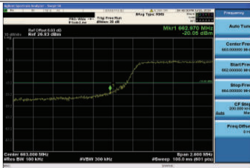
Band71-5MHz-16QAM-133147-25RB#0
