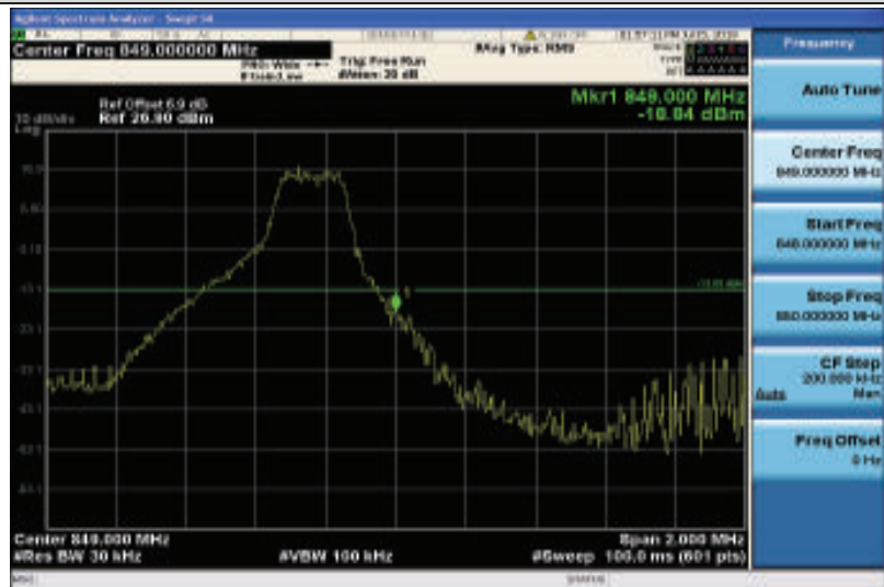
Band5-3MHz-16QAM-20635-1RB#14
