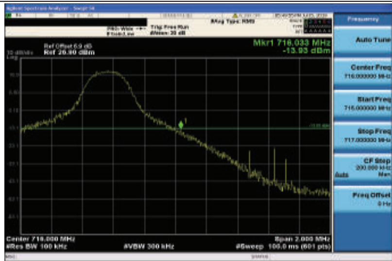
Band12-5MHz-16QAM-23155-1RB#24
