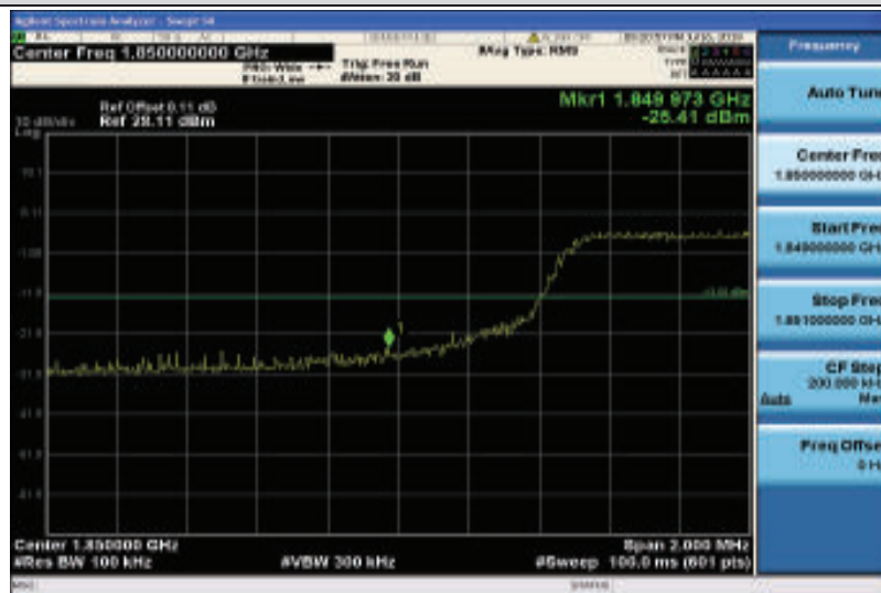
Band25-10MHz-QPSK-26090-50RB#0
