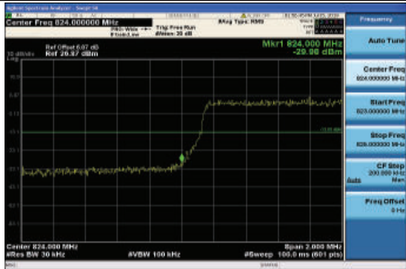
Band5-3MHz-16QAM-20415-15RB#0
