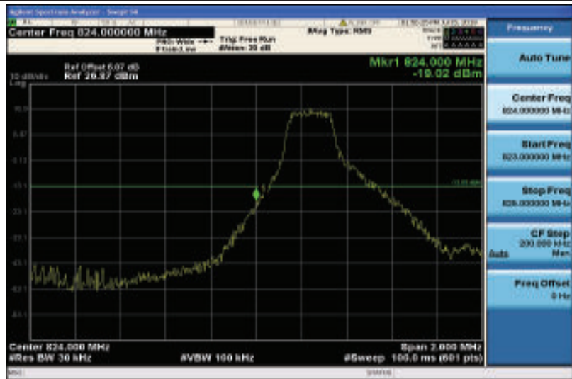
Band5-3MHz-16QAM-20415-1RB#0
