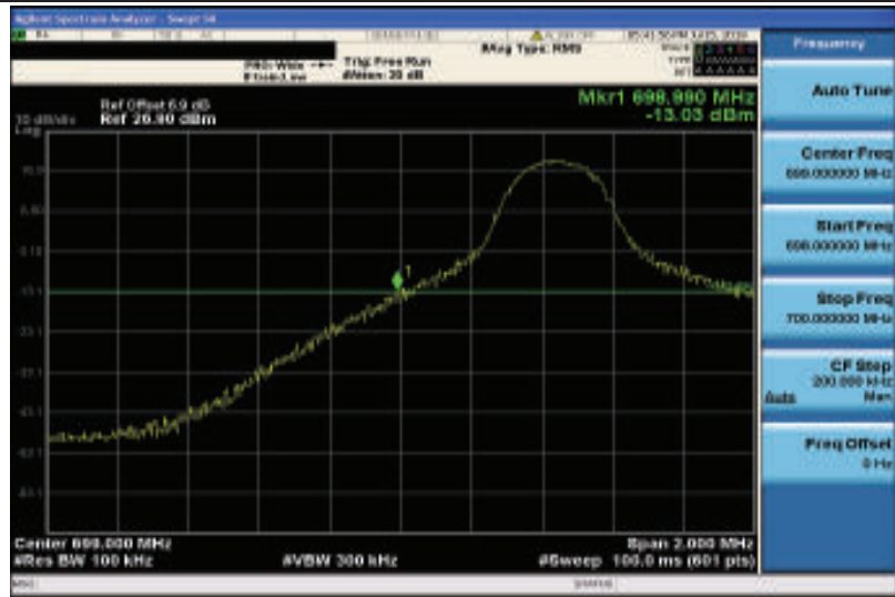
Band12-5MHz-16QAM-23035-1RB#0
