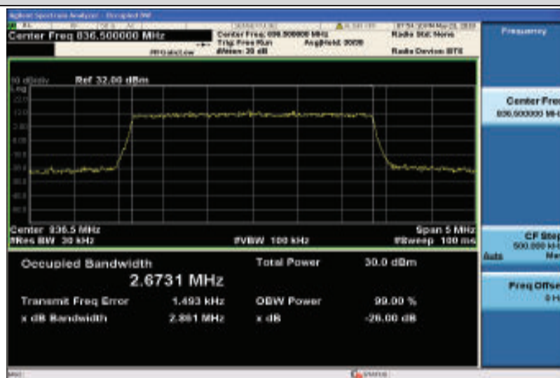
Band5-3MHz-16QAM-20525-15RB#0-2.6731
