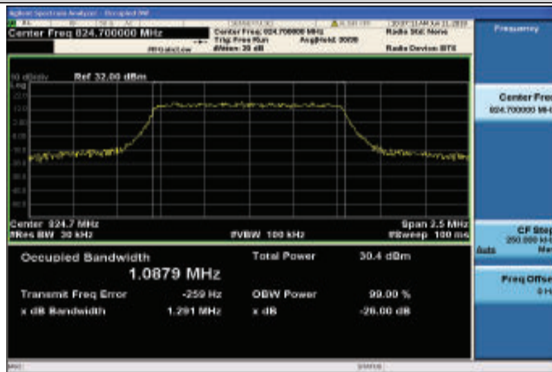
Band5-1.4MHz-QPSK-20407-6RB#0-1.0879
