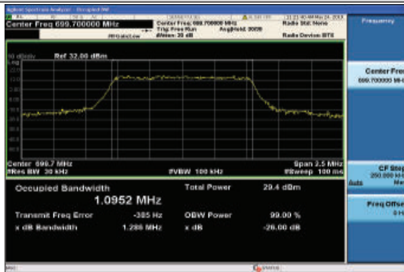
Band12-1.4MHz-16QAM-23017-6RB#0-1.0952
