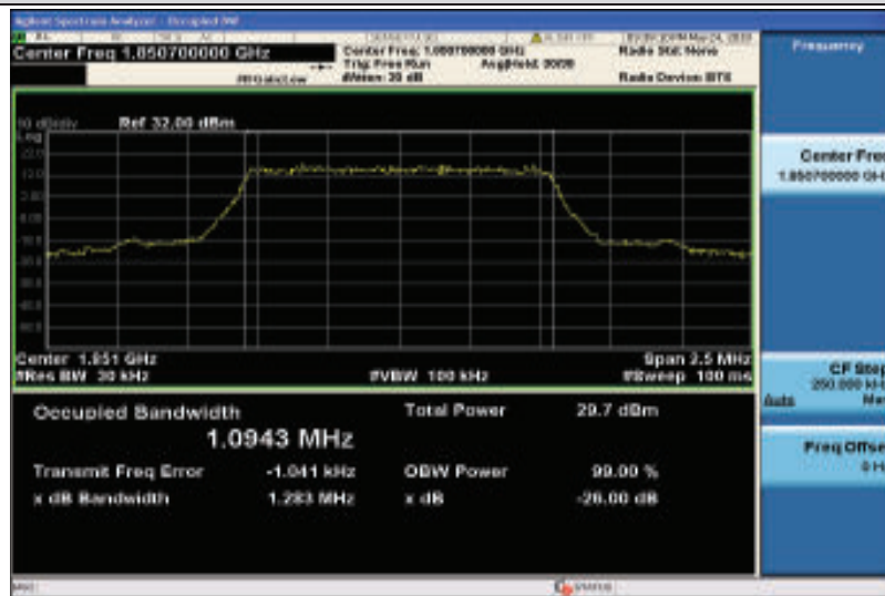
Band25-1.4MHz-QPSK-26047-6RB#0-1.0943
