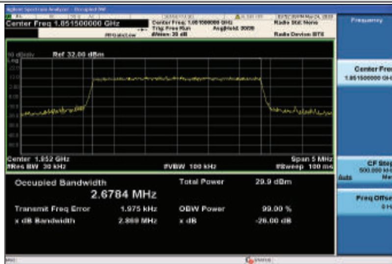
Band25-3MHz-QPSK-26055-15RB#0-2.6784
