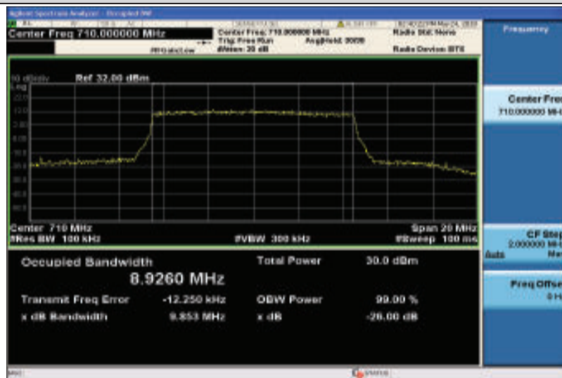
Band17-10MHz-16QAM-23790-50RB#0-8.9260
