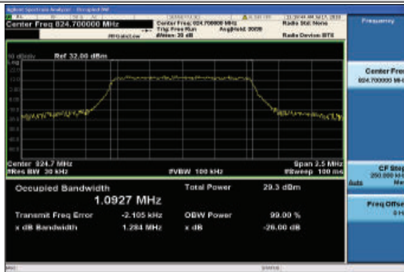
Band26-1.4MHz-QPSK-26797-6RB#0-1.0927
