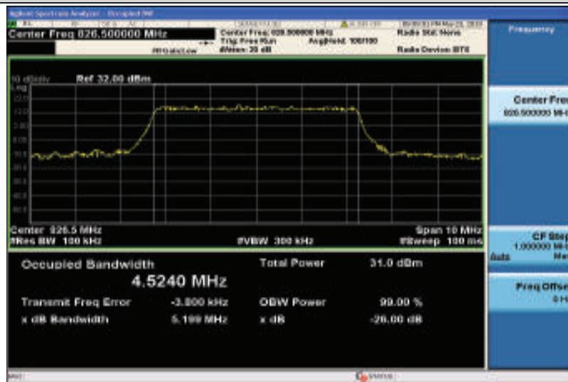
Band5-5MHz-16QAM-20425-25RB#0-4.5240
