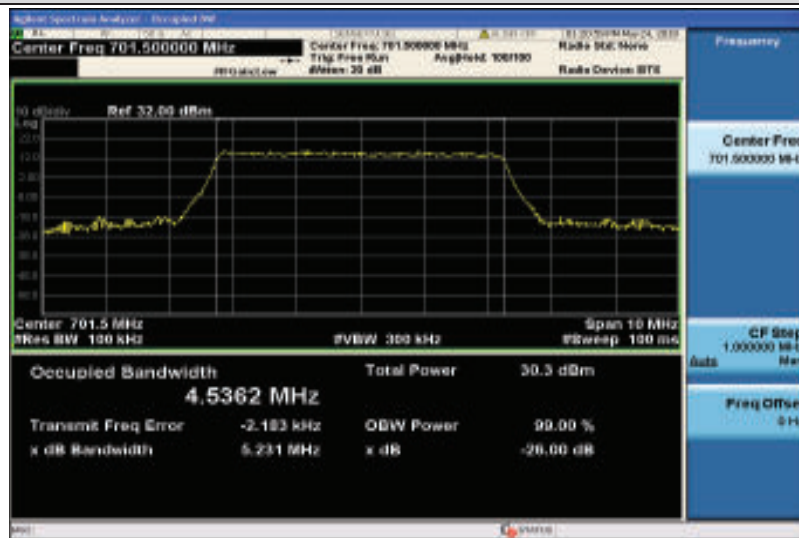
Band12-5MHz-16QAM-23035-25RB#0-4.5362
