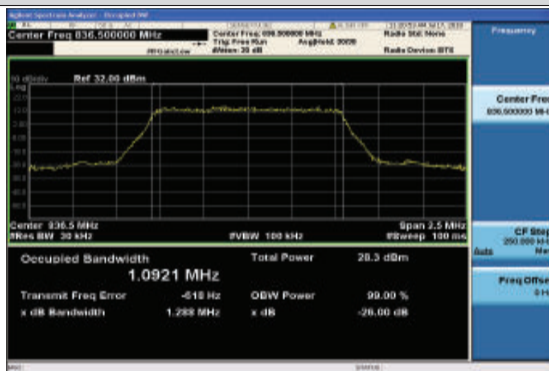
Band26-1.4MHz-16QAM-26915-6RB#0-1.0921
