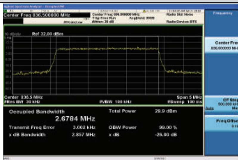
Band26-3MHz-QPSK-26915-15RB#0-2.6784
