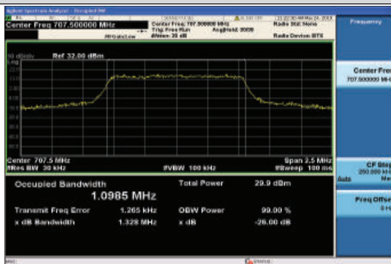
Band12-1.4MHz-16QAM-23095-6RB#0-1.0985
