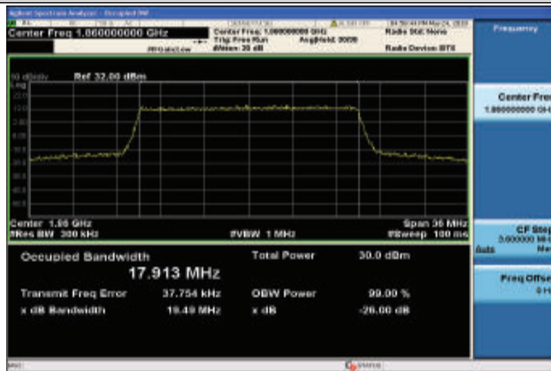
Band25-20MHz-16QAM-26140-100RB#0-17.913
