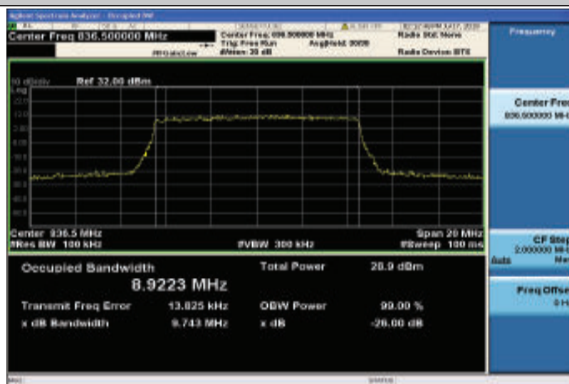
Band26-10MHz-16QAM-26915-50RB#0-8.9223
