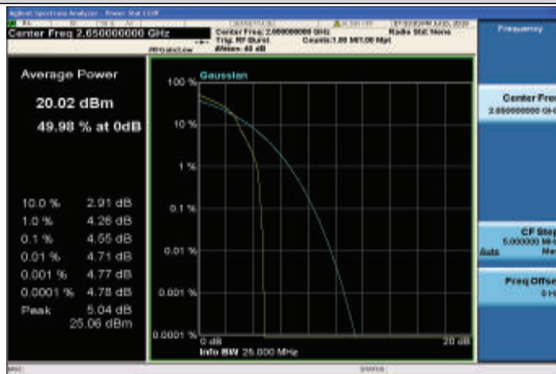
Band41-10MHz-16QAM-41190-1RB#0
