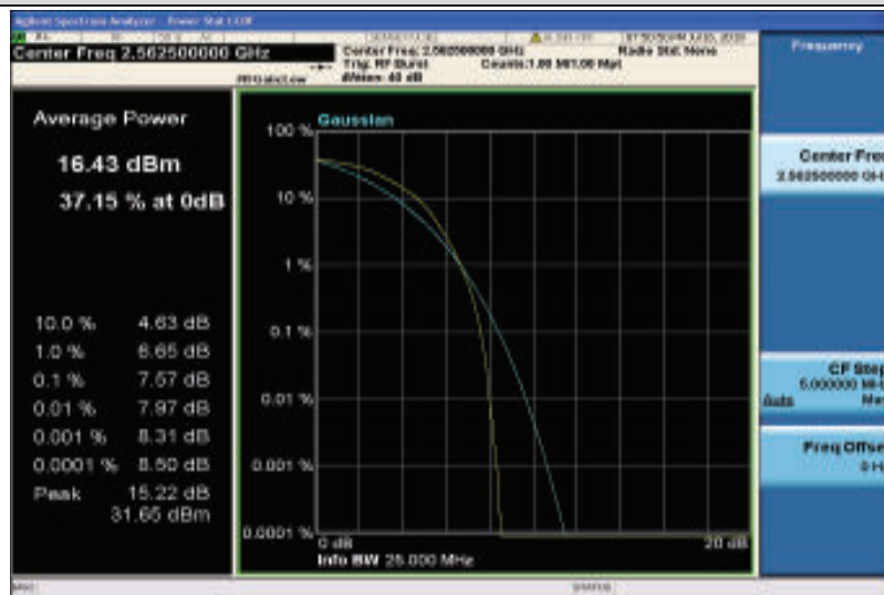
Band41-15MHz-16QAM-40315-75RB#0
