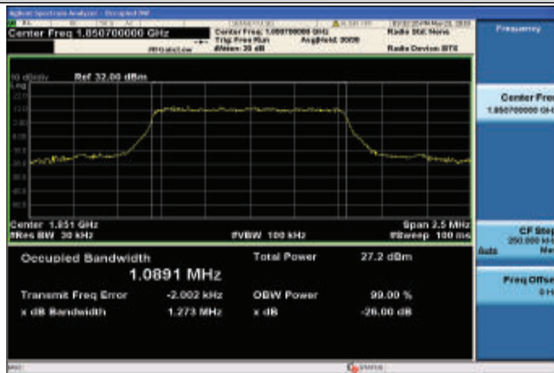
Band2-1.4MHz-16QAM-18607-6RB#0-1.0891
