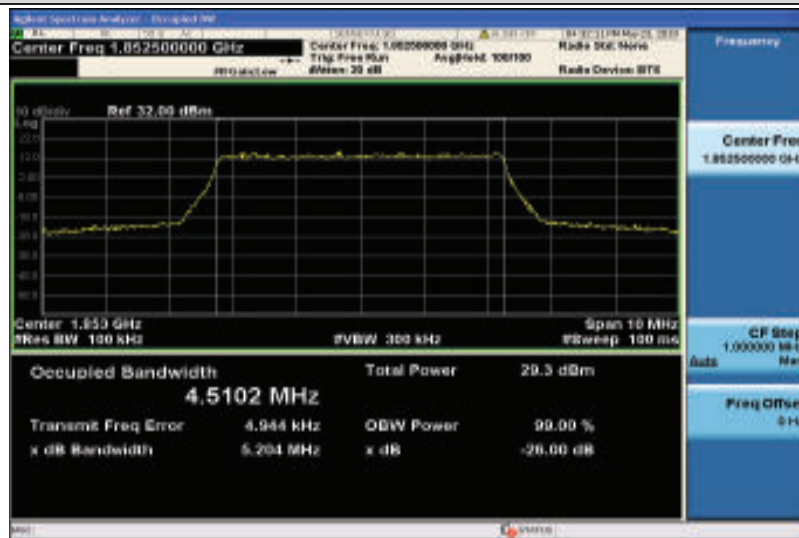
Band2-5MHz-QPSK-18625-25RB#0-4.5102
