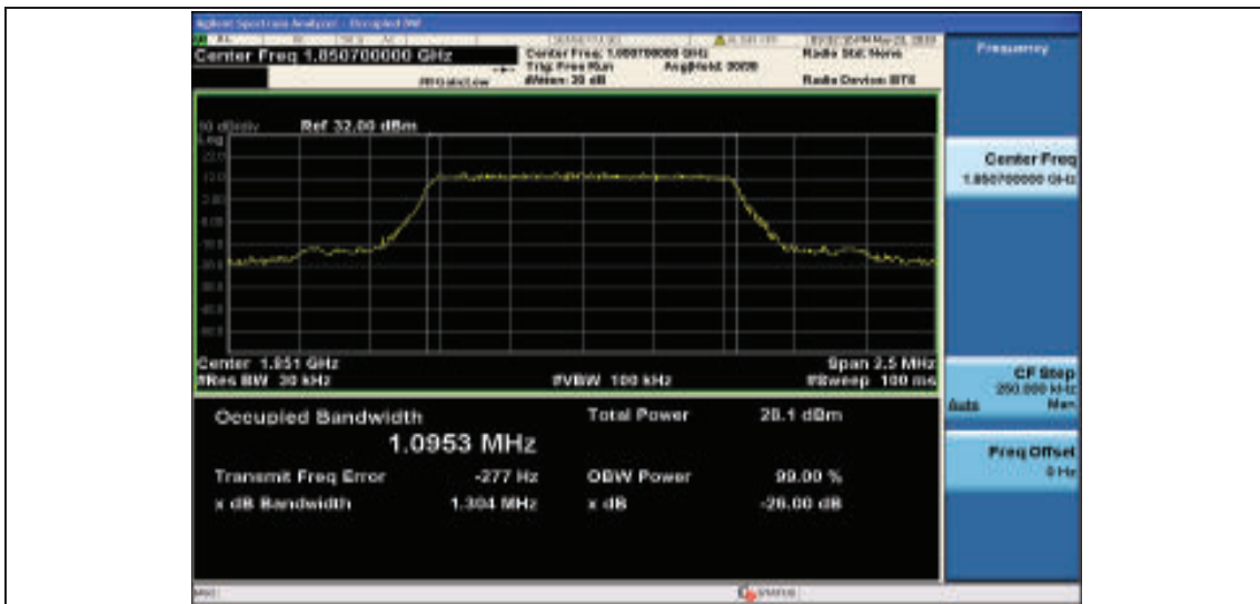
Band2-1.4MHz-QPSK-18607-6RB#0-1.0953
