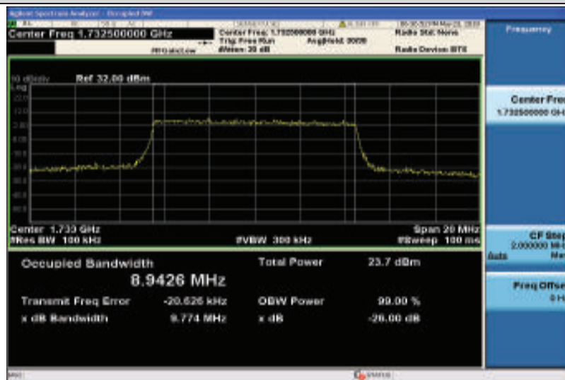
Band4-10MHz-QPSK-20175-50RB#0-8.9426
