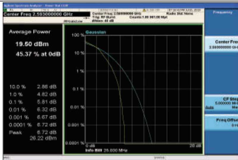
Band41-5MHz-16QAM-40620-25RB#0
