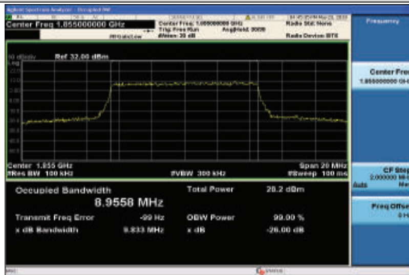
Band2-10MHz-16QAM-18650-50RB#0-8.9558
