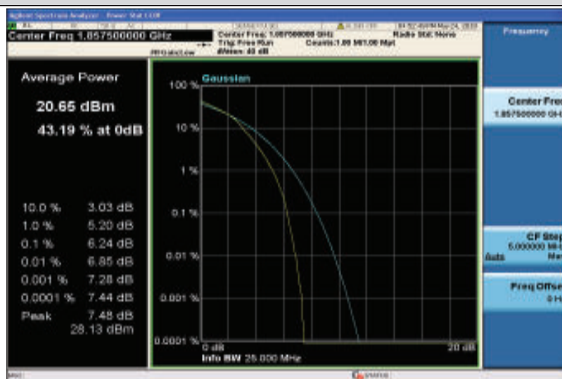
Band25-15MHz-16QAM-26115-75RB#0
