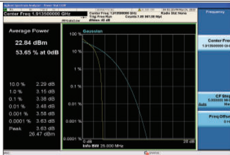
Band25-3MHz-QPSK-26675-1RB#0
