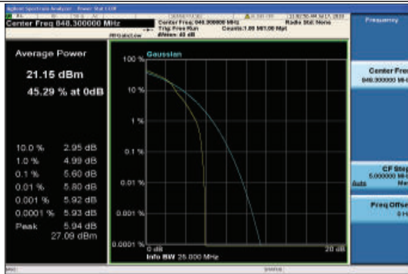
Band26-1.4MHz-16QAM-27033-1RB#0
