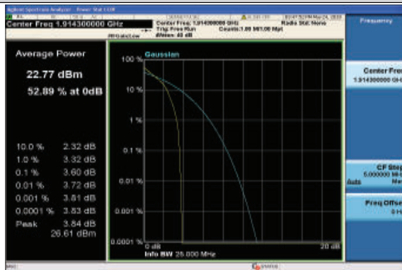
Band25-1.4MHz-QPSK-26683-1RB#0
