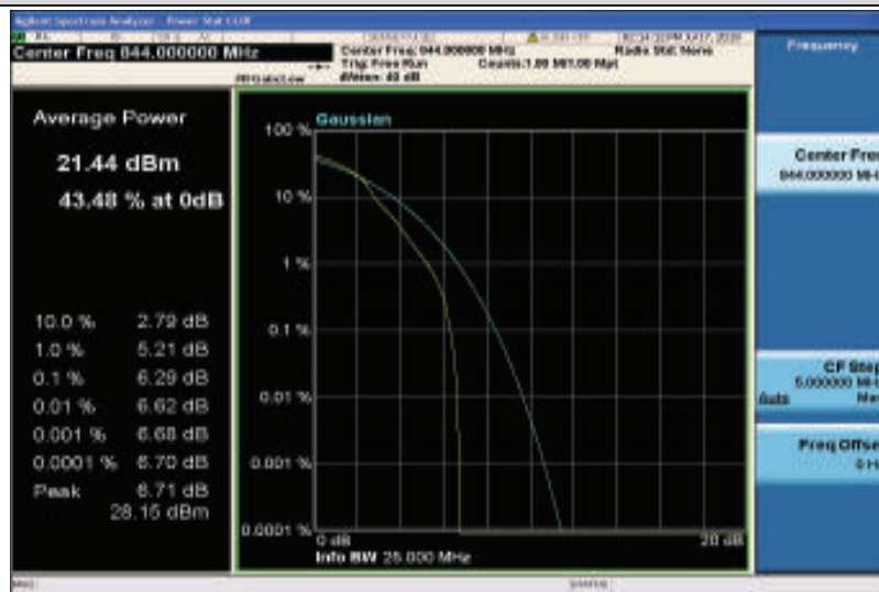
Band26-10MHz-16QAM-26990-1RB#0
