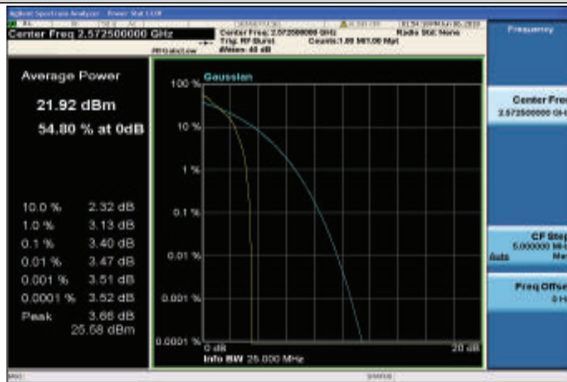
Band38-5MHz-QPSK-37775-1RB#0
