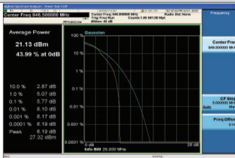
Band26-5MHz-16QAM-27015-1RB#0
