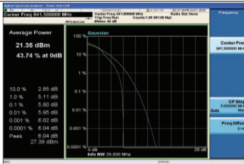
Band26-15MHz-16QAM-26965-1RB#0
