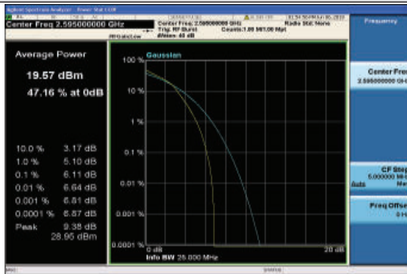
Band38-5MHz-16QAM-38000-25RB#0
