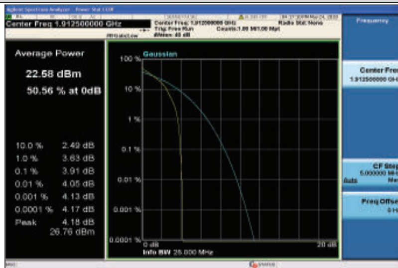
Band25-5MHz-QPSK-26665-1RB#0
