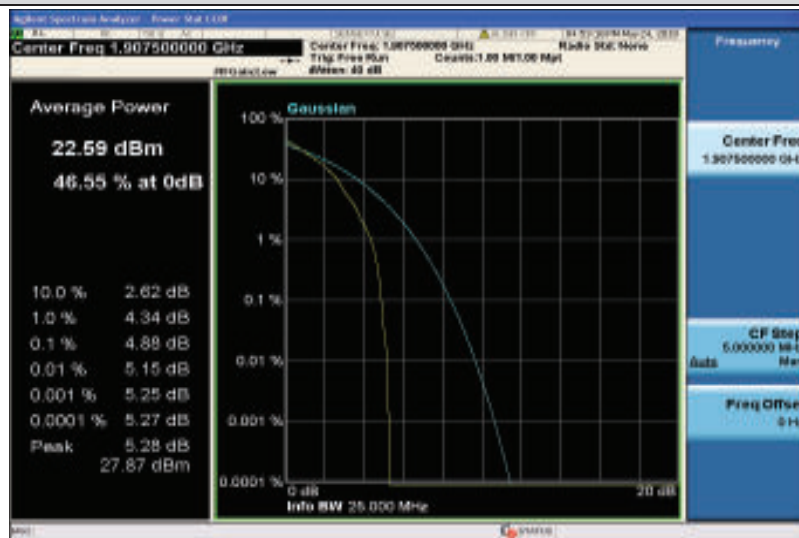
Band25-15MHz-QPSK-26615-1RB#0
