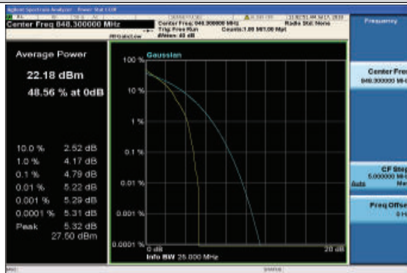
Band26-1.4MHz-QPSK-27033-1RB#0
