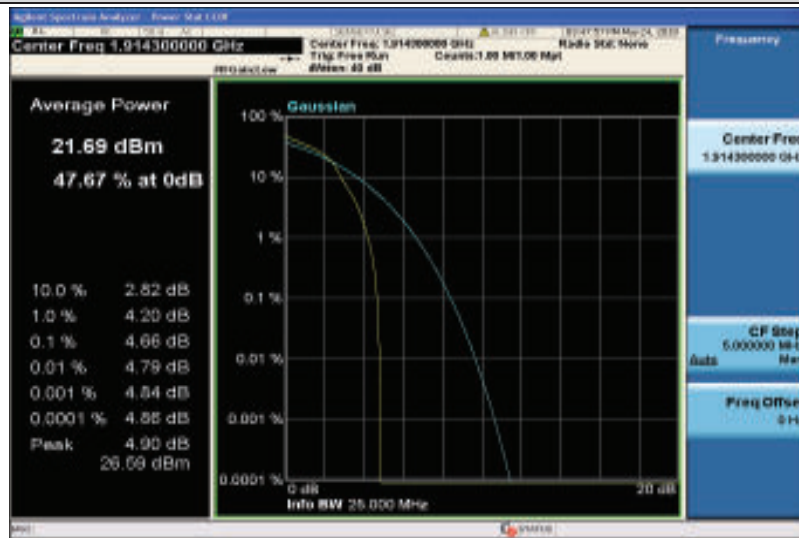
Band25-1.4MHz-16QAM-26683-1RB#0
