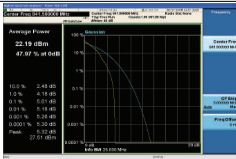
Band26-15MHz-QPSK-26965-1RB#0
