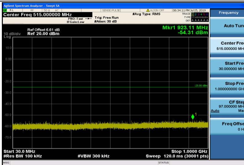
Band38-10MHz-16QAM-38000-1RB#0-Range1:30~1000MHz
