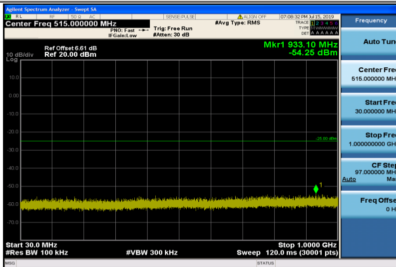
Band38-20MHz-QPSK-38000-1RB#0-Range1:30~1000MHz
