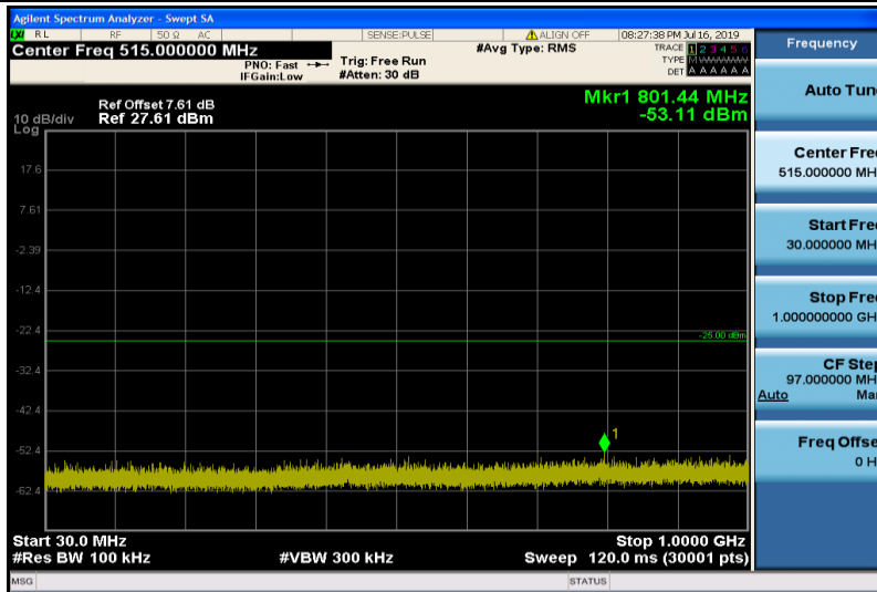
Band41-5MHz-16QAM-41215-1RB#0-30~1000MHz
