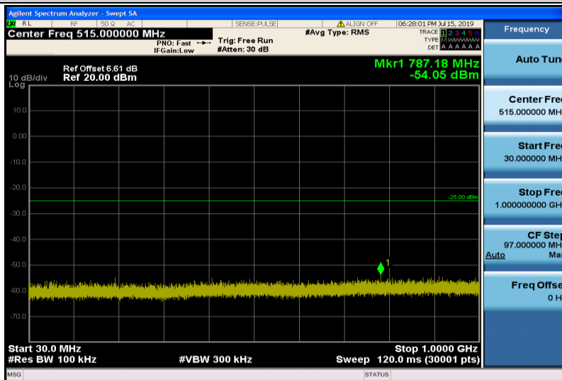
Band38-5MHz-16QAM-38000-1RB#0-Range1:30~1000MHz
