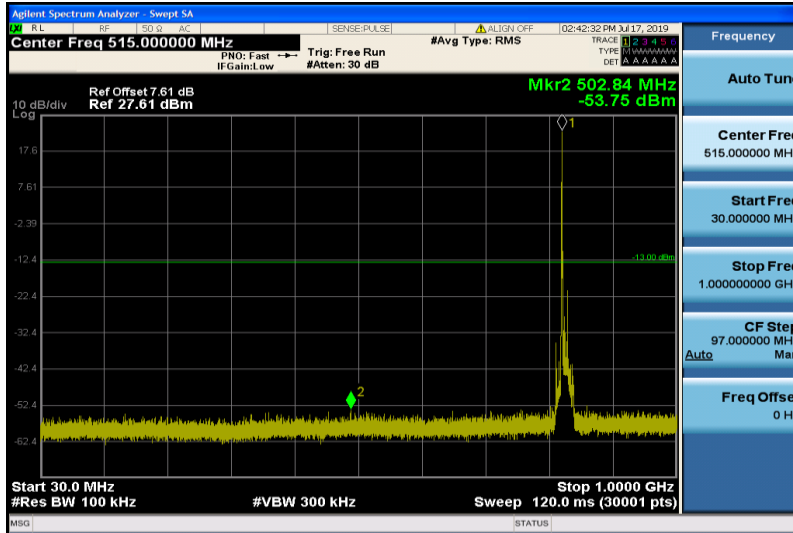
Band26-10MHz-QPSK-26840-1RB#0-30~1000MHz
