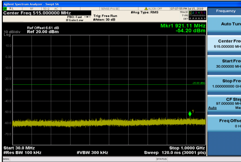
Band38-20MHz-16QAM-37850-1RB#0-Range1:30~1000MHz
