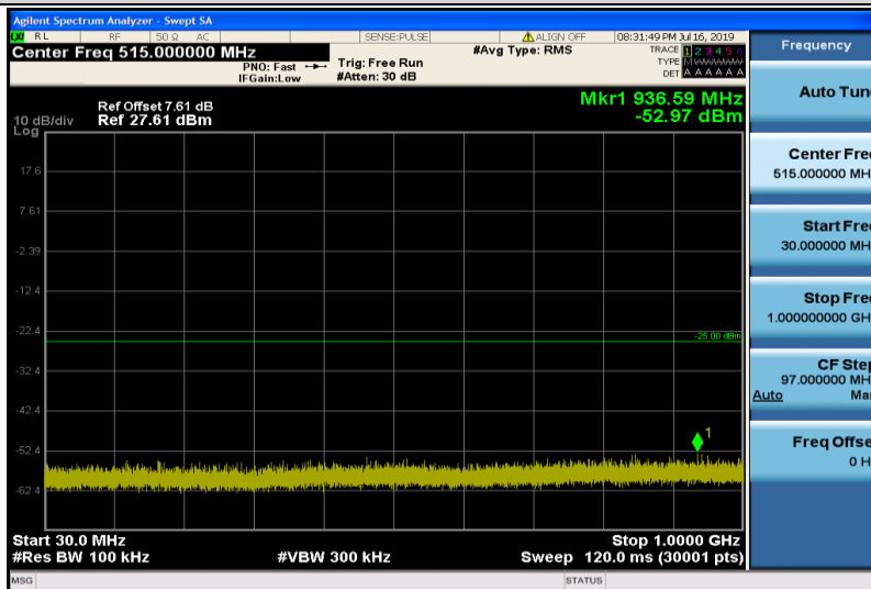
Band41-10MHz-QPSK-40620-1RB#0-30~1000MHz
