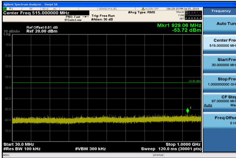
Band38-5MHz-16QAM-38225-1RB#0-Range1:30~1000MHz
