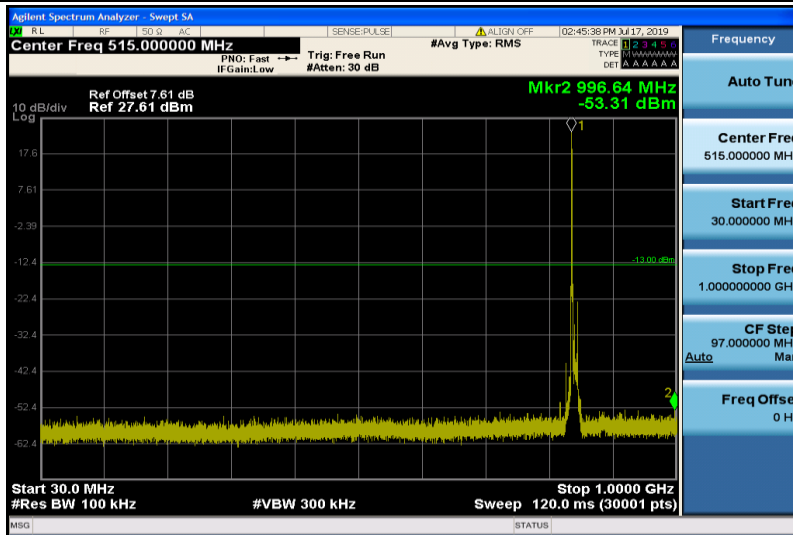
Band26-10MHz-16QAM-26990-1RB#0-30~1000MHz
