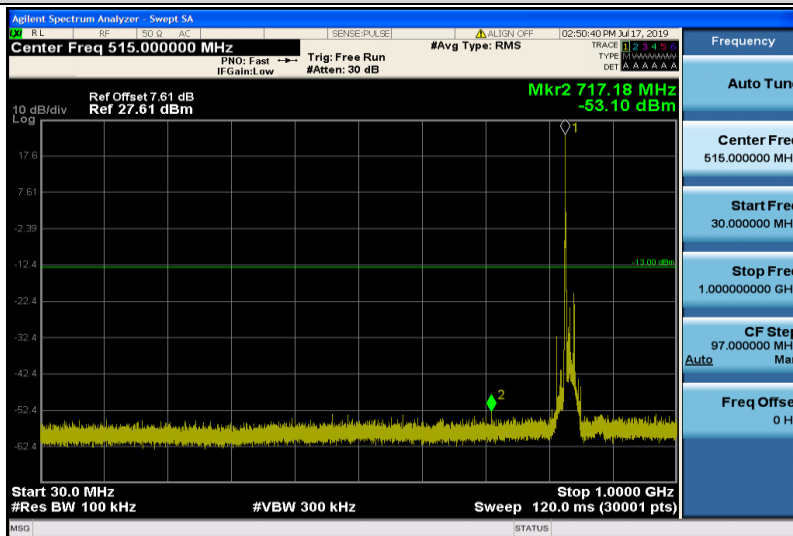
Band26-15MHz-QPSK-26915-1RB#0-30~1000MHz
