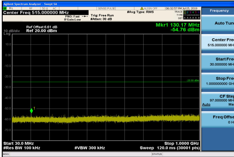
Band38-10MHz-16QAM-37800-1RB#0-Range1:30~1000MHz
