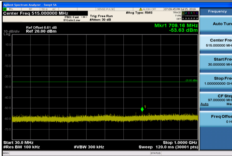
Band38-20MHz-QPSK-38150-1RB#0-Range1:30~1000MHz
