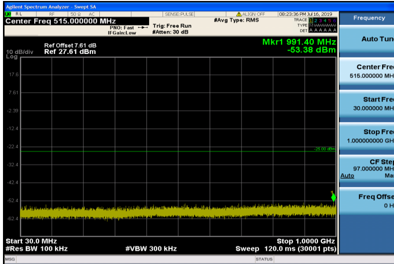
Band41-5MHz-16QAM-40265-1RB#0-30~1000MHz
