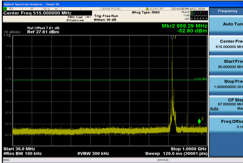
Band26-10MHz-16QAM-26840-1RB#0-30~1000MHz
