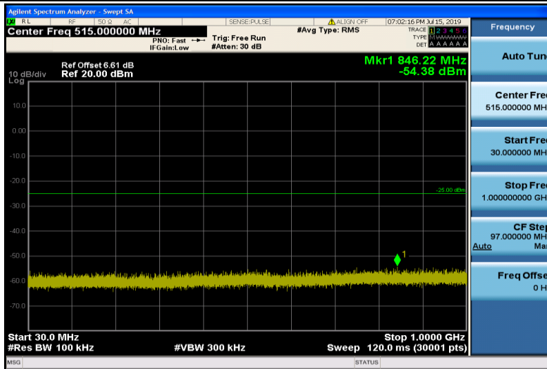
Band38-15MHz-QPSK-38175-1RB#0-Range1:30~1000MHz
