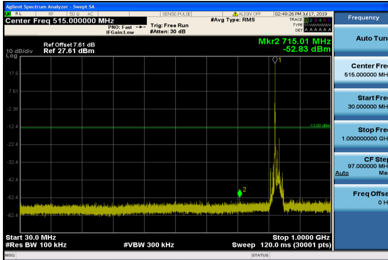
Band26-15MHz-QPSK-26915-1RB#0-30~1000MHz
