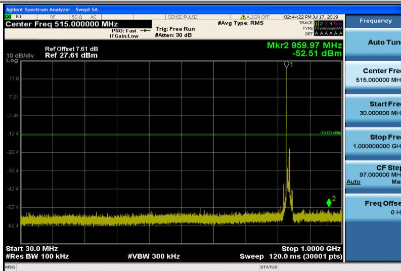
Band26-10MHz-16QAM-26915-1RB#0-30~1000MHz
