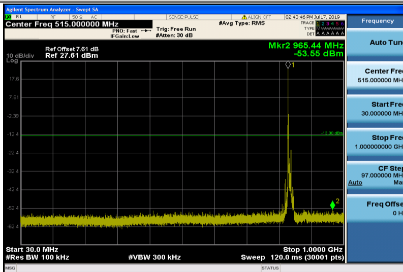
Band26-10MHz-QPSK-26915-1RB#0-30~1000MHz
