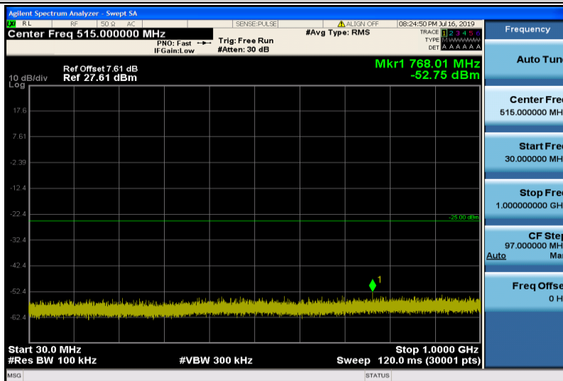
Band41-5MHz-16QAM-40620-1RB#0-30~1000MHz
