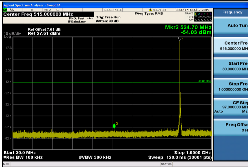
Band26-5MHz-16QAM-27015-1RB#0-30~1000MHz
