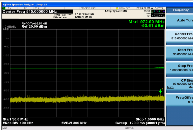
Band38-20MHz-16QAM-38000-1RB#0-Range1:30~1000MHz
