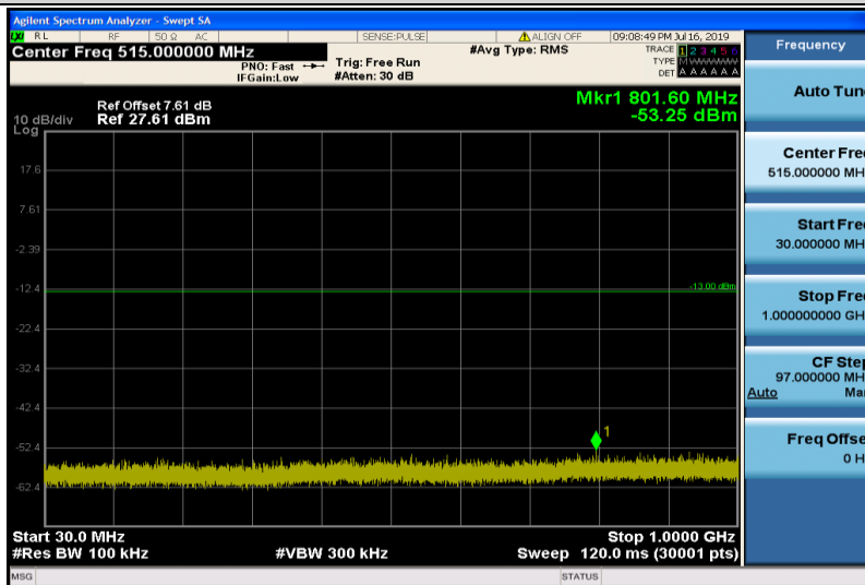
Band25-3MHz-16QAM-26365-1RB#0-30~1000MHz
