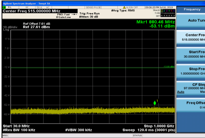
Band25-3MHz-QPSK-26055-1RB#0-30~1000MHz
