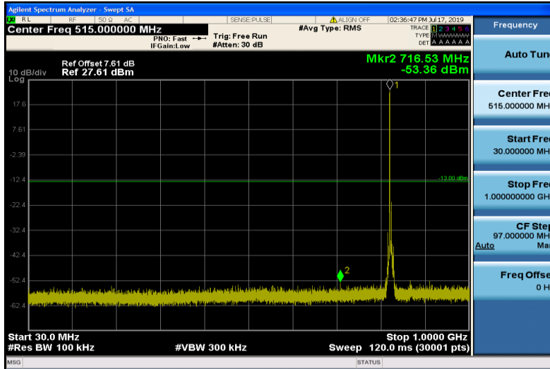
Band26-5MHz-16QAM-26815-1RB#0-30~1000MHz
