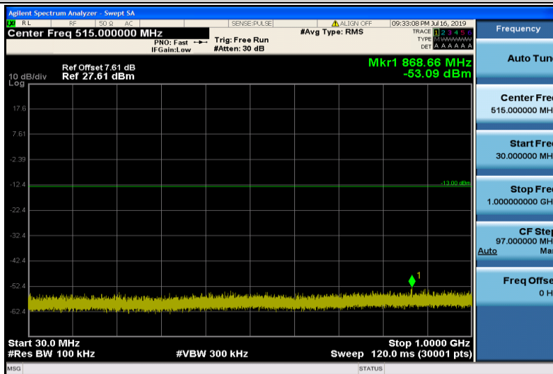
Band25-10MHz-16QAM-26365-1RB#0-30~1000MHz
