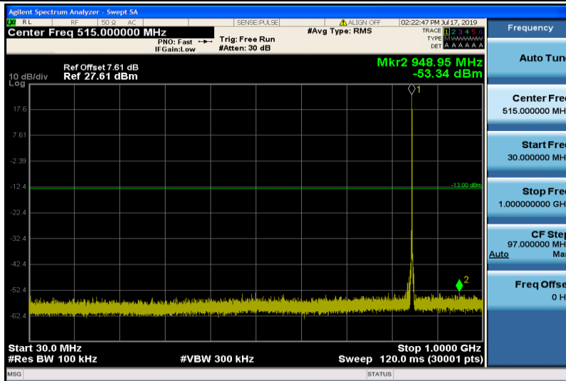
Band26-1.4MHz-16QAM-27033-1RB#0-30~1000MHz
