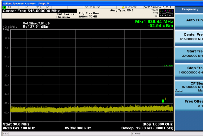
Band25-1.4MHz-16QAM-26047-1RB#0-30~1000MHz
