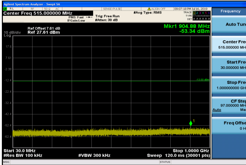
Band25-3MHz-16QAM-26055-1RB#0-30~1000MHz
