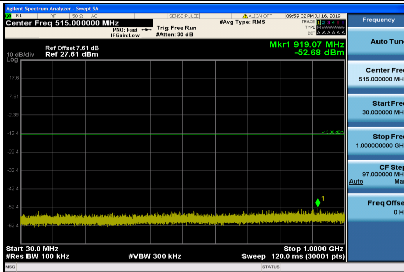
Band25-5MHz-16QAM-26665-1RB#0-30~1000MHz
