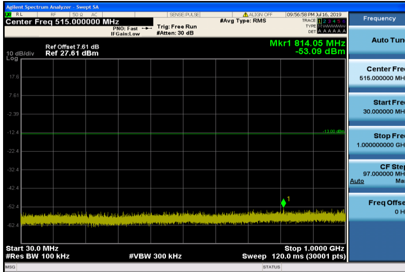
Band25-5MHz-16QAM-26065-1RB#0-30~1000MHz
