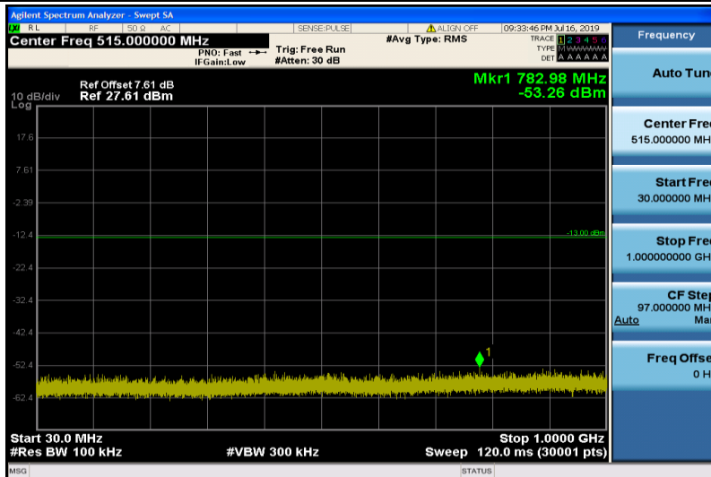
Band25-10MHz-QPSK-26640-1RB#0-30~1000MHz
