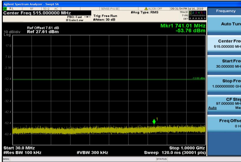
Band25-10MHz-16QAM-26090-1RB#0-30~1000MHz
