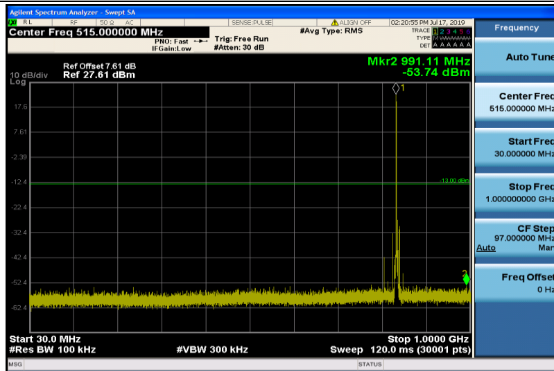
Band26-1.4MHz-QPSK-26915-1RB#0-30~1000MHz
