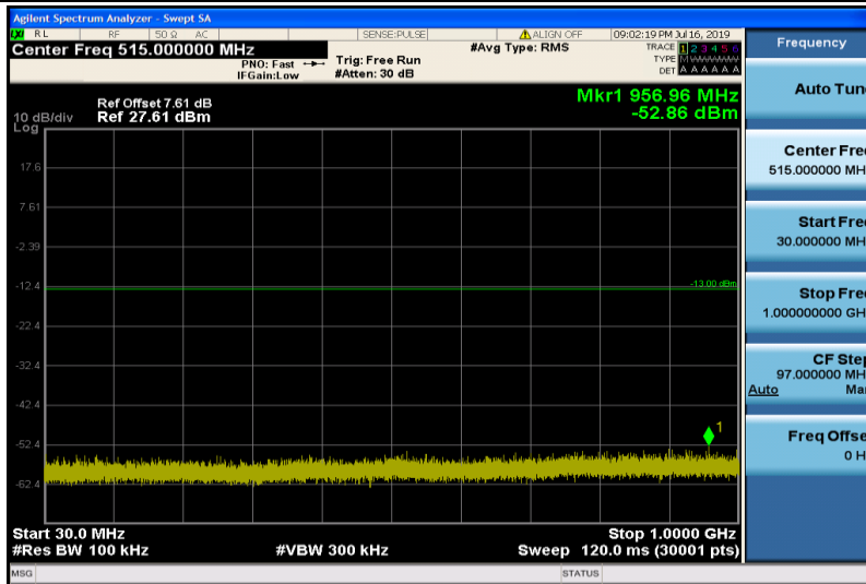
Band25-1.4MHz-QPSK-26683-1RB#0-30~1000MHz
