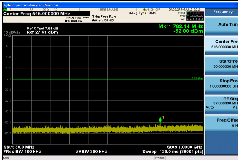
Band25-3MHz-QPSK-26675-1RB#0-30~1000MHz
