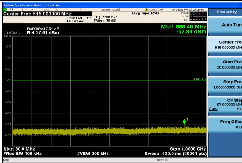
Band25-5MHz-QPSK-26665-1RB#0-30~1000MHz
