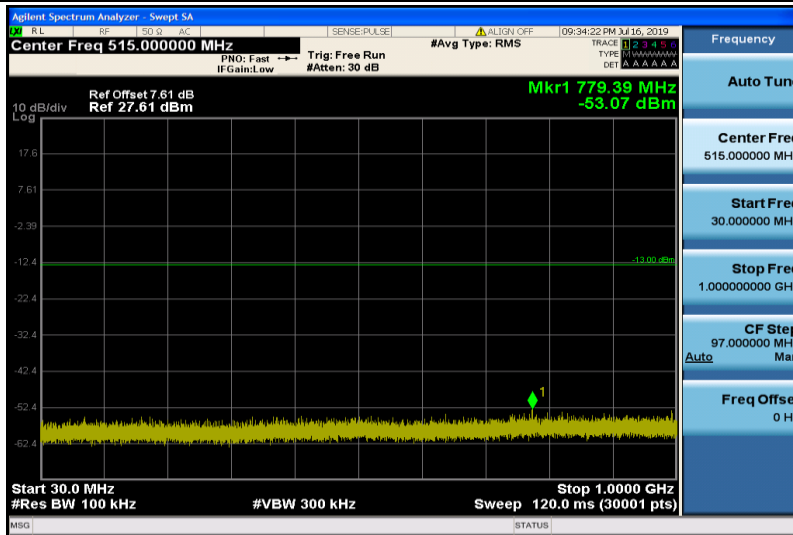
Band25-10MHz-16QAM-26640-1RB#0-30~1000MHz
