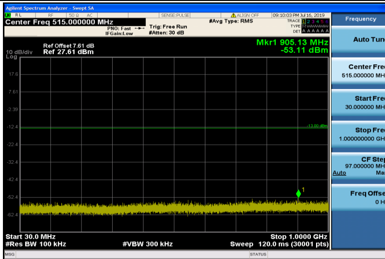
Band25-3MHz-16QAM-26675-1RB#0-30~1000MHz
