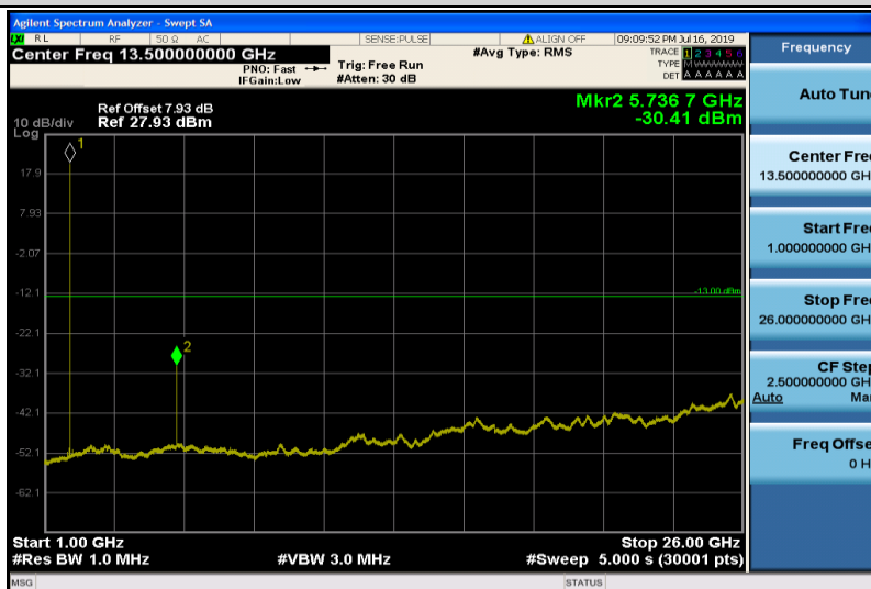
Band25-3MHz-QPSK-26675-1RB#0-1000~26000MHz
