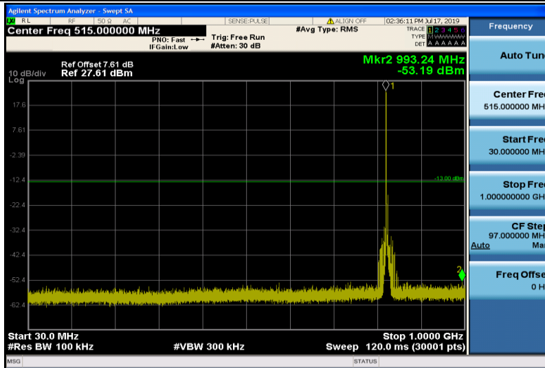
Band26-5MHz-QPSK-26815-1RB#0-30~1000MHz
