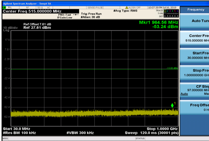
Band25-20MHz-16QAM-26140-1RB#0-30~1000MHz
