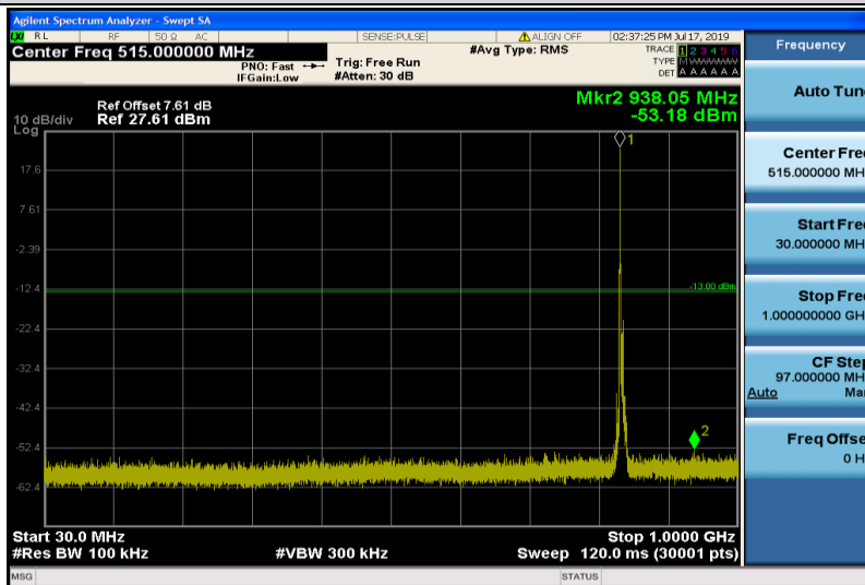
Band26-5MHz-QPSK-26915-1RB#0-30~1000MHz
