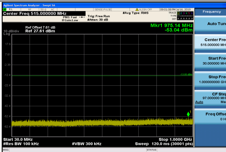
Band25-1.4MHz-16QAM-26365-1RB#0-30~1000MHz
