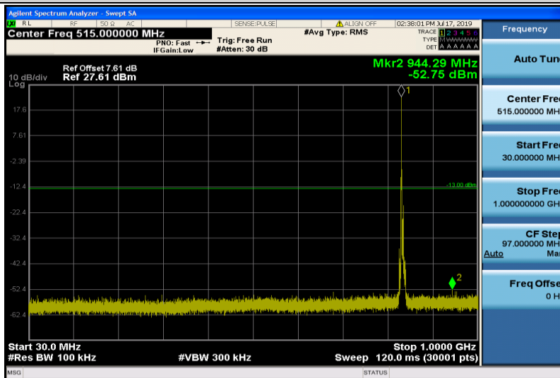
Band26-5MHz-16QAM-26915-1RB#0-30~1000MHz
