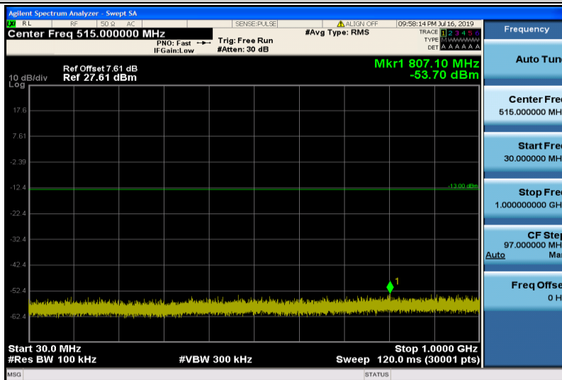
Band25-5MHz-16QAM-26365-1RB#0-30~1000MHz
