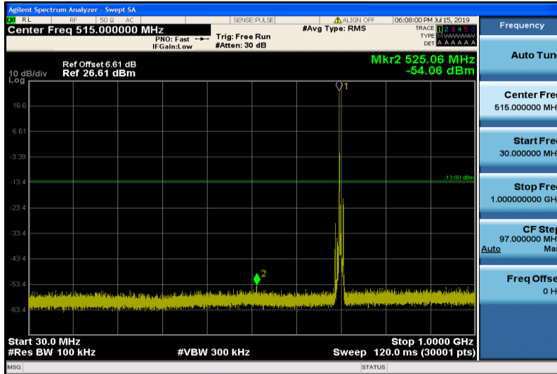
Band17-5MHz-16QAM-23755-1RB#0-Range1:30~1000MHz
