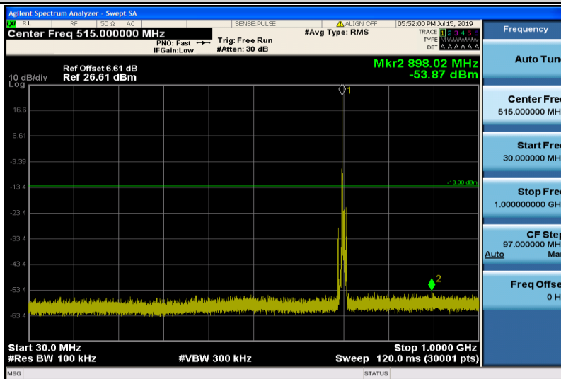
Band12-5MHz-QPSK-23095-1RB#0-Range1:30~1000MHz
