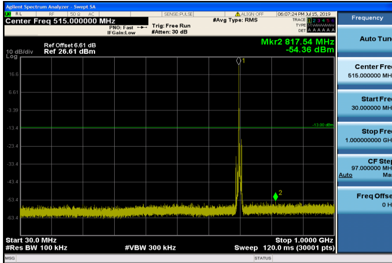
Band17-5MHz-QPSK-23755-1RB#0-Range1:30~1000MHz
