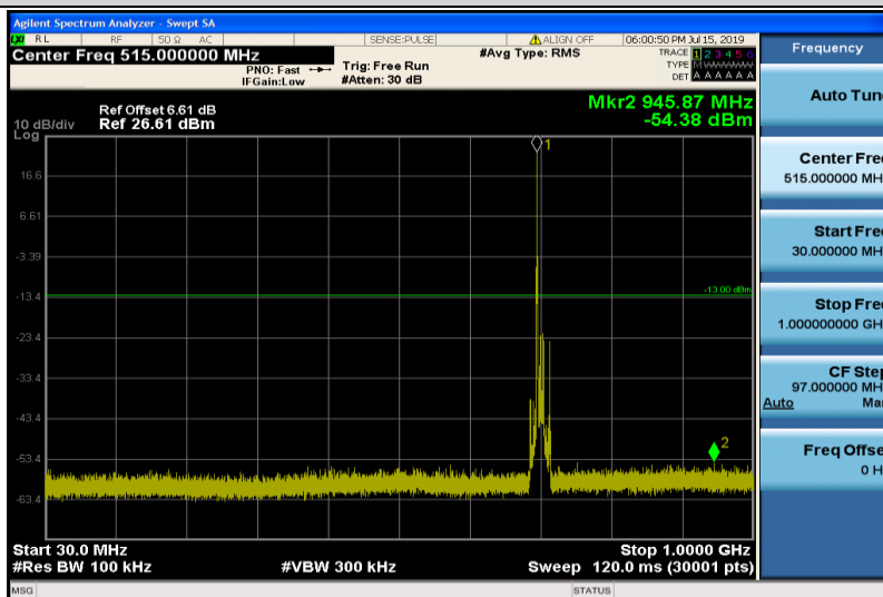
Band12-10MHz-16QAM-23095-1RB#0-Range1:30~1000MHz
