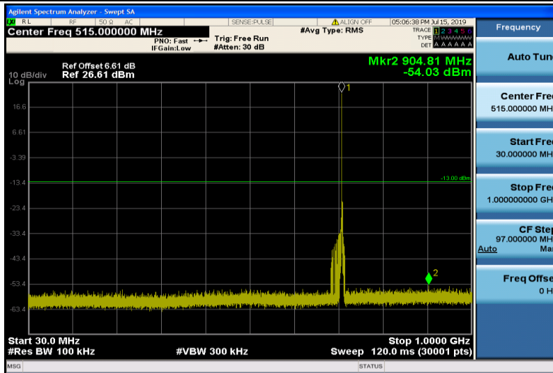
Band12-1.4MHz-16QAM-23173-1RB#0-Range1:30~1000MHz
