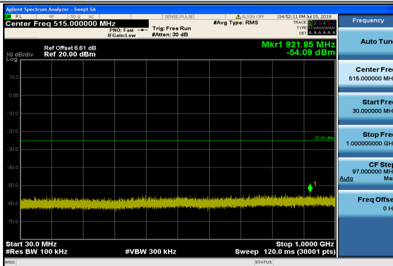
Band7-20MHz-16QAM-21100-1RB#0-Range1:30~1000MHz
