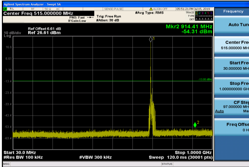
Band12-5MHz-16QAM-23035-1RB#0-Range1:30~1000MHz
