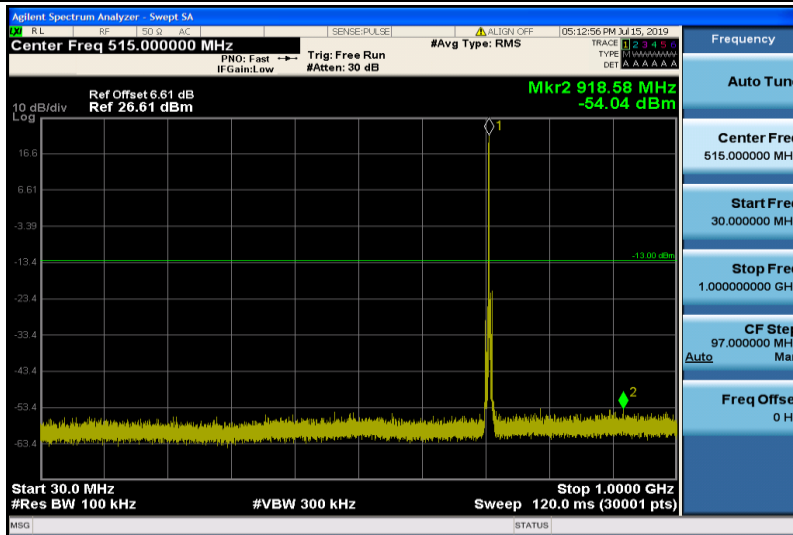
Band12-3MHz-16QAM-23165-1RB#0-Range1:30~1000MHz
