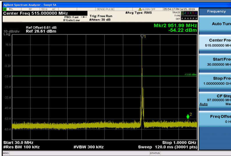
Band12-5MHz-16QAM-23155-1RB#0-Range1:30~1000MHz
