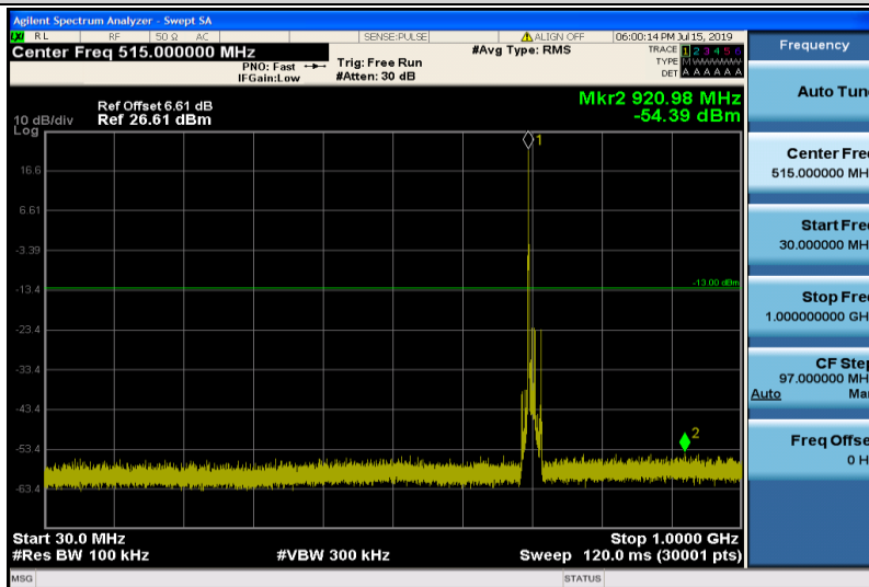
Band12-10MHz-QPSK-23095-1RB#0-Range1:30~1000MHz
