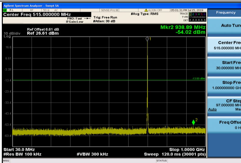
Band12-1.4MHz-QPSK-23095-1RB#0-Range1:30~1000MHz
