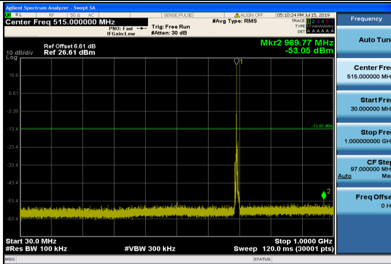
Band12-3MHz-16QAM-23025-1RB#0-Range1:30~1000MHz
