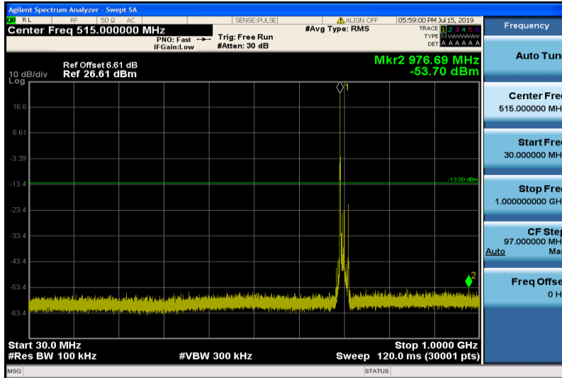
Band12-10MHz-QPSK-23060-1RB#0-Range1:30~1000MHz
