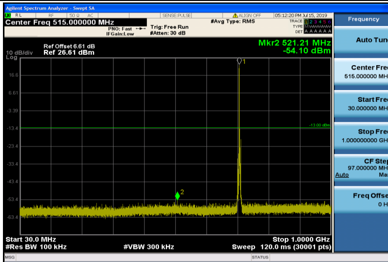
Band12-3MHz-QPSK-23165-1RB#0-Range1:30~1000MHz
