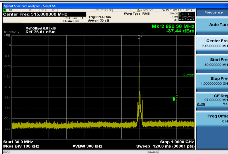
Band17-10MHz-16QAM-23790-1RB#0-Range1:30~1000MHz
