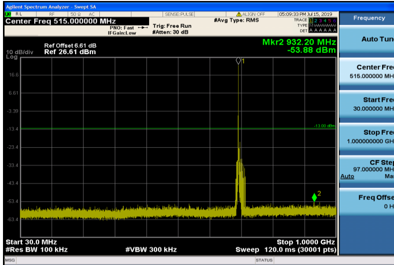
Band12-3MHz-QPSK-23025-1RB#0-Range1:30~1000MHz
