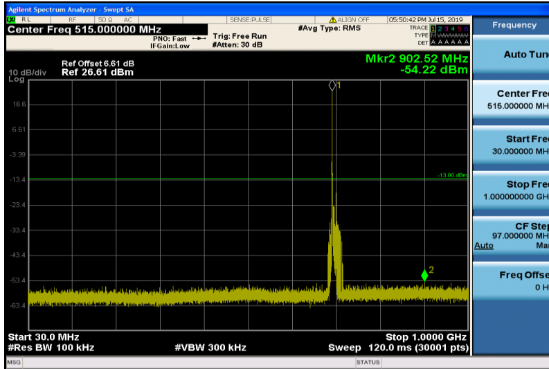
Band12-5MHz-QPSK-23035-1RB#0-Range1:30~1000MHz
