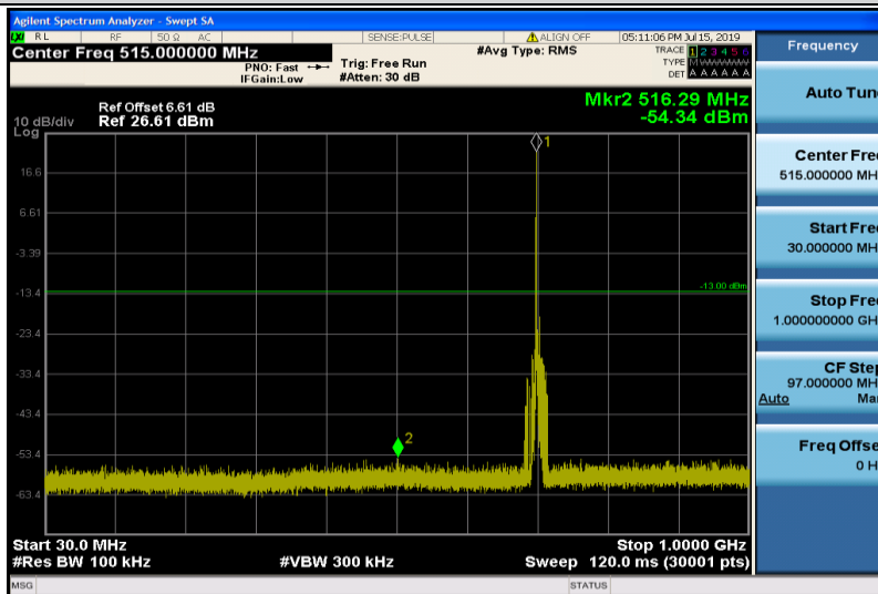
Band12-3MHz-QPSK-23095-1RB#0-Range1:30~1000MHz
