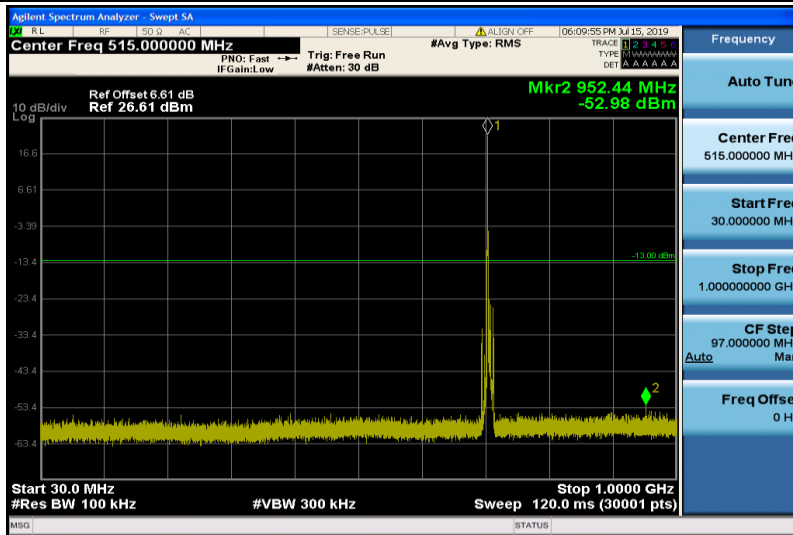
Band17-5MHz-QPSK-23825-1RB#0-Range1:30~1000MHz
