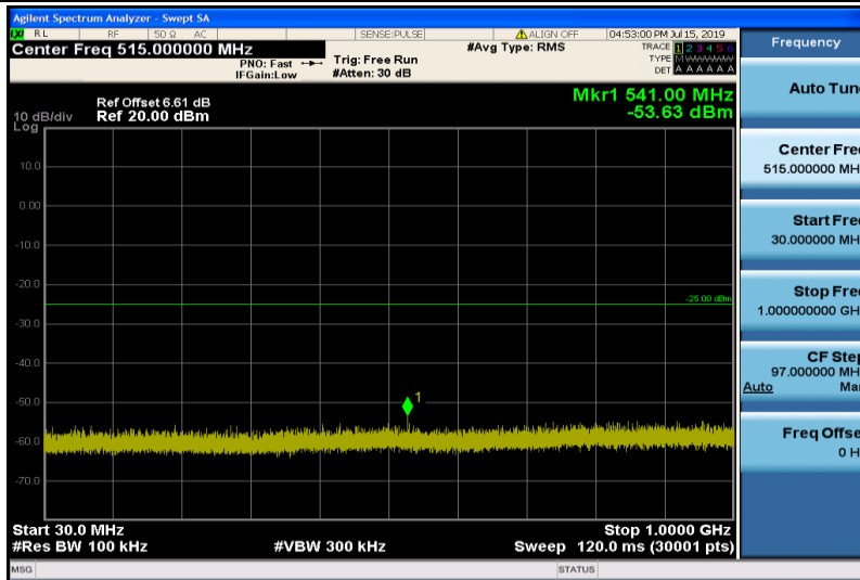
Band7-20MHz-QPSK-21350-1RB#0-Range1:30~1000MHz
