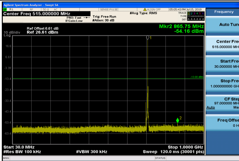
Band12-1.4MHz-QPSK-23173-1RB#0-Range1:30~1000MHz
