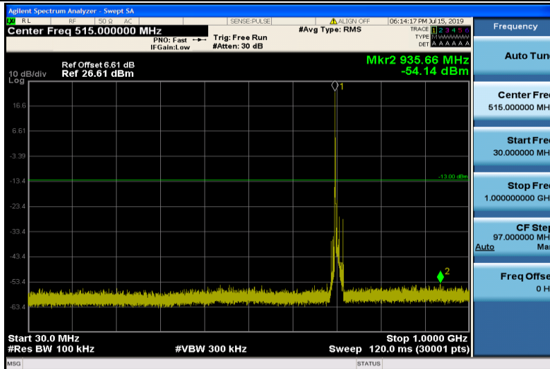
Band17-10MHz-16QAM-23780-1RB#0-Range1:30~1000MHz
