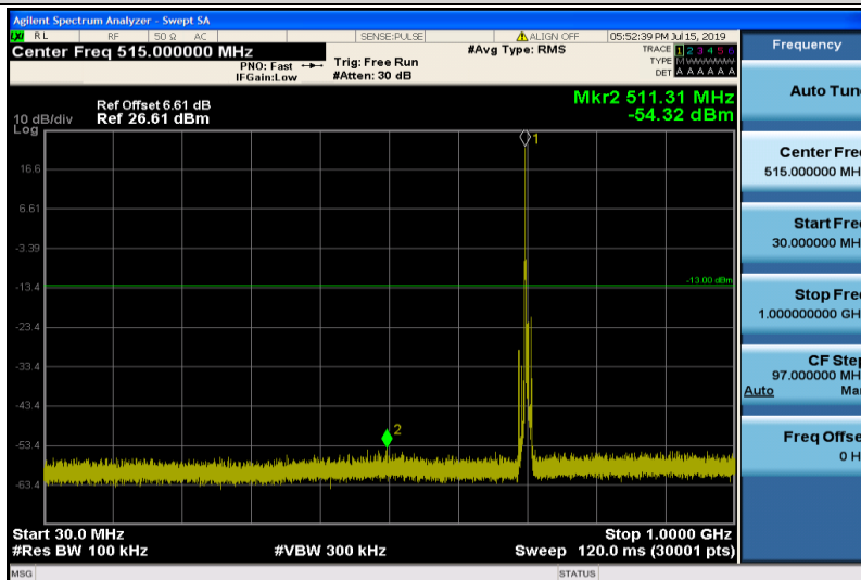
Band12-5MHz-16QAM-23095-1RB#0-Range1:30~1000MHz
