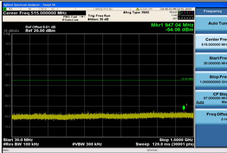
Band7-15MHz-16QAM-21375-1RB#0-Range1:30~1000MHz
