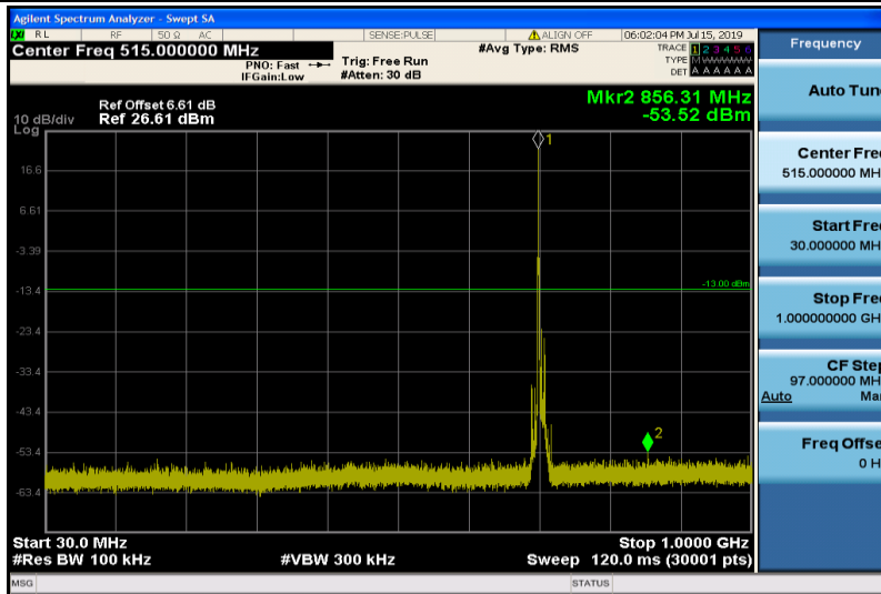
Band12-10MHz-16QAM-23130-1RB#0-Range1:30~1000MHz
