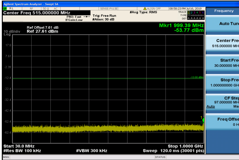
Band25-1.4MHz-QPSK-26047-1RB#0-30~1000MHz
