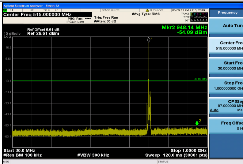
Band17-5MHz-16QAM-23790-1RB#0-Range1:30~1000MHz
