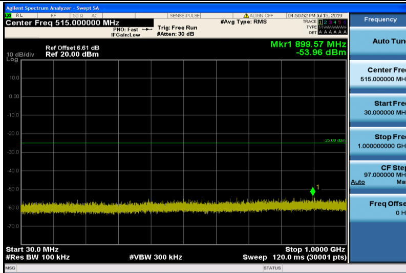
Band7-20MHz-16QAM-20850-1RB#0-Range1:30~1000MHz
