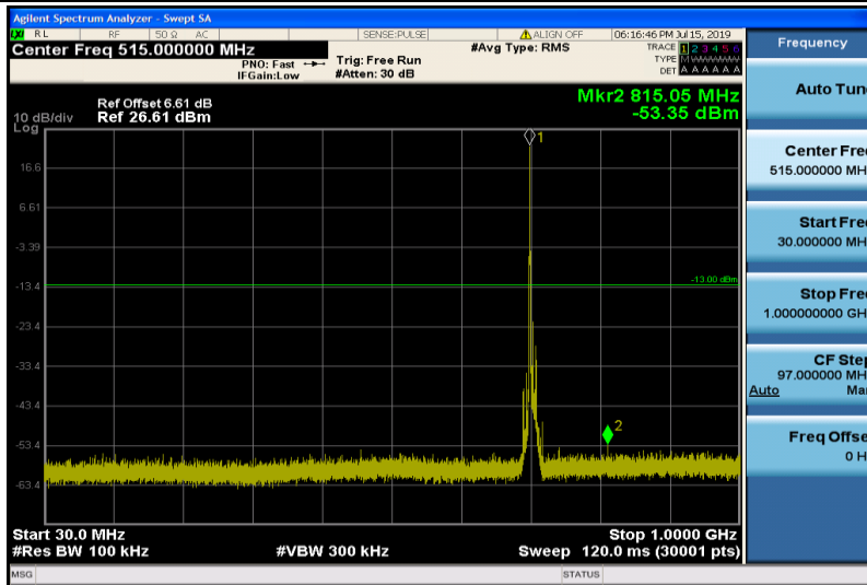
Band17-10MHz-16QAM-23800-1RB#0-Range1:30~1000MHz
