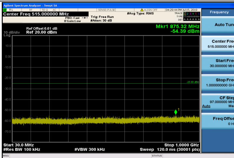
Band7-5MHz-16QAM-21100-1RB#0-Range1:30~1000MHz
