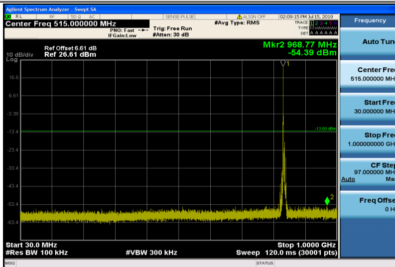
Band5-5MHz-QPSK-20525-1RB#0-Range1:30~1000MHz
