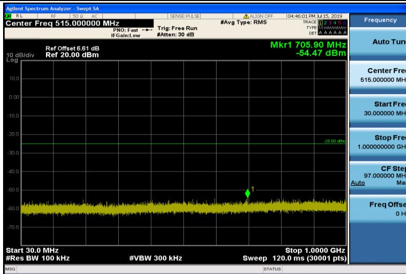
Band7-15MHz-QPSK-21375-1RB#0-Range1:30~1000MHz
