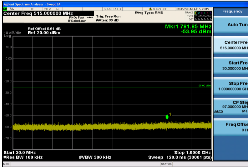
Band7-10MHz-16QAM-20800-1RB#0-Range1:30~1000MHz
