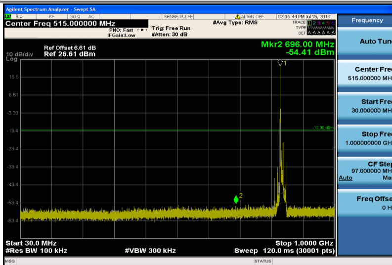
Band5-10MHz-QPSK-20525-1RB#0-Range1:30~1000MHz
