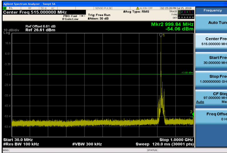
Band5-10MHz-QPSK-20450-1RB#0-Range1:30~1000MHz
