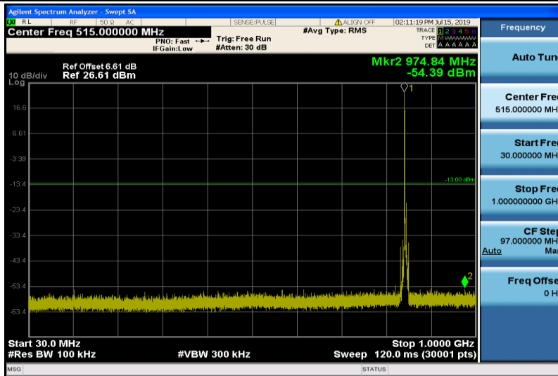
Band5-5MHz-16QAM-20625-1RB#0-Range1:30~1000MHz
