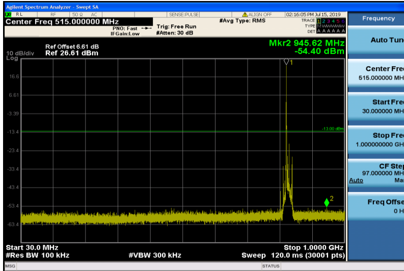
Band5-10MHz-16QAM-20450-1RB#0-Range1:30~1000MHz
