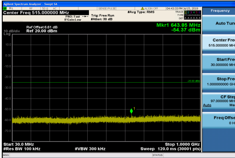
Band7-15MHz-16QAM-20825-1RB#0-Range1:30~1000MHz
