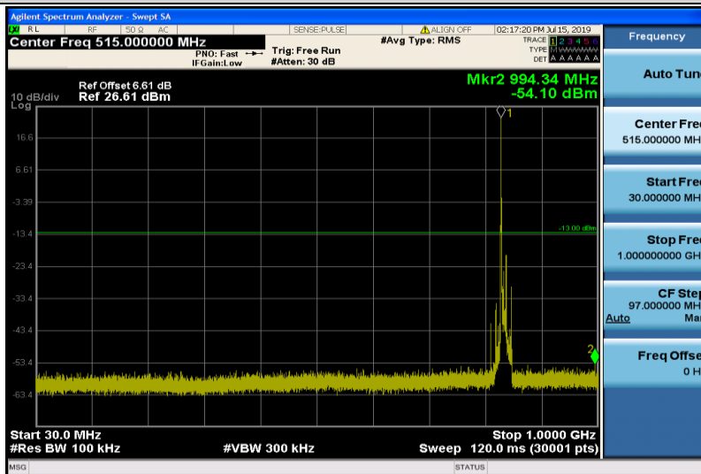
Band5-10MHz-16QAM-20525-1RB#0-Range1:30~1000MHz
