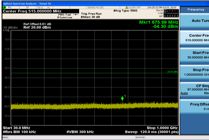
Band7-5MHz-QPSK-20775-1RB#0-Range1:30~1000MHz
