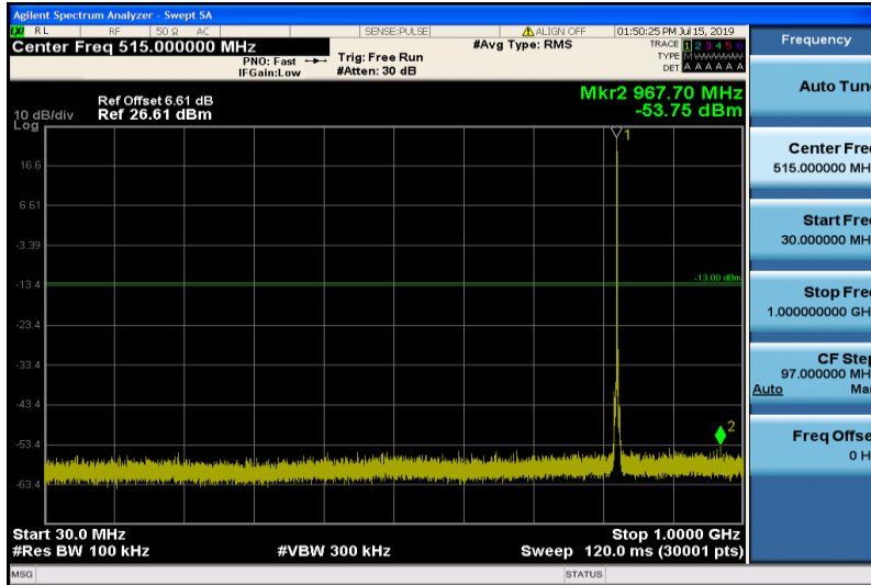
Band5-1.4MHz-16QAM-20407-1RB#0-Range1:30~1000MHz
