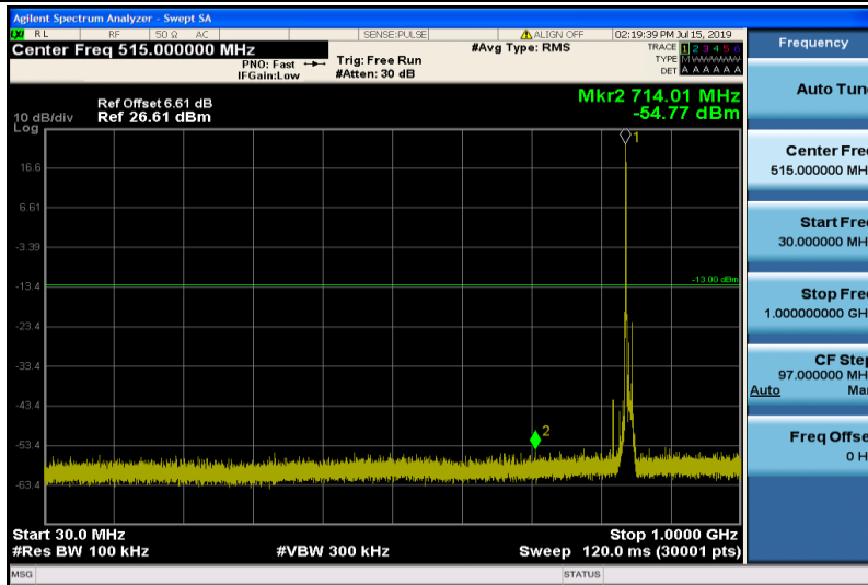
Band5-10MHz-16QAM-20600-1RB#0-Range1:30~1000MHz
