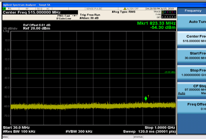
Band7-5MHz-QPSK-21100-1RB#0-Range1:30~1000MHz
