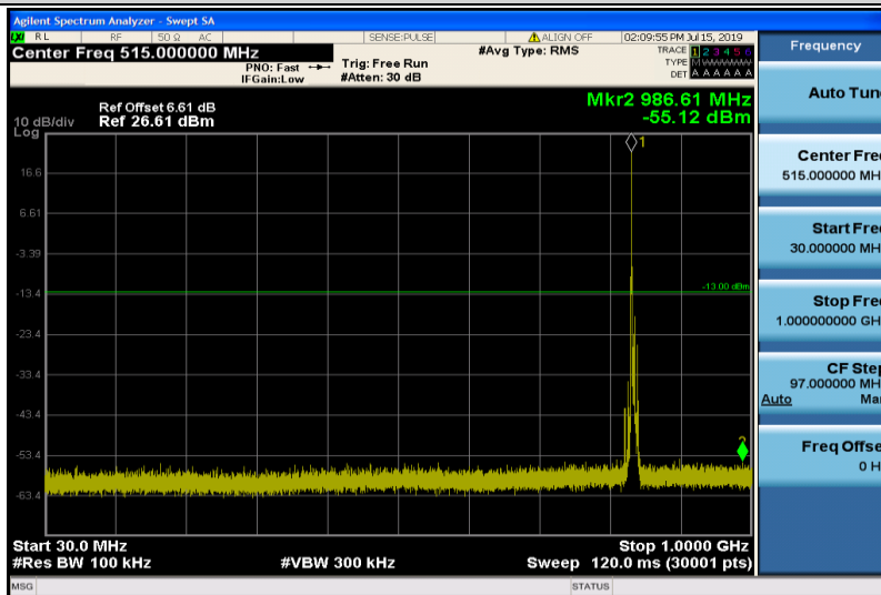
Band5-5MHz-16QAM-20525-1RB#0-Range1:30~1000MHz
