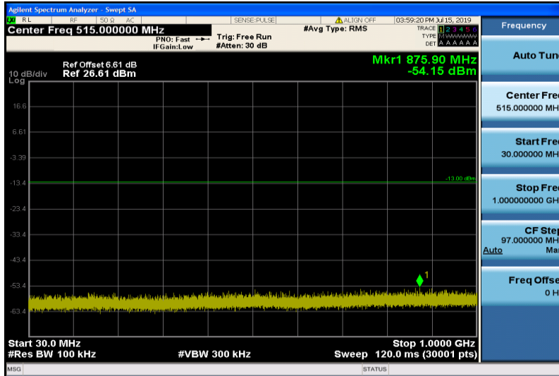
Band4-20MHz-16QAM-20050-1RB#0-Range1:30~1000MHz
