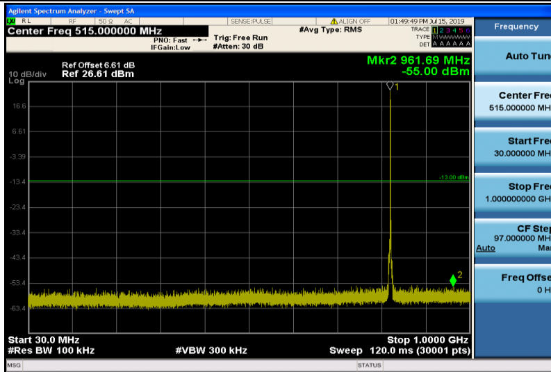
Band5-1.4MHz-QPSK-20407-1RB#0-Range1:30~1000MHz
