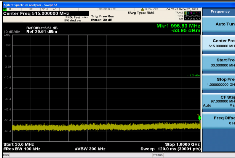
Band4-20MHz-16QAM-20300-1RB#0-Range1:30~1000MHz
