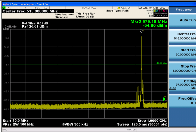
Band5-10MHz-QPSK-20600-1RB#0-Range1:30~1000MHz
