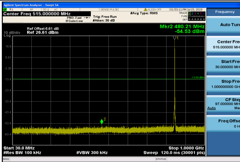
Band5-1.4MHz-QPSK-20643-1RB#0-Range1:30~1000MHz
