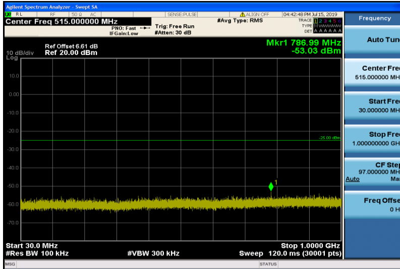
Band7-15MHz-QPSK-20825-1RB#0-Range1:30~1000MHz
