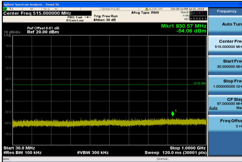
Band7-10MHz-16QAM-21400-1RB#0-Range1:30~1000MHz
