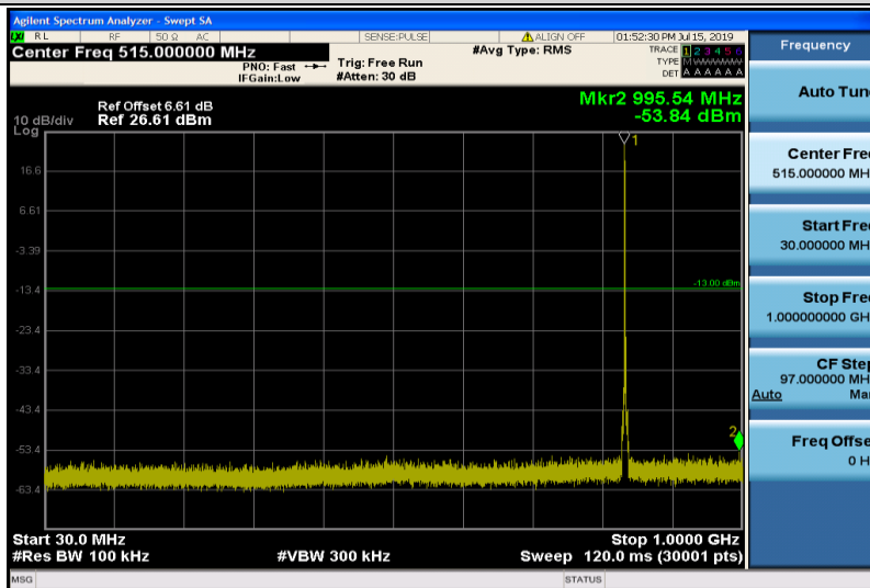
Band5-1.4MHz-16QAM-20525-1RB#0-Range1:30~1000MHz
