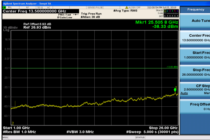
Band5-3MHz-16QAM-20525-1RB#0-Range2:1000~26000MHz
