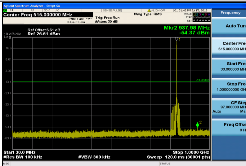
Band5-1.4MHz-QPSK-20525-1RB#0-Range1:30~1000MHz
