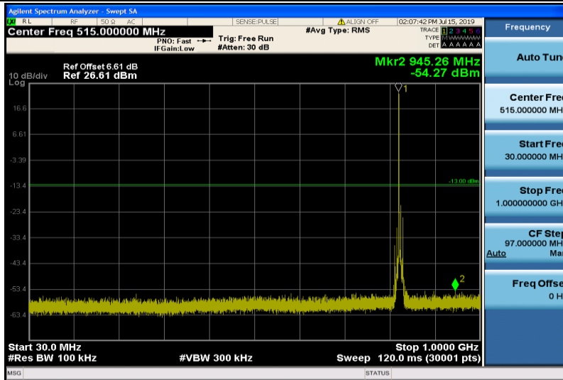
Band5-5MHz-QPSK-20425-1RB#0-Range1:30~1000MHz
