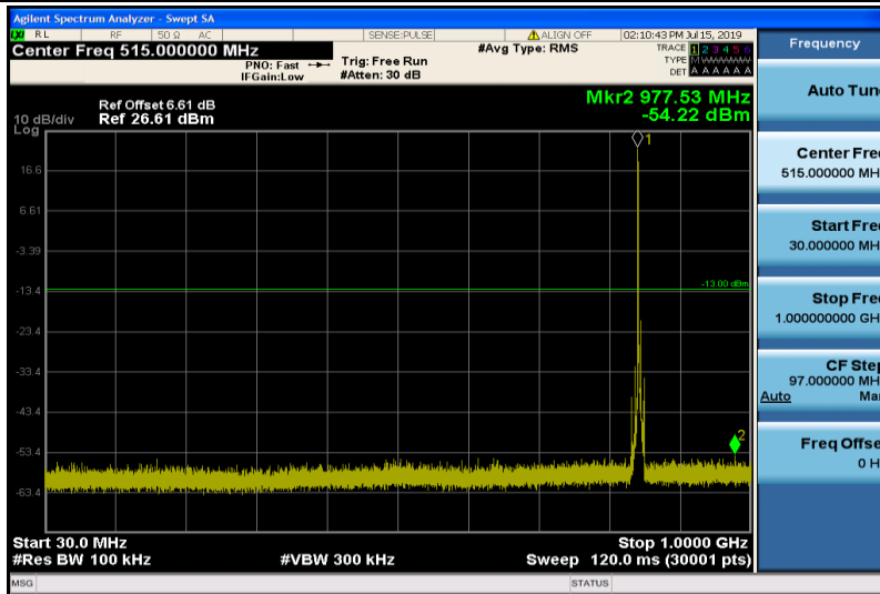
Band5-5MHz-QPSK-20625-1RB#0-Range1:30~1000MHz
