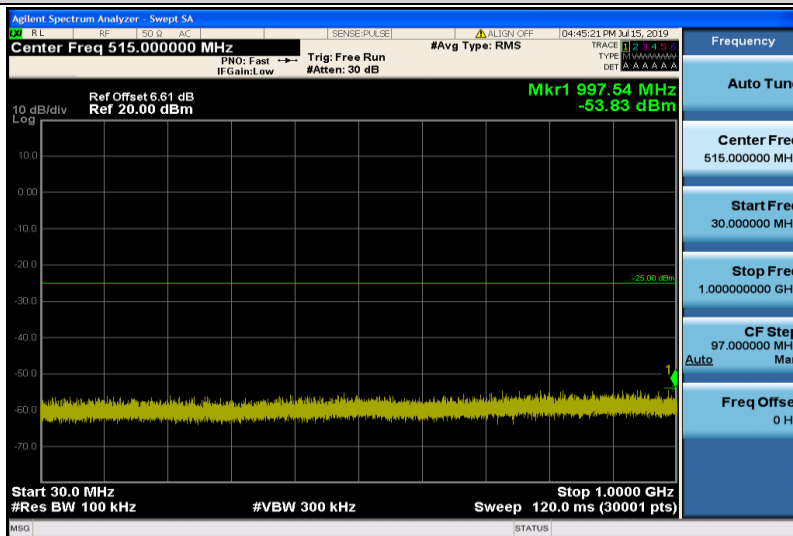
Band7-15MHz-16QAM-21100-1RB#0-Range1:30~1000MHz
