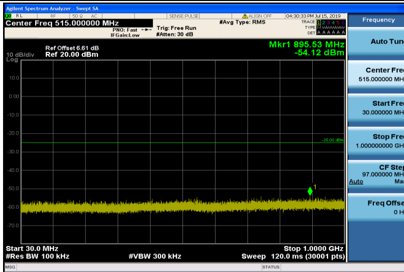
Band7-5MHz-QPSK-21425-1RB#0-Range1:30~1000MHz
