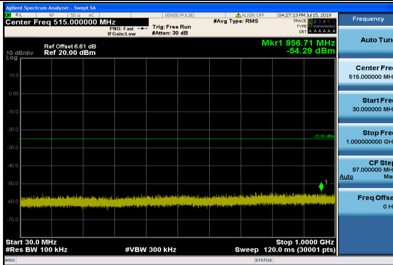
Band7-5MHz-16QAM-20775-1RB#0-Range1:30~1000MHz
