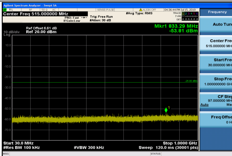
Band7-10MHz-QPSK-21100-1RB#0-Range1:30~1000MHz
