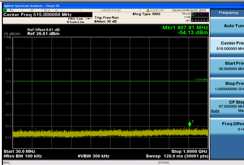
Band4-20MHz-16QAM-20175-1RB#0-Range1:30~1000MHz
