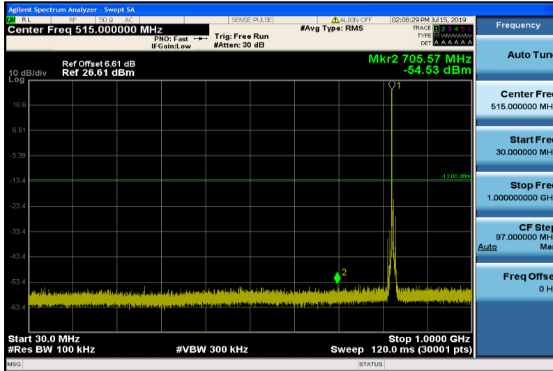
Band5-5MHz-16QAM-20425-1RB#0-Range1:30~1000MHz
