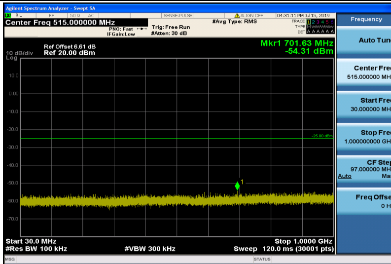
Band7-5MHz-16QAM-21425-1RB#0-Range1:30~1000MHz
