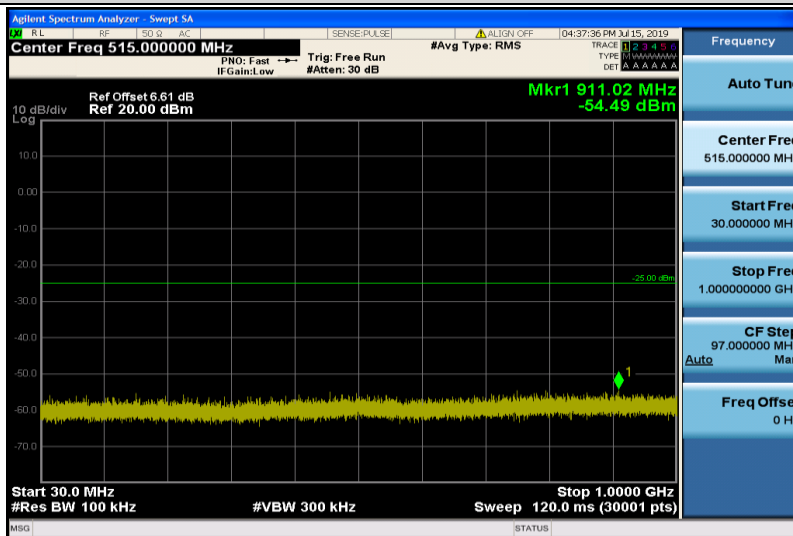
Band7-10MHz-16QAM-21100-1RB#0-Range1:30~1000MHz
