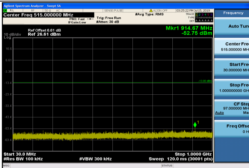
Band4-1.4MHz-16QAM-20175-1RB#0-Range1:30~1000MHz
