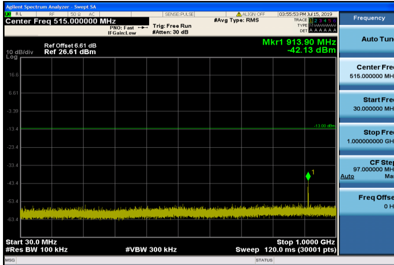
Band4-20MHz-QPSK-20050-1RB#0-Range1:30~1000MHz
