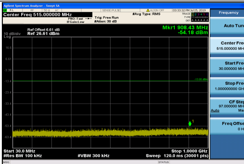
Band4-3MHz-QPSK-20175-1RB#0-Range1:30~1000MHz
