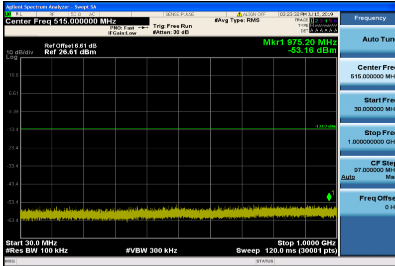
Band4-1.4MHz-16QAM-19957-1RB#0-Range1:30~1000MHz
