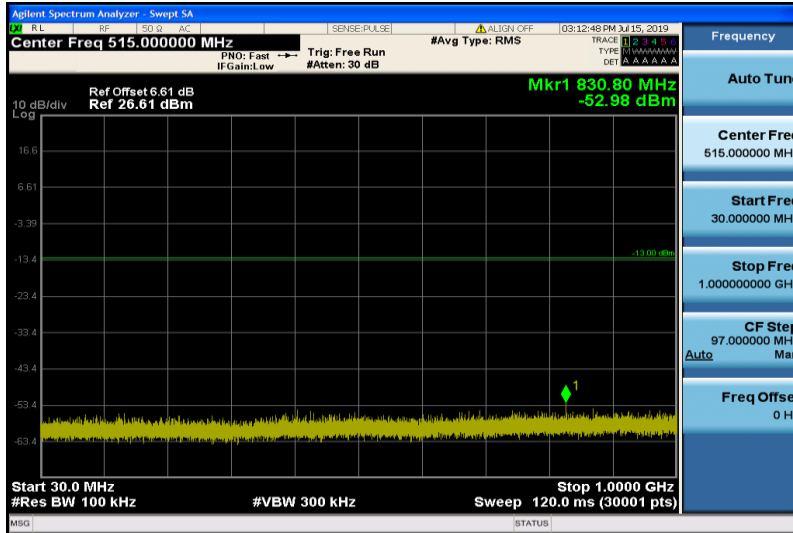
Band2-20MHz-16QAM-18700-1RB#0-Range1:30~1000MHz
