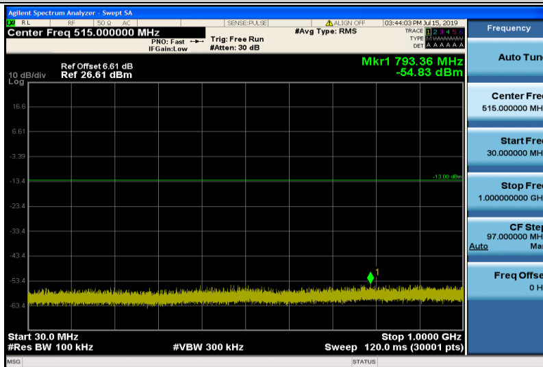
Band4-5MHz-16QAM-20175-1RB#0-Range1:30~1000MHz
