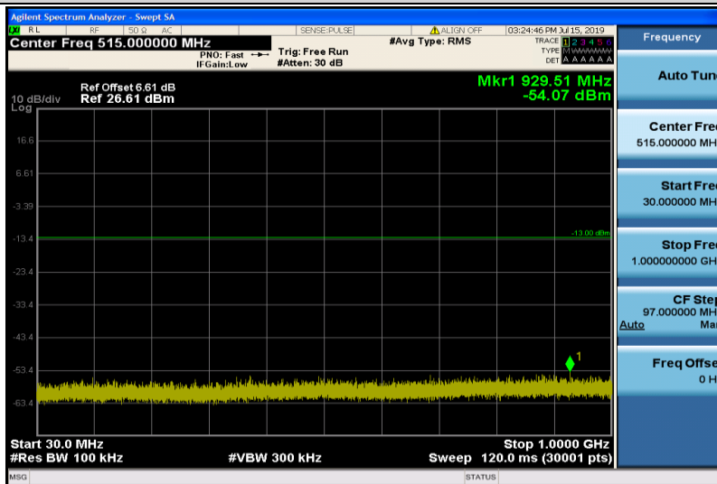
Band4-1.4MHz-QPSK-20175-1RB#0-Range1:30~1000MHz
