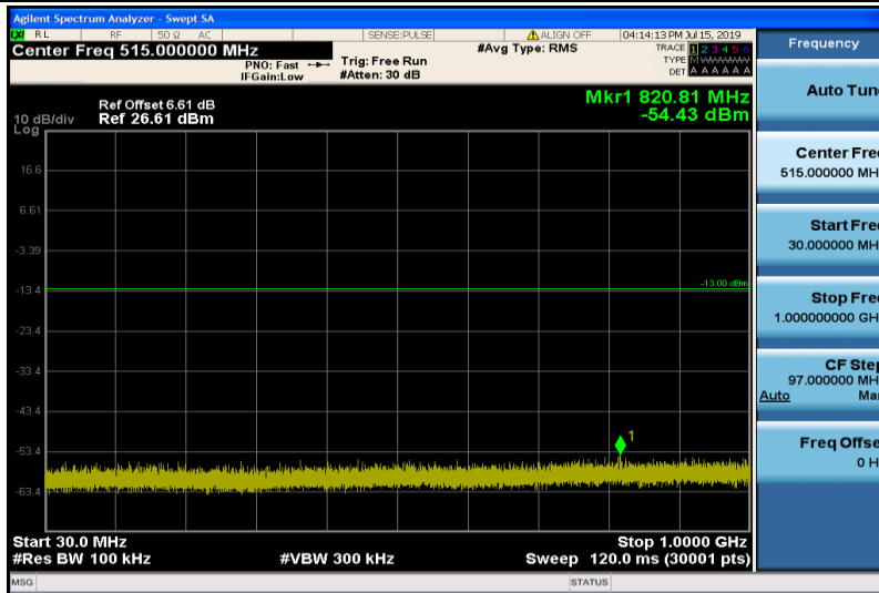
Band4-10MHz-16QAM-20350-1RB#0-Range1:30~1000MHz
