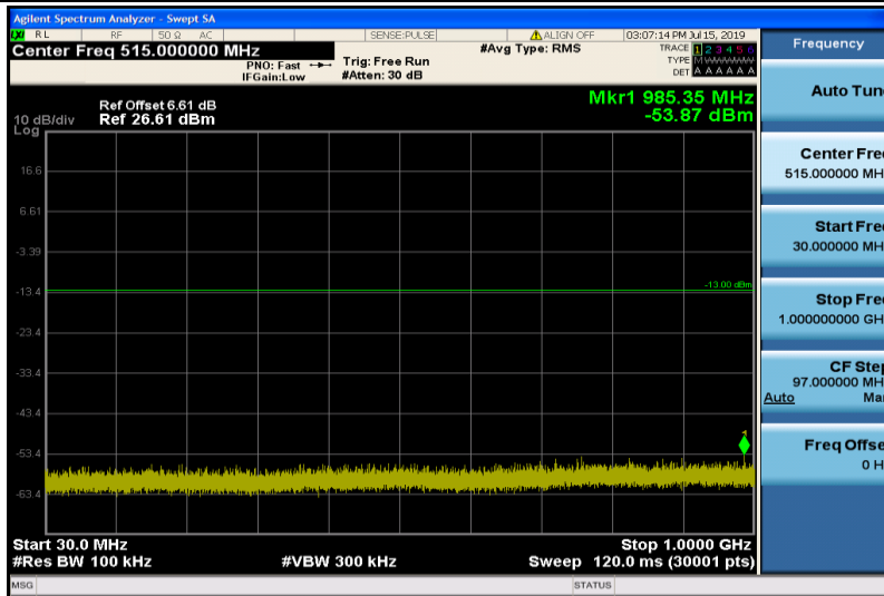
Band2-15MHz-QPSK-19125-1RB#0-Range1:30~1000MHz
