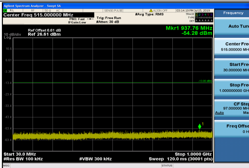
Band2-20MHz-16QAM-18900-1RB#0-Range1:30~1000MHz
