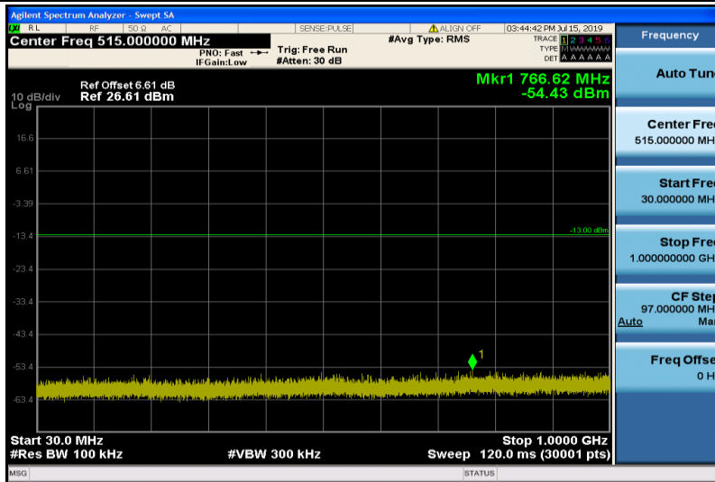
Band4-5MHz-QPSK-20375-1RB#0-Range1:30~1000MHz
