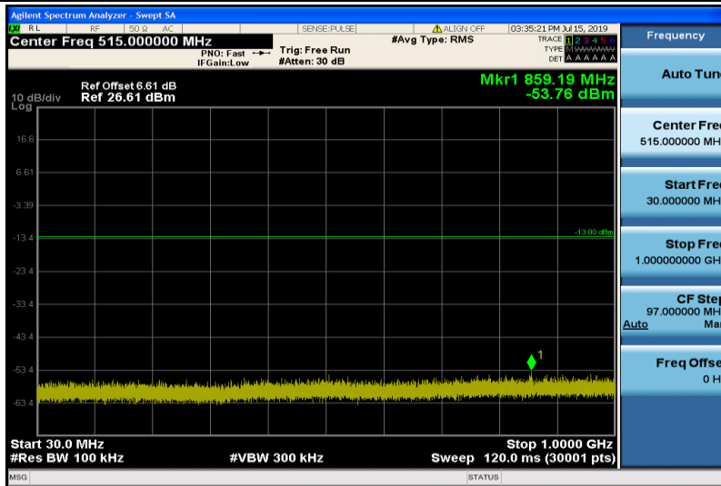
Band4-3MHz-QPSK-20385-1RB#0-Range1:30~1000MHz
