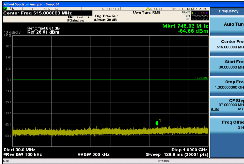
Band4-10MHz-16QAM-20000-1RB#0-Range1:30~1000MHz
