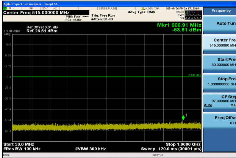
Band4-15MHz-QPSK-20025-1RB#0-Range1:30~1000MHz
