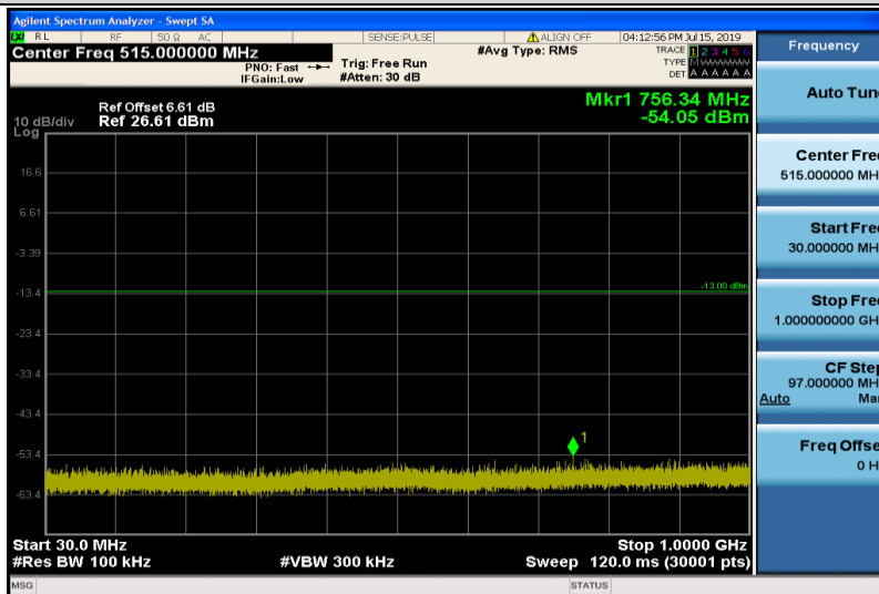
Band4-10MHz-16QAM-20175-1RB#0-Range1:30~1000MHz
