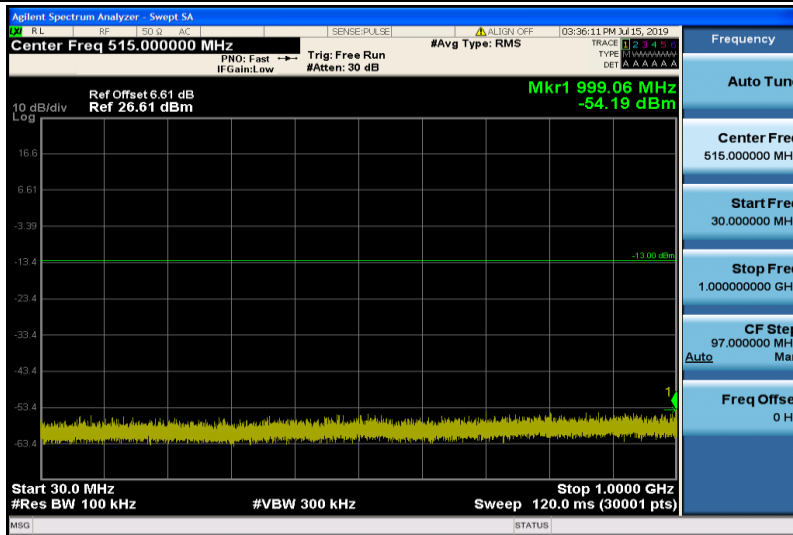
Band4-3MHz-16QAM-20385-1RB#0-Range1:30~1000MHz
