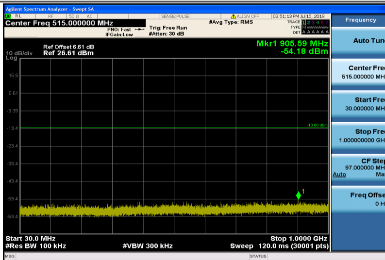
Band4-15MHz-16QAM-20175-1RB#0-Range1:30~1000MHz
