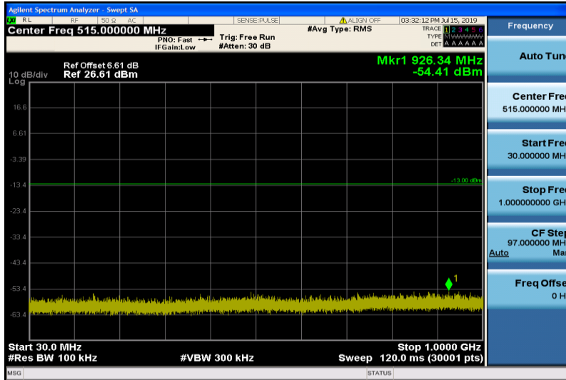
Band4-3MHz-QPSK-19965-1RB#0-Range1:30~1000MHz
