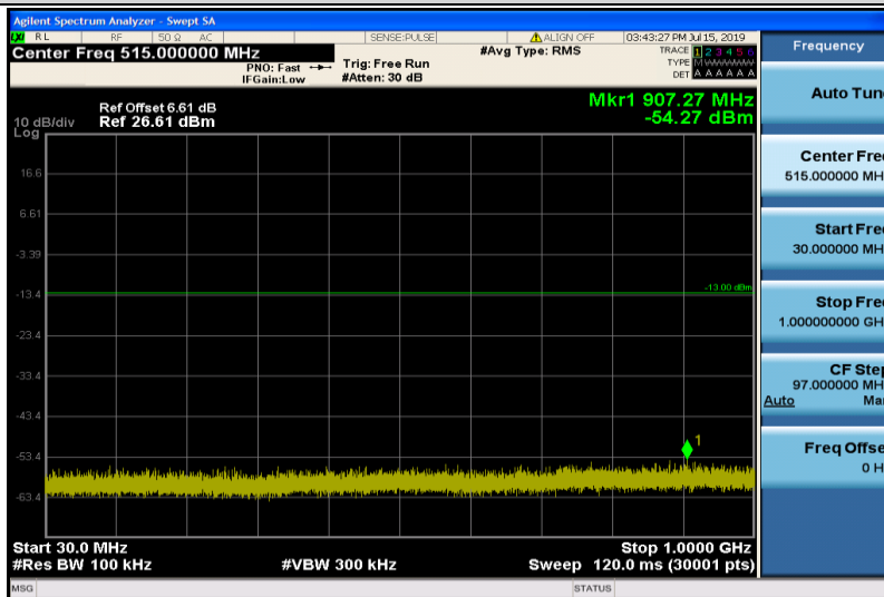
Band4-5MHz-QPSK-20175-1RB#0-Range1:30~1000MHz
