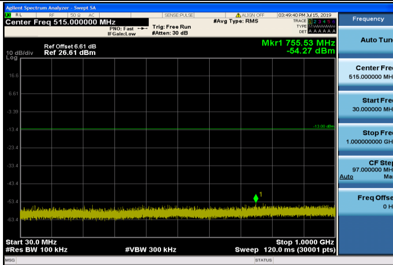
Band4-15MHz-16QAM-20025-1RB#0-Range1:30~1000MHz
