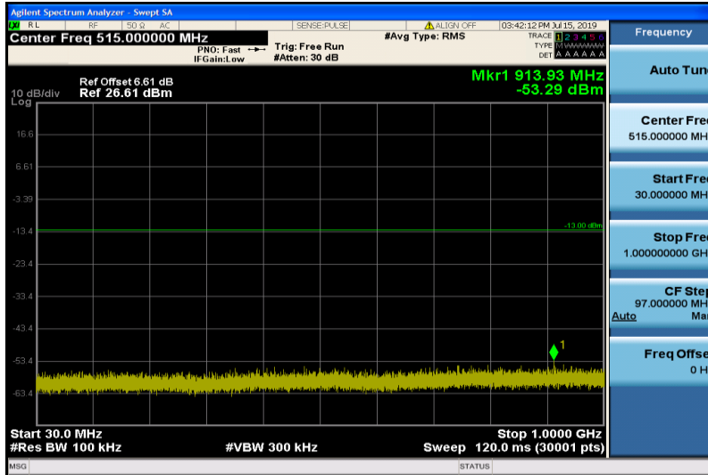
Band4-5MHz-QPSK-19975-1RB#0-Range1:30~1000MHz
