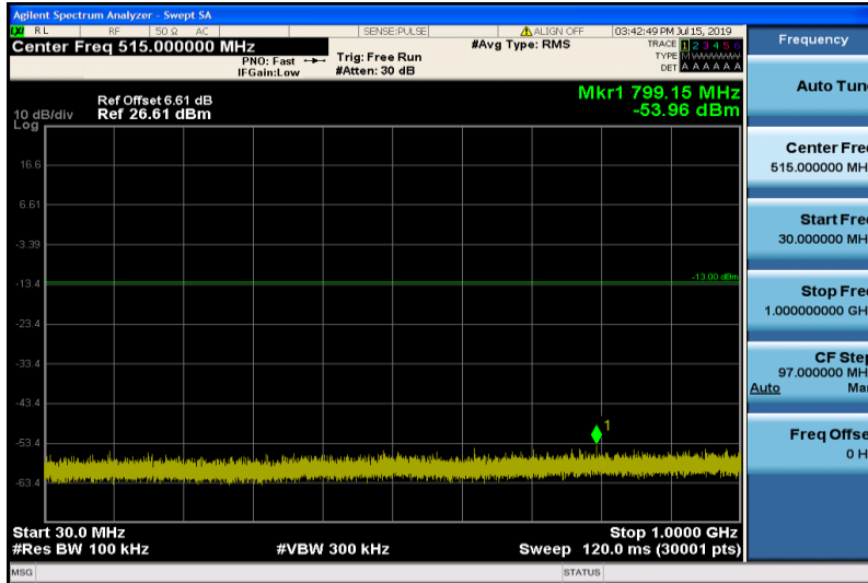
Band4-5MHz-16QAM-19975-1RB#0-Range1:30~1000MHz
