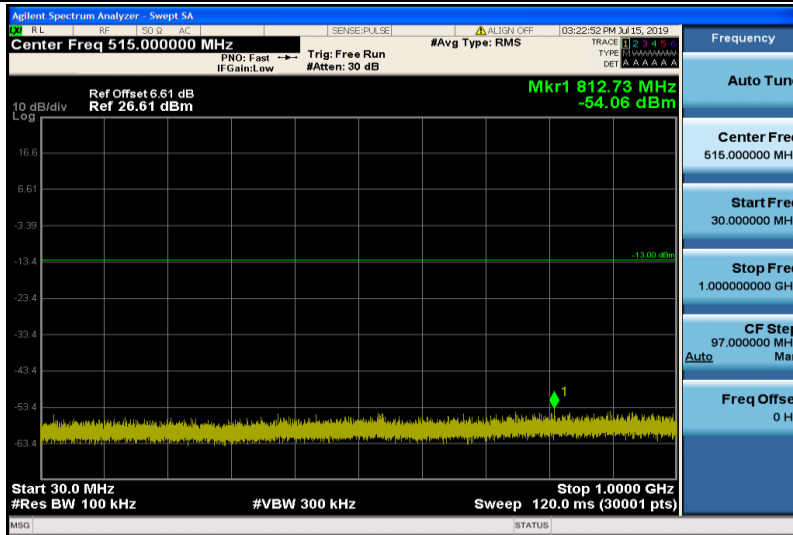
Band4-1.4MHz-QPSK-19957-1RB#0-Range1:30~1000MHz
