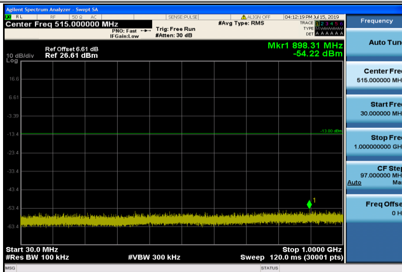
Band4-10MHz-QPSK-20175-1RB#0-Range1:30~1000MHz
