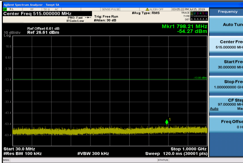
Band2-15MHz-16QAM-18675-1RB#0-Range1:30~1000MHz
