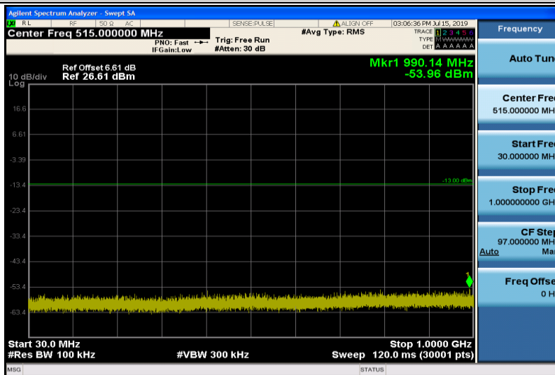
Band2-15MHz-16QAM-18900-1RB#0-Range1:30~1000MHz
