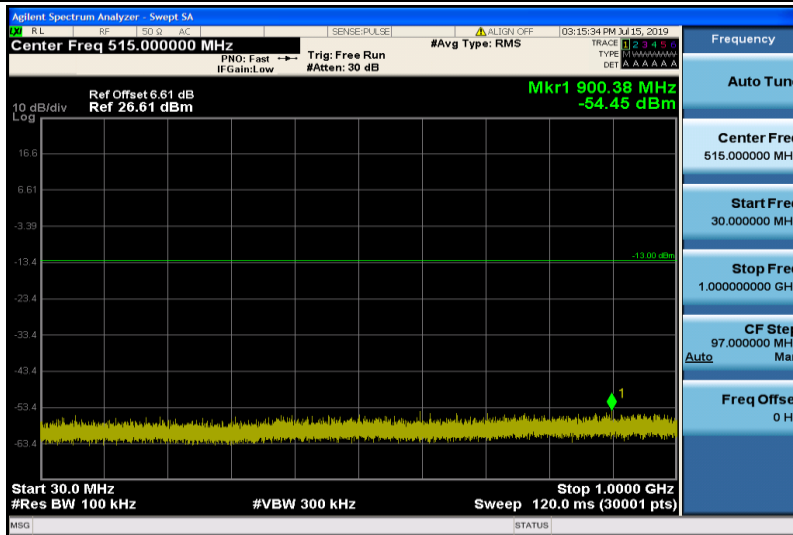
Band2-20MHz-16QAM-19100-1RB#0-Range1:30~1000MHz
