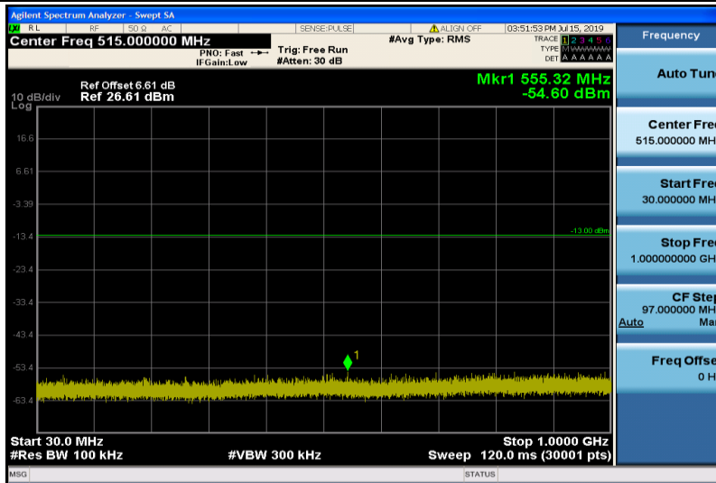
Band4-15MHz-QPSK-20325-1RB#0-Range1:30~1000MHz
