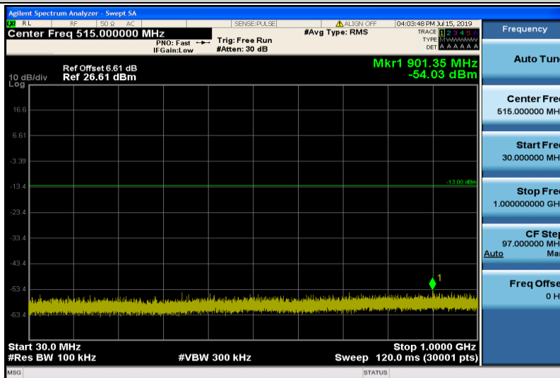
Band4-20MHz-QPSK-20175-1RB#0-Range1:30~1000MHz
