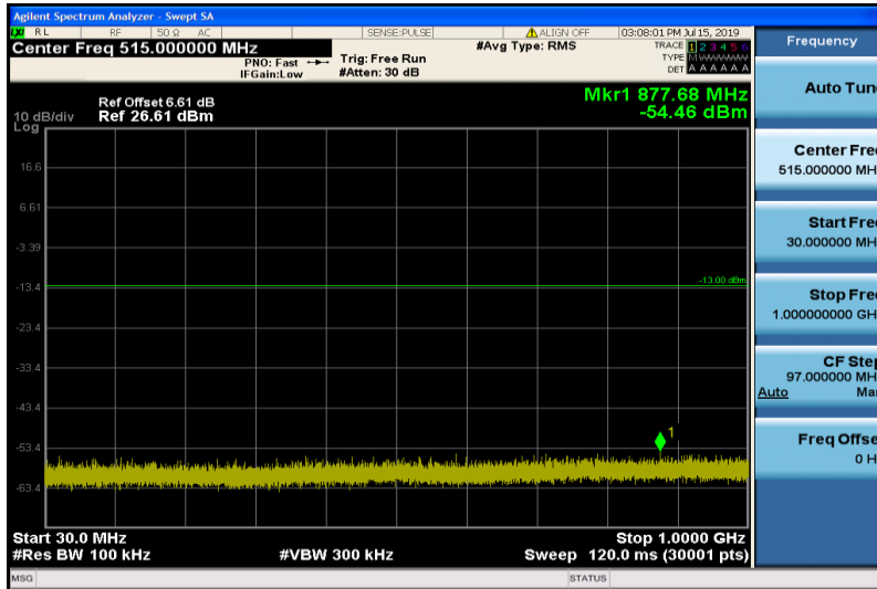
Band2-15MHz-16QAM-19125-1RB#0-Range1:30~1000MHz
