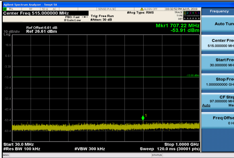
Band4-3MHz-16QAM-19965-1RB#0-Range1:30~1000MHz
