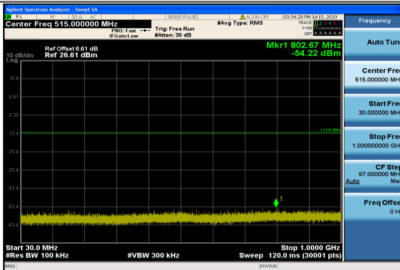
Band4-3MHz-16QAM-20175-1RB#0-Range1:30~1000MHz
