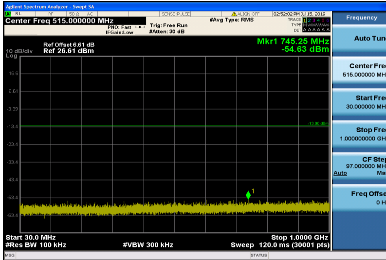
Band2-10MHz-16QAM-18650-1RB#0-Range1:30~1000MHz
