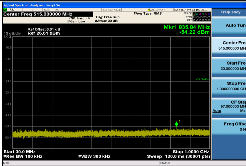
Band2-10MHz-QPSK-19150-1RB#0-Range1:30~1000MHz
