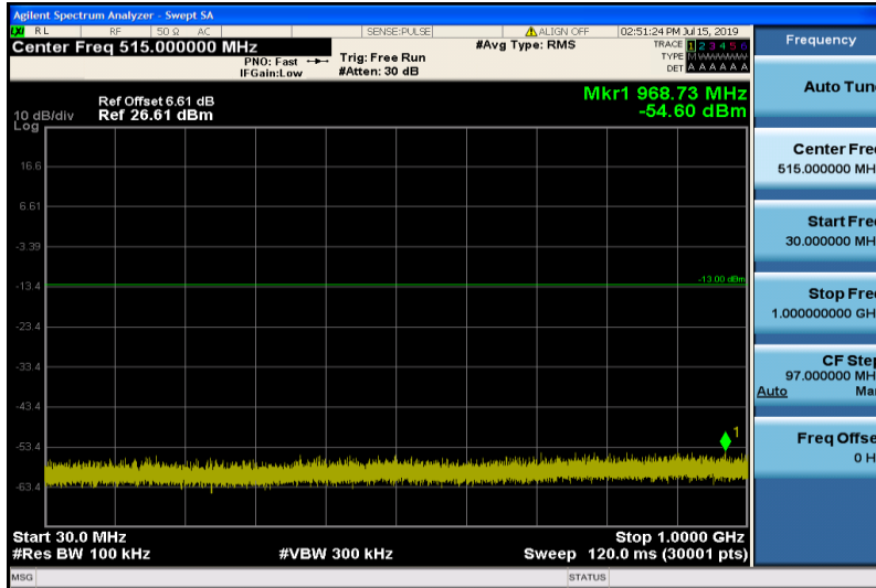
Band2-10MHz-QPSK-18650-1RB#0-Range1:30~1000MHz
