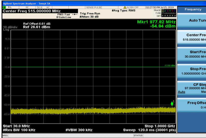
Band2-1.4MHz-16QAM-18607-1RB#0-Range1:30~1000MHz
