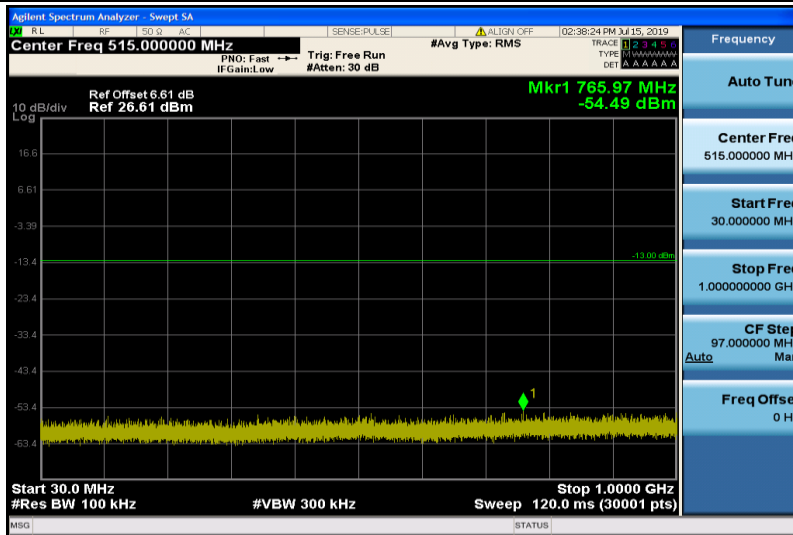
Band2-3MHz-16QAM-19185-1RB#0-Range1:30~1000MHz
