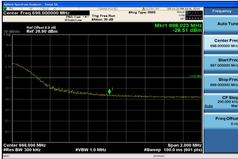
Band71-20MHz-16QAM-133372-100RB#0
