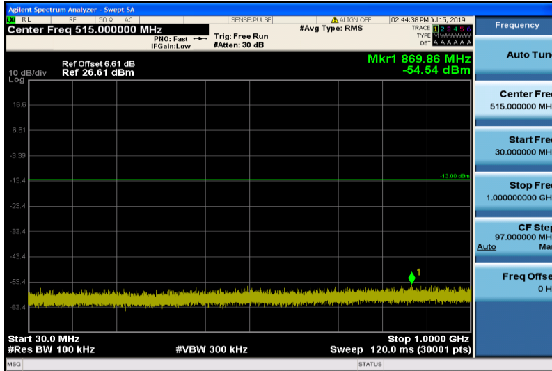
Band2-5MHz-16QAM-18625-1RB#0-Range1:30~1000MHz
