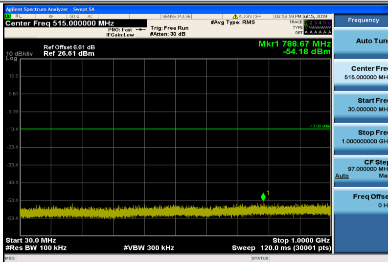
Band2-10MHz-QPSK-18900-1RB#0-Range1:30~1000MHz
