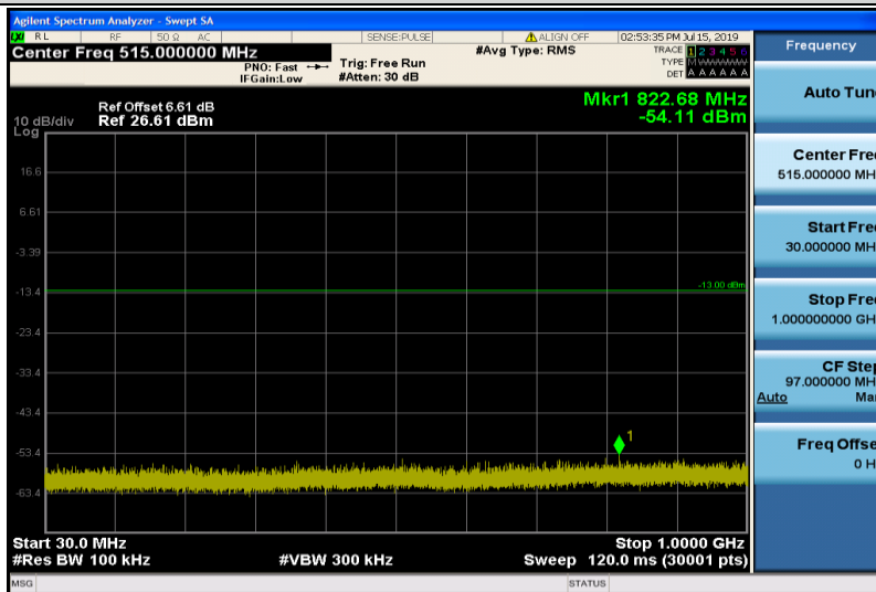
Band2-10MHz-16QAM-18900-1RB#0-Range1:30~1000MHz
