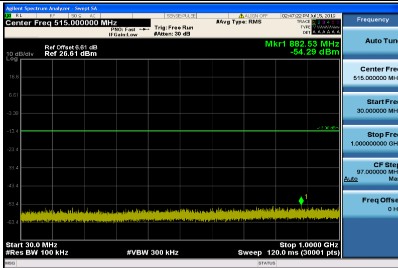
Band2-5MHz-QPSK-19175-1RB#0-Range1:30~1000MHz
