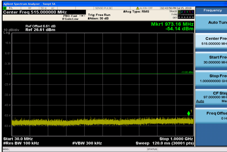
Band2-5MHz-QPSK-18625-1RB#0-Range1:30~1000MHz
