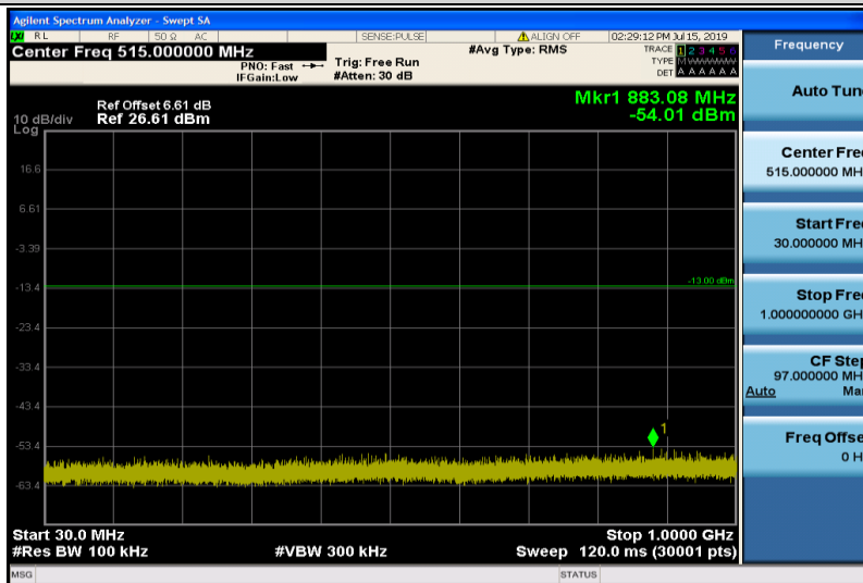
Band2-1.4MHz-16QAM-18900-1RB#0-Range1:30~1000MHz
