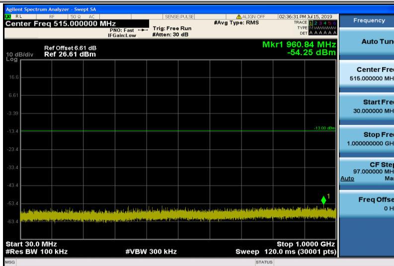
Band2-3MHz-QPSK-18900-1RB#0-Range1:30~1000MHz
