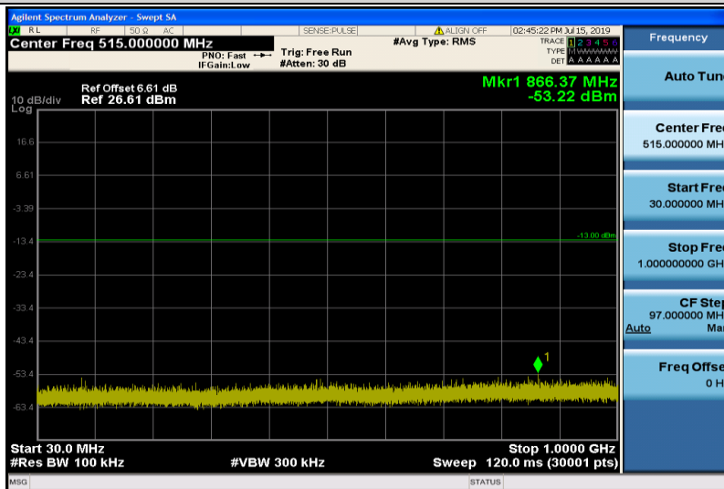
Band2-5MHz-QPSK-18900-1RB#0-Range1:30~1000MHz
