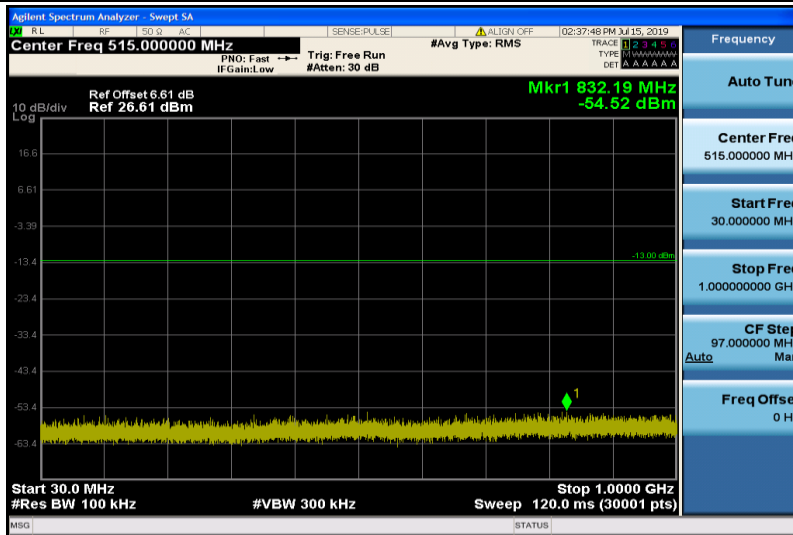
Band2-3MHz-QPSK-19185-1RB#0-Range1:30~1000MHz
