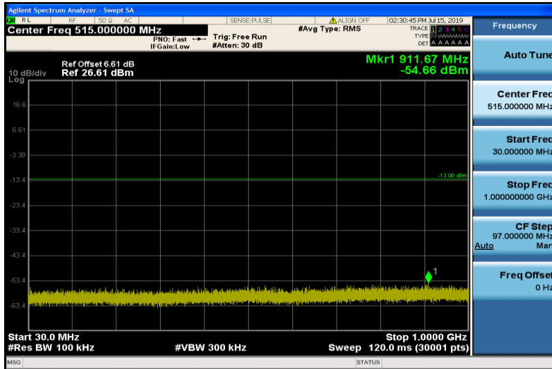
Band2-1.4MHz-16QAM-19193-1RB#0-Range1:30~1000MHz
