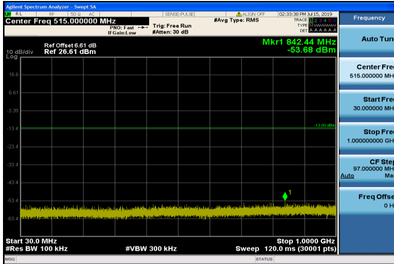
Band2-3MHz-QPSK-18615-1RB#0-Range1:30~1000MHz
