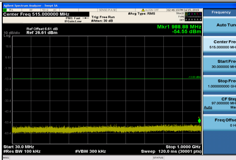
Band2-5MHz-16QAM-18900-1RB#0-Range1:30~1000MHz
