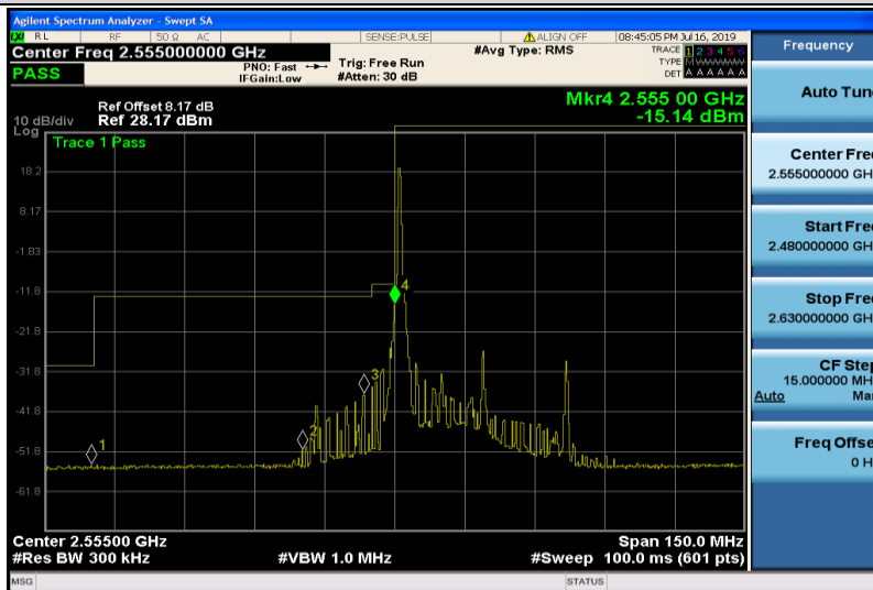
Band41-20MHz-16QAM-40340-1RB#0
