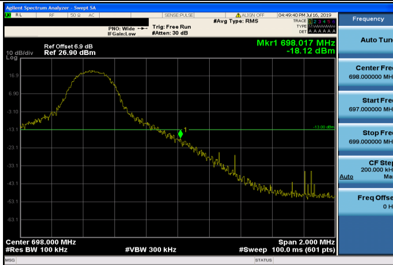
Band71-5MHz-16QAM-133447-1RB#24
