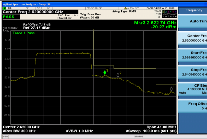
Band38-15MHz-16QAM-38175-75RB#0
