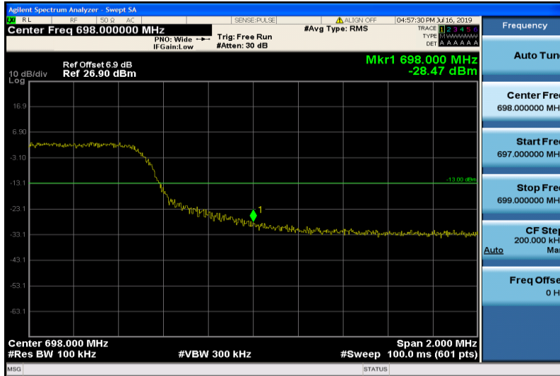
Band71-10MHz-16QAM-133422-50RB#0
