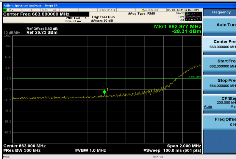
Band71-20MHz-16QAM-133222-100RB#0
