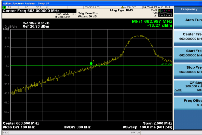
Band71-10MHz-16QAM-133172-1RB#0
