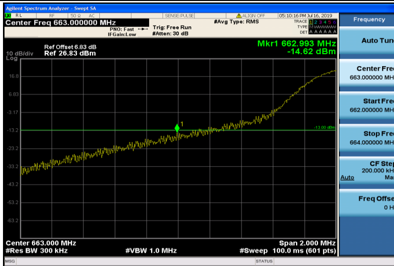
Band71-20MHz-16QAM-133222-1RB#0
