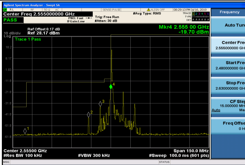
Band41-10MHz-16QAM-40290-1RB#0
