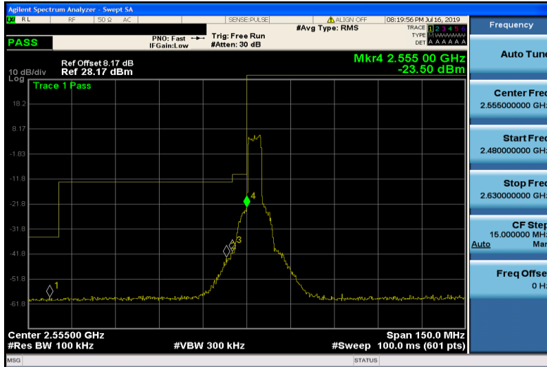
Band41-5MHz-16QAM-40265-25RB#0
