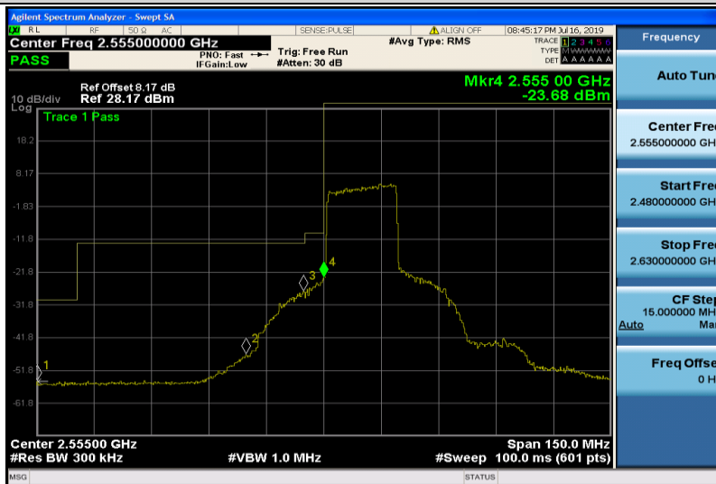
Band41-20MHz-QPSK-40340-100RB#0
