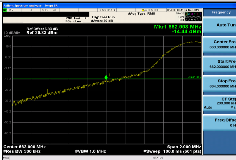
Band71-15MHz-16QAM-133197-1RB#0
