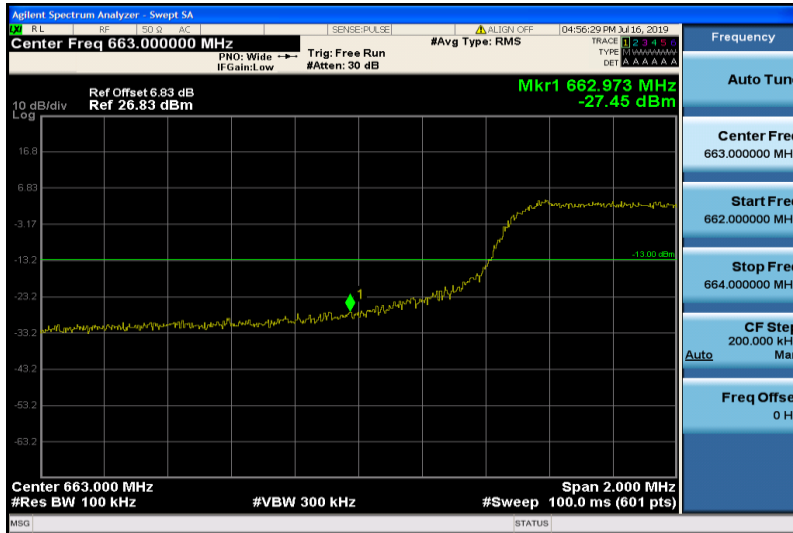
Band71-10MHz-16QAM-133172-50RB#0
