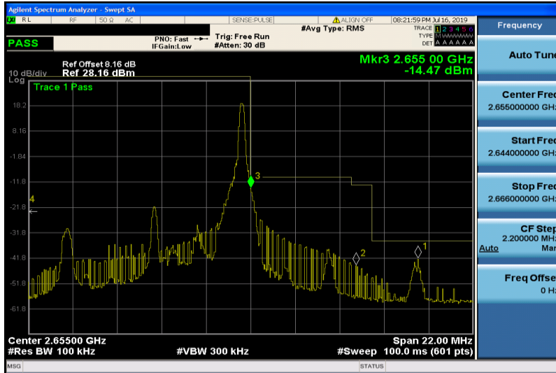
Band41-5MHz-QPSK-41215-1RB#24
