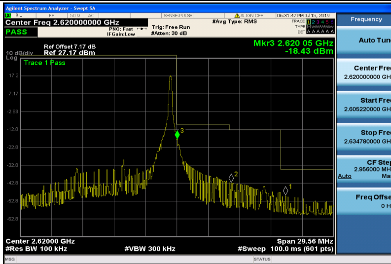
Band38-10MHz-16QAM-38200-1RB#49
