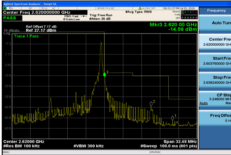
Band38-10MHz-QPSK-38200-1RB#49
