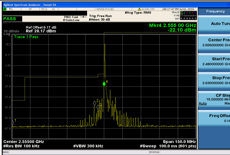
Band41-5MHz-QPSK-40265-1RB#0
