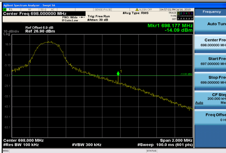
Band71-10MHz-16QAM-133422-1RB#49
