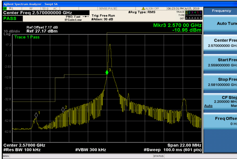
Band38-5MHz-16QAM-37775-1RB#0
