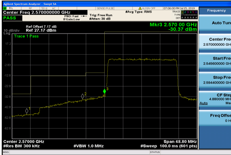
Band38-20MHz-QPSK-37850-100RB#0
