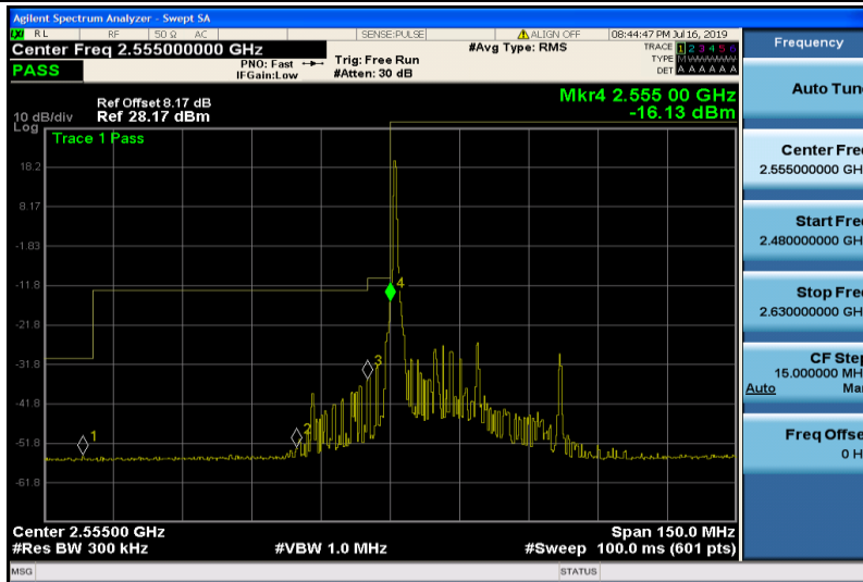
Band41-20MHz-QPSK-40340-1RB#0
