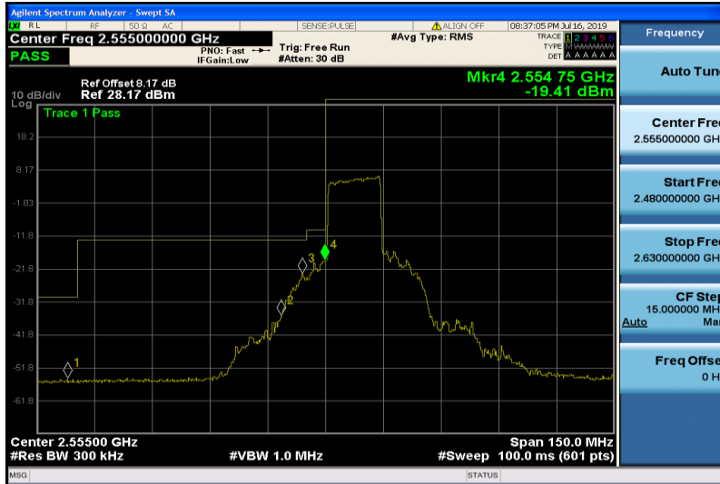
Band41-15MHz-QPSK-40315-75RB#0
