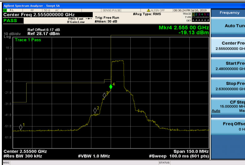
Band41-15MHz-QPSK-40315-1RB#0
