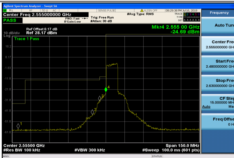
Band41-10MHz-16QAM-40290-50RB#0
