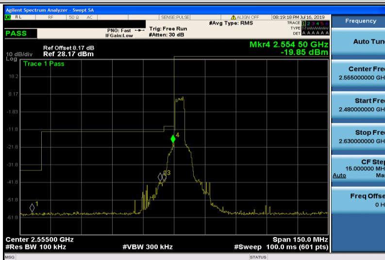
Band41-5MHz-QPSK-40265-25RB#0
