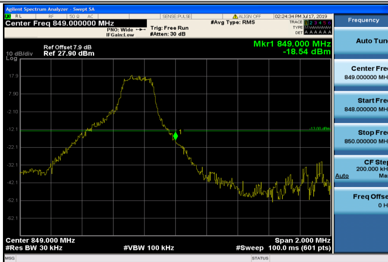
Band26-3MHz-QPSK-27025-1RB#14
