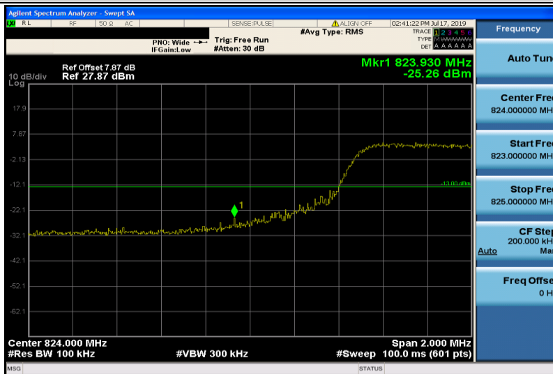
Band26-10MHz-QPSK-26840-50RB#0
