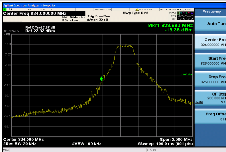
Band26-1.4MHz-16QAM-26797-1RB#0
