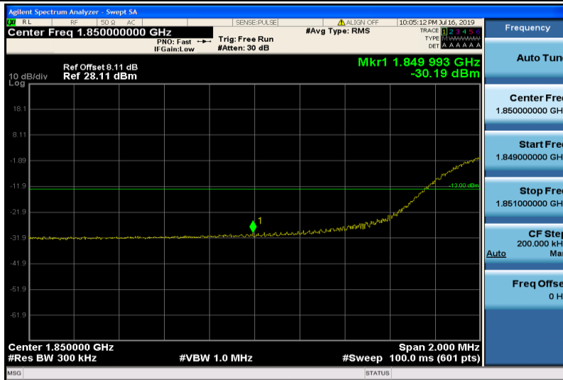
Band25-20MHz-16QAM-26140-100RB#0
