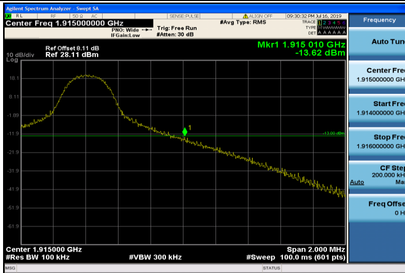
Band25-10MHz-16QAM-26640-1RB#49
