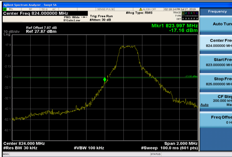
Band26-1.4MHz-QPSK-26797-1RB#0
