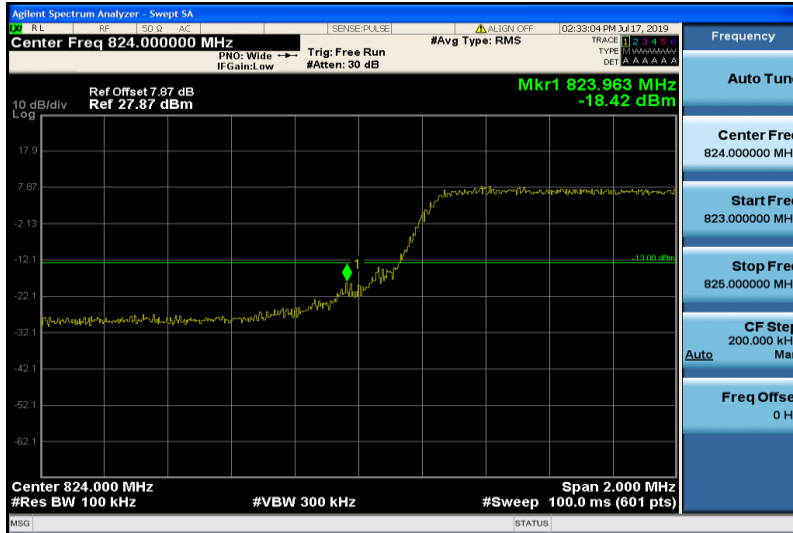
Band26-5MHz-QPSK-26815-25RB#0
