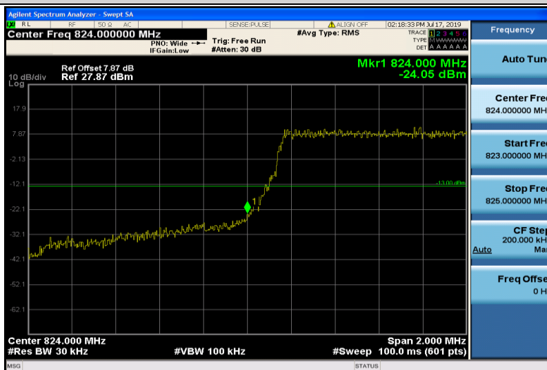
Band26-1.4MHz-QPSK-26797-6RB#0
