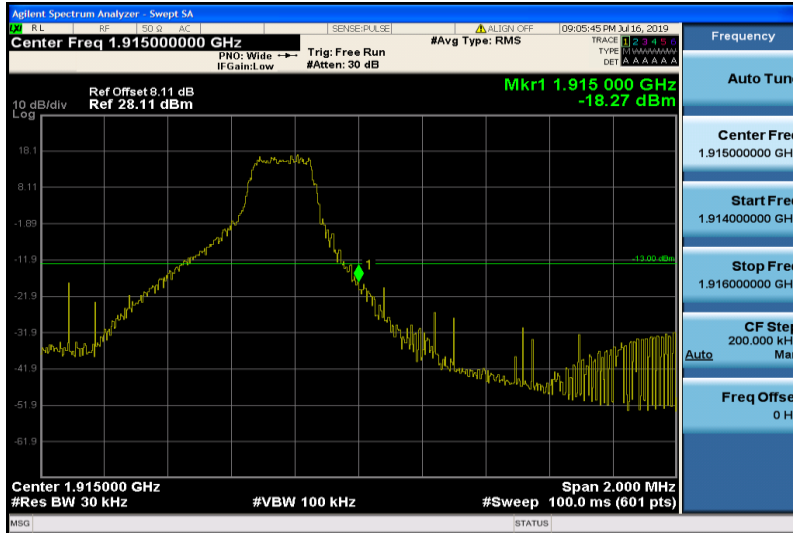
Band25-3MHz-16QAM-26675-1RB#14
