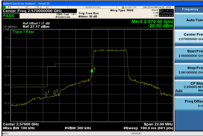
Band38-5MHz-QPSK-37775-25RB#0
