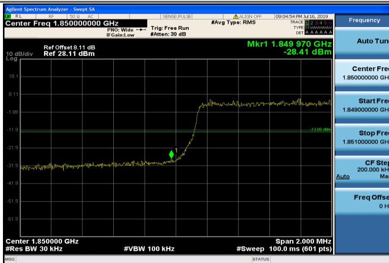
Band25-3MHz-16QAM-26055-15RB#0
