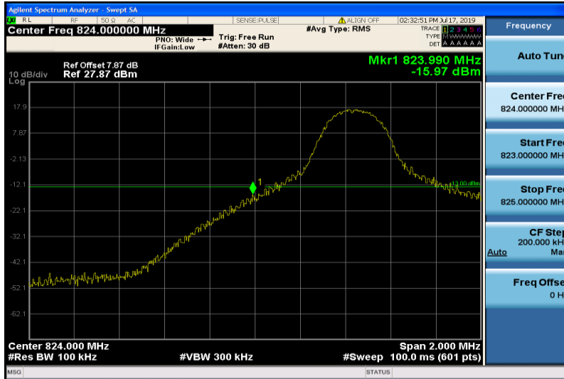
Band26-5MHz-16QAM-26815-1RB#0
