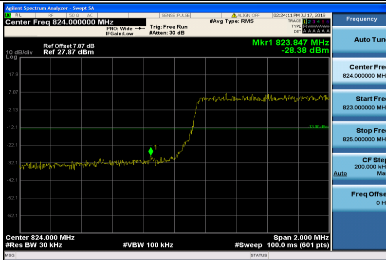
Band26-3MHz-QPSK-26805-15RB#0
