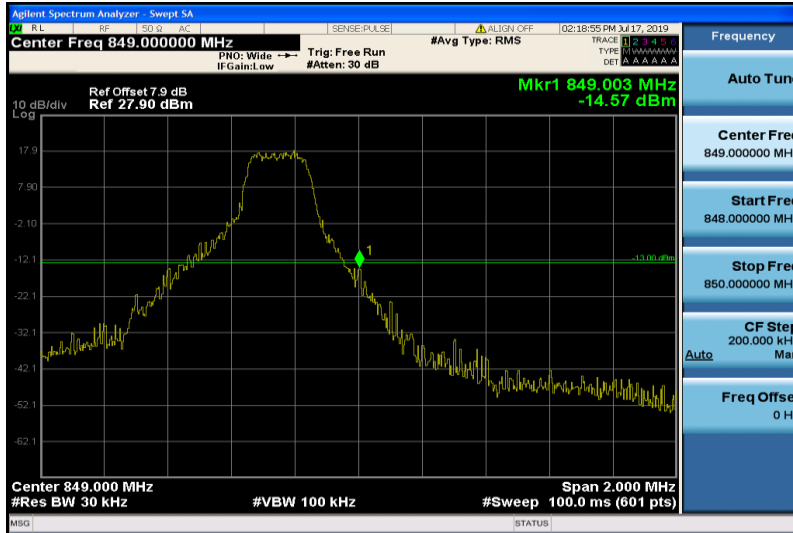
Band26-1.4MHz-QPSK-27033-1RB#5
