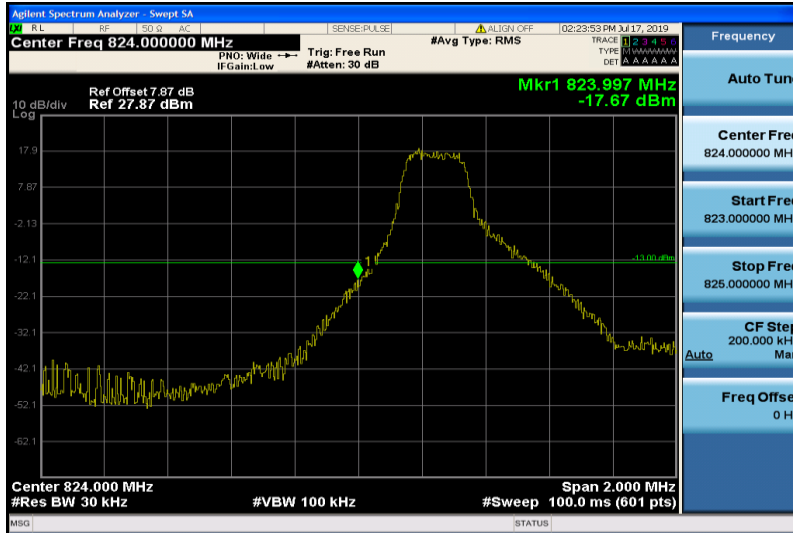
Band26-3MHz-QPSK-26805-1RB#0
