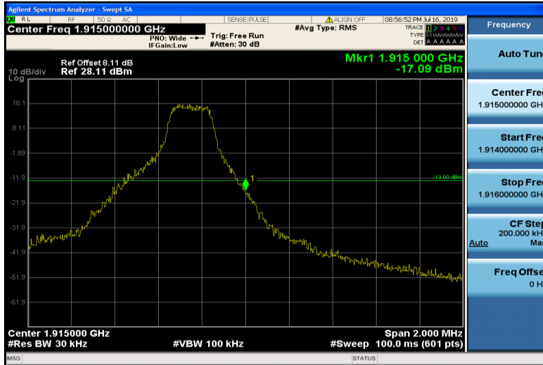
Band25-1.4MHz-QPSK-26683-1RB#5
