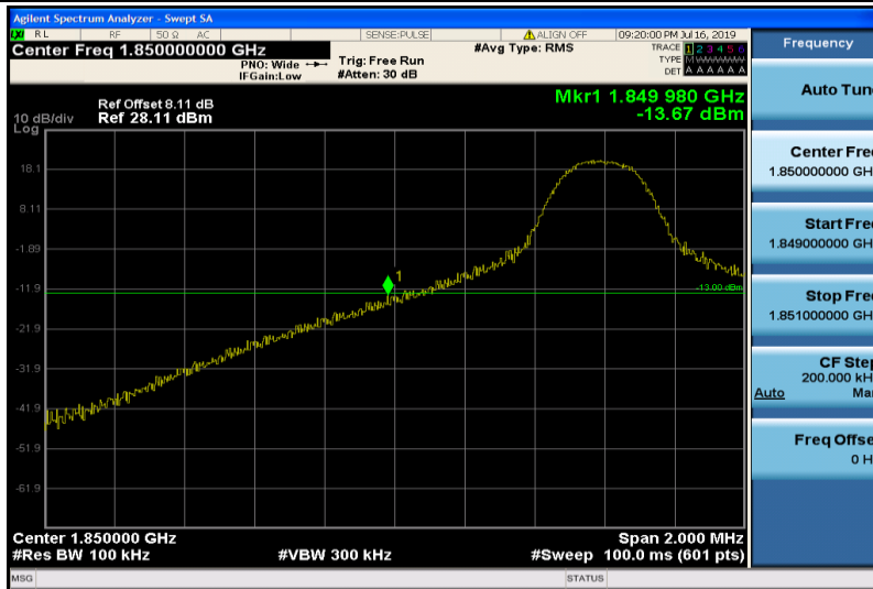
Band25-10MHz-QPSK-26090-1RB#0
