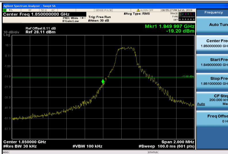
Band25-1.4MHz-16QAM-26047-1RB#0
