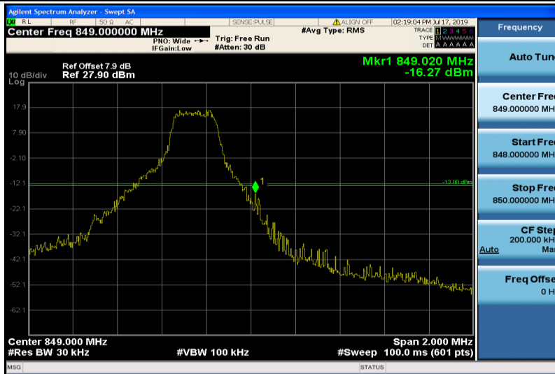
Band26-1.4MHz-16QAM-27033-1RB#5
