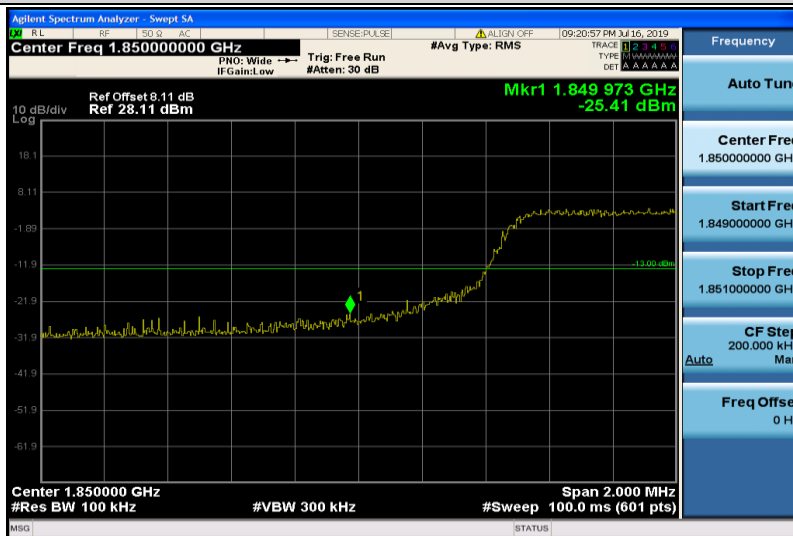
Band25-10MHz-QPSK-26090-50RB#0
