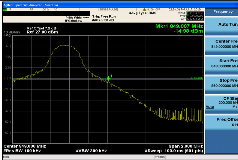
Band26-5MHz-QPSK-27015-1RB#24
