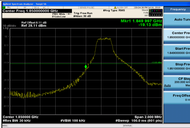
Band25-3MHz-16QAM-26055-1RB#0
