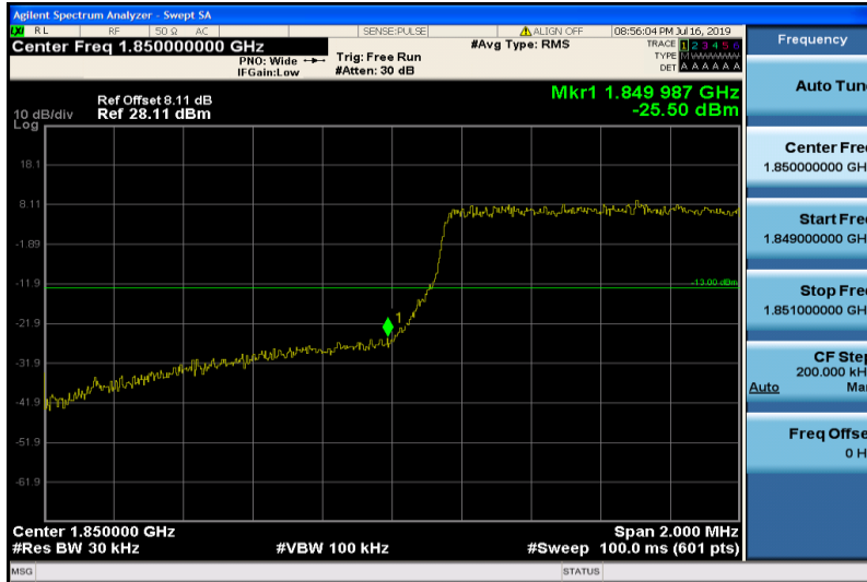
Band25-1.4MHz-16QAM-26047-6RB#0
