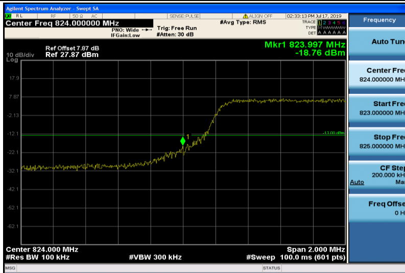
Band26-5MHz-16QAM-26815-25RB#0
