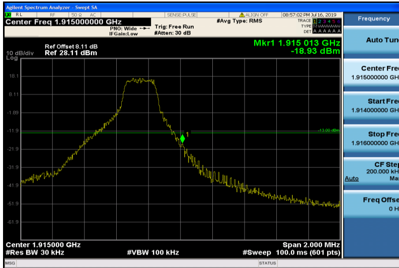
Band25-1.4MHz-16QAM-26683-1RB#5
