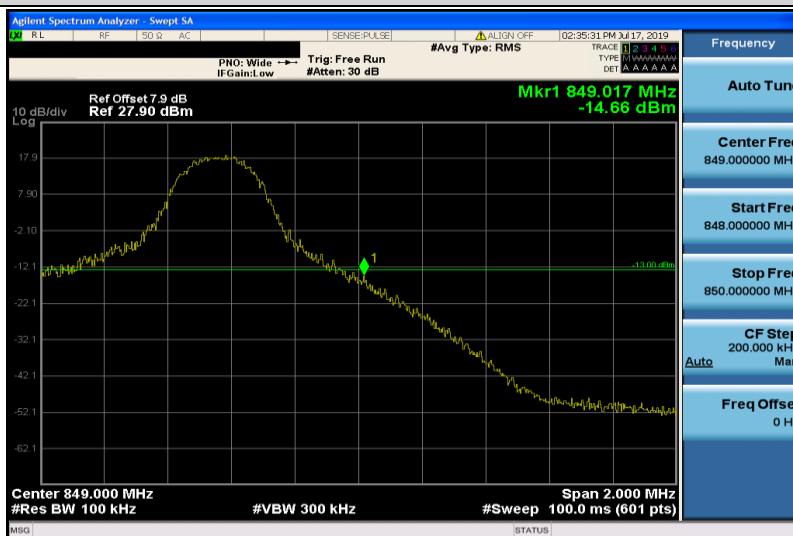
Band26-5MHz-16QAM-27015-1RB#24
