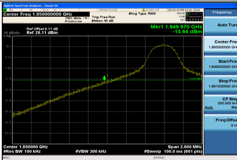
Band25-10MHz-16QAM-26090-1RB#0
