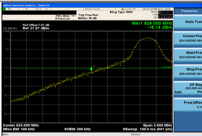
Band26-10MHz-16QAM-26840-1RB#0
