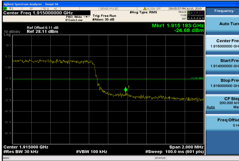
Band25-3MHz-QPSK-26675-15RB#0
