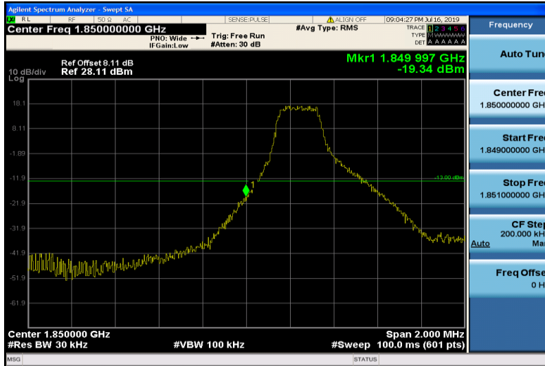
Band25-3MHz-QPSK-26055-1RB#0
