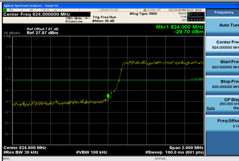
Band26-3MHz-16QAM-26805-15RB#0
