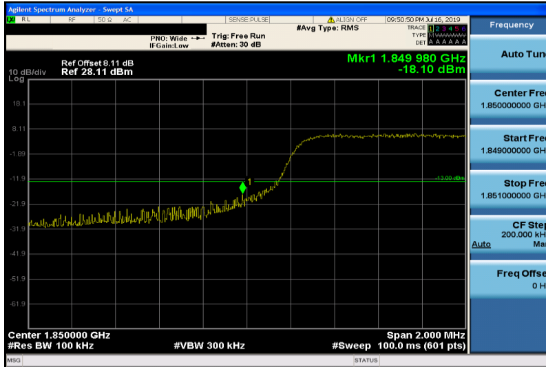
Band25-5MHz-QPSK-26065-25RB#0
