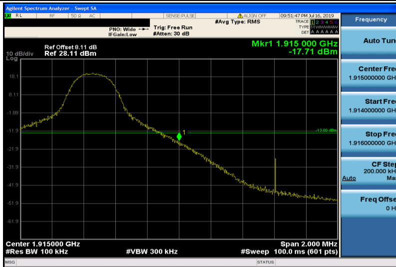
Band25-5MHz-QPSK-26665-1RB#24
