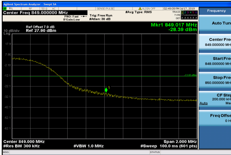
Band26-15MHz-16QAM-26965-75RB#0
