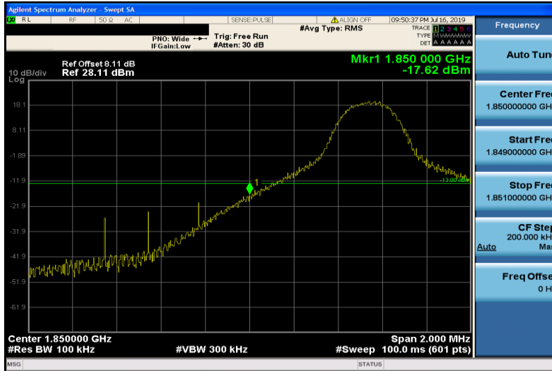
Band25-5MHz-16QAM-26065-1RB#0
