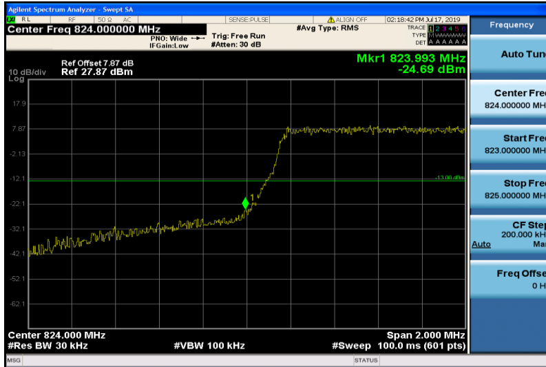
Band26-1.4MHz-16QAM-26797-6RB#0
