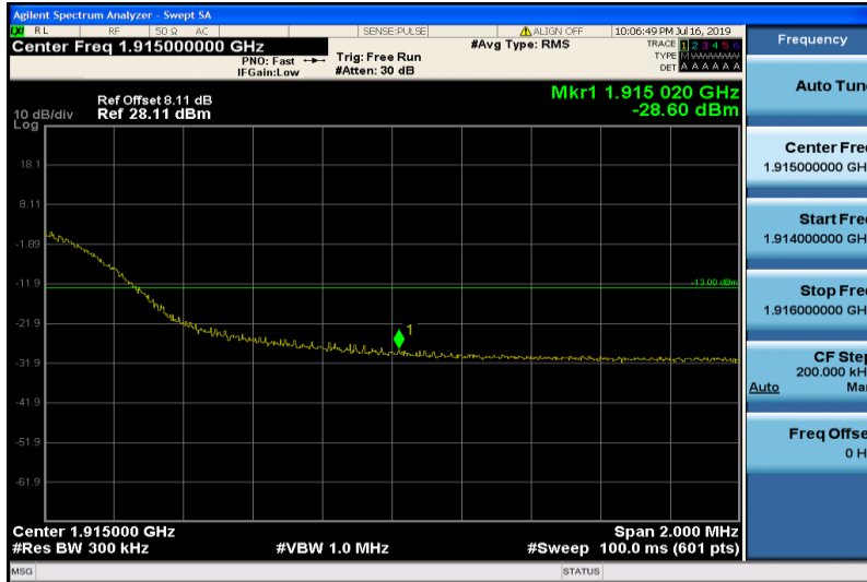
Band25-20MHz-16QAM-26590-100RB#0
