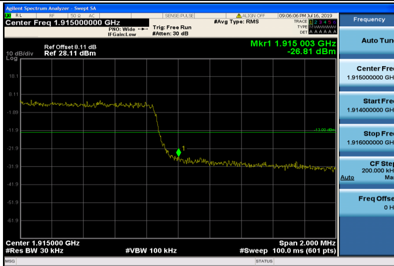
Band25-3MHz-16QAM-26675-15RB#0
