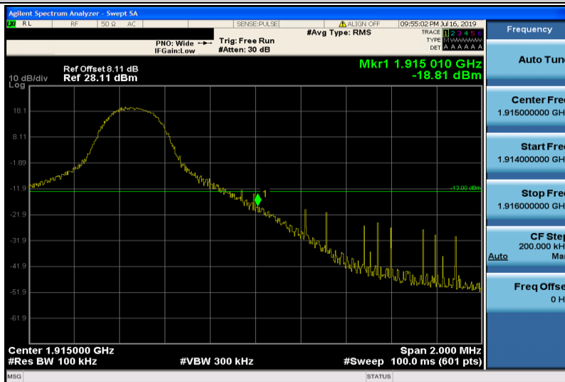
Band25-5MHz-16QAM-26665-1RB#24
