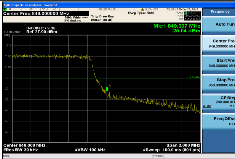
Band26-1.4MHz-QPSK-27033-6RB#0
