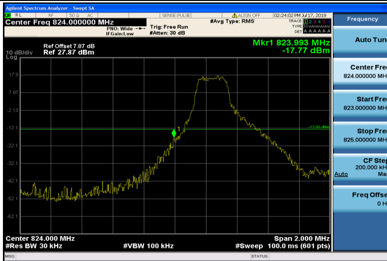
Band26-3MHz-16QAM-26805-1RB#0
