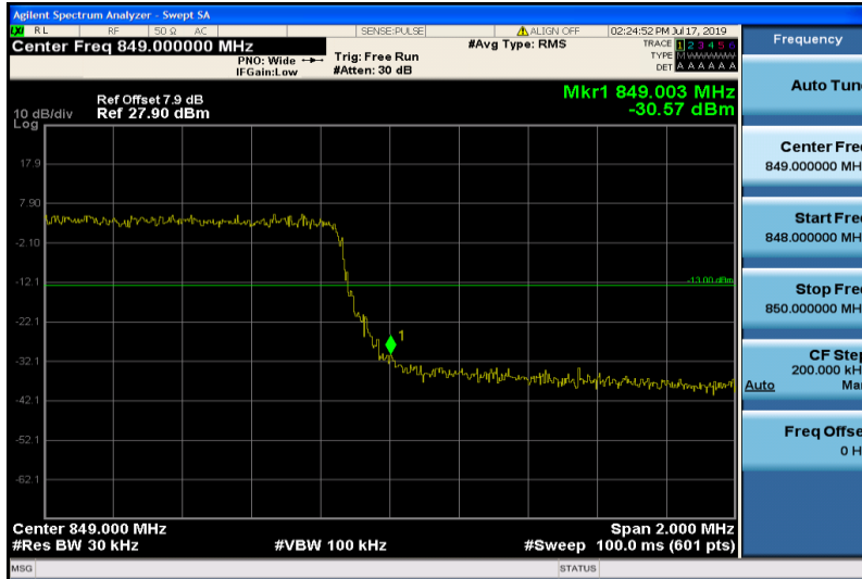
Band26-3MHz-QPSK-27025-15RB#0
