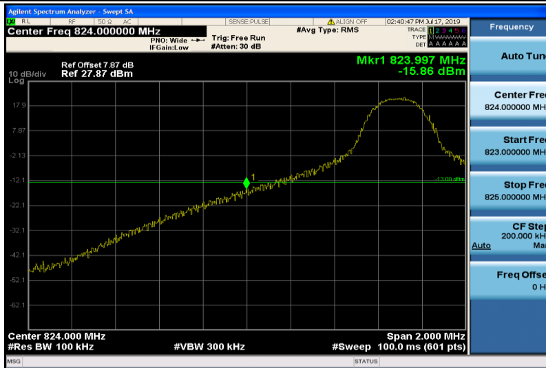
Band26-10MHz-QPSK-26840-1RB#0
