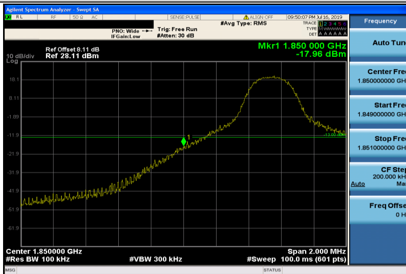
Band25-5MHz-QPSK-26065-1RB#0
