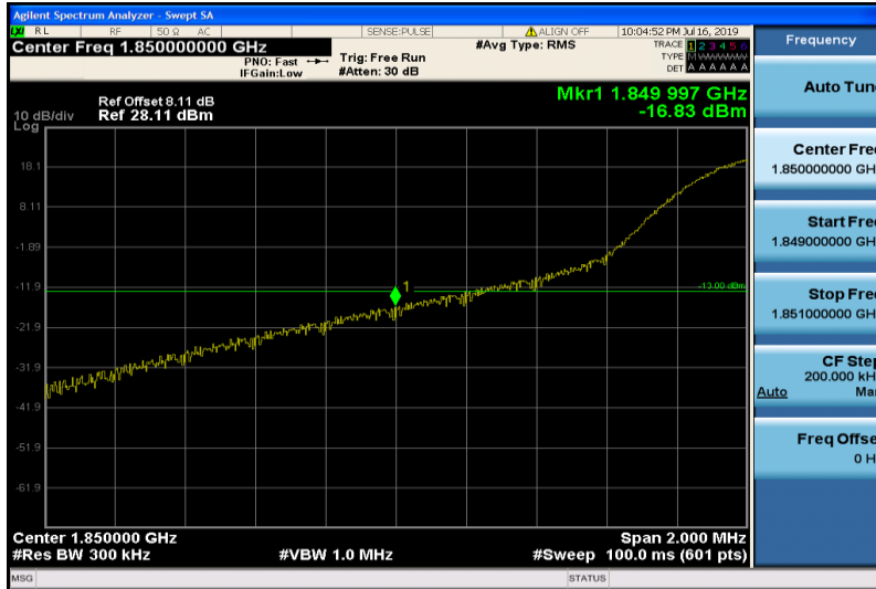
Band25-20MHz-16QAM-26140-1RB#0
