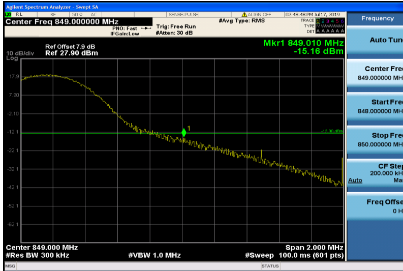
Band26-15MHz-16QAM-26965-1RB#74
