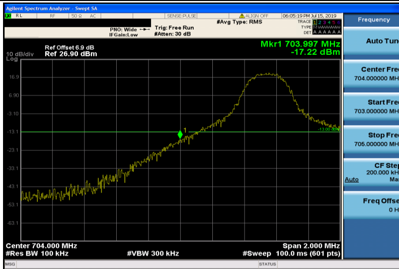
Band17-5MHz-16QAM-23755-1RB#0
