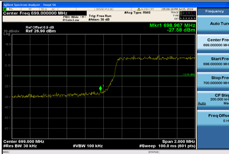
Band12-3MHz-QPSK-23025-15RB#0
