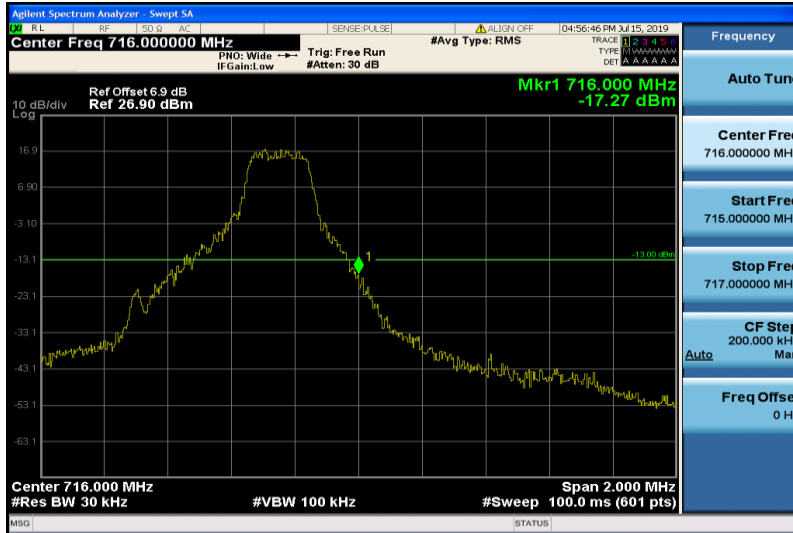
Band12-1.4MHz-QPSK-23173-1RB#5
