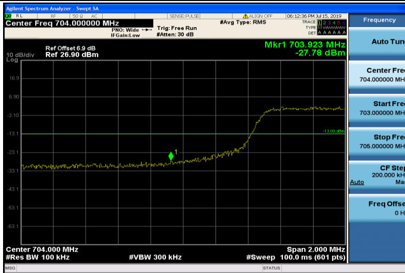
Band17-10MHz-16QAM-23780-50RB#0
