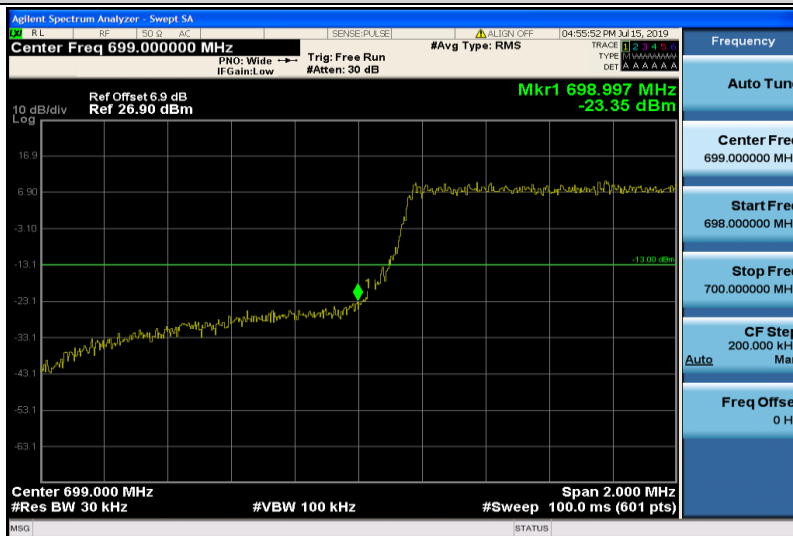
Band12-1.4MHz-QPSK-23017-6RB#0
