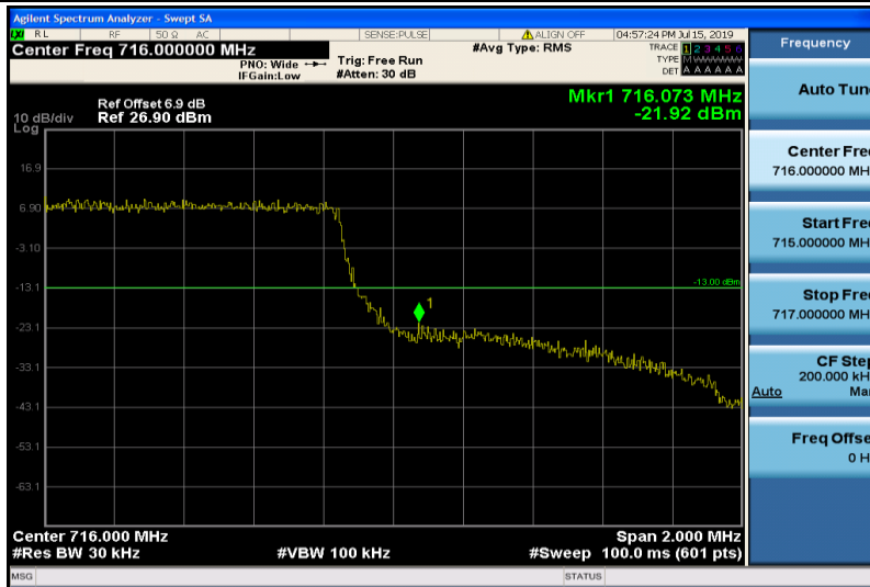
Band12-1.4MHz-QPSK-23173-6RB#0
