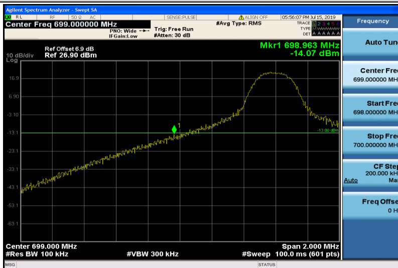
Band12-10MHz-QPSK-23060-1RB#0
