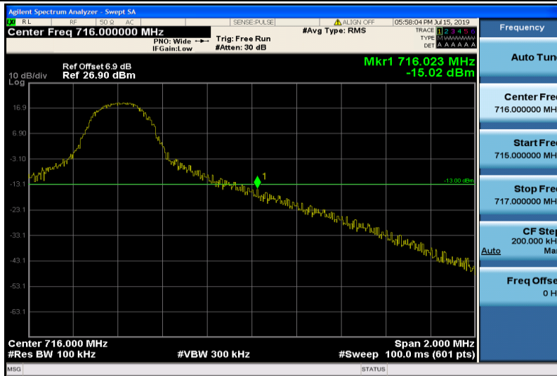
Band12-10MHz-16QAM-23130-1RB#49
