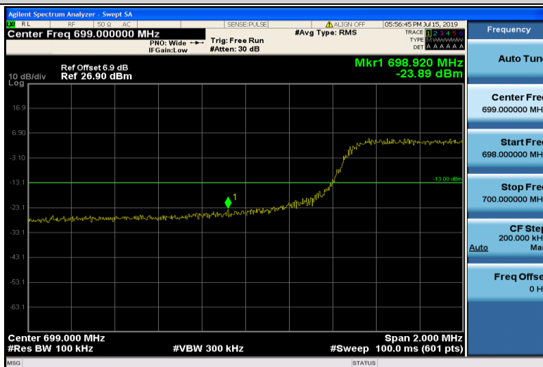
Band12-10MHz-QPSK-23060-50RB#0
