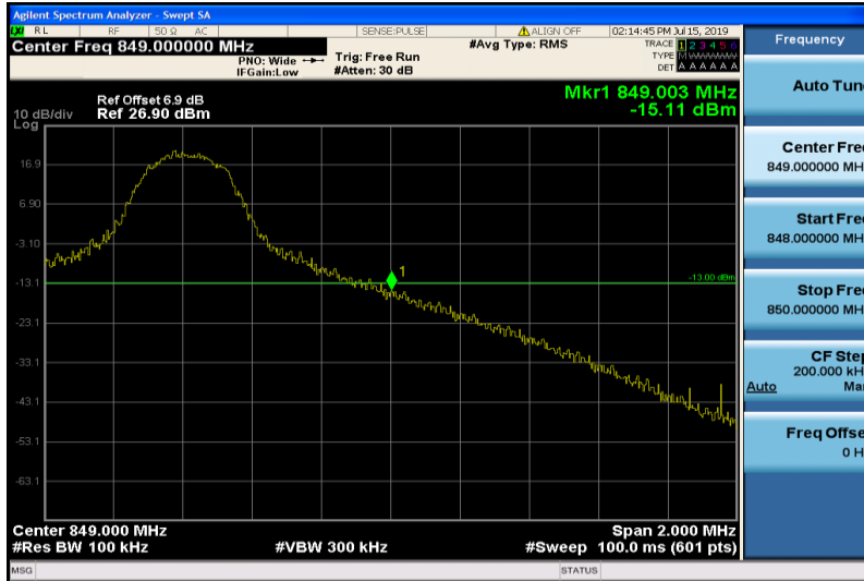
Band5-10MHz-16QAM-20600-1RB#49
