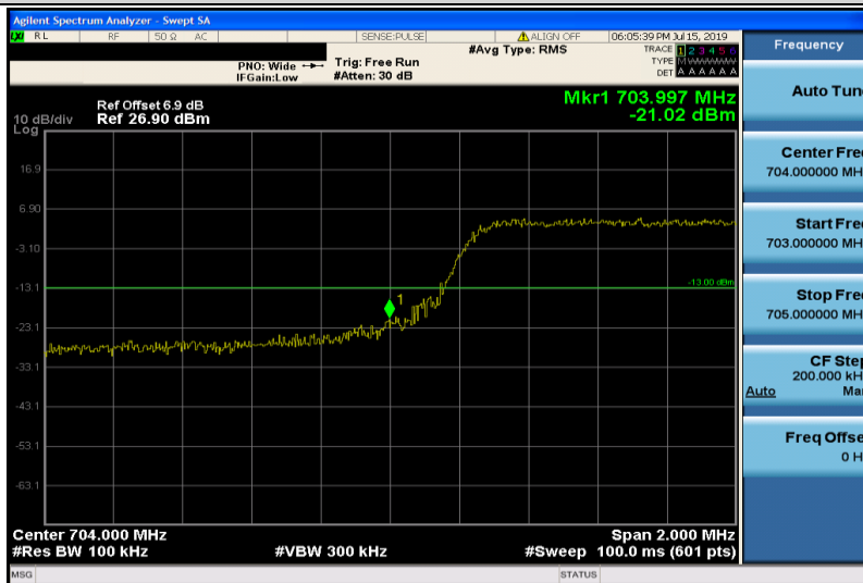
Band17-5MHz-16QAM-23755-25RB#0
