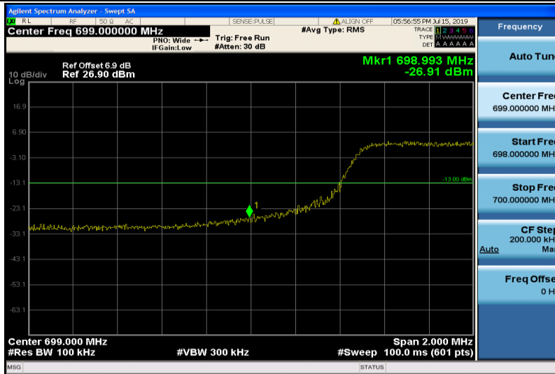
Band12-10MHz-16QAM-23060-50RB#0
