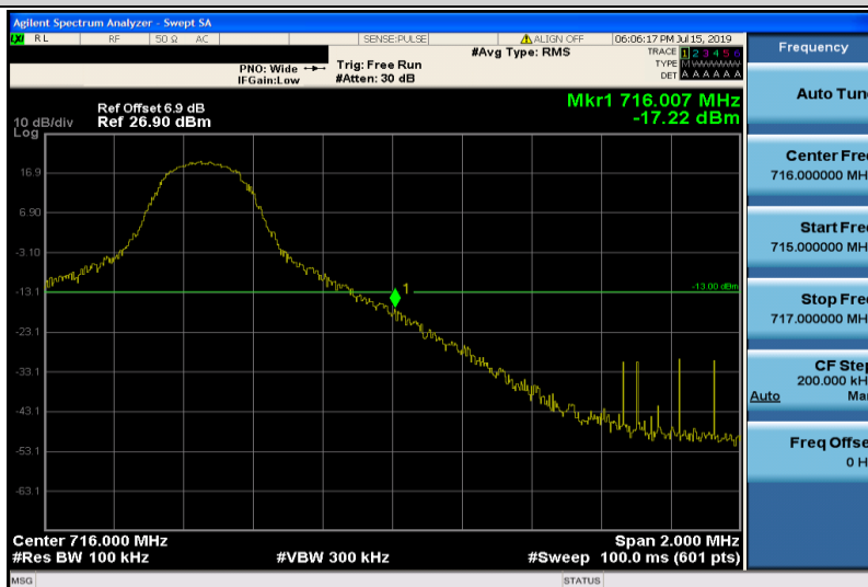
Band17-5MHz-QPSK-23825-1RB#24
