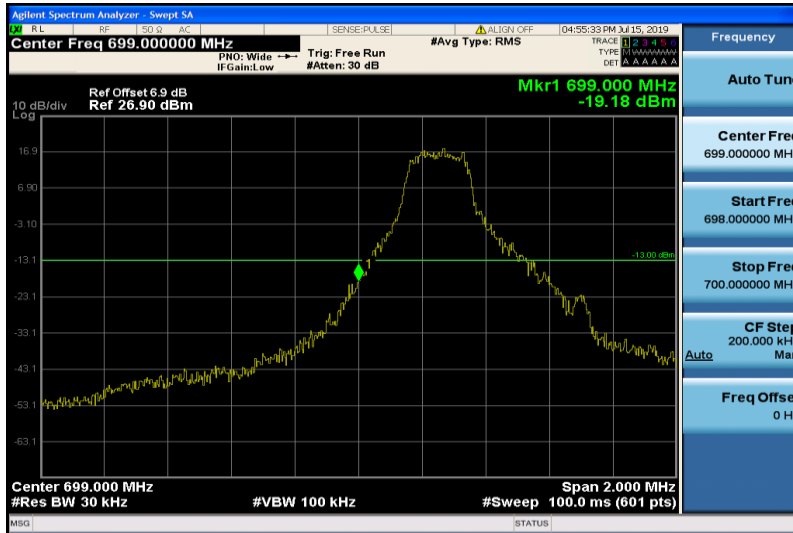
Band12-1.4MHz-QPSK-23017-1RB#0
