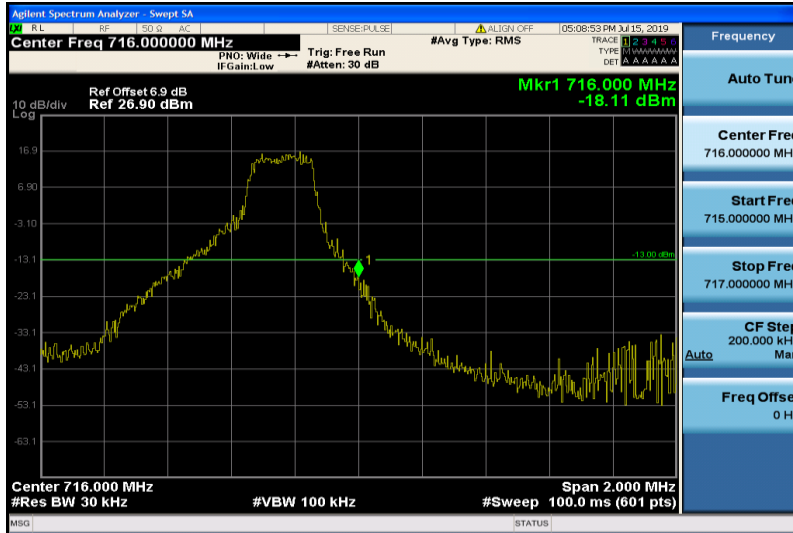
Band12-3MHz-16QAM-23165-1RB#14
