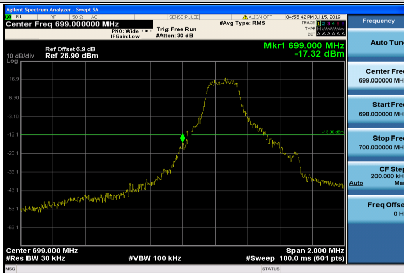
Band12-1.4MHz-16QAM-23017-1RB#0
