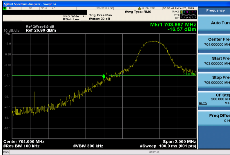
Band17-5MHz-QPSK-23755-1RB#0
