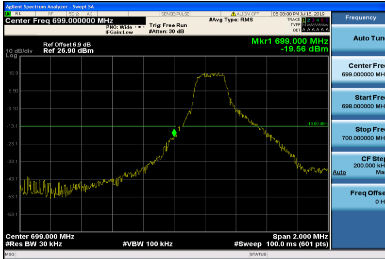
Band12-3MHz-QPSK-23025-1RB#0
