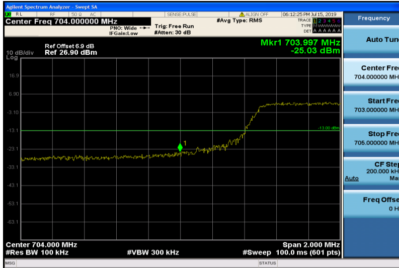
Band17-10MHz-QPSK-23780-50RB#0
