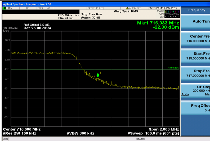
Band12-5MHz-16QAM-23155-25RB#0
