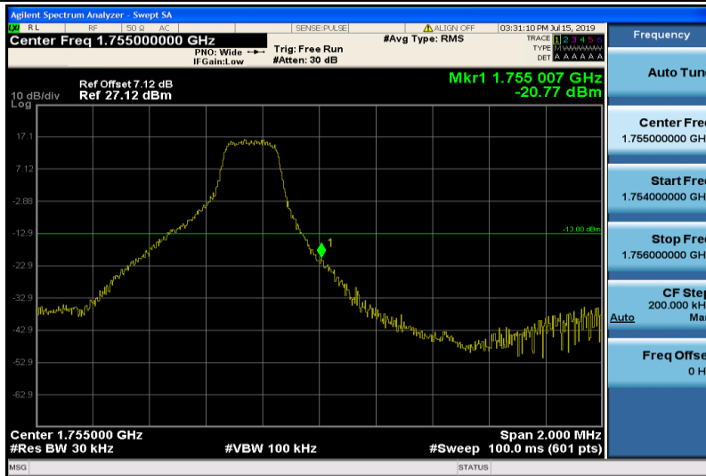
Band4-3MHz-QPSK-20385-1RB#14
