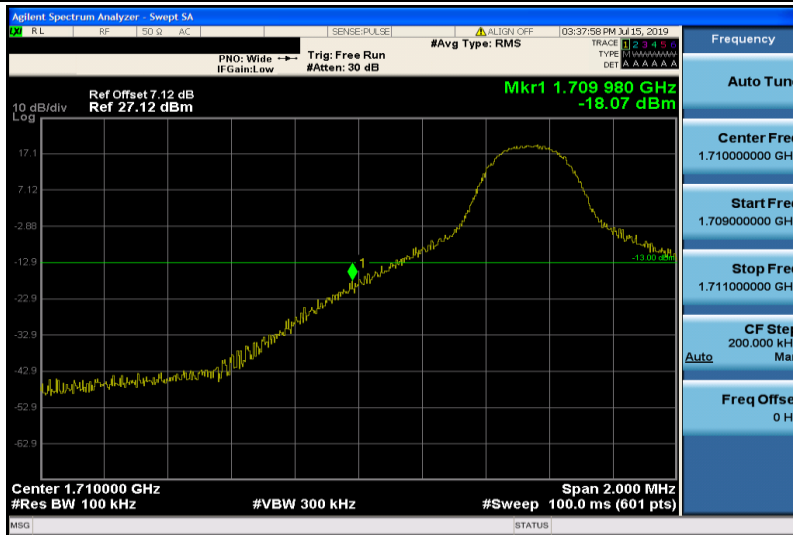
Band4-5MHz-QPSK-19975-1RB#0
