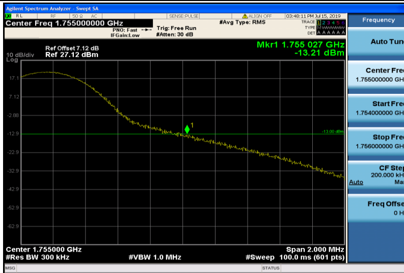
Band4-15MHz-QPSK-20325-1RB#74
