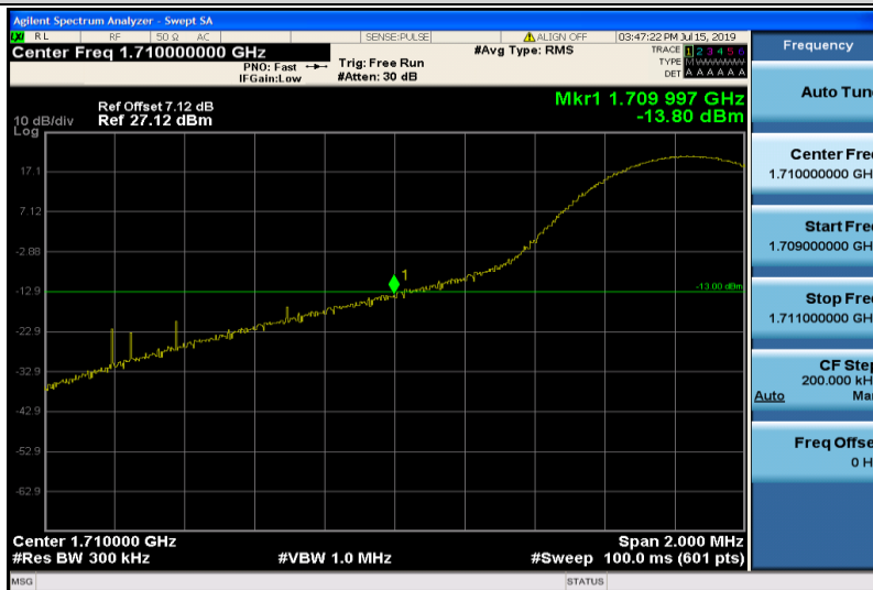
Band4-15MHz-QPSK-20025-1RB#0
