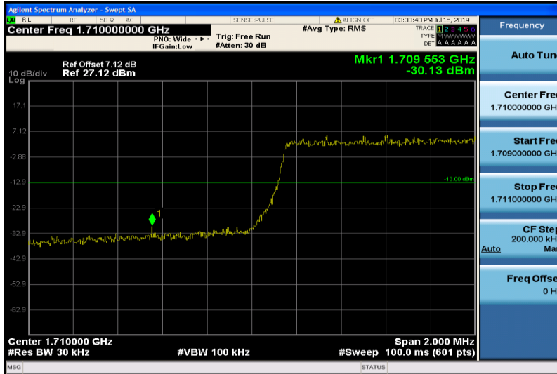
Band4-3MHz-QPSK-19965-15RB#0
