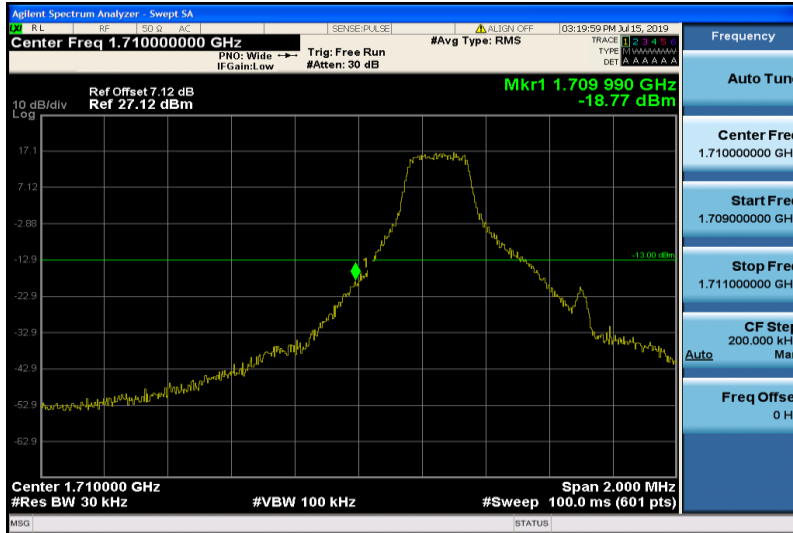
Band4-1.4MHz-QPSK-19957-1RB#0
