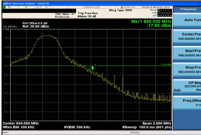
Band5-5MHz-QPSK-20625-1RB#24
