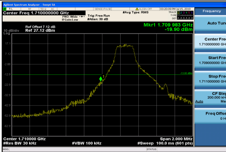
Band4-1.4MHz-16QAM-19957-1RB#0
