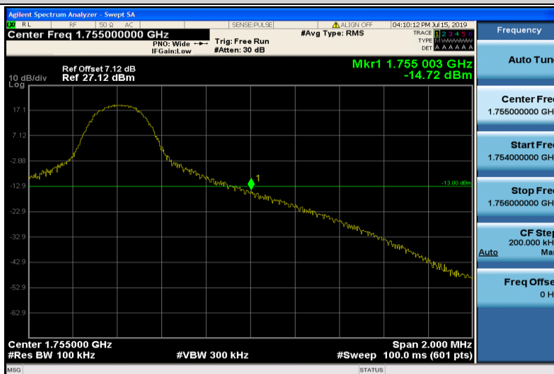
Band4-10MHz-QPSK-20350-1RB#49
