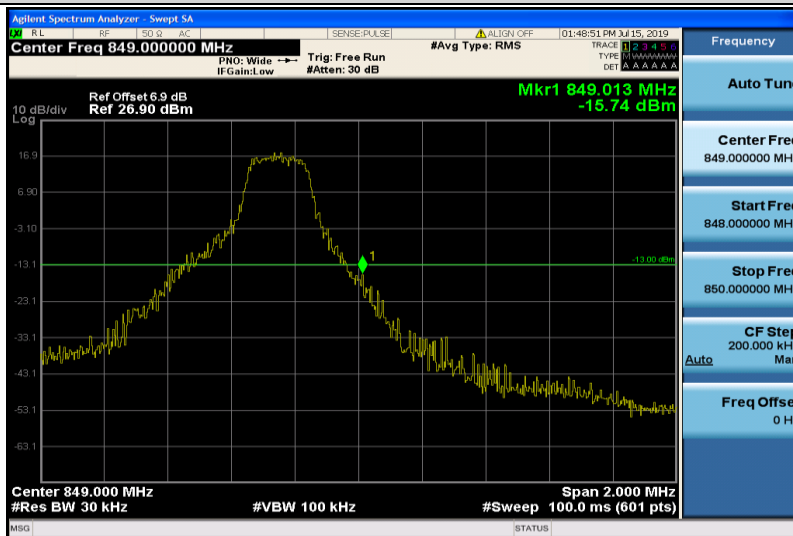
Band5-1.4MHz-QPSK-20643-1RB#5
