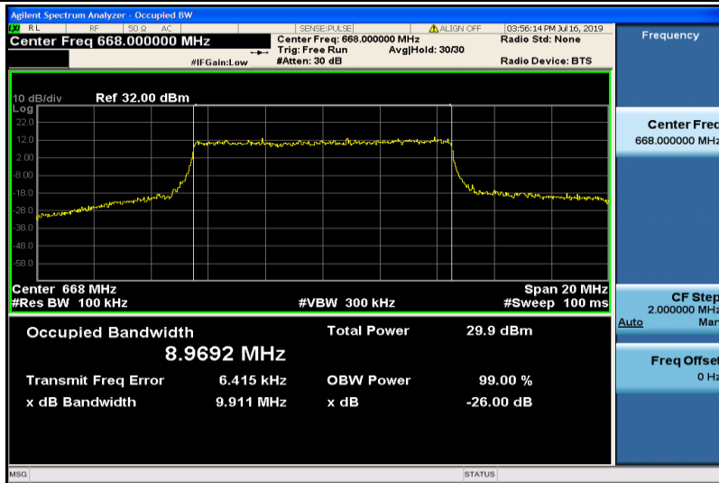
Band71-10MHz-QPSK-133172-50RB#0-8.9692
