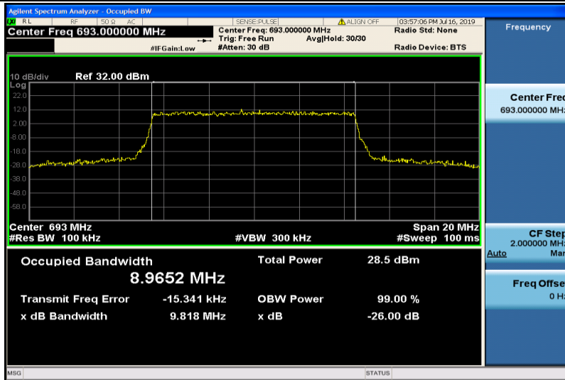
Band71-10MHz-16QAM-133422-50RB#0-8.9652
