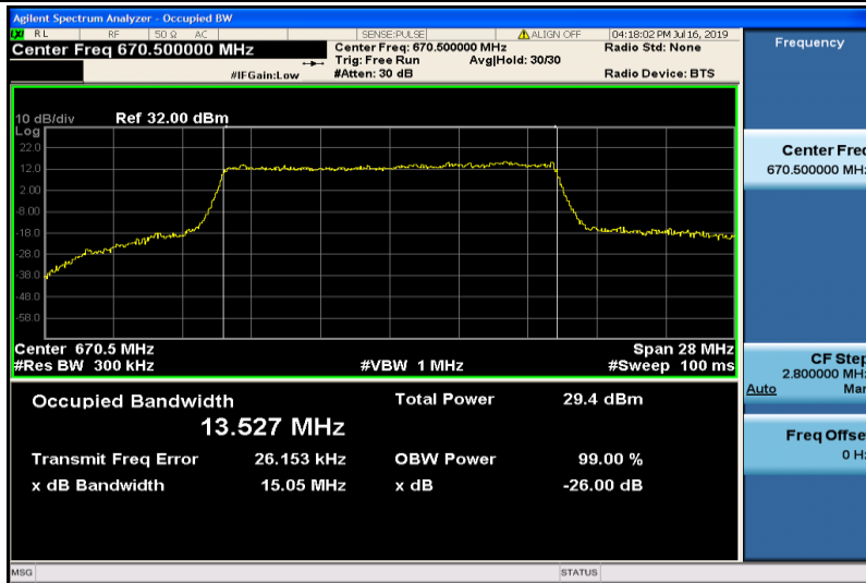
Band71-15MHz-16QAM-133197-75RB#0-13.527
