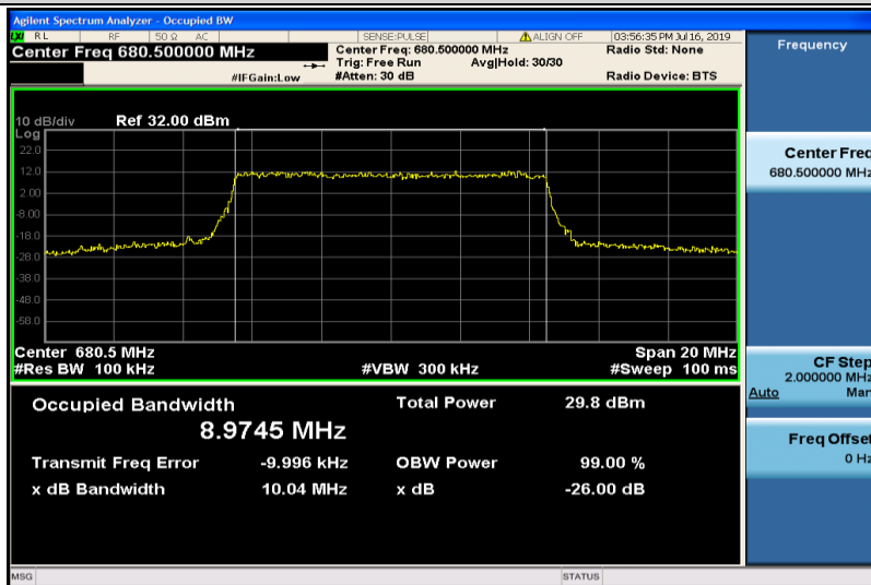
Band71-10MHz-QPSK-133297-50RB#0-8.9745
