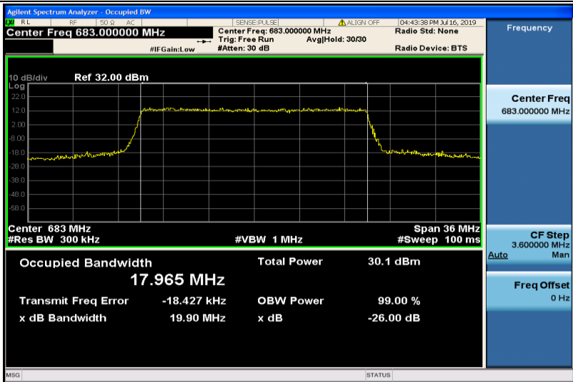
Band71-20MHz-QPSK-133322-100RB#0-17.965
