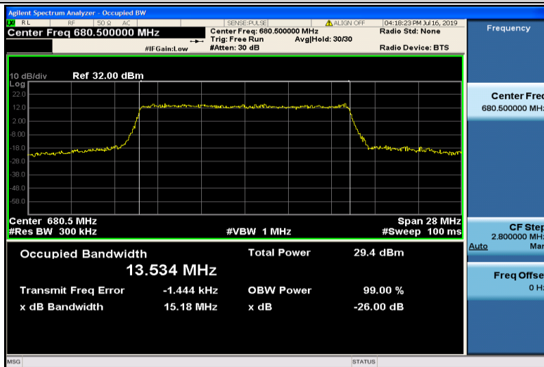
Band71-15MHz-16QAM-133297-75RB#0-13.534
