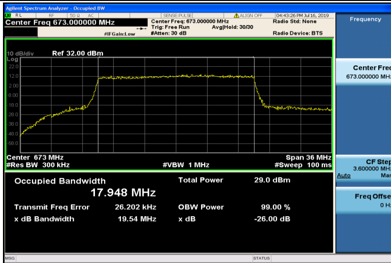
Band71-20MHz-16QAM-133222-100RB#0-17.948
