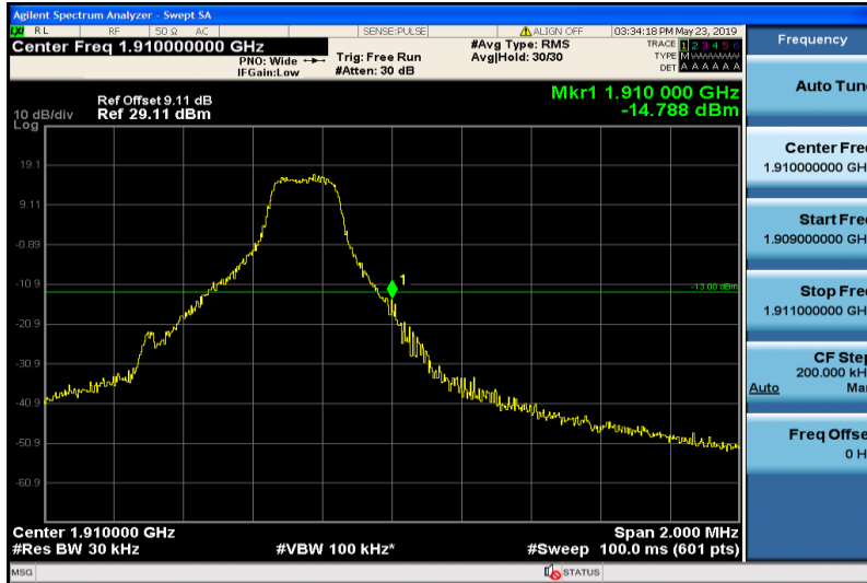
Band2-1.4MHz-16QAM-19193-1RB#5
