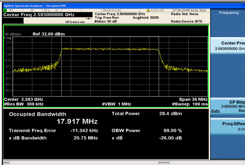
Band41-20MHz-16QAM-40620-100RB#0-17.917
