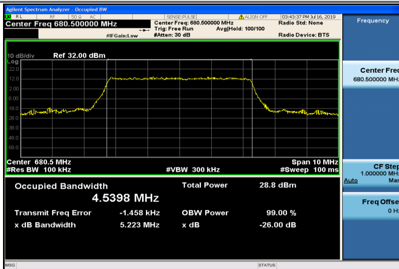
Band71-5MHz-16QAM-133297-25RB#0-4.5398
