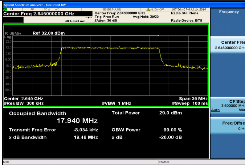
Band41-20MHz-QPSK-41140-100RB#0-17.940
