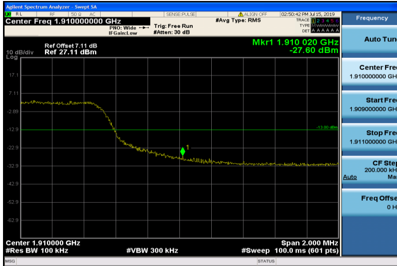
Band2-10MHz-QPSK-19150-50RB#0
