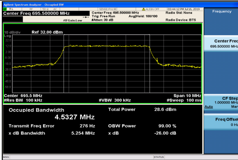
Band71-5MHz-16QAM-133447-25RB#0-4.5327
