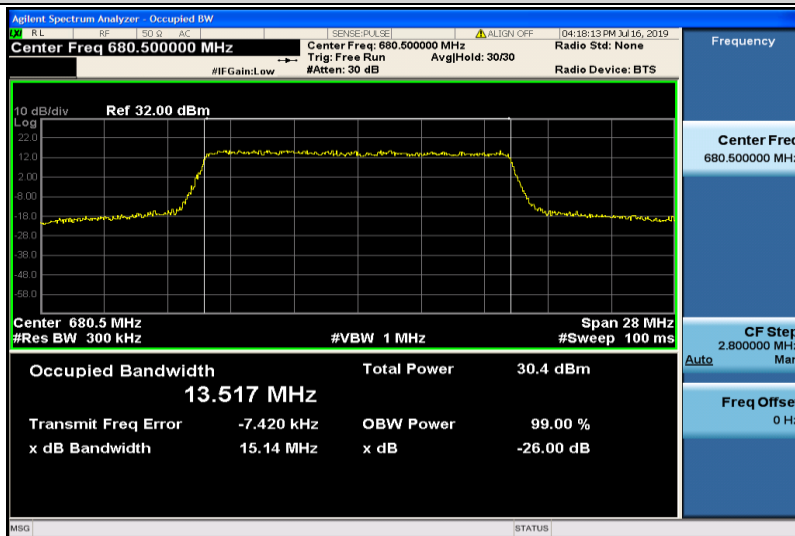
Band71-15MHz-QPSK-133297-75RB#0-13.517
