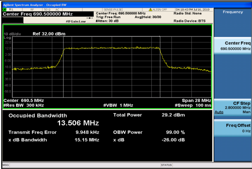
Band71-15MHz-16QAM-133397-75RB#0-13.506
