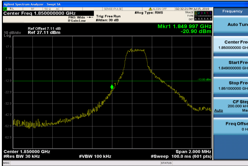
Band2-3MHz-16QAM-18615-1RB#0
