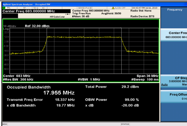
Band71-20MHz-16QAM-133322-100RB#0-17.955
