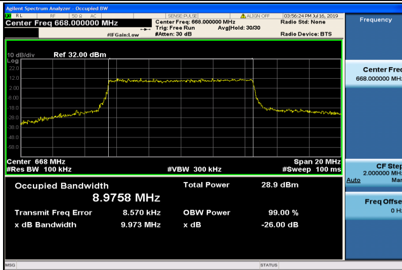
Band71-10MHz-16QAM-133172-50RB#0-8.9758
