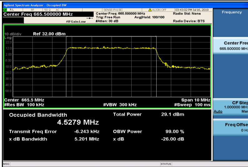
Band71-5MHz-16QAM-133147-25RB#0-4.5279
