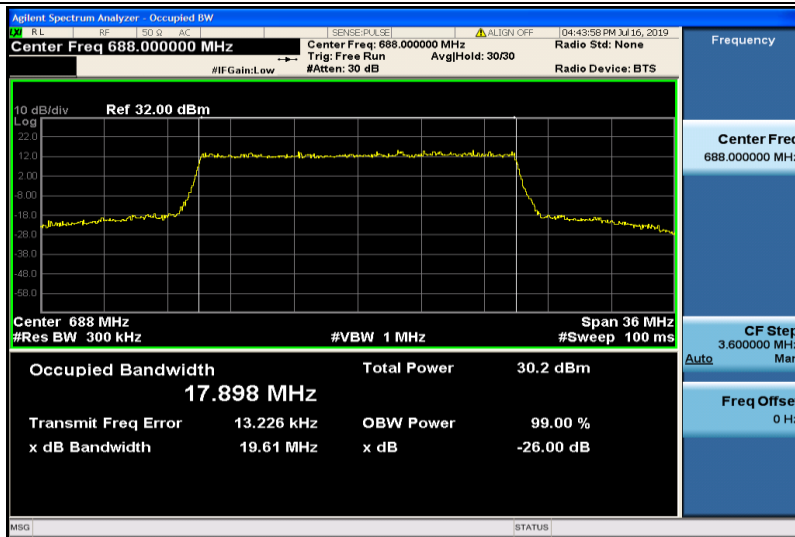
Band71-20MHz-QPSK-133372-100RB#0-17.898
