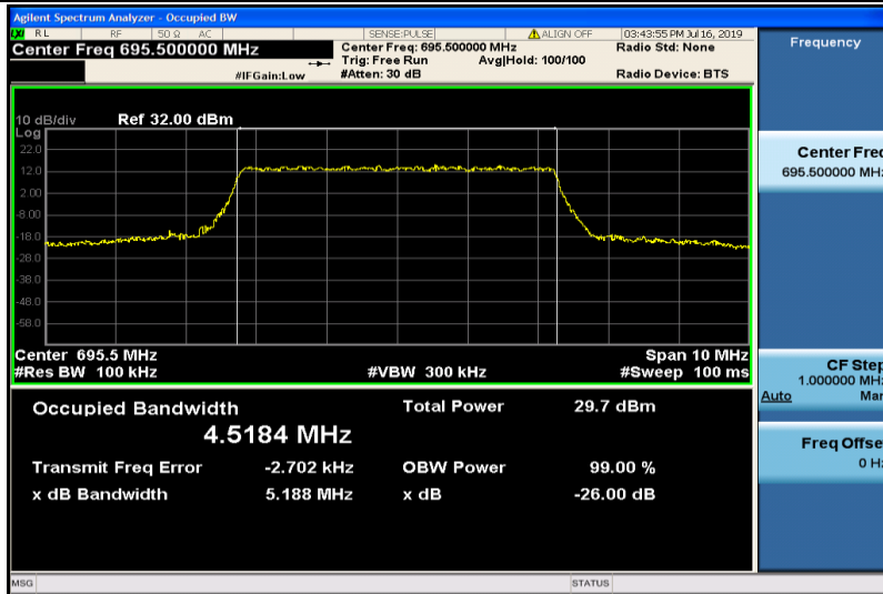
Band71-5MHz-QPSK-133447-25RB#0-4.5184
