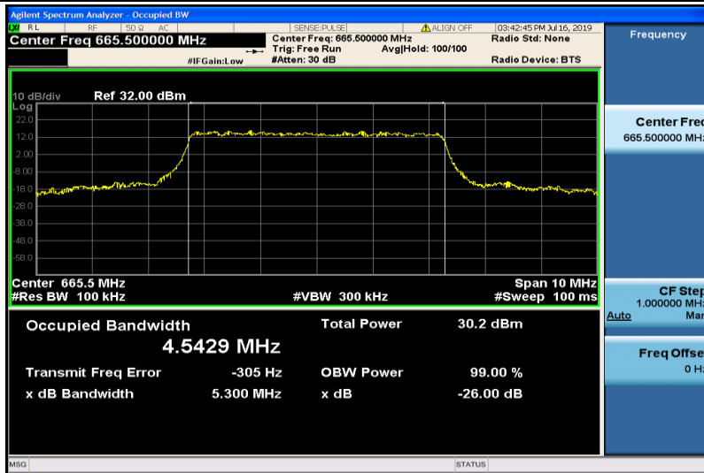
Band71-5MHz-QPSK-133147-25RB#0-4.5429
