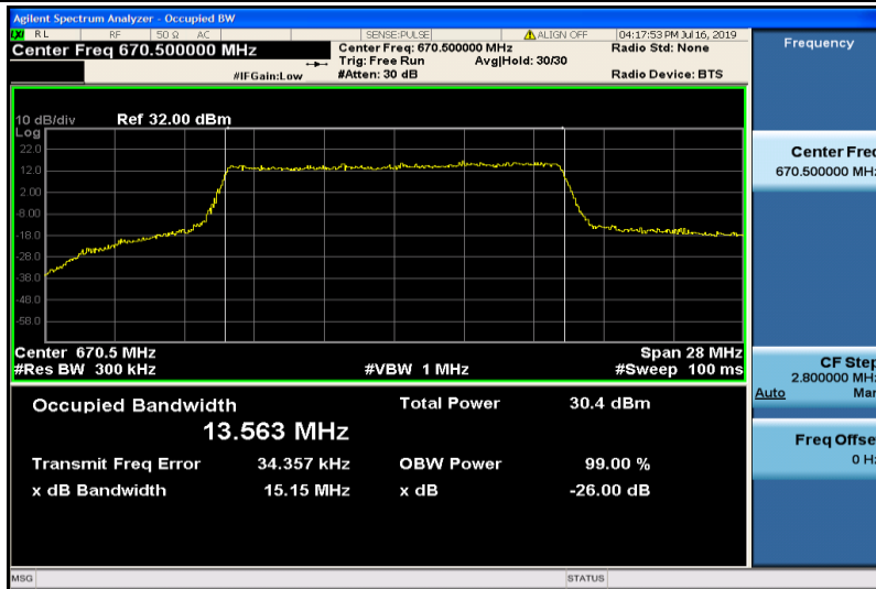
Band71-15MHz-QPSK-133197-75RB#0-13.563
