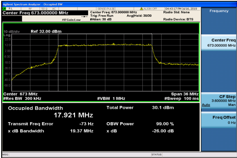
Band71-20MHz-QPSK-133222-100RB#0-17.921
