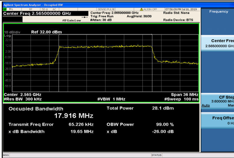
Band41-20MHz-16QAM-40340-100RB#0-17.916
