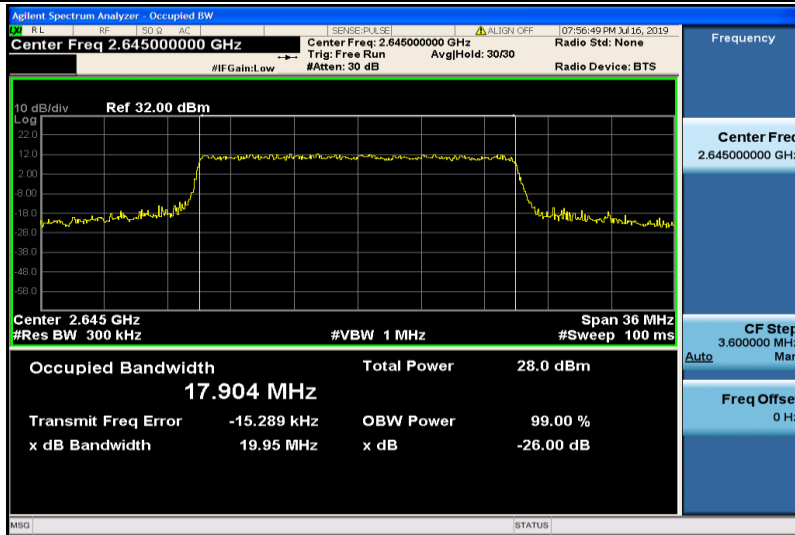
Band41-20MHz-16QAM-41140-100RB#0-17.904
