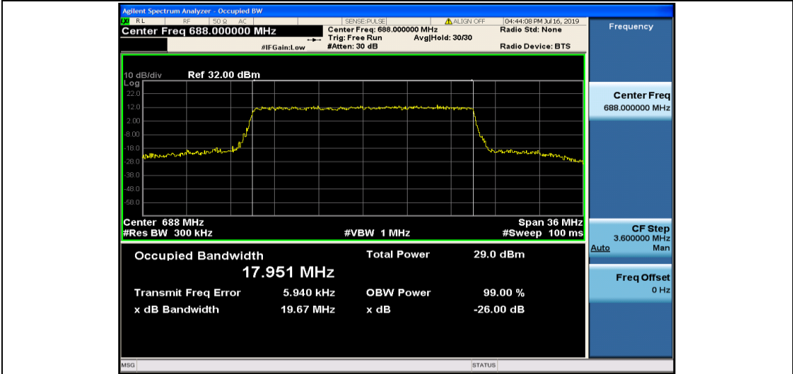
Band71-20MHz-16QAM-133372-100RB#0-17.951
