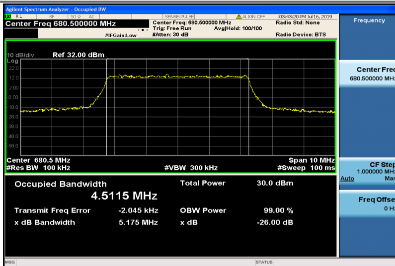
Band71-5MHz-QPSK-133297-25RB#0-4.5115
