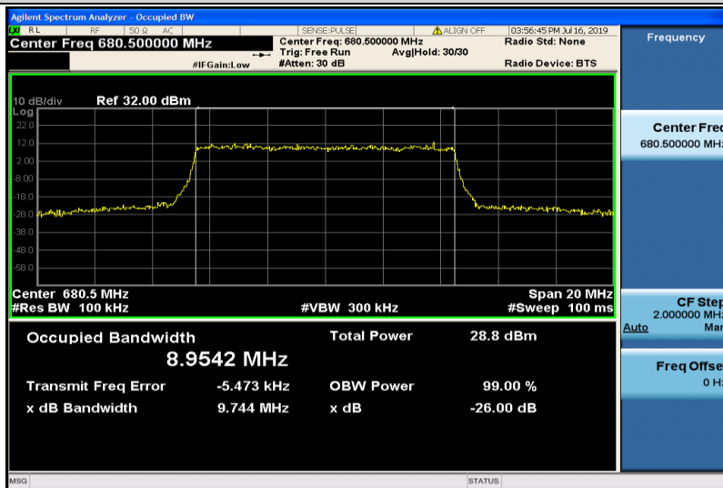
Band71-10MHz-16QAM-133297-50RB#0-8.9542
