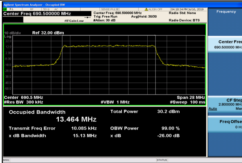
Band71-15MHz-QPSK-133397-75RB#0-13.464
