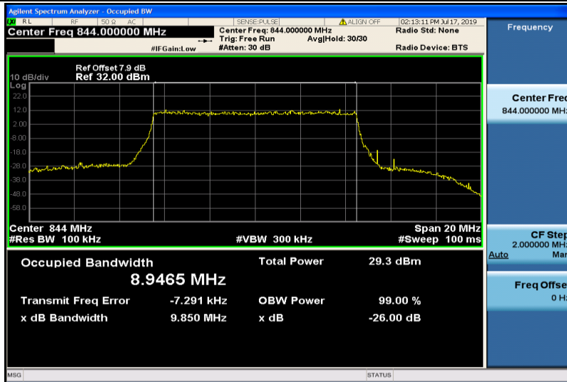
Band26-10MHz-16QAM-26990-50RB#0-8.9465
