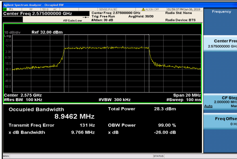
Band38-10MHz-16QAM-37800-50RB#0-8.9462
