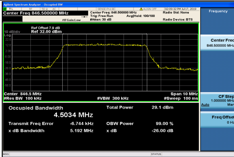
Band26-5MHz-16QAM-27015-25RB#0-4.5034
