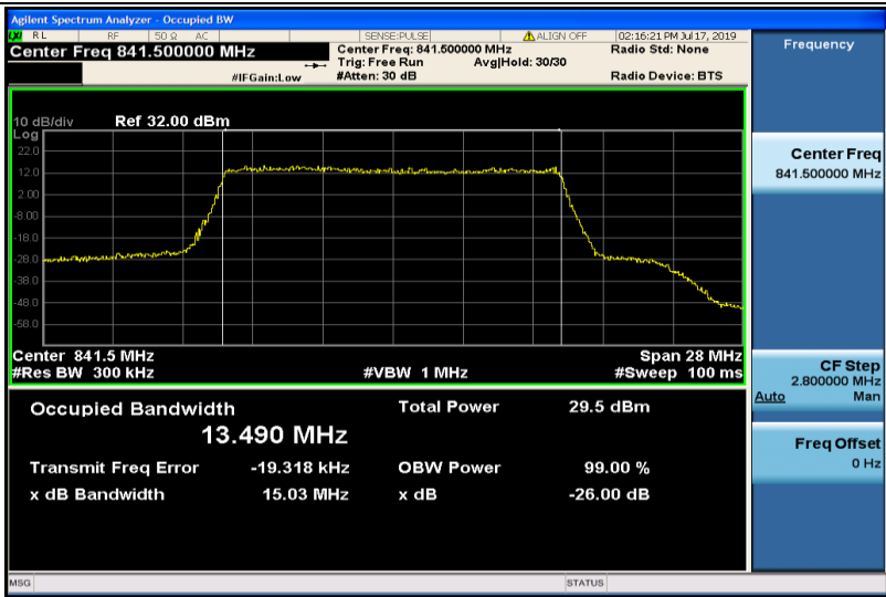
Band26-15MHz-16QAM-26965-75RB#0-13.490
