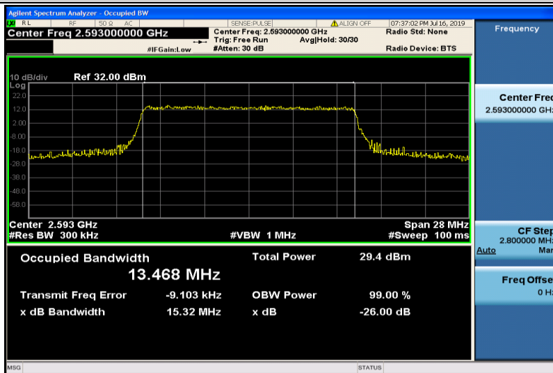
Band41-15MHz-QPSK-40620-75RB#0-13.468
