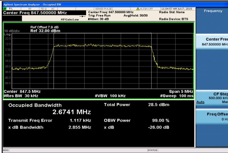
Band26-3MHz-16QAM-27025-15RB#0-2.6741
