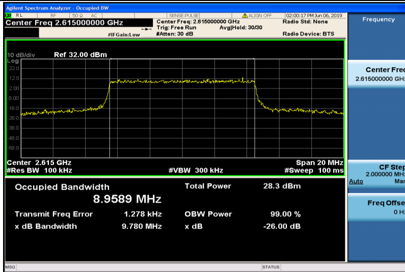
Band38-10MHz-16QAM-38200-50RB#0-8.9589
