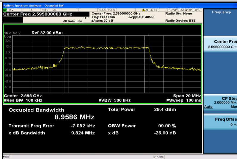
Band38-10MHz-QPSK-38000-50RB#0-8.9586
