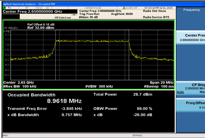
Band41-10MHz-QPSK-41190-50RB#0-8.9618
