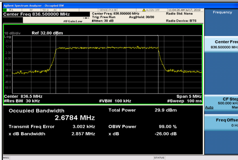
Band26-3MHz-QPSK-26915-15RB#0-2.6784
