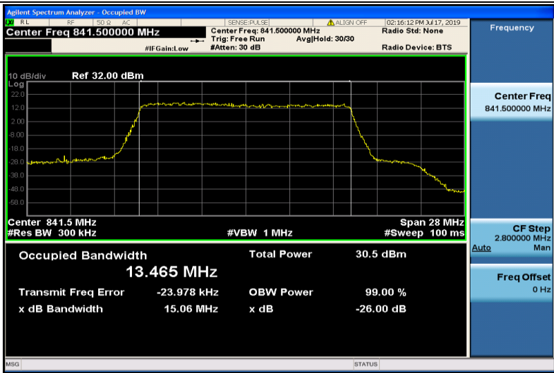
Band26-15MHz-QPSK-26965-75RB#0-13.465
