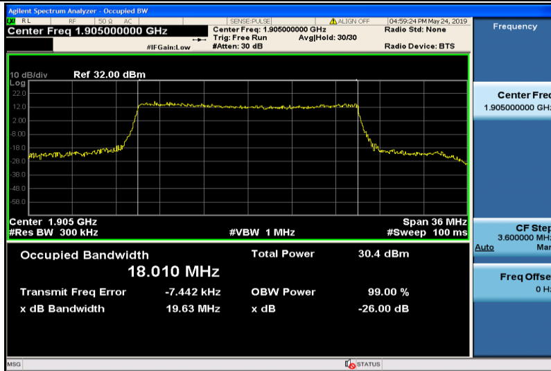
Band25-20MHz-16QAM-26590-100RB#0-18.010
