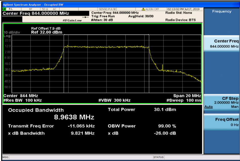
Band26-10MHz-QPSK-26990-50RB#0-8.9638
