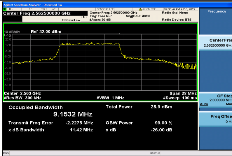
Band41-15MHz-QPSK-40315-75RB#0-9.1532
