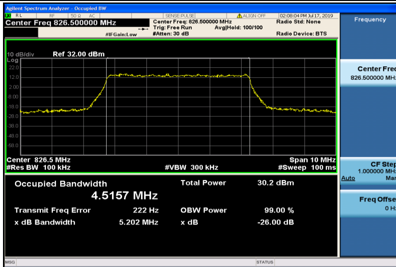
Band26-5MHz-QPSK-26815-25RB#0-4.5157
