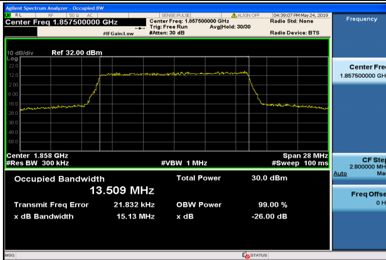
Band25-15MHz-16QAM-26115-75RB#0-13.509
