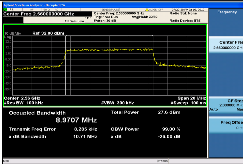
Band41-10MHz-16QAM-40290-50RB#0-8.9707
