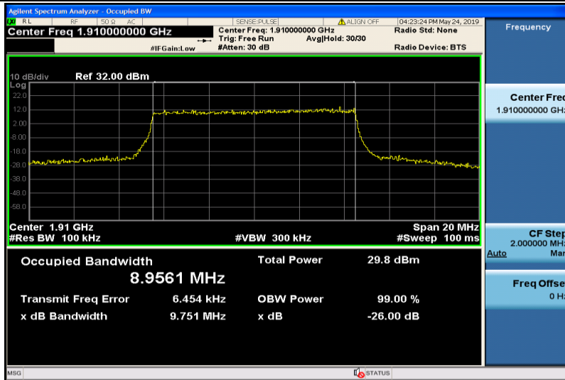
Band25-10MHz-16QAM-26640-50RB#0-8.9561
