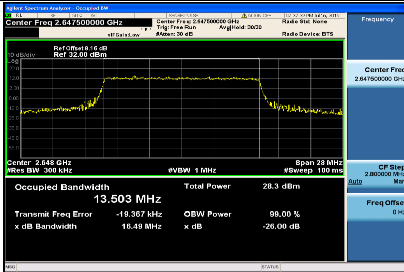
Band41-15MHz-16QAM-41165-75RB#0-13.503
