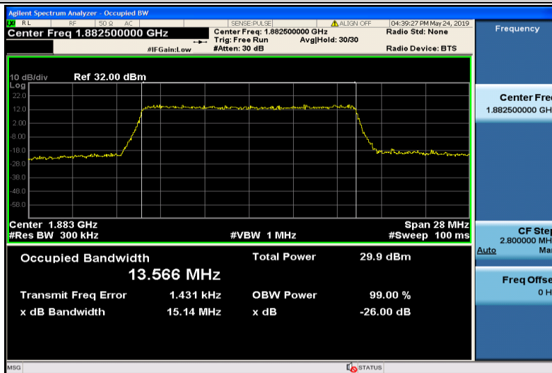
Band25-15MHz-16QAM-26365-75RB#0-13.566
