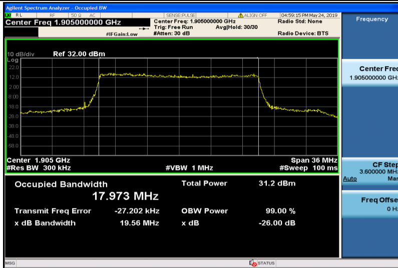
Band25-20MHz-QPSK-26590-100RB#0-17.973
