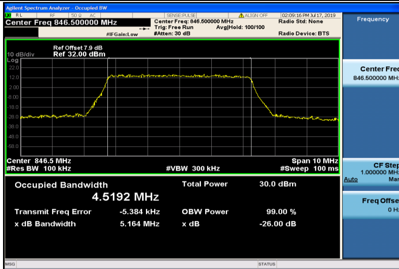
Band26-5MHz-QPSK-27015-25RB#0-4.5192
