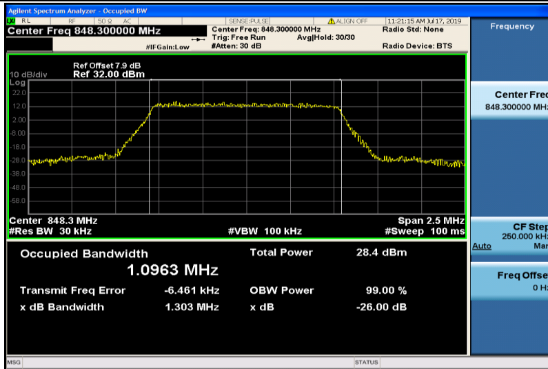
Band26-1.4MHz-16QAM-27033-6RB#0-1.0963
