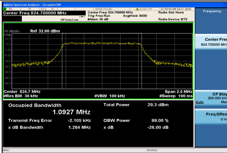
Band26-1.4MHz-QPSK-26797-6RB#0-1.0927
