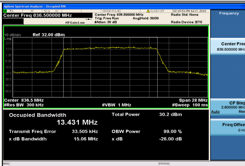
Band26-15MHz-QPSK-26915-75RB#0-13.431
