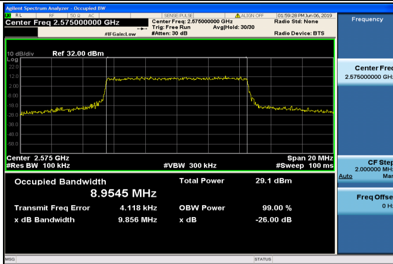
Band38-10MHz-QPSK-37800-50RB#0-8.9545
