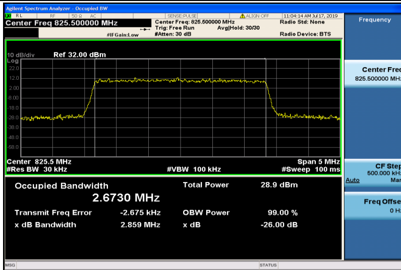
Band26-3MHz-16QAM-26805-15RB#0-2.6730
