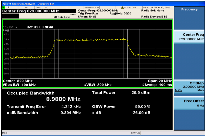
Band26-10MHz-16QAM-26840-50RB#0-8.9809
