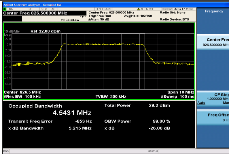
Band26-5MHz-16QAM-26815-25RB#0-4.5431
