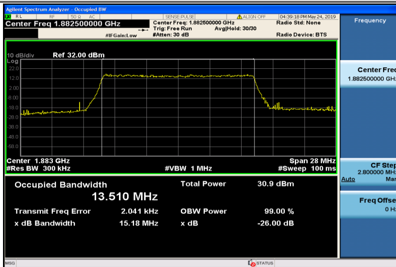
Band25-15MHz-QPSK-26365-75RB#0-13.510
