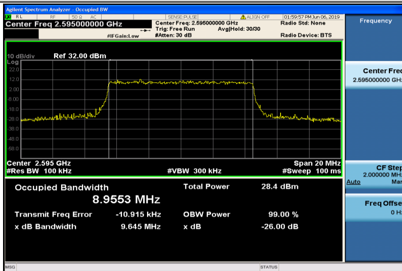
Band38-10MHz-16QAM-38000-50RB#0-8.9553
