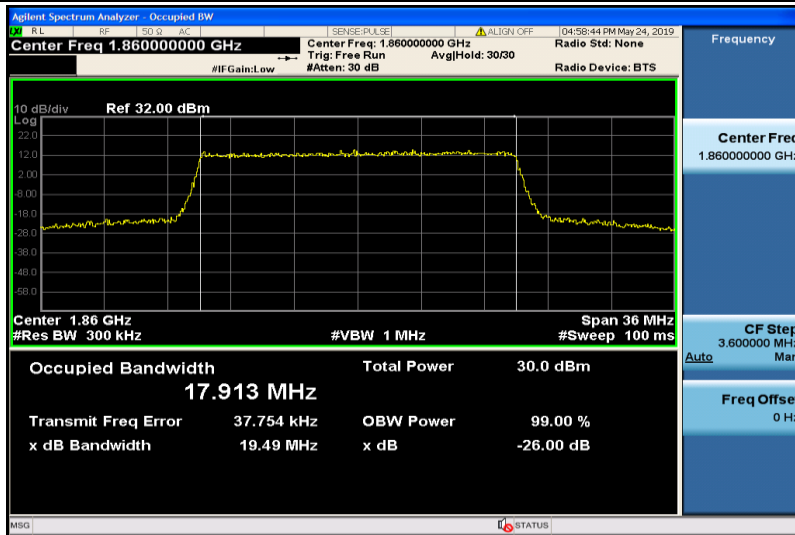
Band25-20MHz-16QAM-26140-100RB#0-17.913
