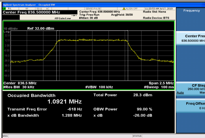
Band26-1.4MHz-16QAM-26915-6RB#0-1.0921
