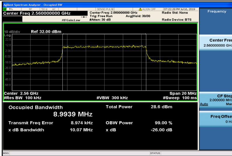
Band41-10MHz-QPSK-40290-50RB#0-8.9939
