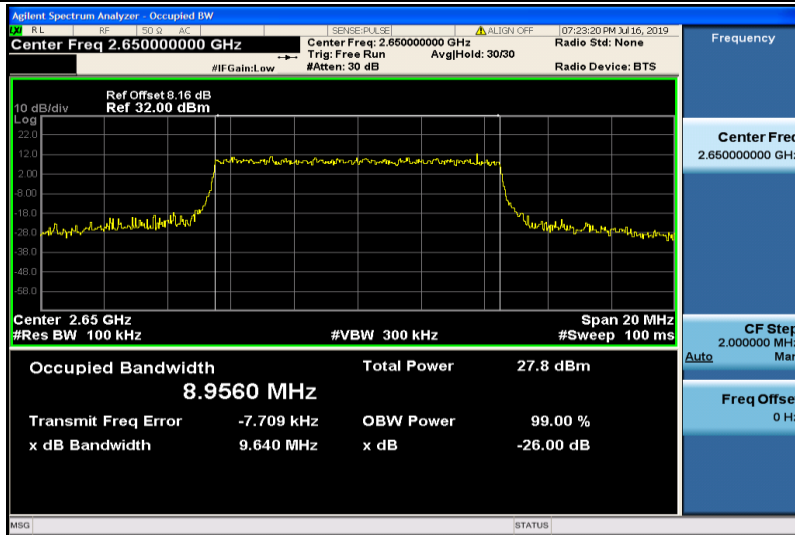
Band41-10MHz-16QAM-41190-50RB#0-8.9560
