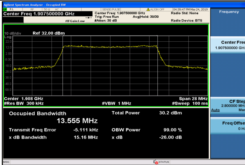
Band25-15MHz-16QAM-26615-75RB#0-13.555
