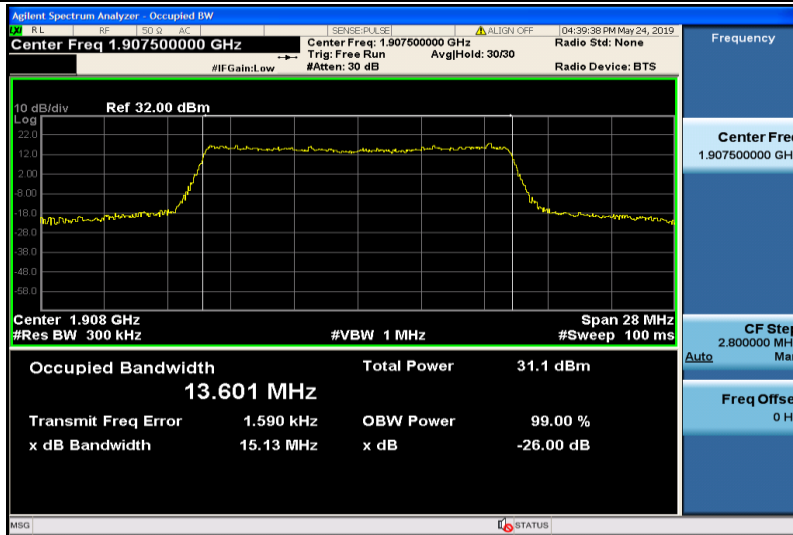
Band25-15MHz-QPSK-26615-75RB#0-13.601
