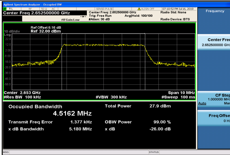
Band41-5MHz-16QAM-41215-25RB#0-4.5162
