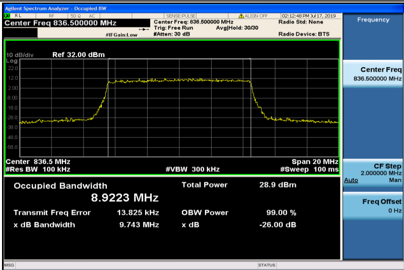
Band26-10MHz-16QAM-26915-50RB#0-8.9223
