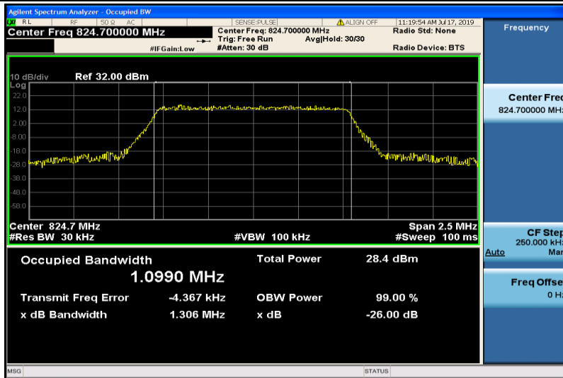
Band26-1.4MHz-16QAM-26797-6RB#0-1.0990
