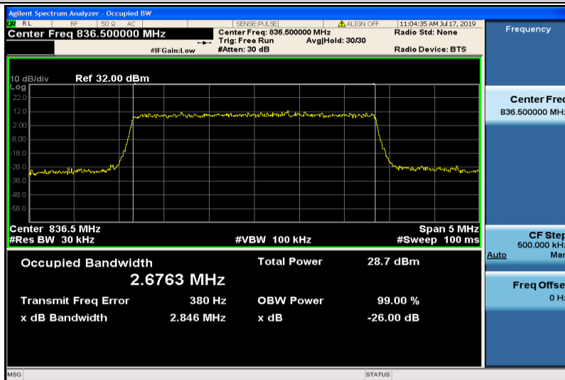
Band26-3MHz-16QAM-26915-15RB#0-2.6763
