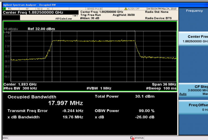
Band25-20MHz-16QAM-26365-100RB#0-17.997
