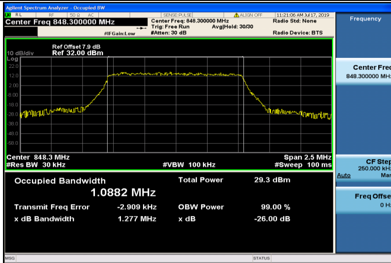
Band26-1.4MHz-QPSK-27033-6RB#0-1.0882
