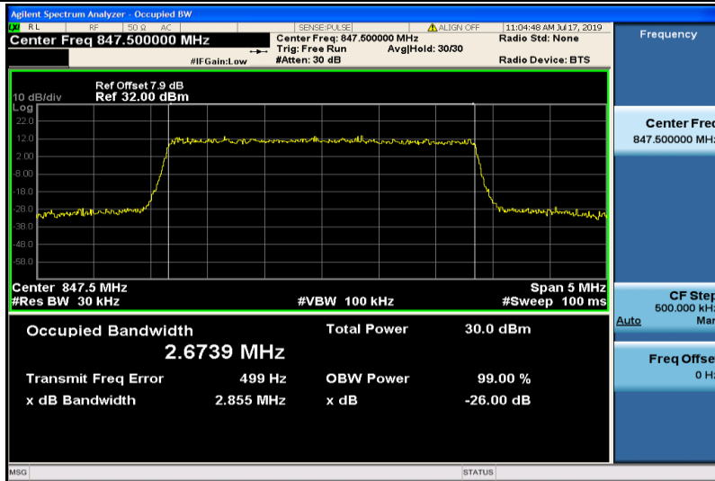
Band26-3MHz-QPSK-27025-15RB#0-2.6739
