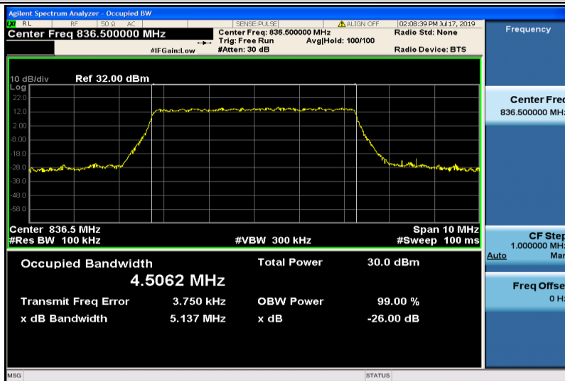
Band26-5MHz-QPSK-26915-25RB#0-4.5062
