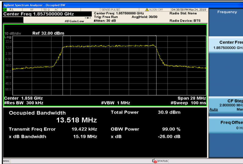
Band25-15MHz-QPSK-26115-75RB#0-13.518
