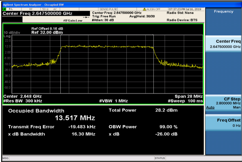
Band41-15MHz-QPSK-41165-75RB#0-13.517
