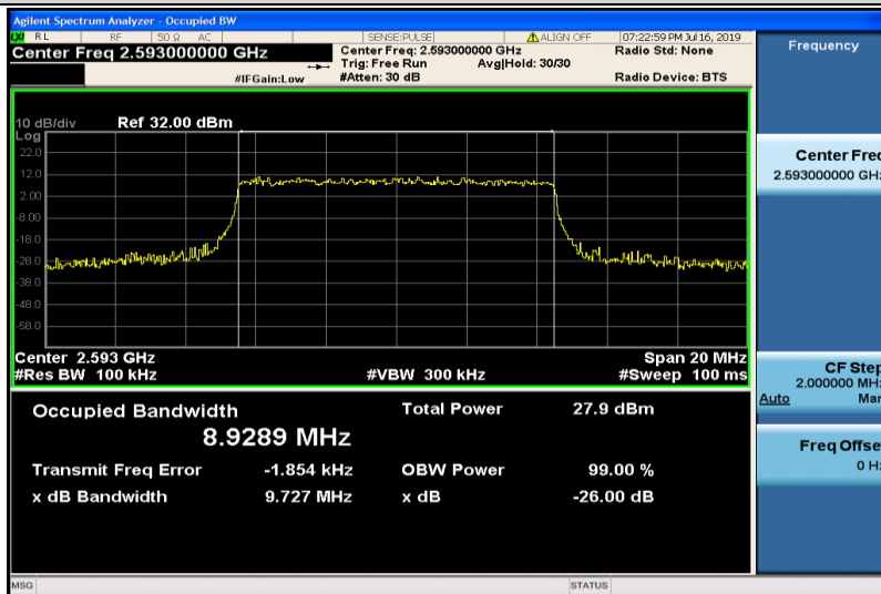
Band41-10MHz-16QAM-40620-50RB#0-8.9289
