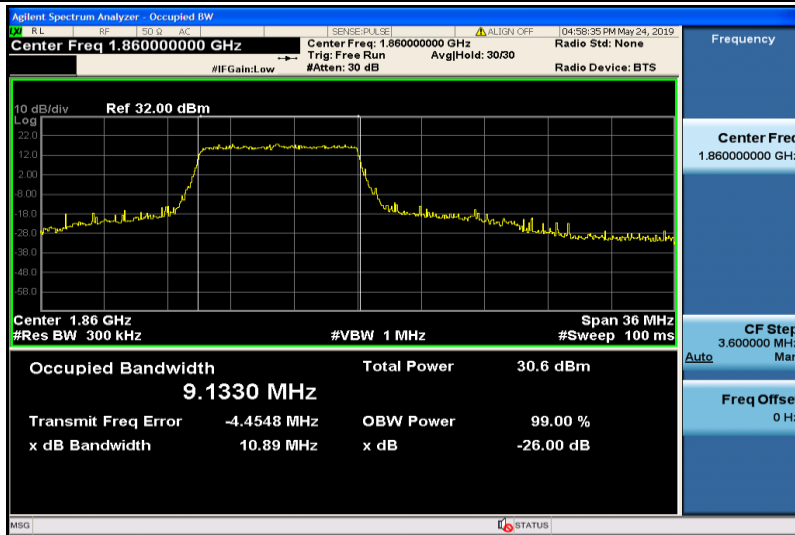
Band25-20MHz-QPSK-26140-100RB#0-9.1330
