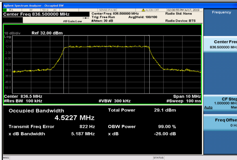
Band26-5MHz-16QAM-26915-25RB#0-4.5227
