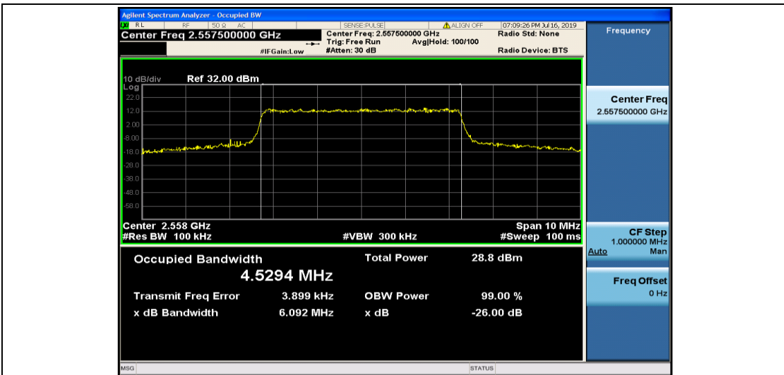
Band41-5MHz-QPSK-40265-25RB#0-4.5294
