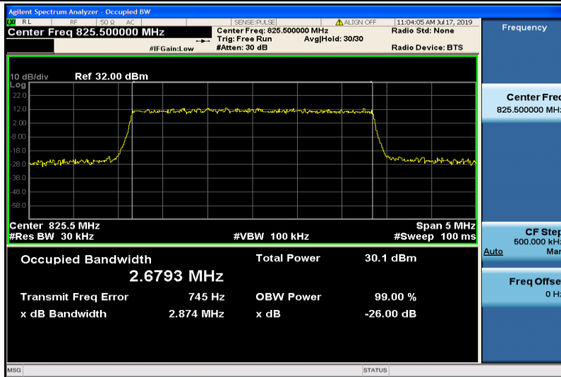
Band26-3MHz-QPSK-26805-15RB#0-2.6793
