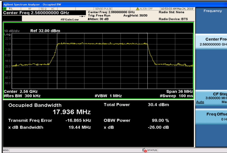
Band7-20MHz-QPSK-21350-100RB#0-17.936
