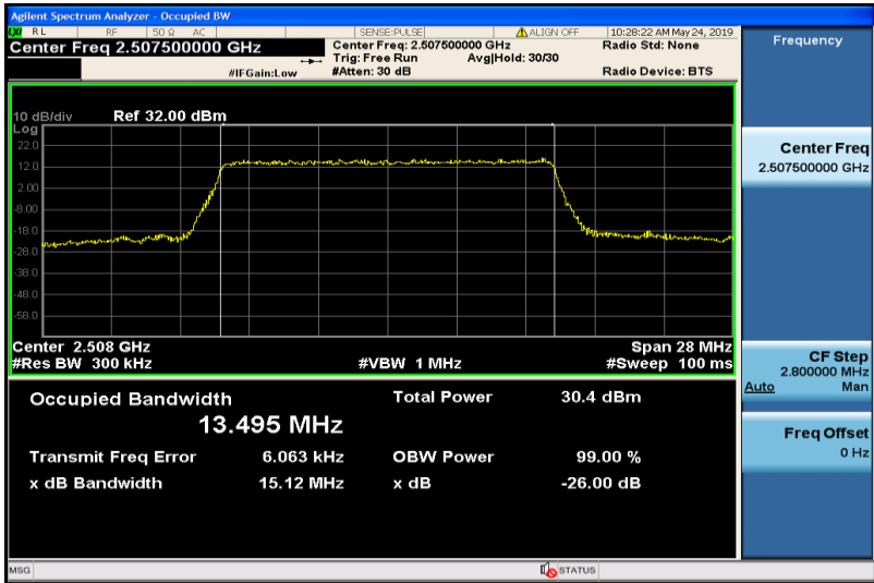
Band7-15MHz-QPSK-20825-75RB#0-13.495
