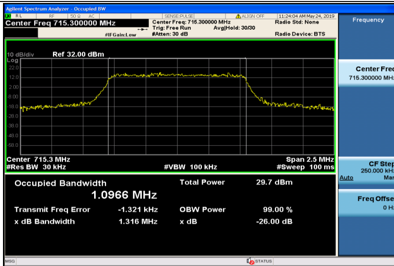
Band12-1.4MHz-16QAM-23173-6RB#0-1.0966
