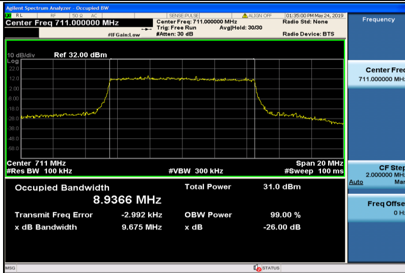
Band12-10MHz-QPSK-23130-50RB#0-8.9366
