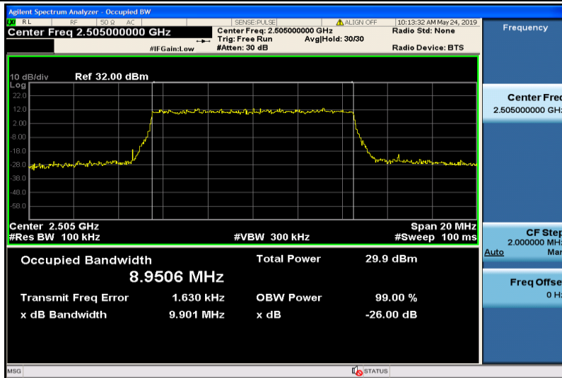
Band7-10MHz-QPSK-20800-50RB#0-8.9506
