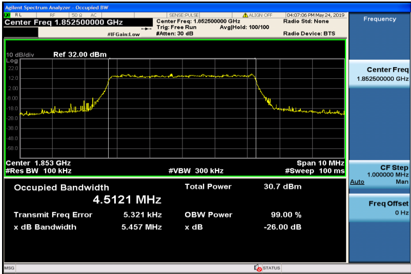
Band25-5MHz-QPSK-26065-25RB#0-4.5121
