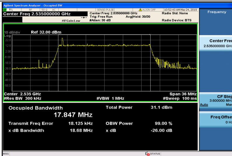
Band7-20MHz-QPSK-21100-100RB#0-17.847
