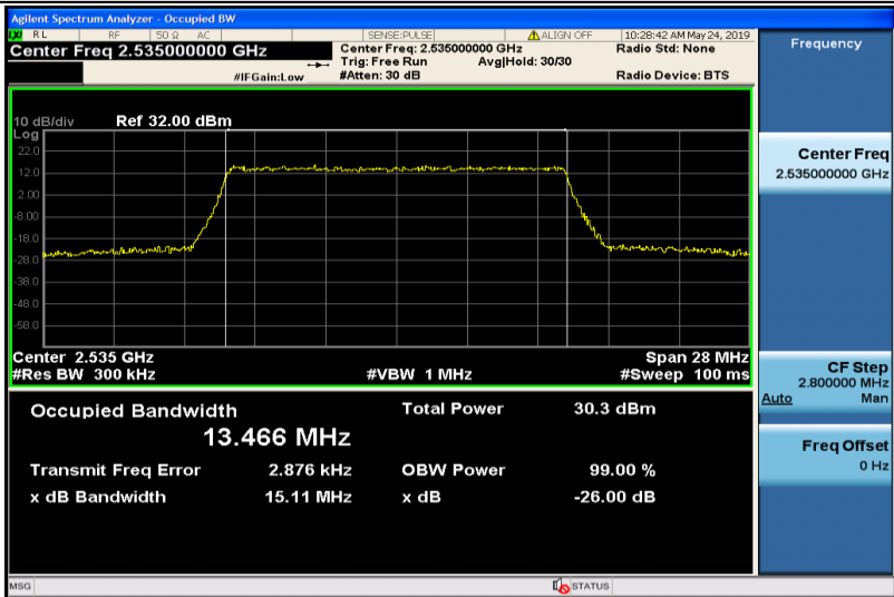
Band7-15MHz-QPSK-21100-75RB#0-13.466
