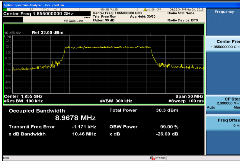
Band25-10MHz-QPSK-26090-50RB#0-8.9678
