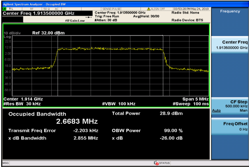
Band25-3MHz-16QAM-26675-15RB#0-2.6683
