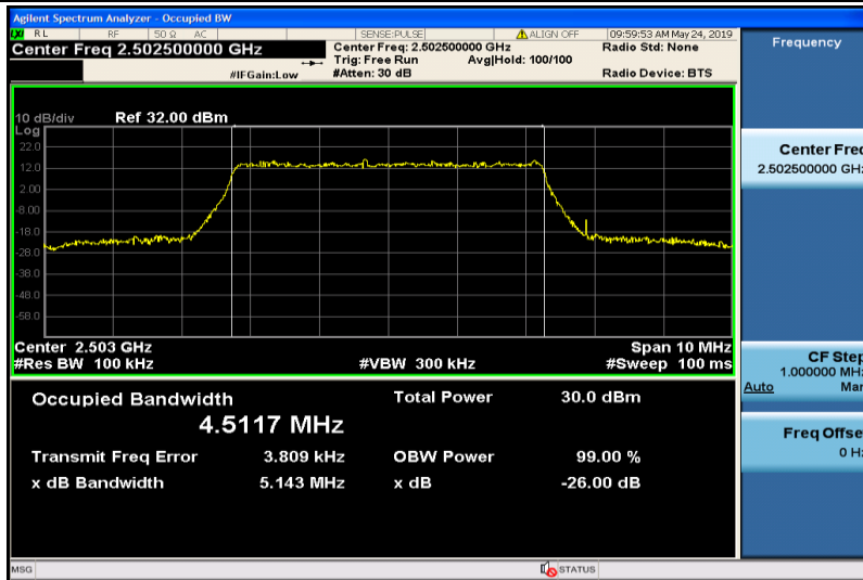
Band7-5MHz-QPSK-20775-25RB#0-4.5117
