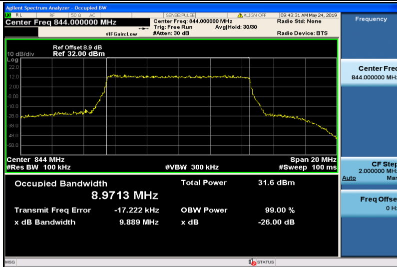
Band5-10MHz-QPSK-20600-50RB#0-8.9713
