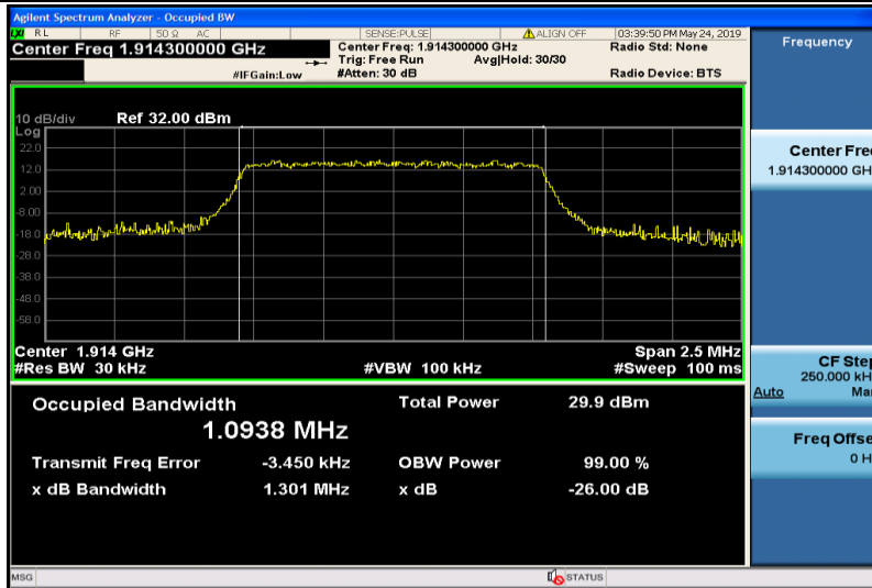
Band25-1.4MHz-QPSK-26683-6RB#0-1.0938
