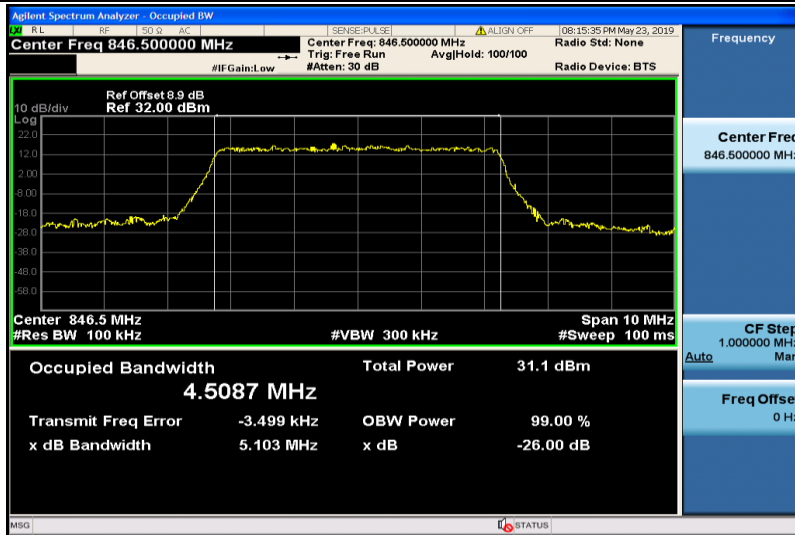
Band5-5MHz-16QAM-20625-25RB#0-4.5087
