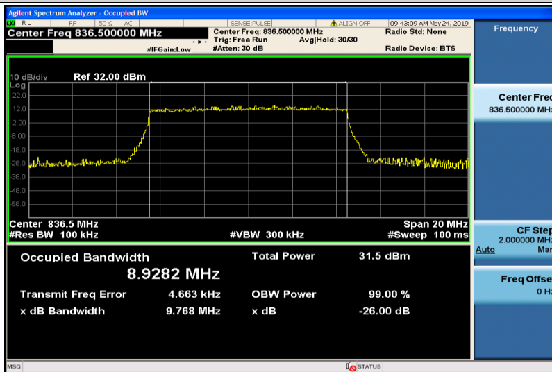
Band5-10MHz-QPSK-20525-50RB#0-8.9282
