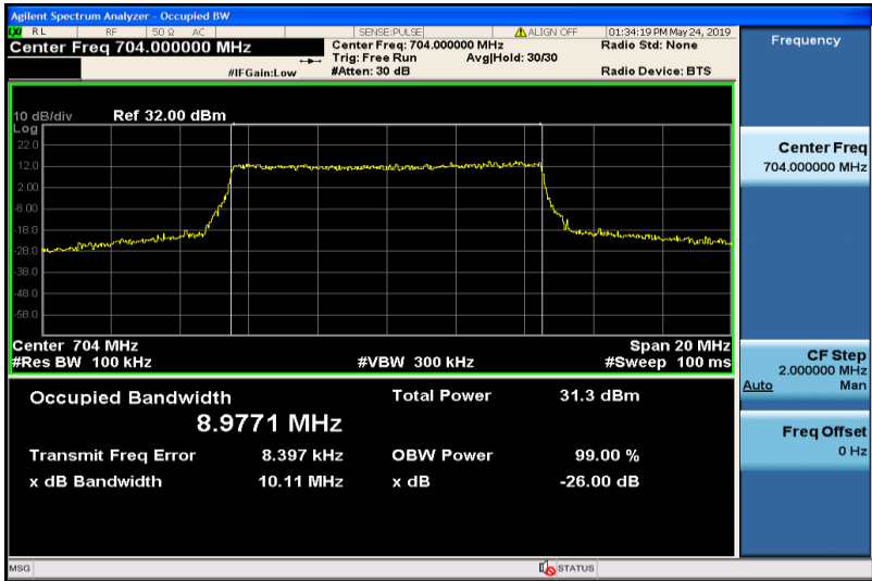
Band12-10MHz-QPSK-23060-50RB#0-8.9771
