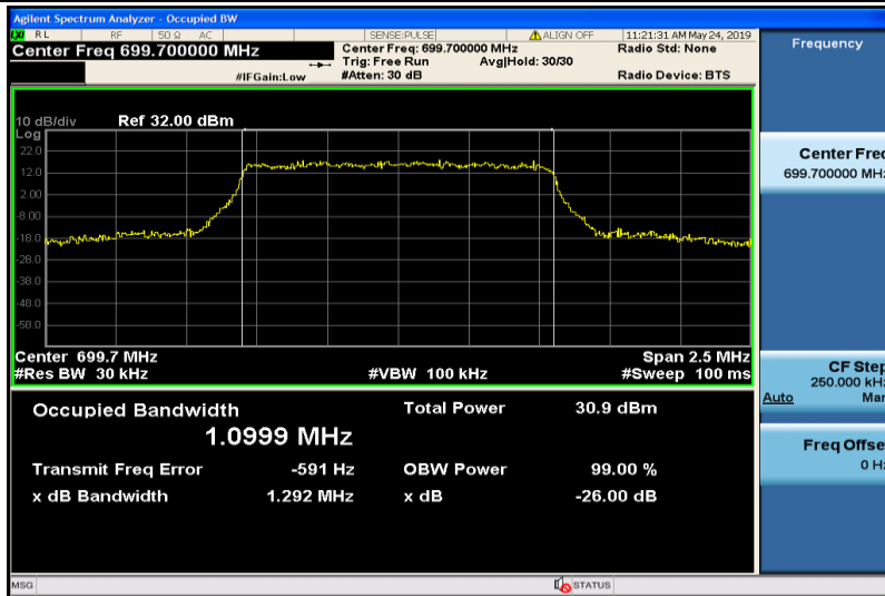
Band12-1.4MHz-QPSK-23017-6RB#0-1.0999
