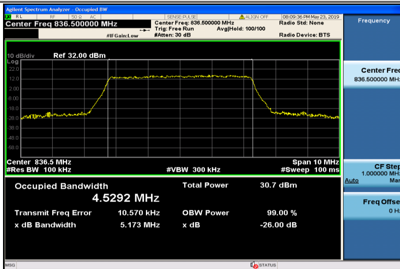
Band5-5MHz-16QAM-20525-25RB#0-4.5292
