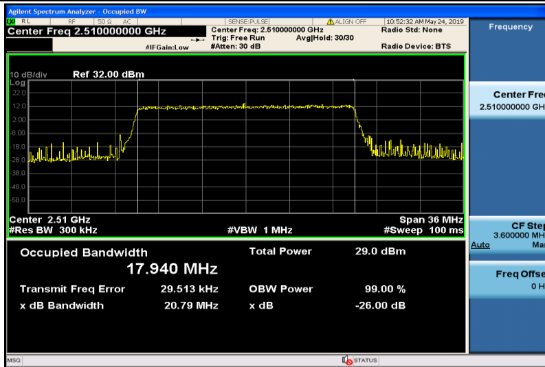
Band7-20MHz-16QAM-20850-100RB#0-17.940
