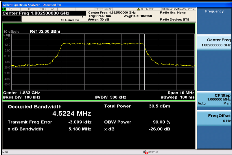
Band25-5MHz-QPSK-26365-25RB#0-4.5224
