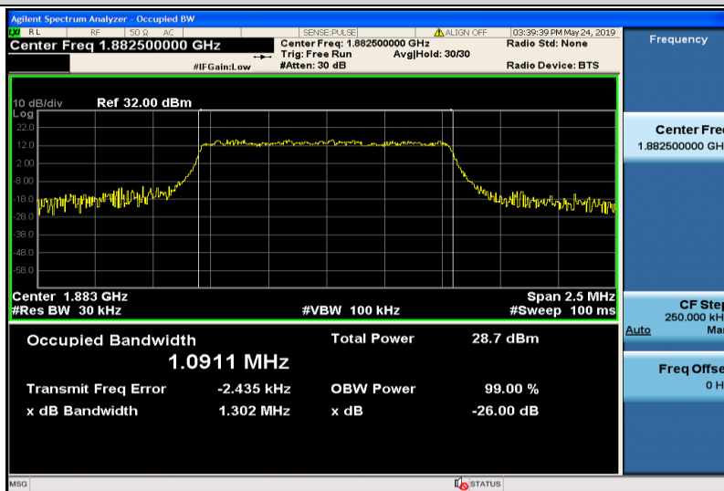
Band25-1.4MHz-16QAM-26365-6RB#0-1.0911
