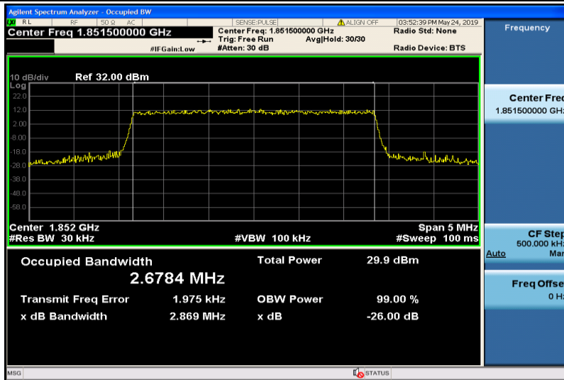
Band25-3MHz-QPSK-26055-15RB#0-2.6784
