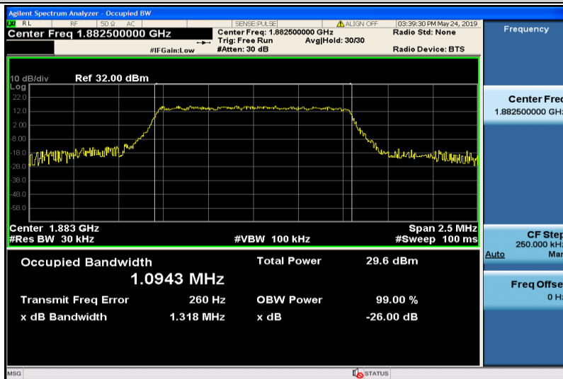
Band25-1.4MHz-QPSK-26365-6RB#0-1.0943
