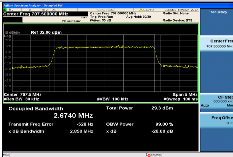
Band12-3MHz-16QAM-23095-15RB#0-2.6740
