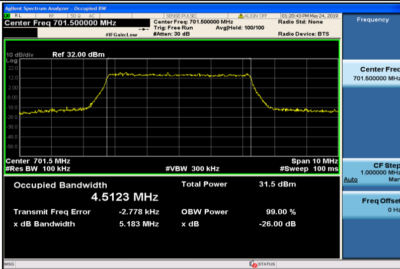
Band12-5MHz-QPSK-23035-25RB#0-4.5123
