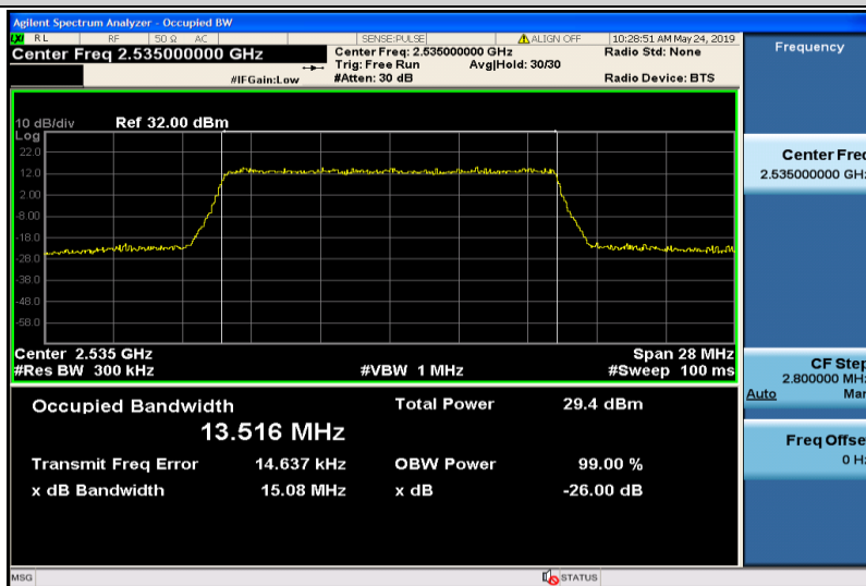
Band7-15MHz-16QAM-21100-75RB#0-13.516
