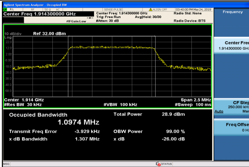
Band25-1.4MHz-16QAM-26683-6RB#0-1.0974
