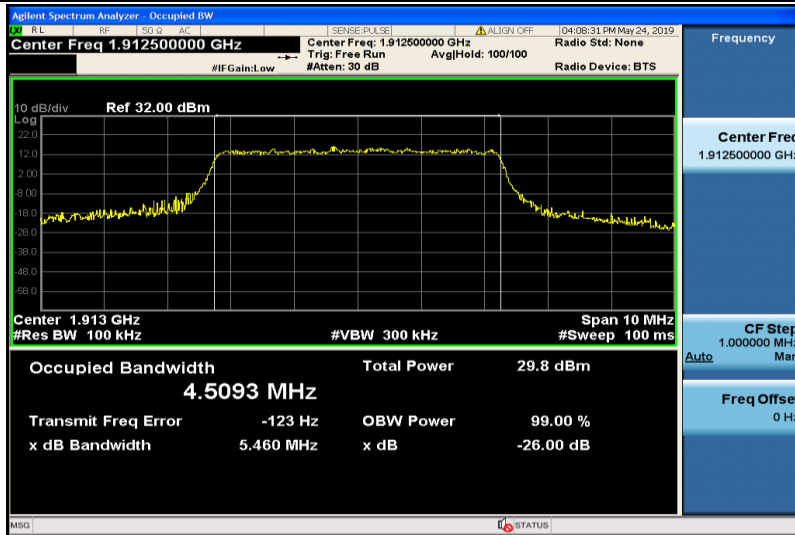
Band25-5MHz-16QAM-26665-25RB#0-4.5093
