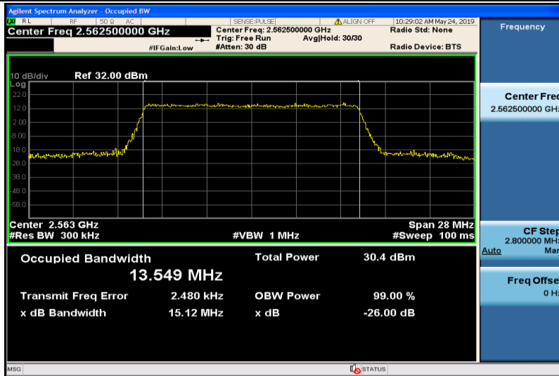
Band7-15MHz-QPSK-21375-75RB#0-13.549
