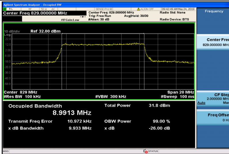
Band5-10MHz-QPSK-20450-50RB#0-8.9913
