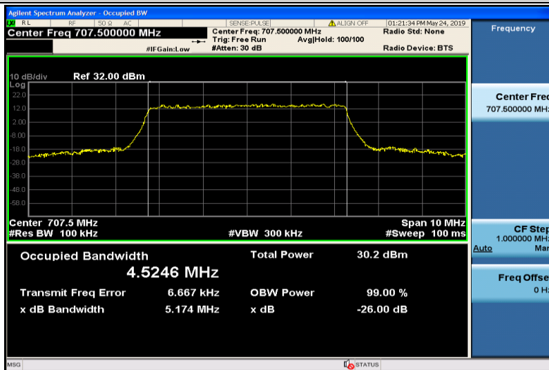
Band12-5MHz-16QAM-23095-25RB#0-4.5246
