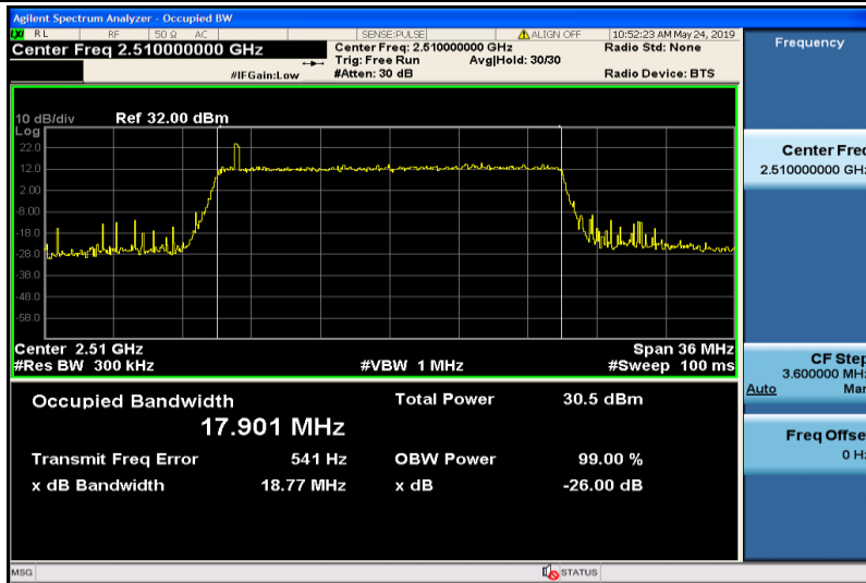
Band7-20MHz-QPSK-20850-100RB#0-17.901
