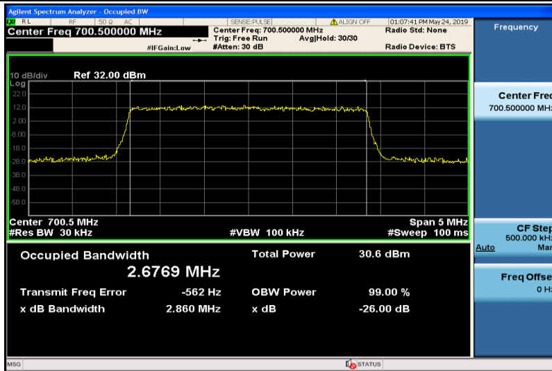
Band12-3MHz-QPSK-23025-15RB#0-2.6769
