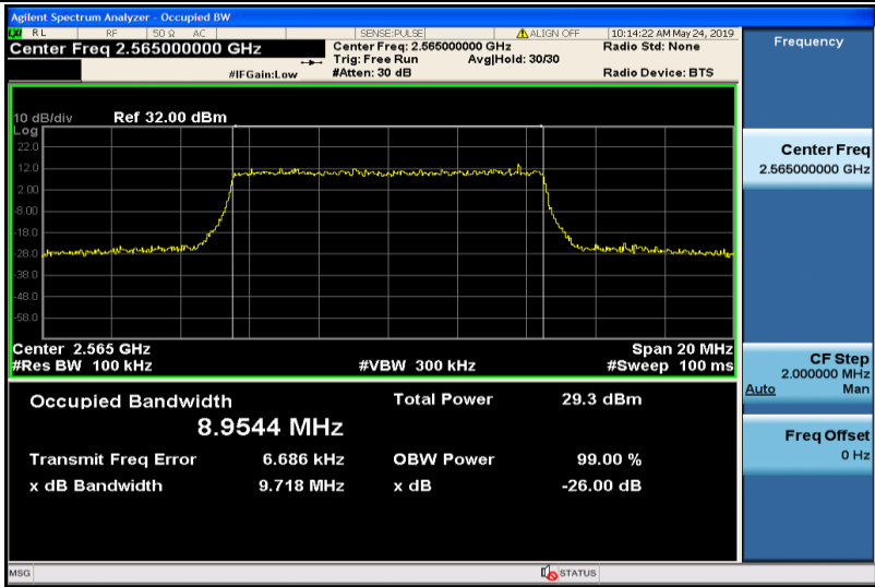
Band7-10MHz-16QAM-21400-50RB#0-8.9544
