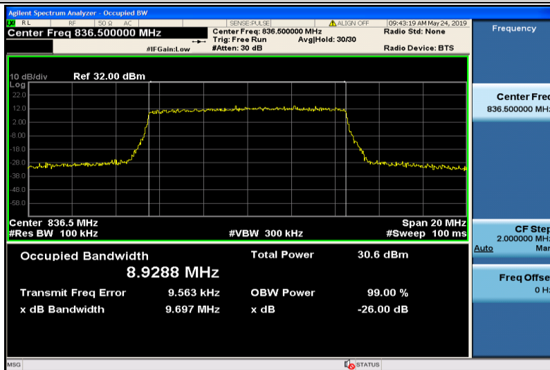
Band5-10MHz-16QAM-20525-50RB#0-8.9288
