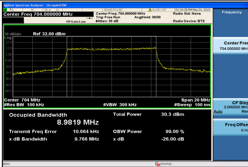
Band12-10MHz-16QAM-23060-50RB#0-8.9819
