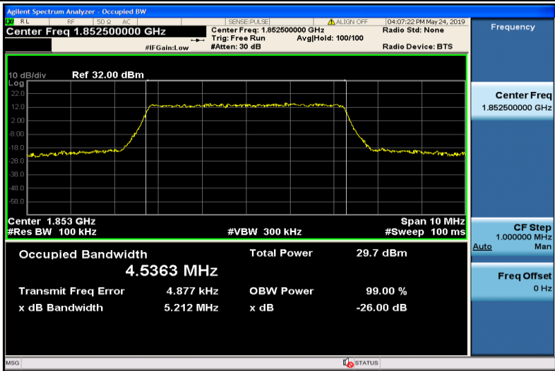
Band25-5MHz-16QAM-26065-25RB#0-4.5363
