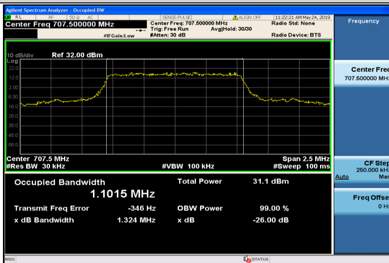
Band12-1.4MHz-QPSK-23095-6RB#0-1.1015
