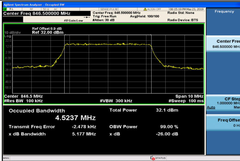
Band5-5MHz-QPSK-20625-25RB#0-4.5237
