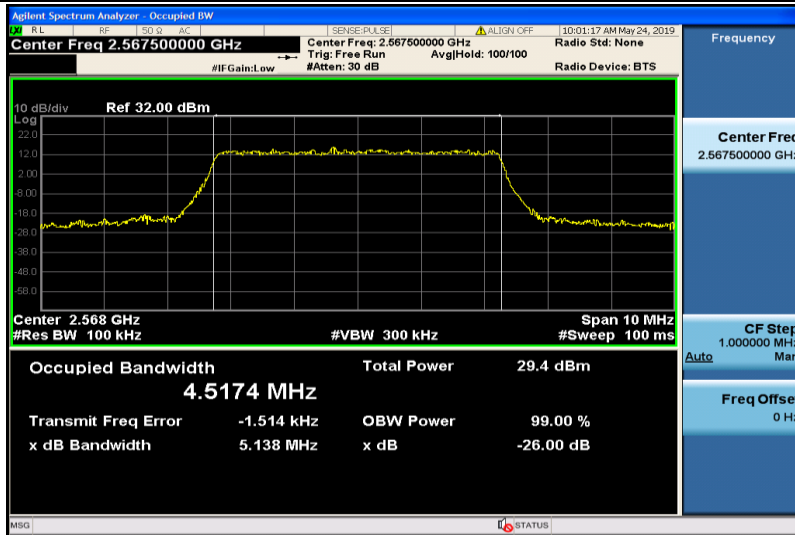
Band7-5MHz-16QAM-21425-25RB#0-4.5174
