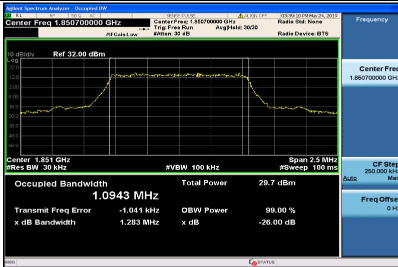
Band25-1.4MHz-QPSK-26047-6RB#0-1.0943
