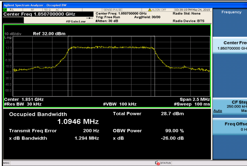
Band25-1.4MHz-16QAM-26047-6RB#0-1.0946
