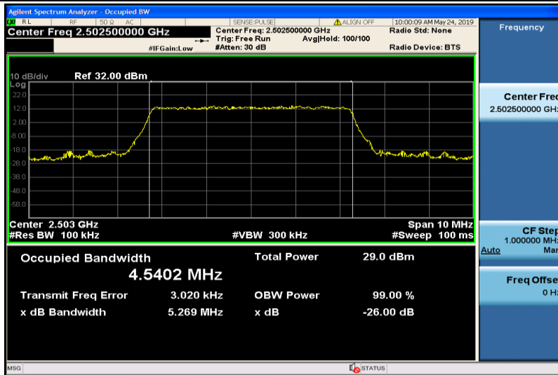
Band7-5MHz-16QAM-20775-25RB#0-4.5402
