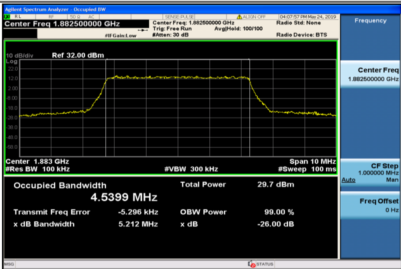
Band25-5MHz-16QAM-26365-25RB#0-4.5399
