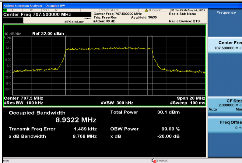
Band12-10MHz-16QAM-23095-50RB#0-8.9322
