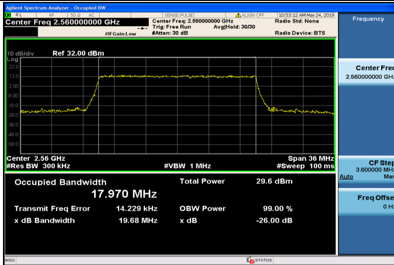
Band7-20MHz-16QAM-21350-100RB#0-17.970
