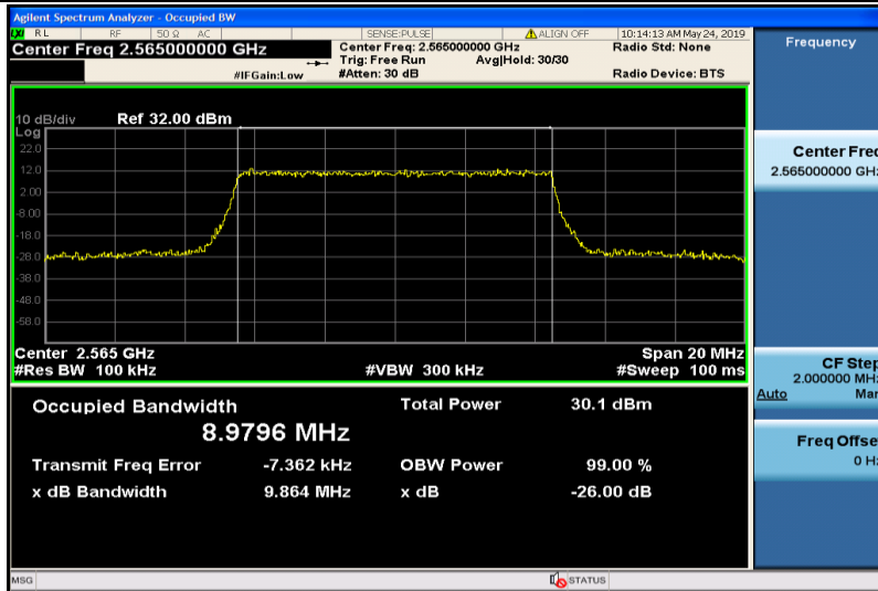
Band7-10MHz-QPSK-21400-50RB#0-8.9796
