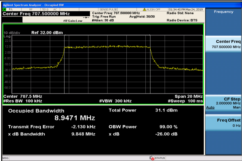
Band12-10MHz-QPSK-23095-50RB#0-8.9471
