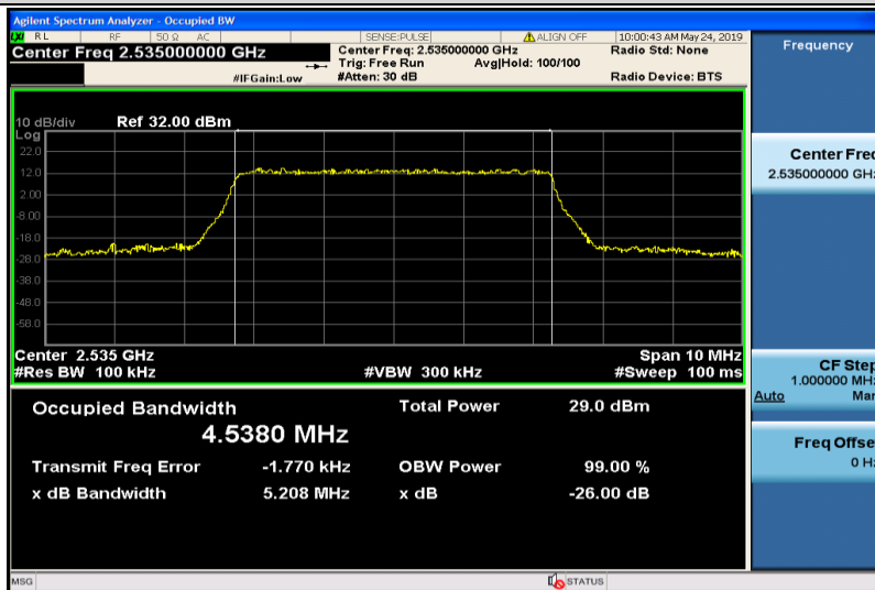
Band7-5MHz-16QAM-21100-25RB#0-4.5380
