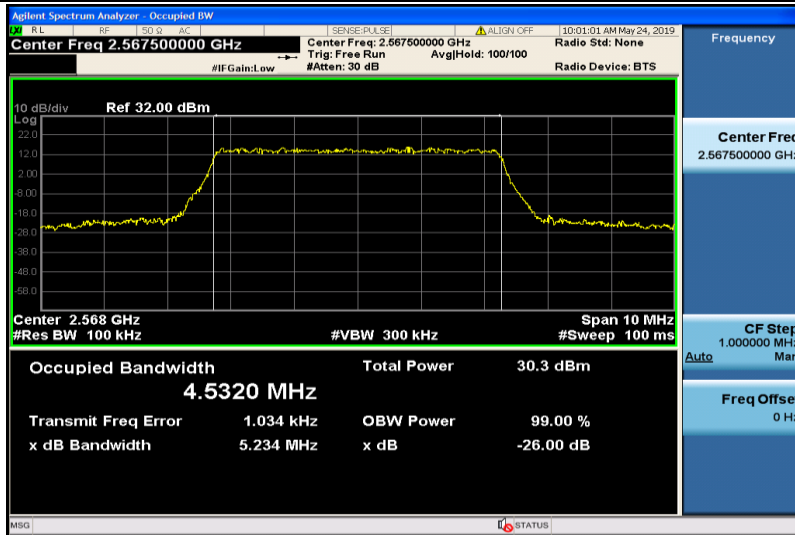
Band7-5MHz-QPSK-21425-25RB#0-4.5320
