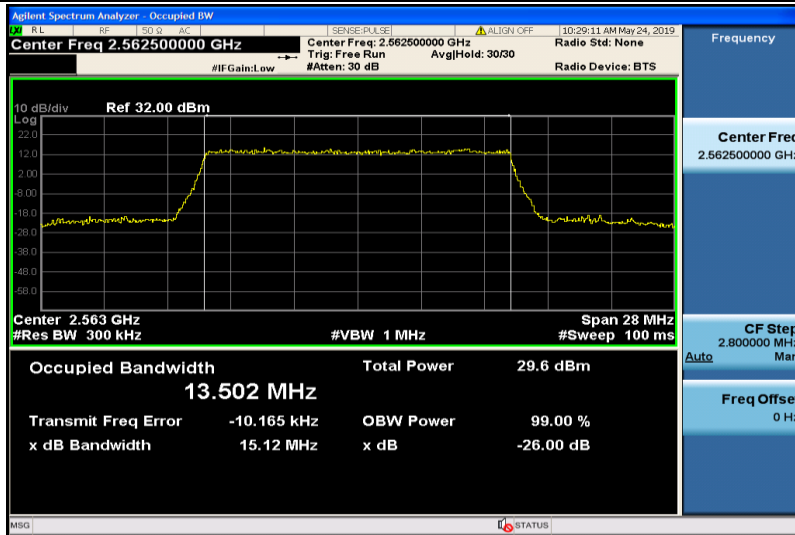
Band7-15MHz-16QAM-21375-75RB#0-13.502
