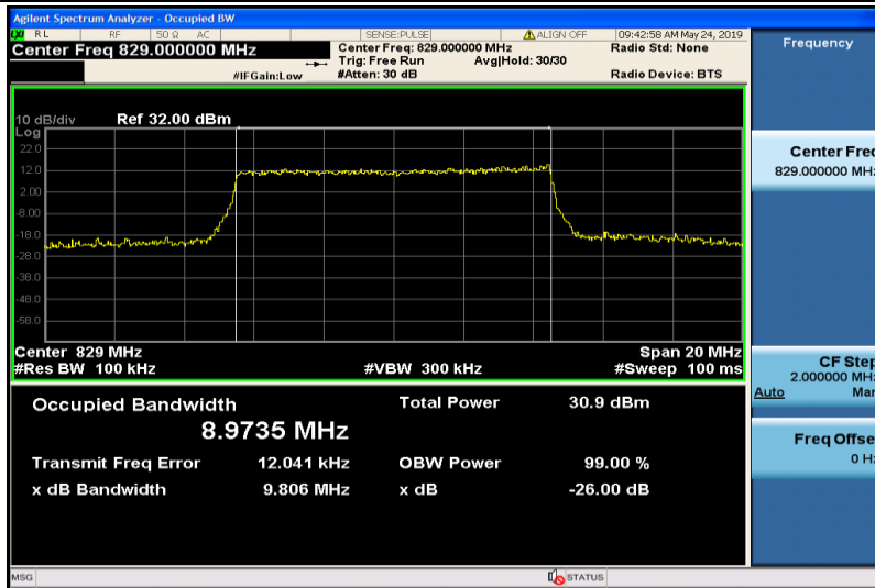
Band5-10MHz-16QAM-20450-50RB#0-8.9735
