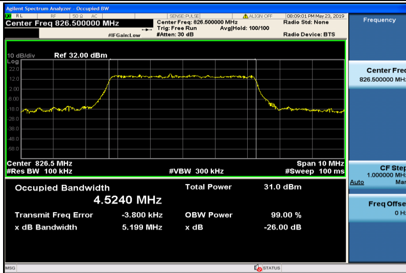
Band5-5MHz-16QAM-20425-25RB#0-4.5240
