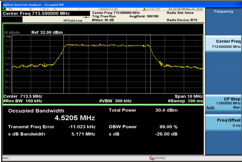
Band12-5MHz-16QAM-23155-25RB#0-4.5205
