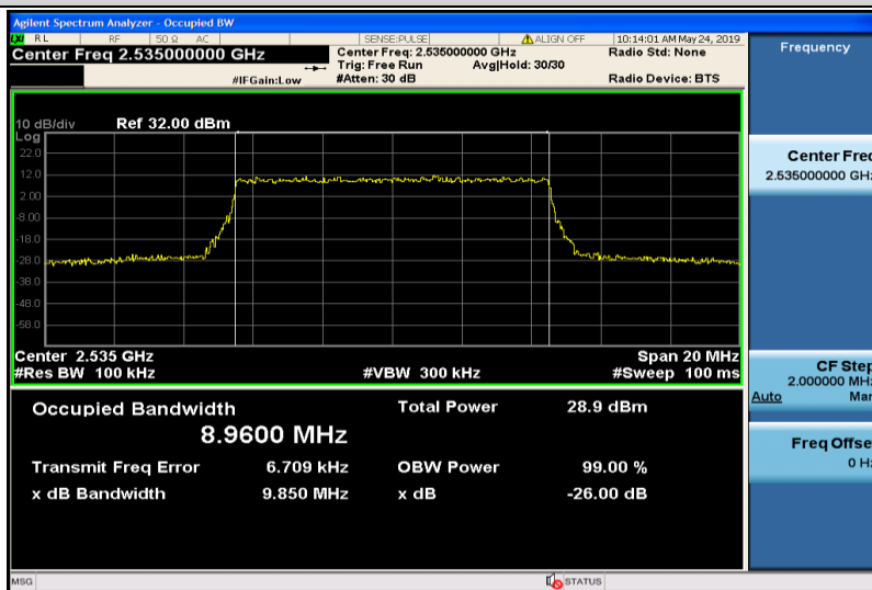
Band7-10MHz-16QAM-21100-50RB#0-8.9600
