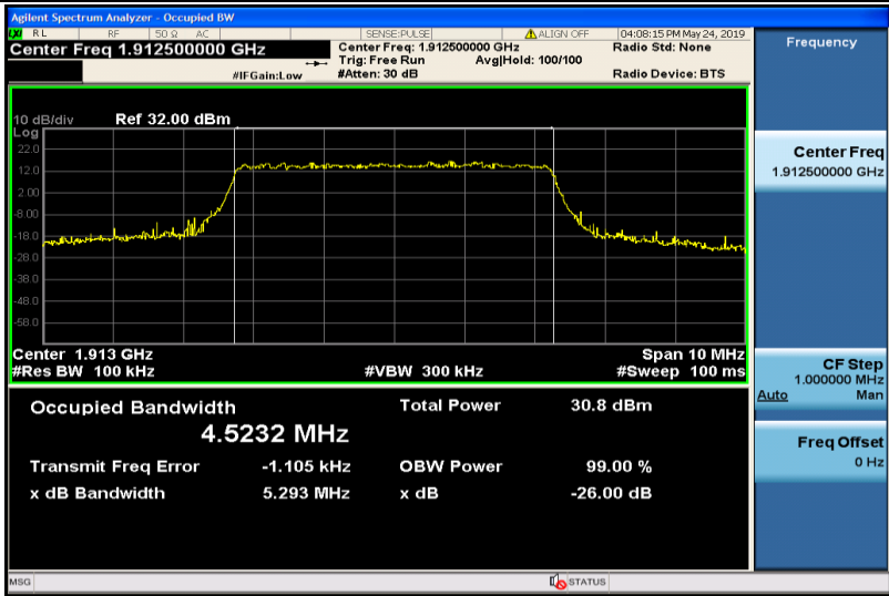
Band25-5MHz-QPSK-26665-25RB#0-4.5232
