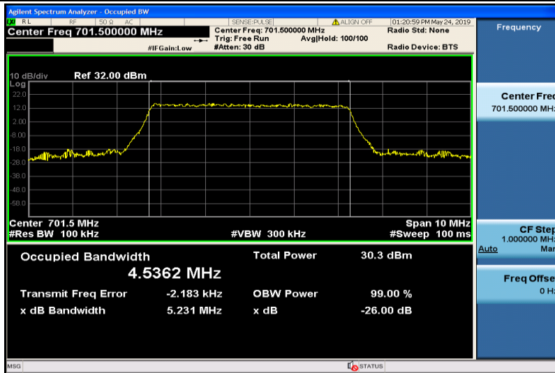
Band12-5MHz-16QAM-23035-25RB#0-4.5362
