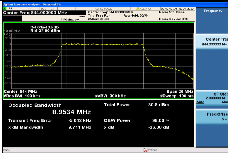
Band5-10MHz-16QAM-20600-50RB#0-8.9534
