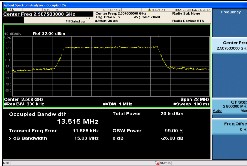
Band7-15MHz-16QAM-20825-75RB#0-13.515
