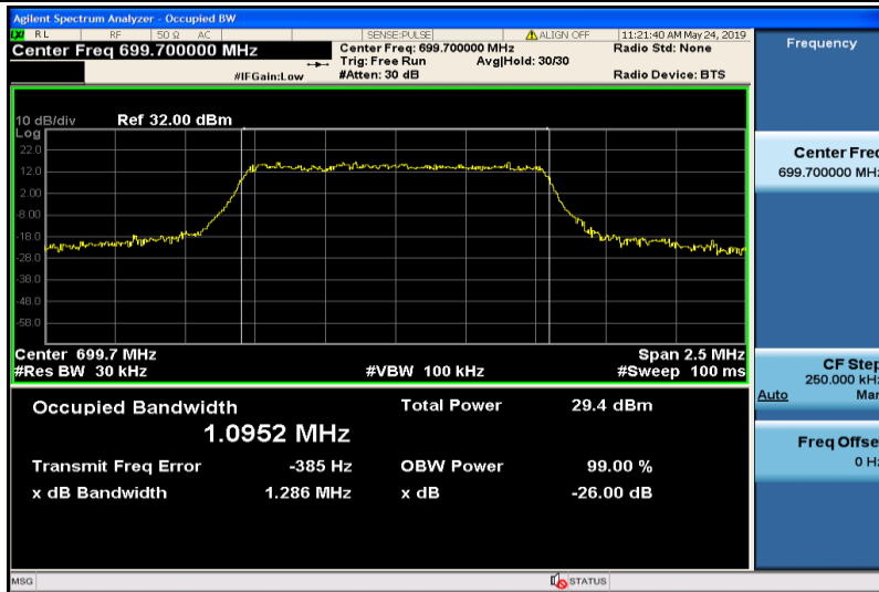
Band12-1.4MHz-16QAM-23017-6RB#0-1.0952
