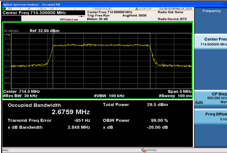
Band12-3MHz-16QAM-23165-15RB#0-2.6759
