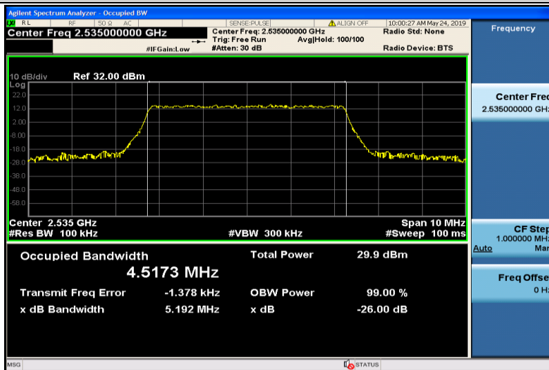
Band7-5MHz-QPSK-21100-25RB#0-4.5173
