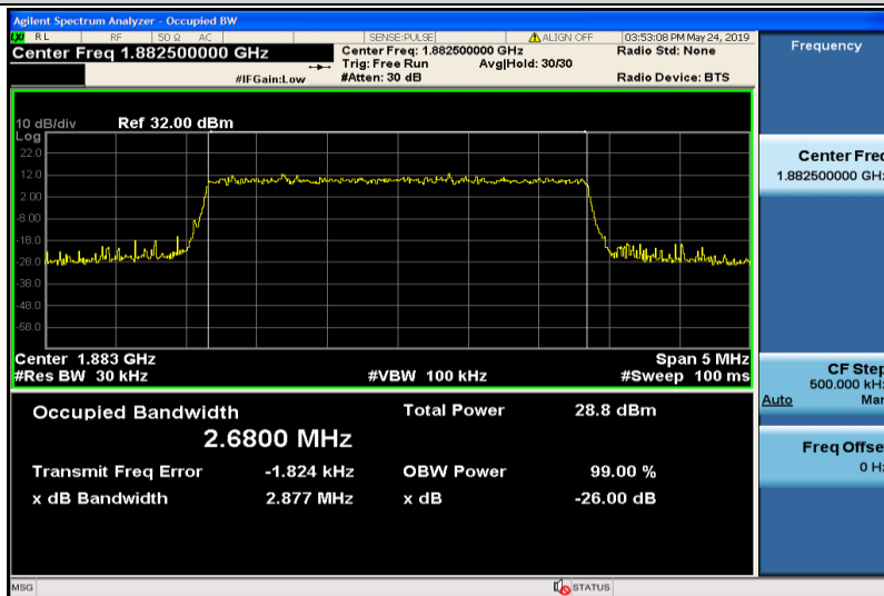
Band25-3MHz-16QAM-26365-15RB#0-2.6800
