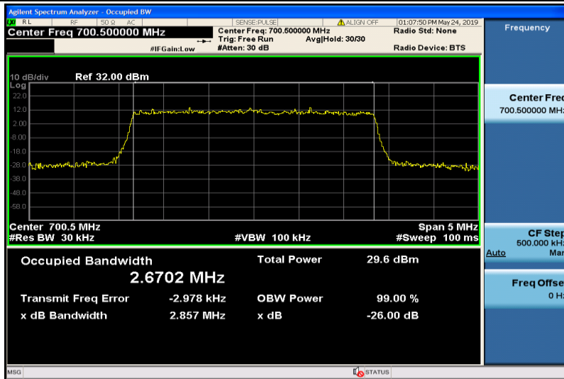
Band12-3MHz-16QAM-23025-15RB#0-2.6702
