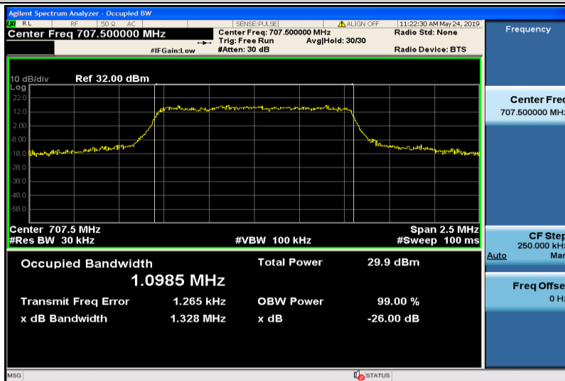
Band12-1.4MHz-16QAM-23095-6RB#0-1.0985
