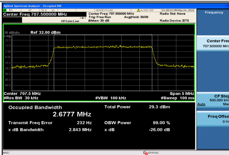
Band12-3MHz-QPSK-23095-15RB#0-2.6777
