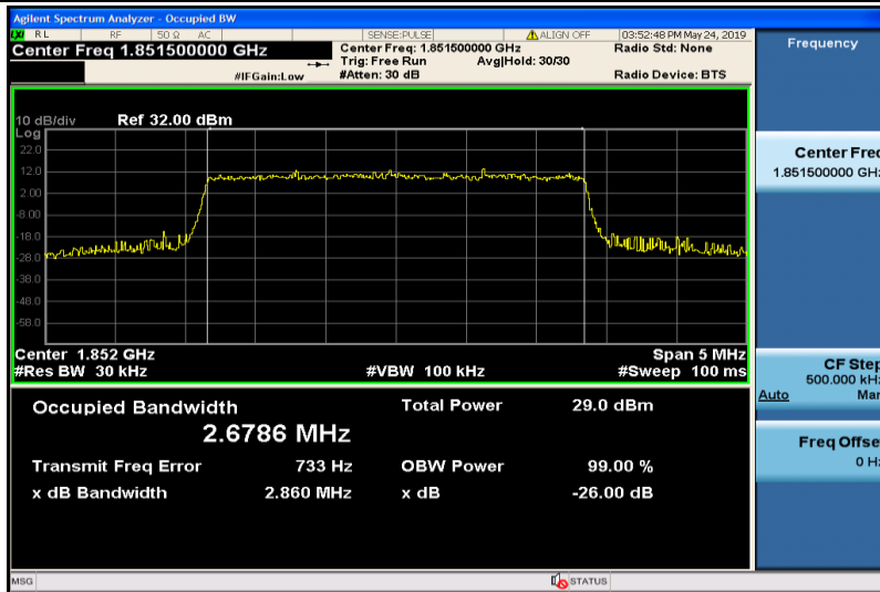
Band25-3MHz-16QAM-26055-15RB#0-2.6786
