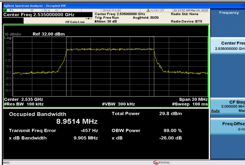
Band7-10MHz-QPSK-21100-50RB#0-8.9514
