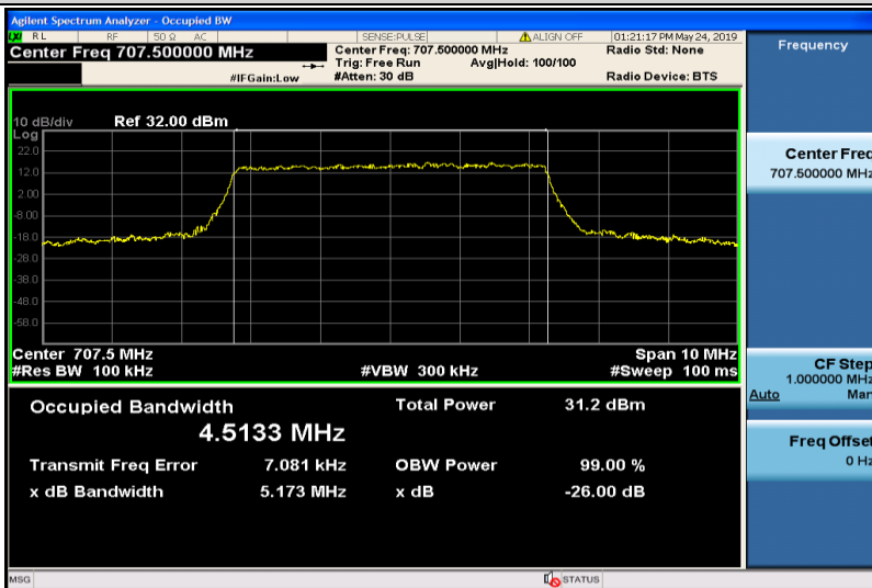
Band12-5MHz-QPSK-23095-25RB#0-4.5133
