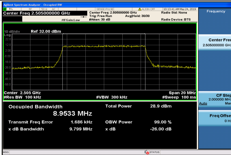
Band7-10MHz-16QAM-20800-50RB#0-8.9533
