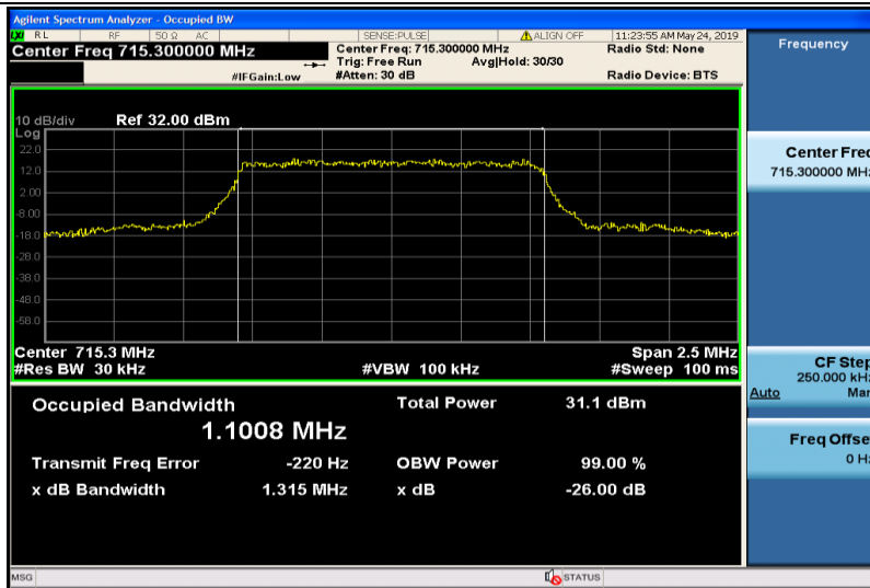
Band12-1.4MHz-QPSK-23173-6RB#0-1.1008
