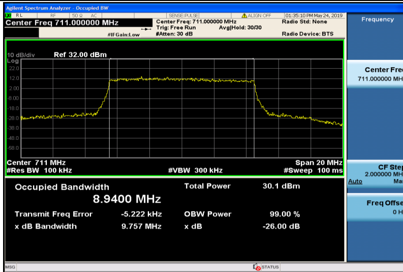
Band12-10MHz-16QAM-23130-50RB#0-8.9400
