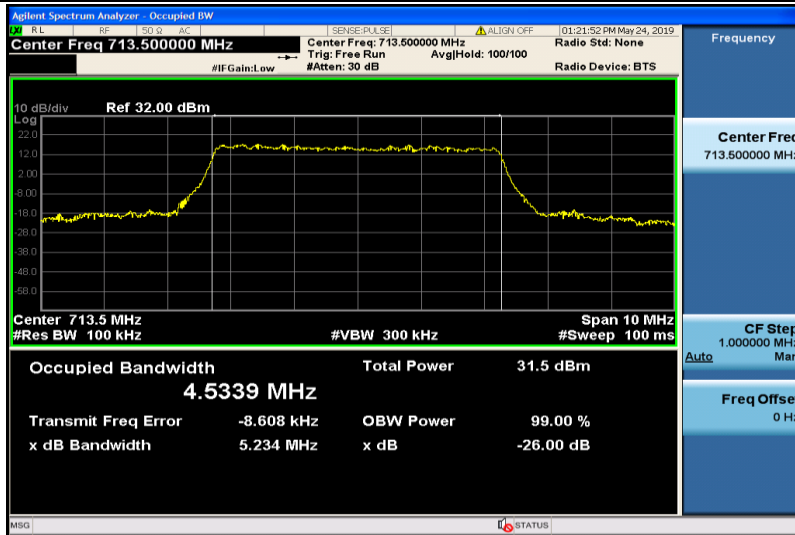
Band12-5MHz-QPSK-23155-25RB#0-4.5339
