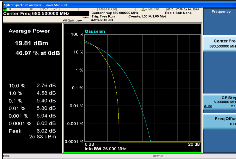
Band71-5MHz-16QAM-133297-25RB#0
