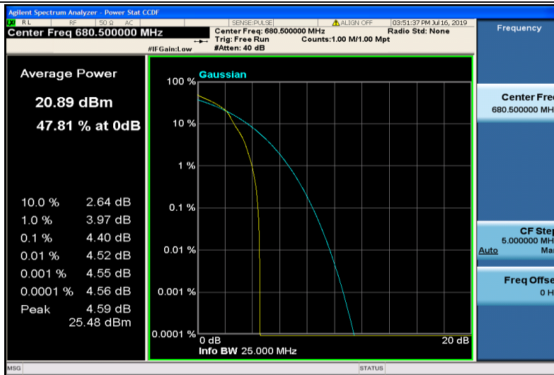
Band71-5MHz-16QAM-133297-1RB#0
