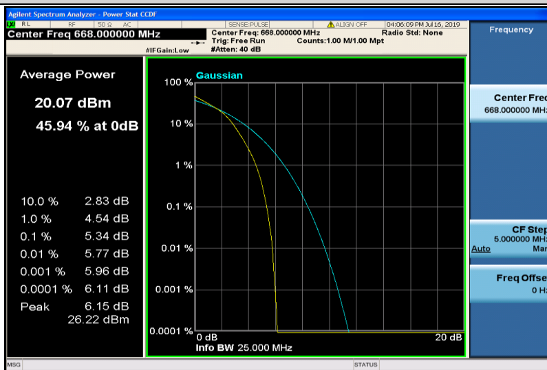
Band71-10MHz-16QAM-133172-50RB#0
