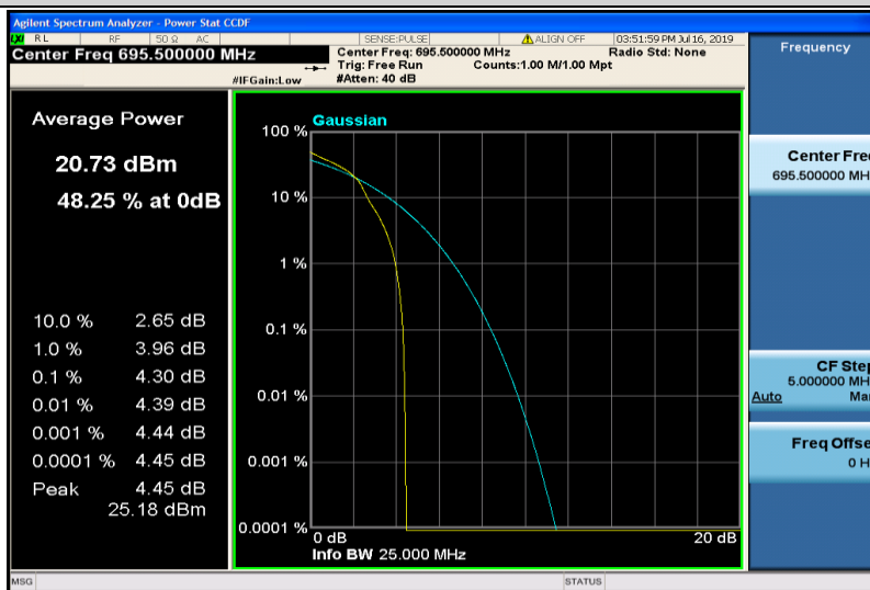
Band71-5MHz-16QAM-133447-1RB#0
