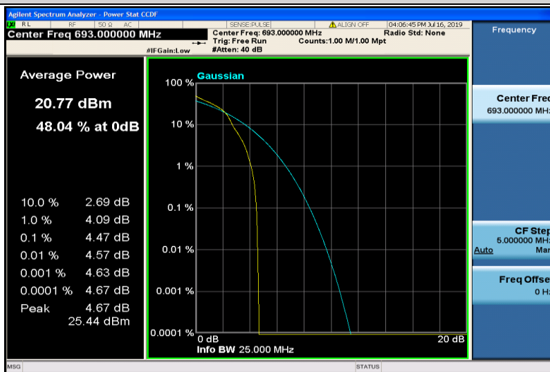
Band71-10MHz-16QAM-133422-1RB#0
