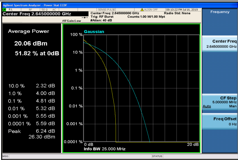
Band41-20MHz-QPSK-41140-100RB#0
