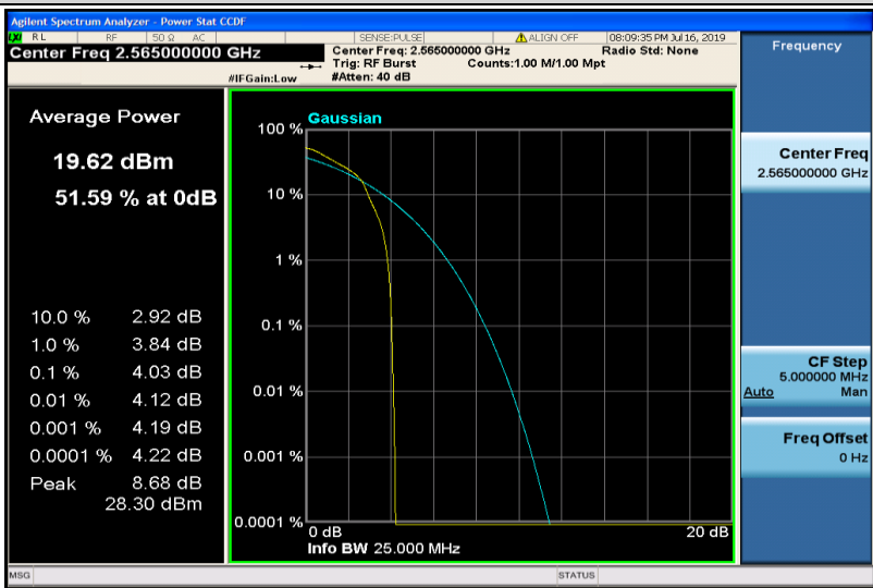
Band41-20MHz-16QAM-40340-1RB#0
