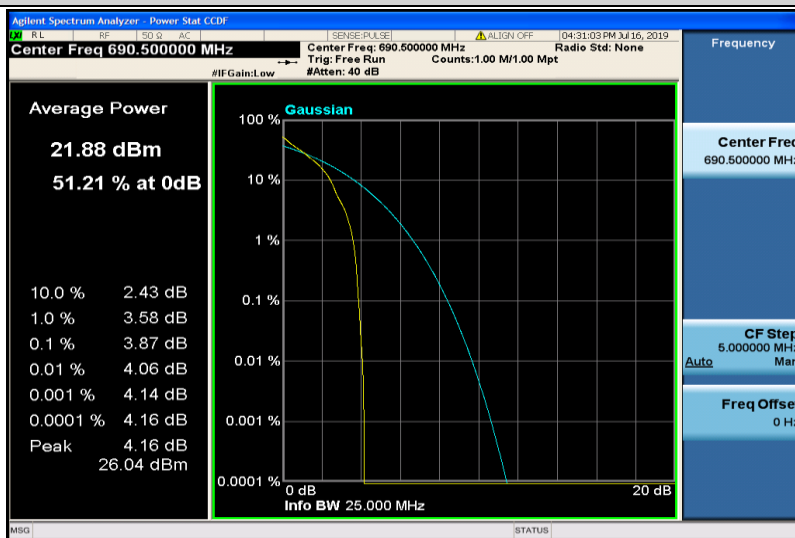
Band71-15MHz-QPSK-133397-1RB#0
