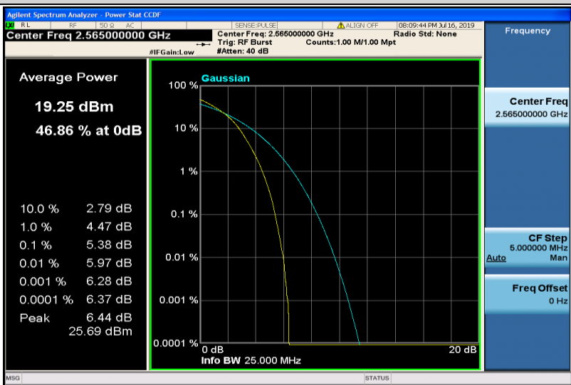
Band41-20MHz-16QAM-40340-100RB#0
