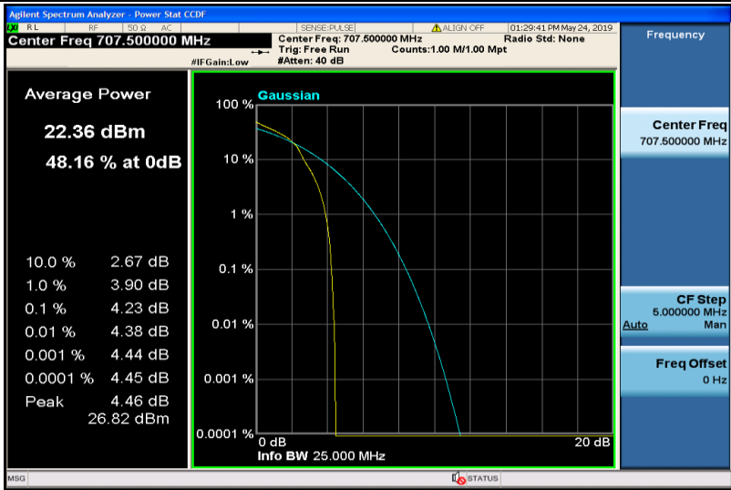
Band12-5MHz-16QAM-23095-1RB#0
