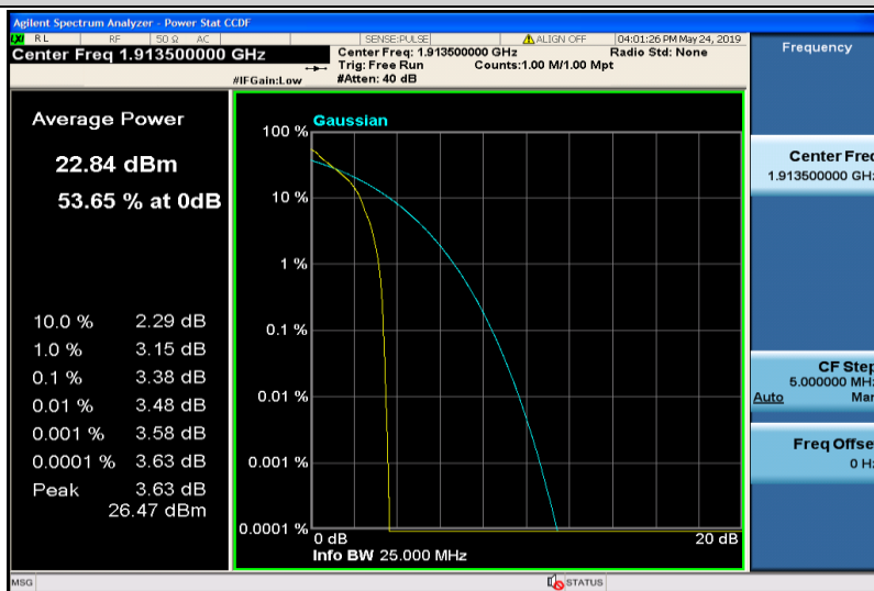
Band25-3MHz-QPSK-26675-1RB#0
