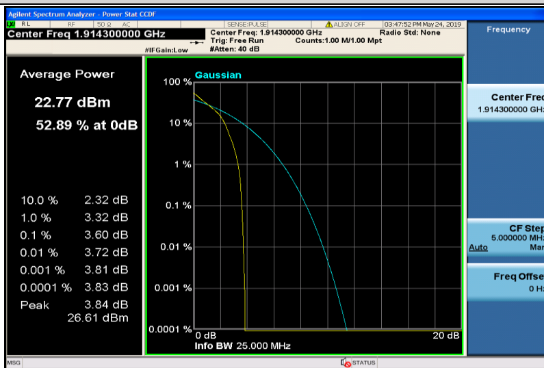
Band25-1.4MHz-QPSK-26683-1RB#0
