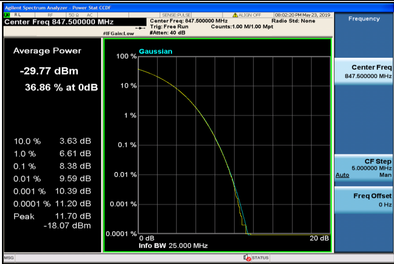
Band5-3MHz-16QAM-20635-15RB#0
