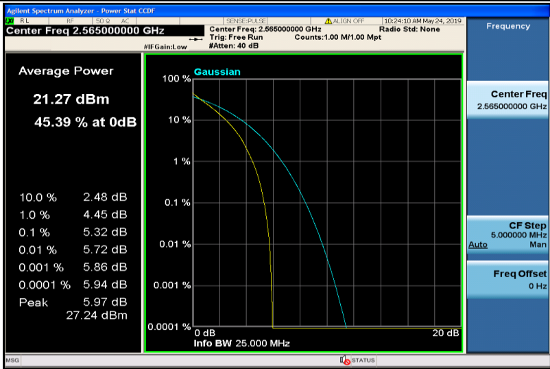
Band7-10MHz-QPSK-21400-50RB#0
