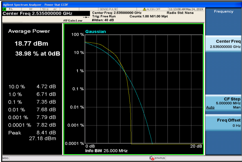
Band7-20MHz-QPSK-21100-1RB#0
