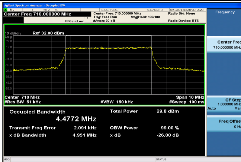
Band17-5MHz-QPSK-23790-25RB#0-4.4772
