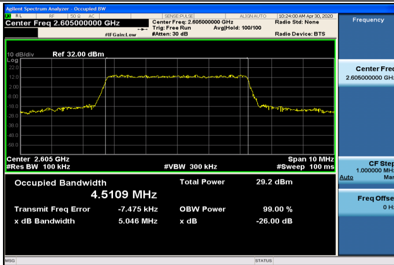
Band41-5MHz-16QAM-40740-25RB#0-4.5109
