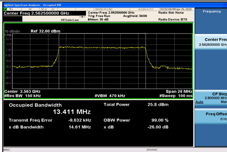
Band7-15MHz-QPSK-21375-75RB#0-13.411
