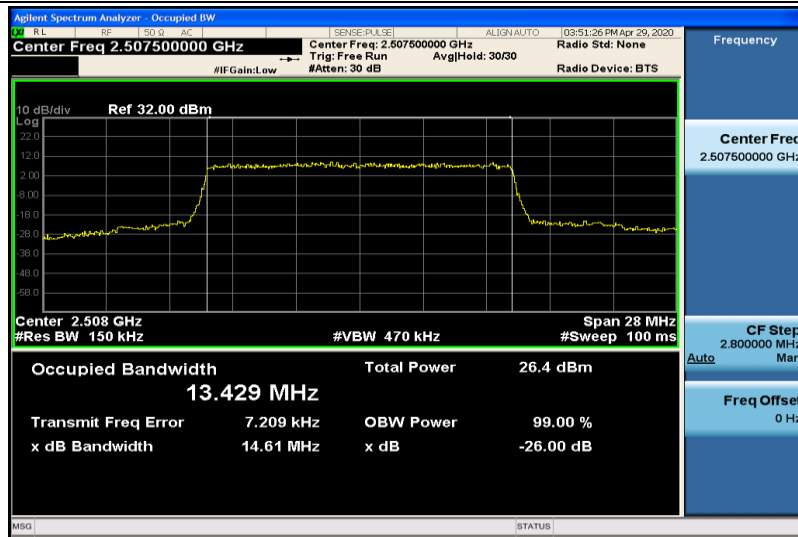
Band7-15MHz-QPSK-20825-75RB#0-13.429
