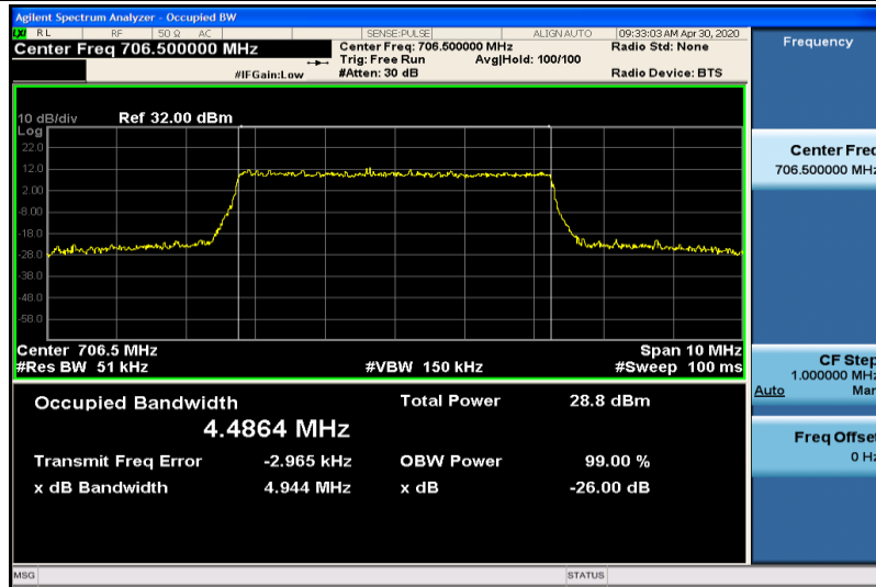
Band17-5MHz-16QAM-23755-25RB#0-4.4864
