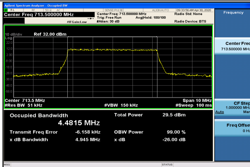
Band17-5MHz-QPSK-23825-25RB#0-4.4815
