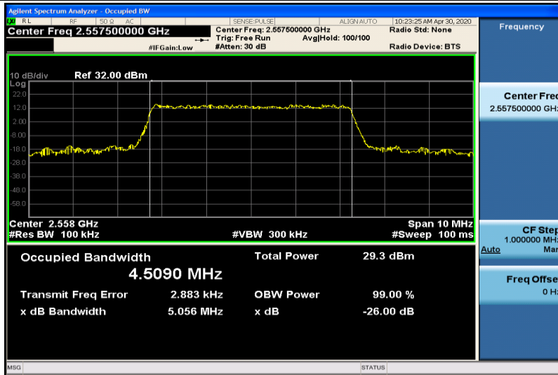
Band41-5MHz-16QAM-40265-25RB#0-4.5090
