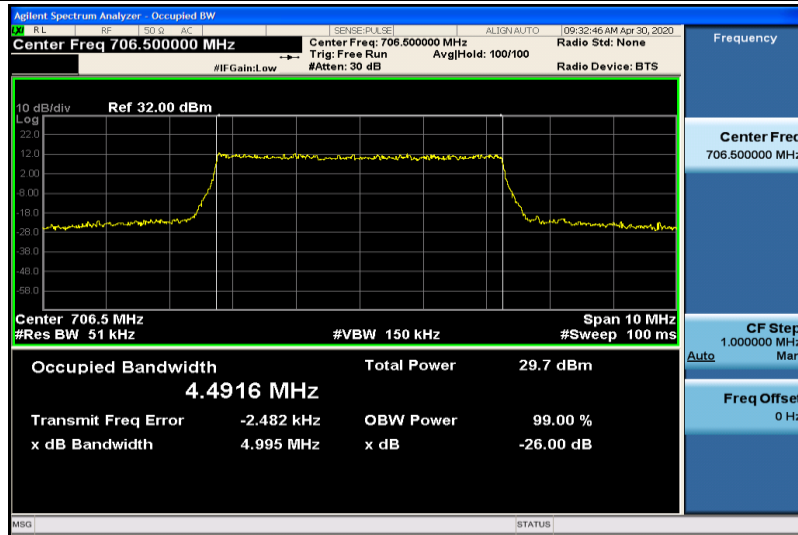
Band17-5MHz-QPSK-23755-25RB#0-4.4916
