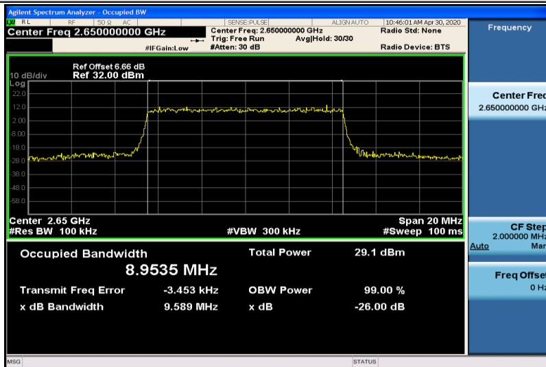
Band41-10MHz-16QAM-41190-50RB#0-8.9535
