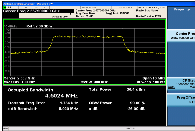
Band41-5MHz-QPSK-40265-25RB#0-4.5024
