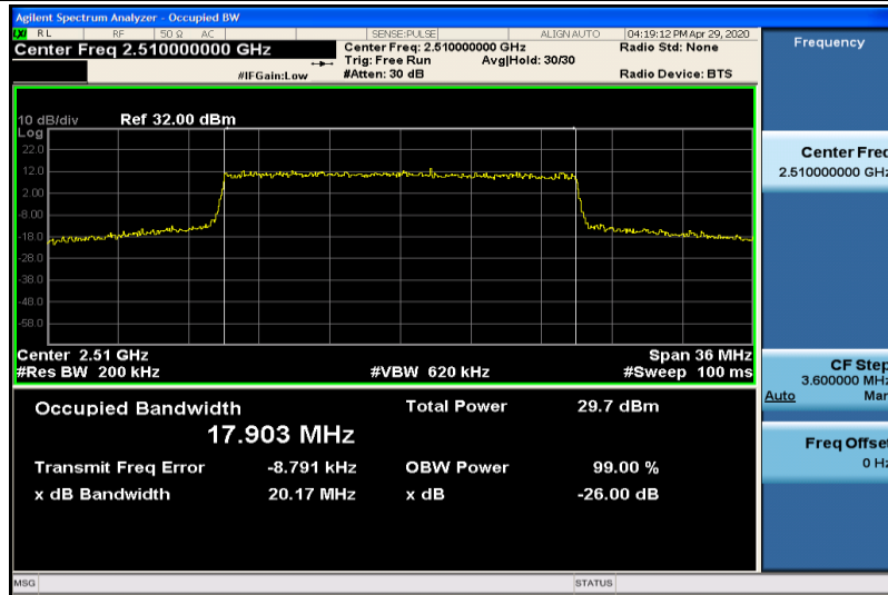
Band7-20MHz-QPSK-20850-100RB#0-17.903
