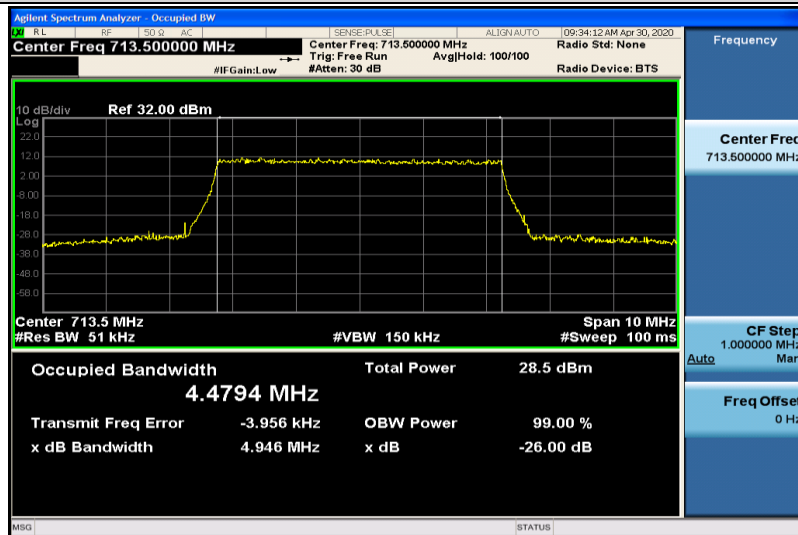
Band17-5MHz-16QAM-23825-25RB#0-4.4794
