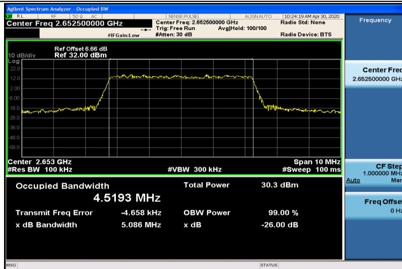
Band41-5MHz-QPSK-41215-25RB#0-4.5193
