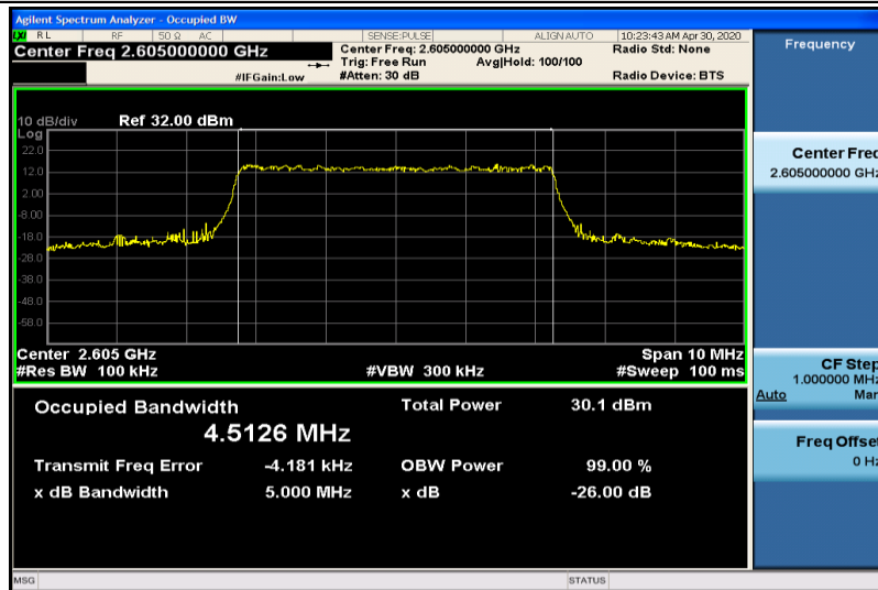
Band41-5MHz-QPSK-40740-25RB#0-4.5126
