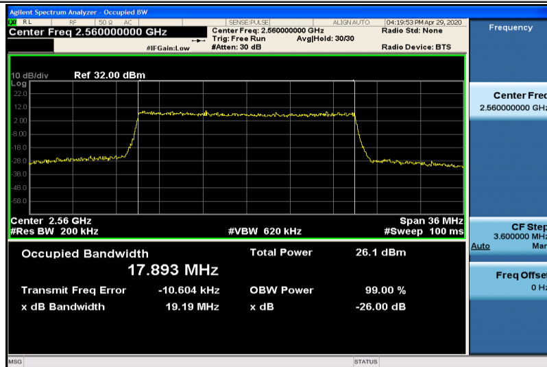
Band7-20MHz-QPSK-21350-100RB#0-17.893
