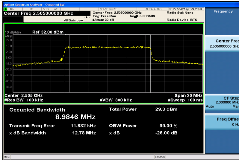
Band7-10MHz-QPSK-20800-50RB#0-8.9846
