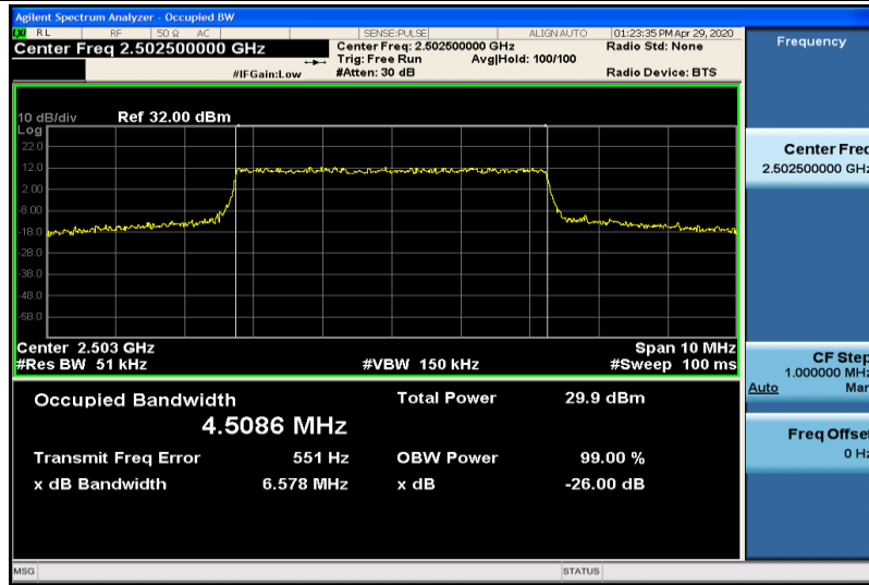
Band7-5MHz-QPSK-20775-25RB#0-4.5086
