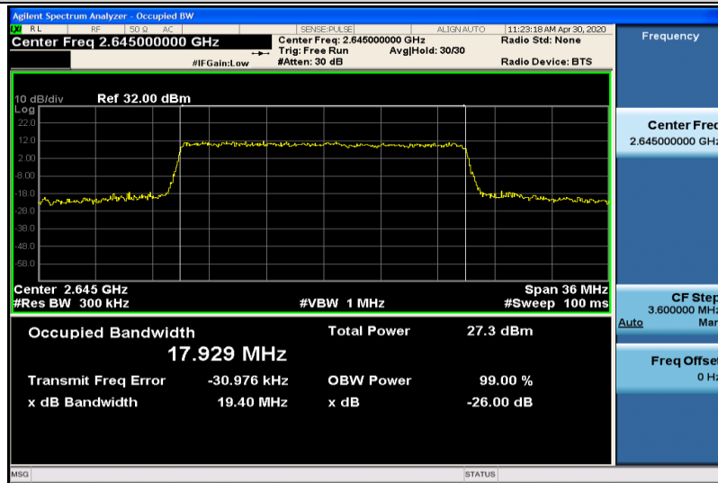
Band41-20MHz-16QAM-41140-100RB#0-17.929
