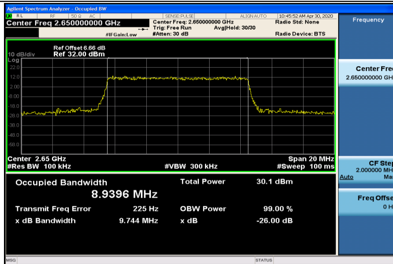
Band41-10MHz-QPSK-41190-50RB#0-8.9396
