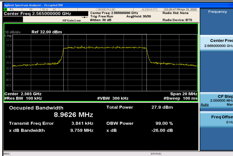
Band7-10MHz-16QAM-21400-50RB#0-8.9626
