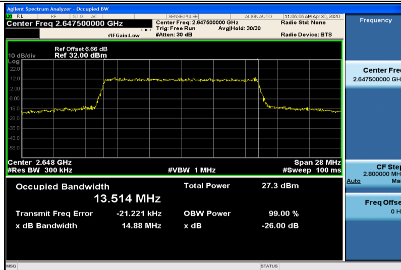
Band41-15MHz-QPSK-41165-75RB#0-13.514
