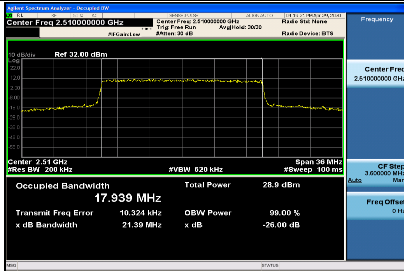
Band7-20MHz-16QAM-20850-100RB#0-17.939
