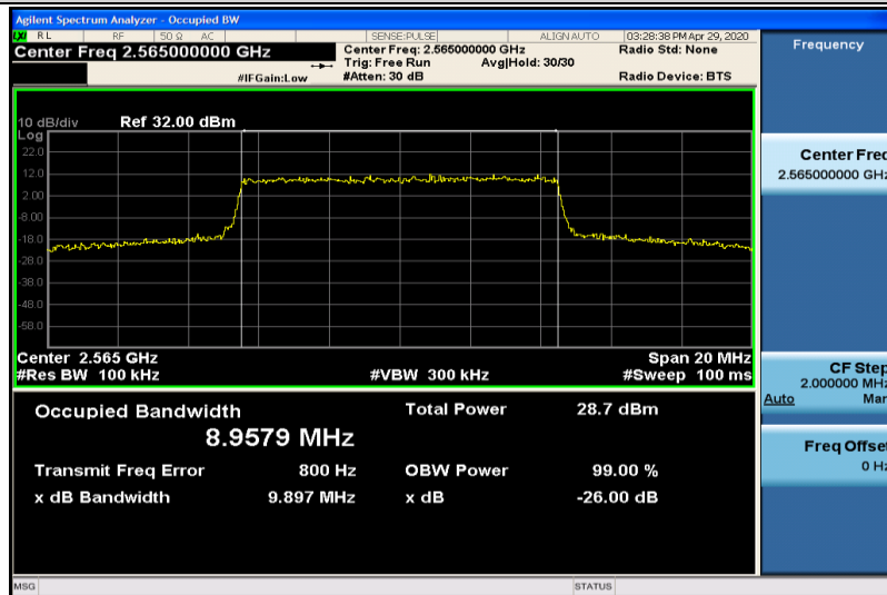
Band7-10MHz-QPSK-21400-50RB#0-8.9579
