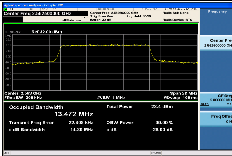
Band41-15MHz-QPSK-40315-75RB#0-13.472
