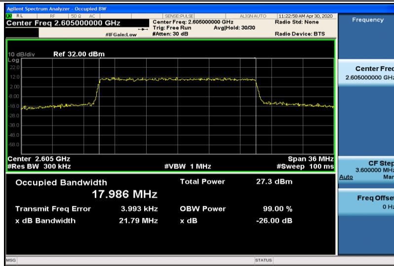
Band41-20MHz-16QAM-40740-100RB#0-17.986
