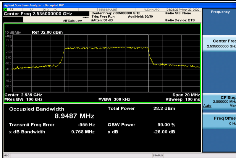
Band7-10MHz-16QAM-21100-50RB#0-8.9487
