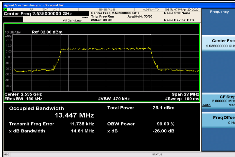
Band7-15MHz-QPSK-21100-75RB#0-13.447
