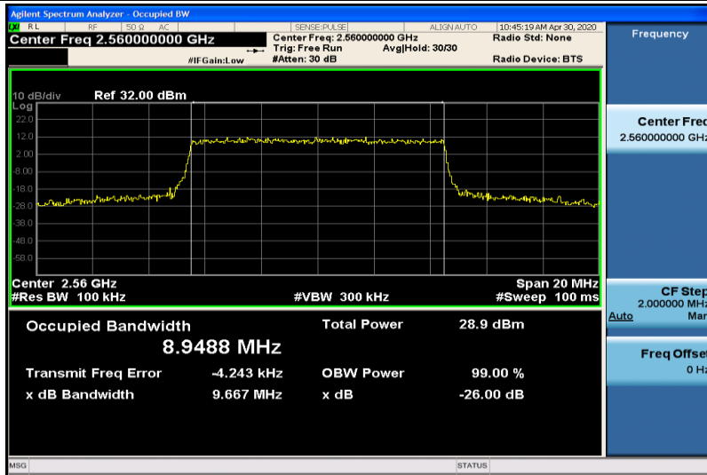
Band41-10MHz-16QAM-40290-50RB#0-8.9488
