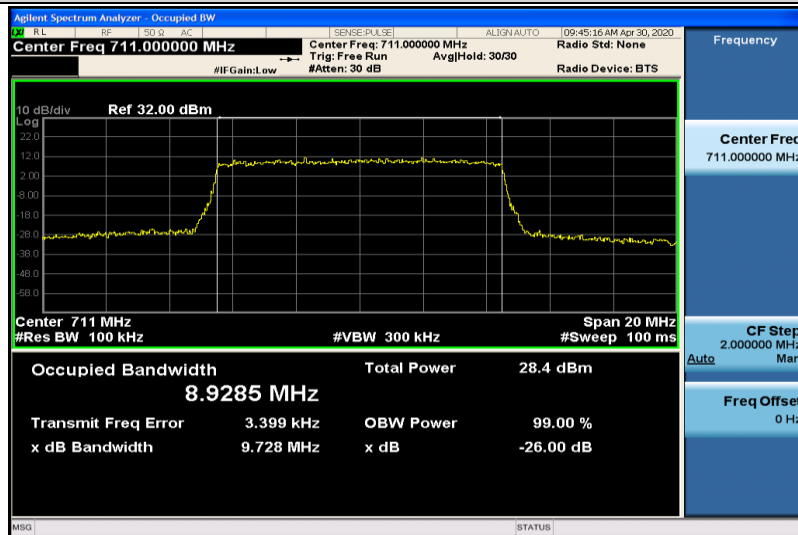
Band17-10MHz-16QAM-23800-50RB#0-8.9285
