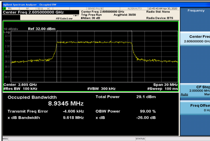
Band41-10MHz-16QAM-40740-50RB#0-8.9345
