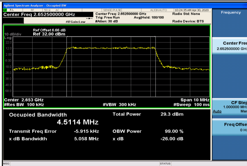
Band41-5MHz-16QAM-41215-25RB#0-4.5114
