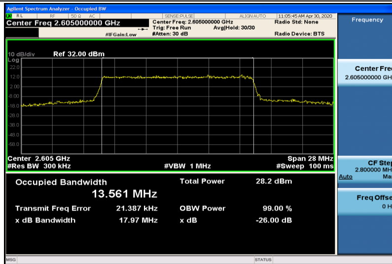
Band41-15MHz-QPSK-40740-75RB#0-13.561
