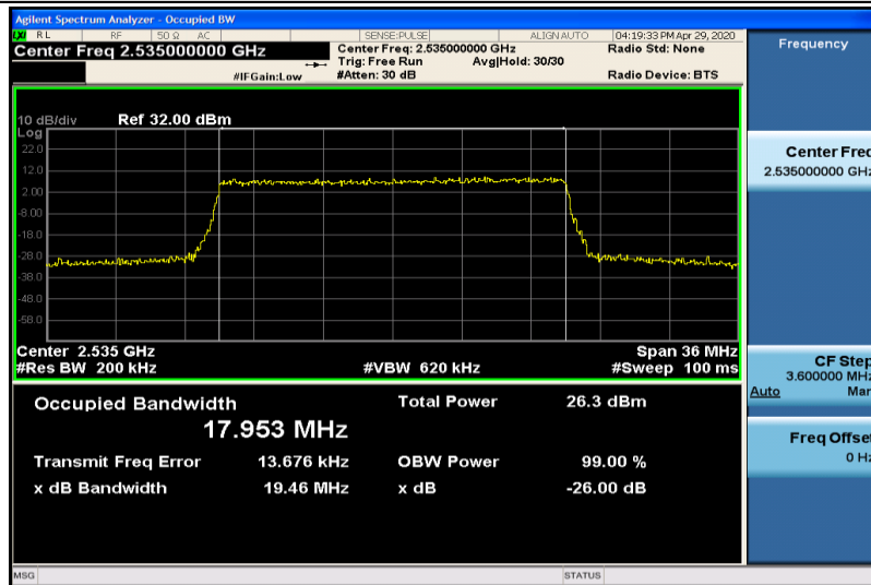
Band7-20MHz-QPSK-21100-100RB#0-17.953
