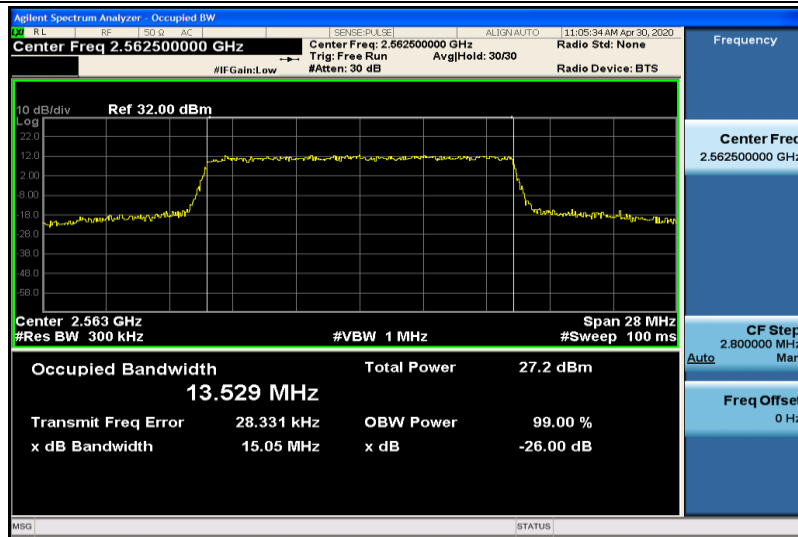
Band41-15MHz-16QAM-40315-75RB#0-13.529
