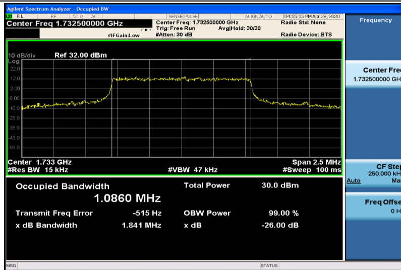
Band4-1.4MHz-16QAM-20175-6RB#0-1.0860
