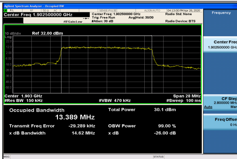
Band2-15MHz-QPSK-19125-75RB#0-13.389
