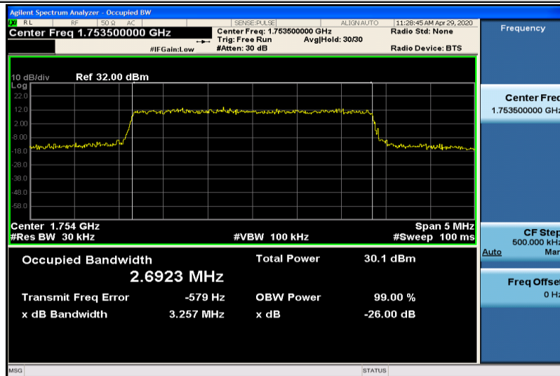
Band4-3MHz-16QAM-20385-15RB#0-2.6923
