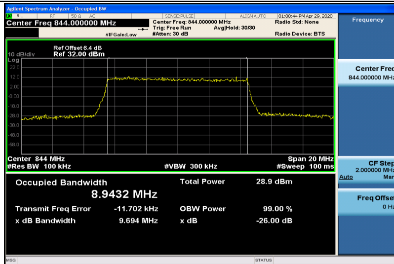
Band5-10MHz-16QAM-20600-50RB#0-8.9432
