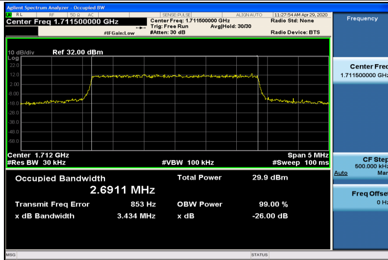
Band4-3MHz-QPSK-19965-15RB#0-2.6911
