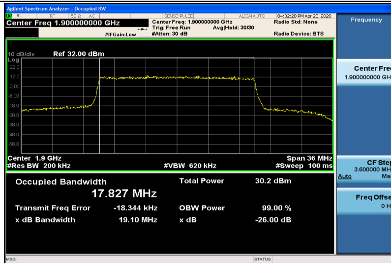
Band2-20MHz-QPSK-19100-100RB#0-17.827
