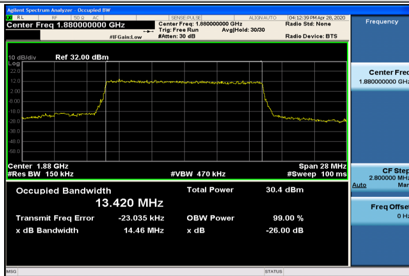
Band2-15MHz-QPSK-18900-75RB#0-13.420
