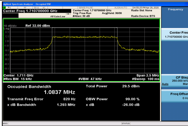
Band4-1.4MHz-QPSK-19957-6RB#0-1.0837
