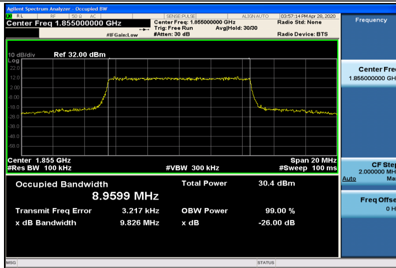
Band2-10MHz-QPSK-18650-50RB#0-8.9599
