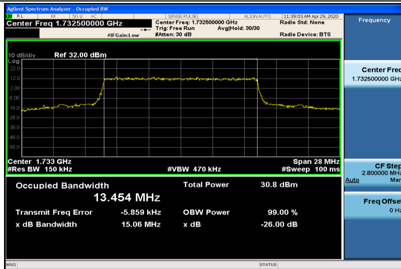
Band4-15MHz-QPSK-20175-75RB#0-13.454
