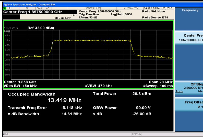
Band2-15MHz-16QAM-18675-75RB#0-13.419
