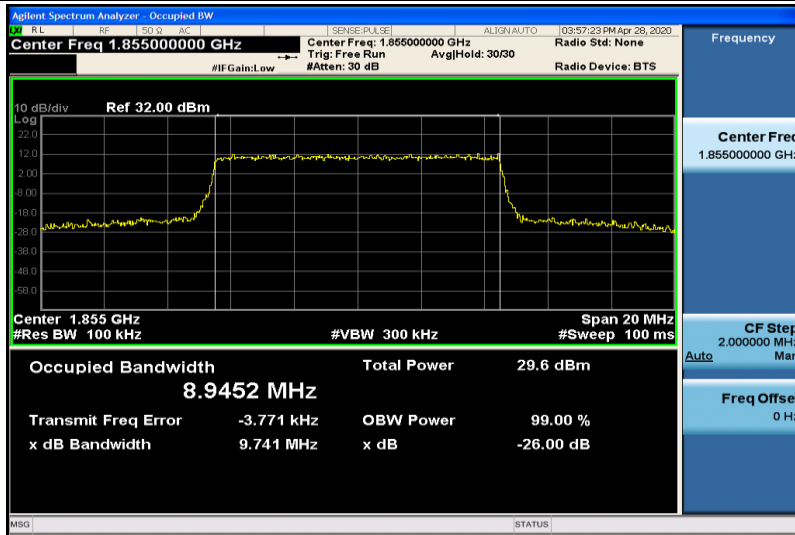
Band2-10MHz-16QAM-18650-50RB#0-8.9452
