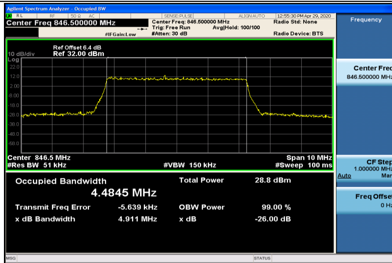
Band5-5MHz-16QAM-20625-25RB#0-4.4845
