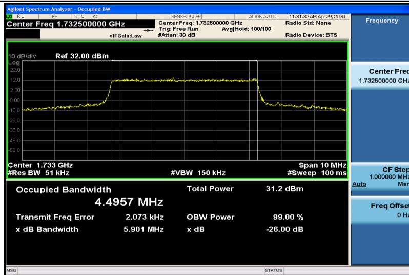
Band4-5MHz-QPSK-17325-25RB#0-4.4957
