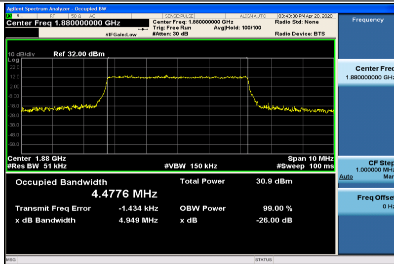
Band2-5MHz-QPSK-18900-25RB#0-4.4776
