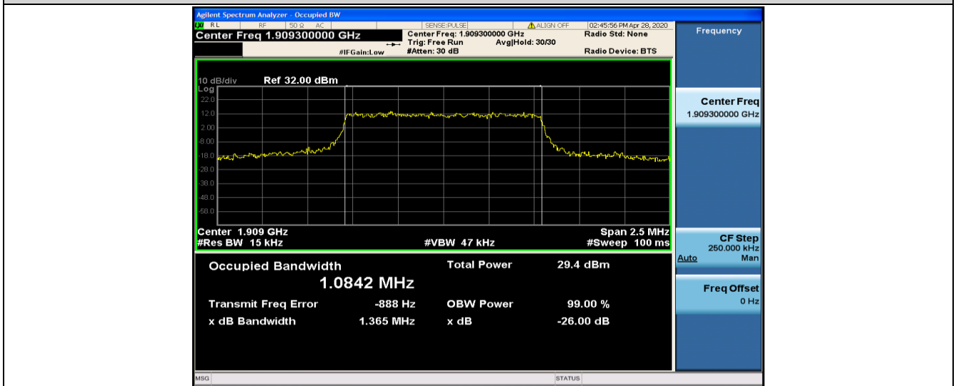
Band2-1.4MHz-QPSK-19193-6RB#0-1.0842
