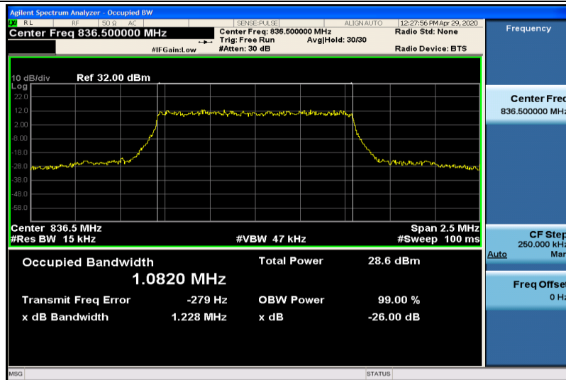
Band5-1.4MHz-QPSK-20525-6RB#0-1.0820
