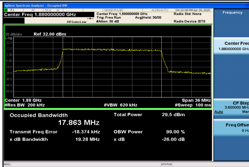
Band2-20MHz-16QAM-18900-100RB#0-17.863
