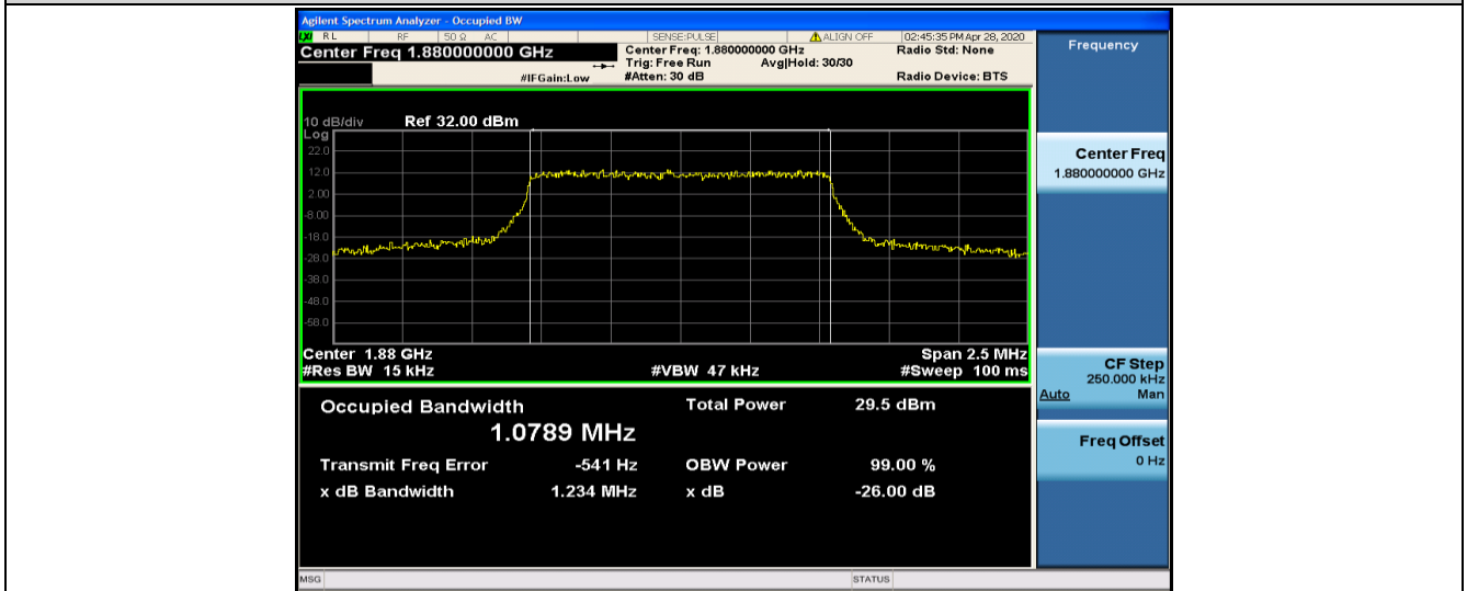
Band2-1.4MHz-QPSK-18900-6RB#0-1.0789
