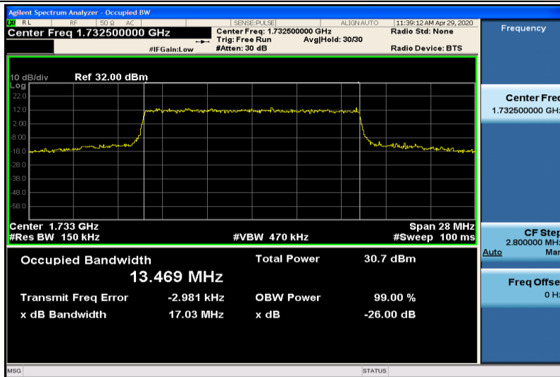
Band4-15MHz-16QAM-20175-75RB#0-13.469
