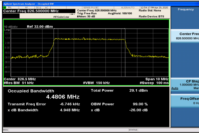
Band5-5MHz-16QAM-20425-25RB#0-4.4806
