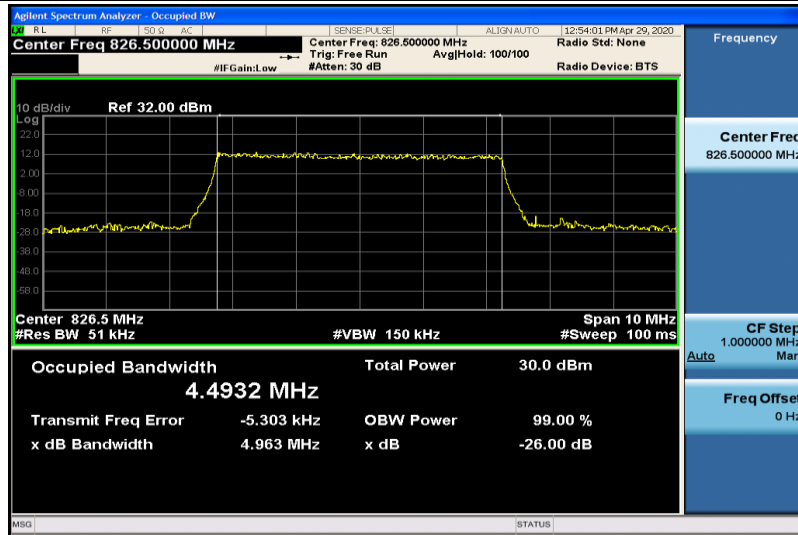
Band5-5MHz-QPSK-20425-25RB#0-4.4932
