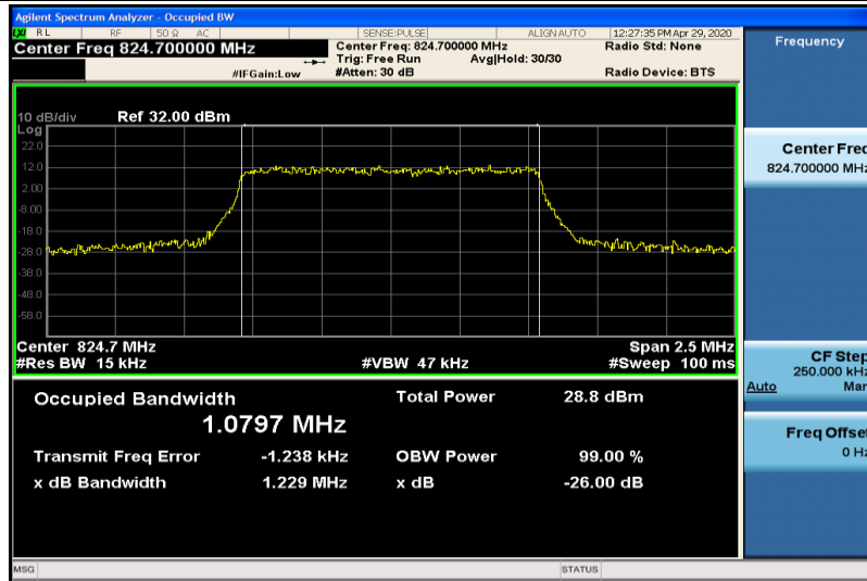
Band5-1.4MHz-QPSK-20407-6RB#0-1.0797
