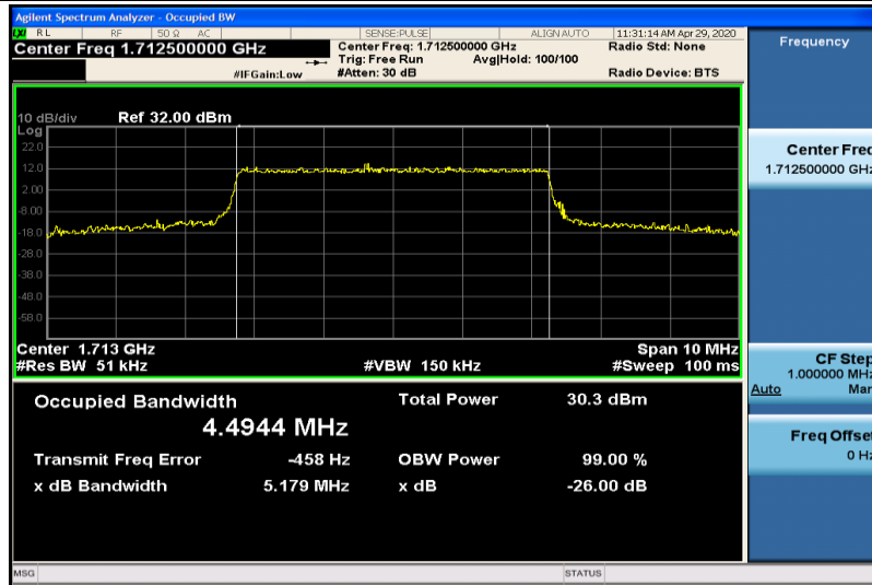
Band4-5MHz-16QAM-19975-25RB#0-4.4944
