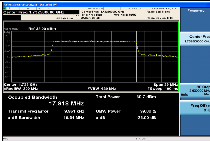
Band4-20MHz-16QAM-20175-100RB#0-17.918
