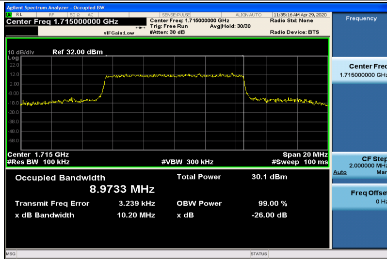
Band4-10MHz-16QAM-20000-50RB#0-8.9733
