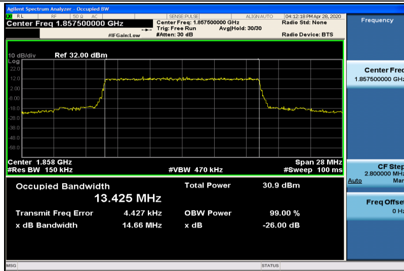
Band2-15MHz-QPSK-18675-75RB#0-13.425
