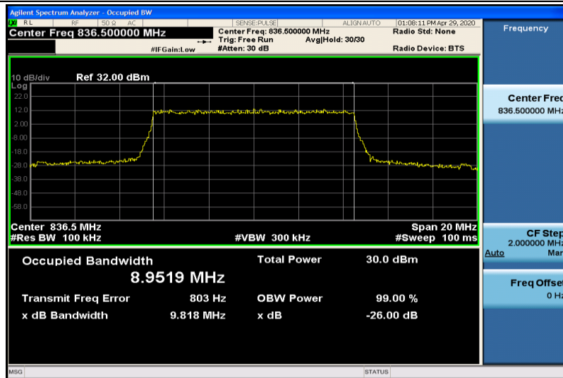
Band5-10MHz-QPSK-20525-50RB#0-8.9519
