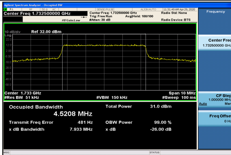
Band4-5MHz-16QAM-20175-25RB#0-4.5208
