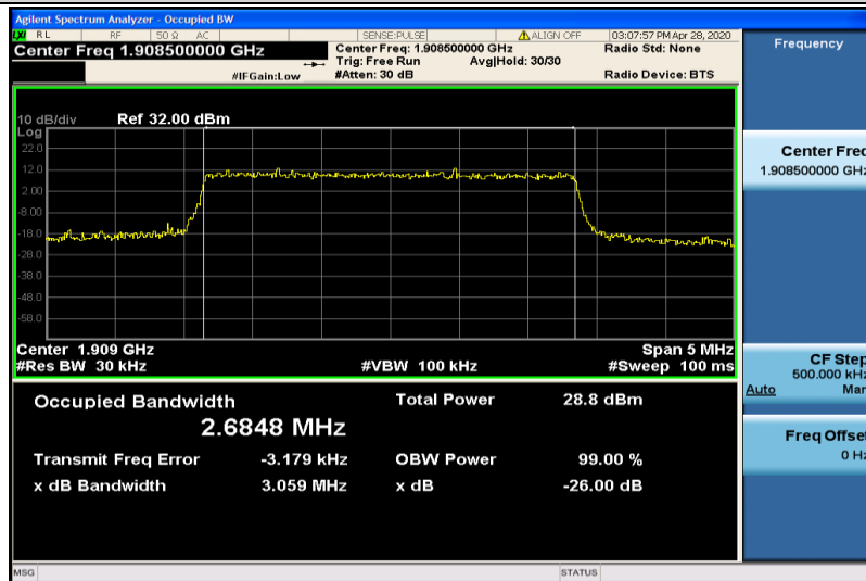
Band2-3MHz-16QAM-19185-15RB#0-2.6848
