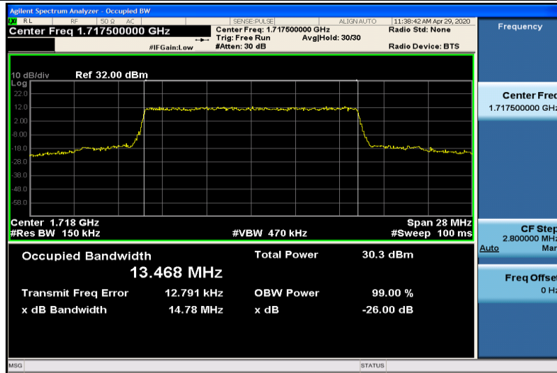
Band4-15MHz-QPSK-20025-75RB#0-13.468
