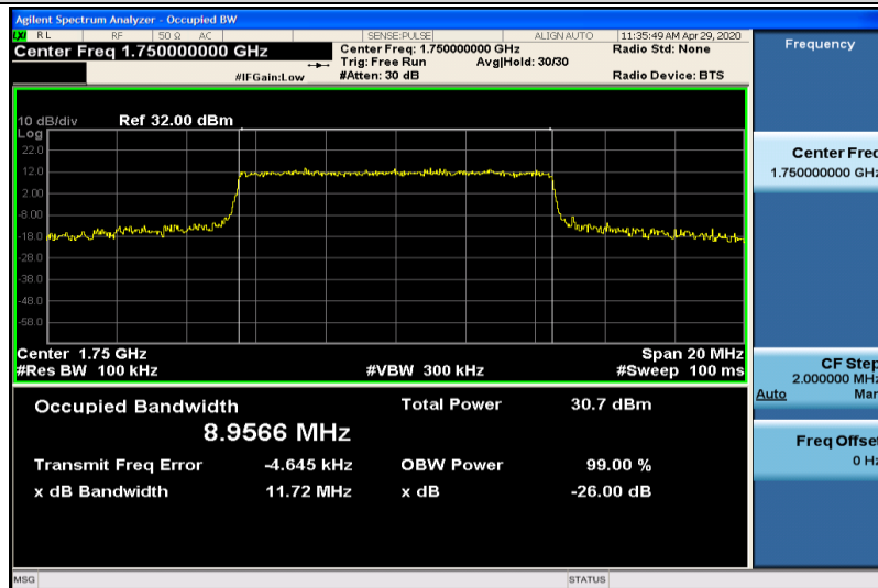
Band4-10MHz-QPSK-20350-50RB#0-8.9566
