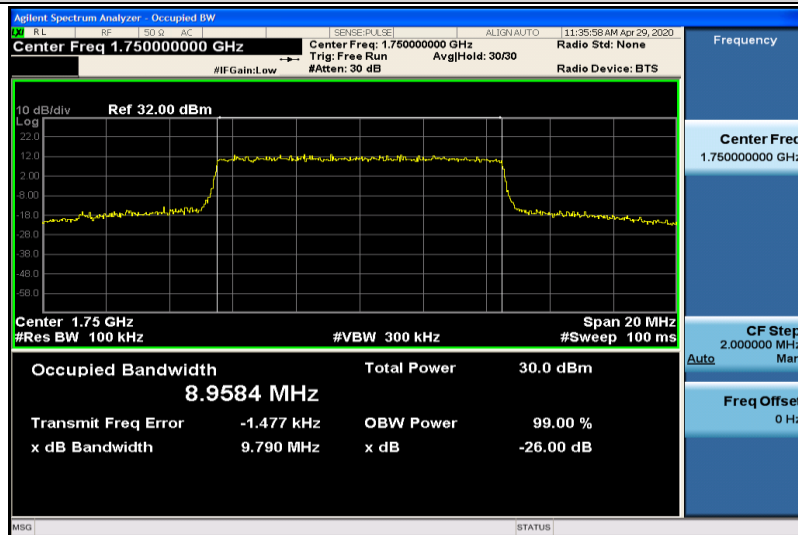
Band4-10MHz-16QAM-20350-50RB#0-8.9584
