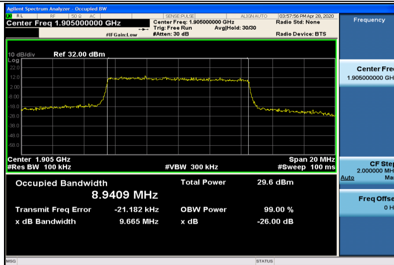
Band2-10MHz-QPSK-19150-50RB#0-8.9409
