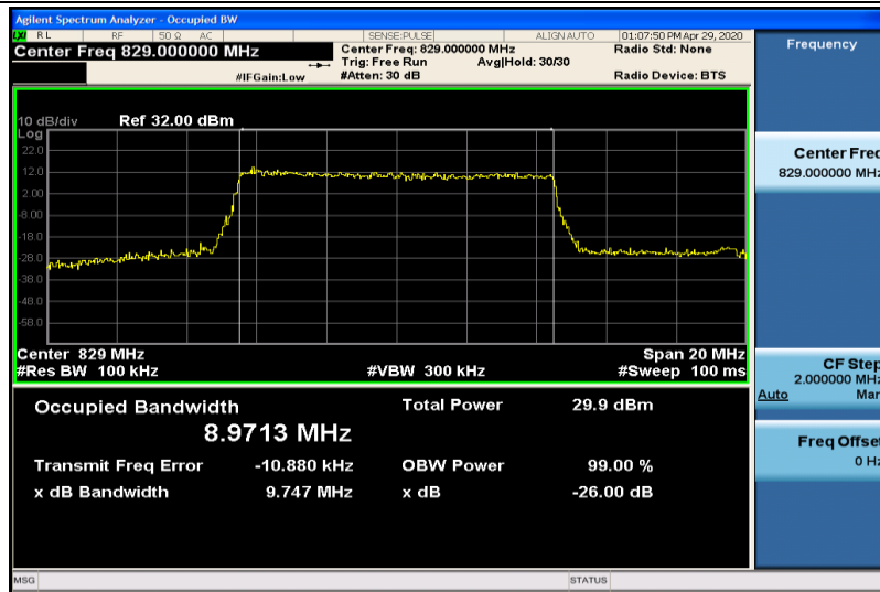
Band5-10MHz-QPSK-20450-50RB#0-8.9713
