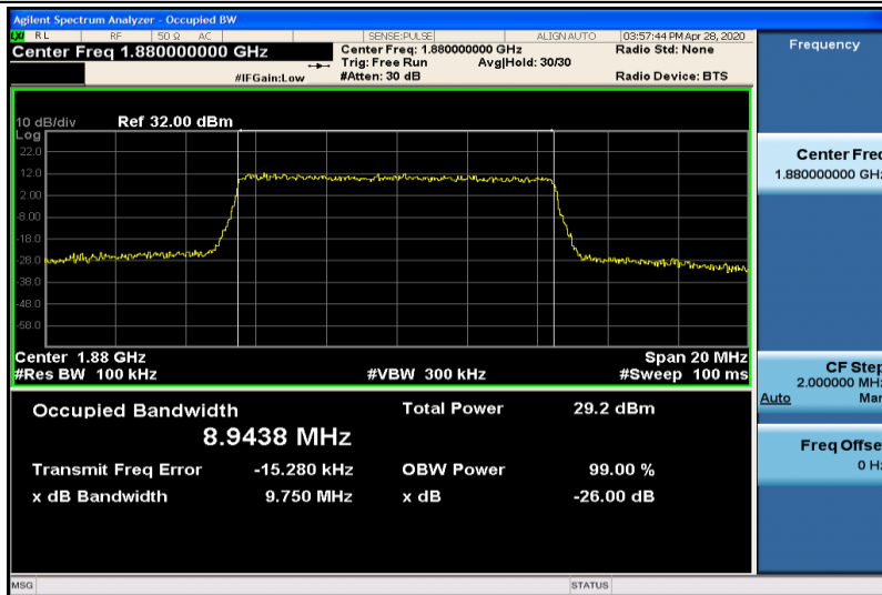
Band2-10MHz-16QAM-18900-50RB#0-8.9438
