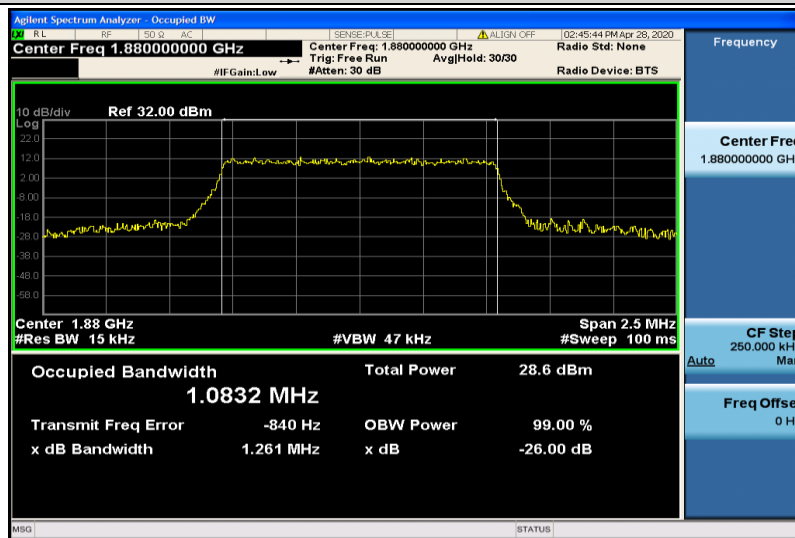
Band2-1.4MHz-16QAM-18900-6RB#0-1.0832
