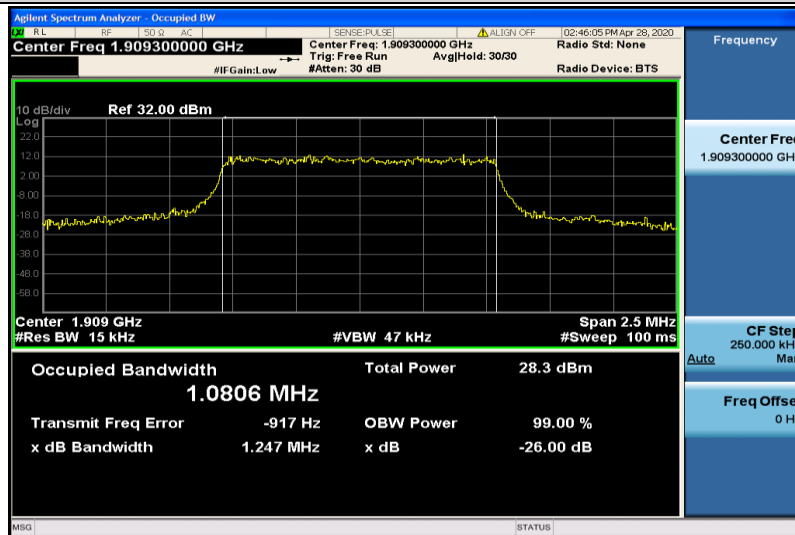
Band2-1.4MHz-16QAM-19193-6RB#0-1.0806
