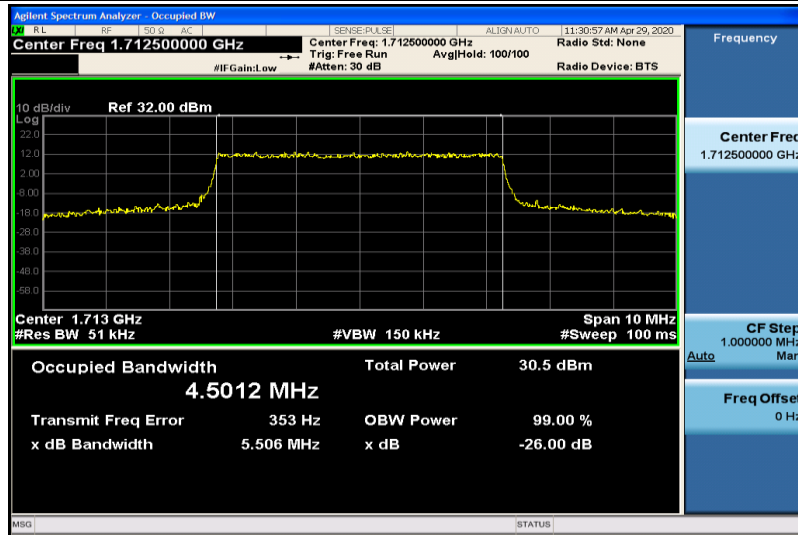
Band4-5MHz-QPSK-19975-25RB#0-4.5012
