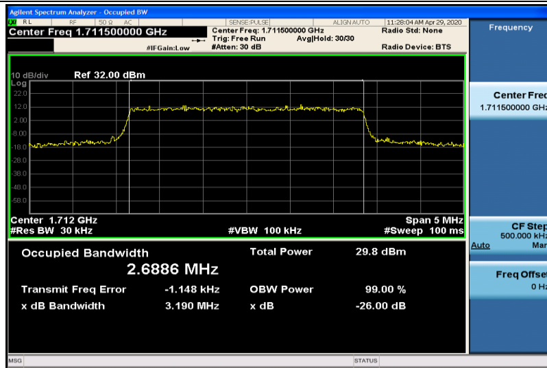
Band4-3MHz-16QAM-19965-15RB#0-2.6886
