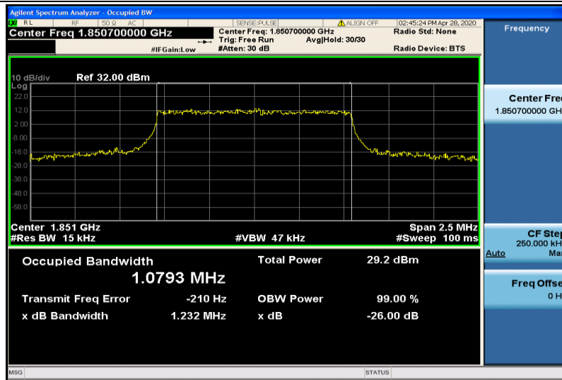
Band2-1.4MHz-16QAM-18607-6RB#0-1.0793
