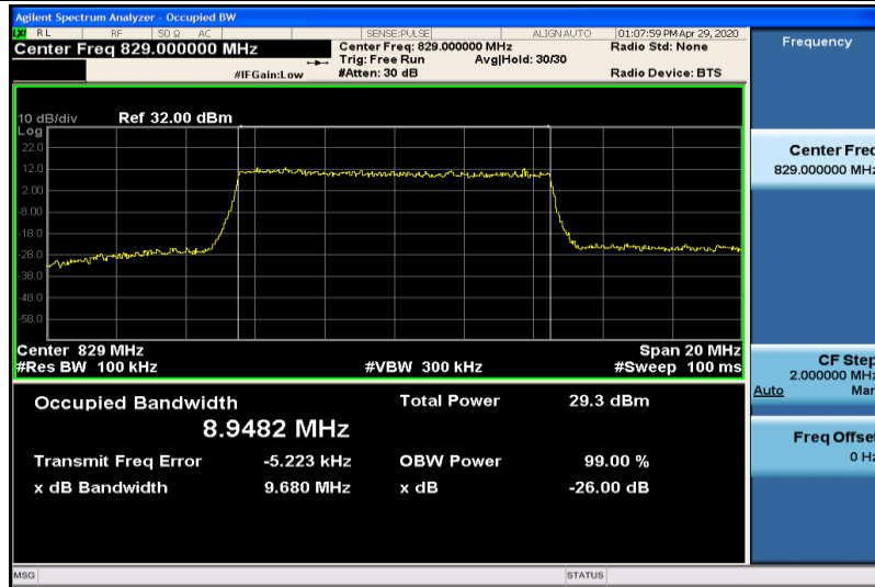
Band5-10MHz-16QAM-20450-50RB#0-8.9482
