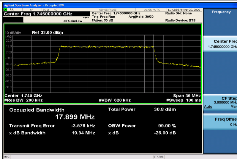
Band4-20MHz-QPSK-20300-100RB#0-17.899
