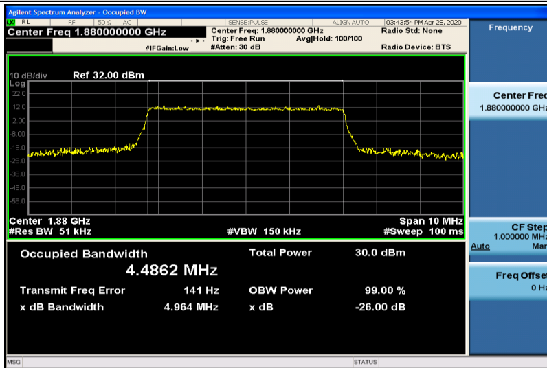
Band2-5MHz-16QAM-18900-25RB#0-4.4862
