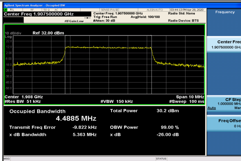
Band2-5MHz-QPSK-19175-25RB#0-4.4885
