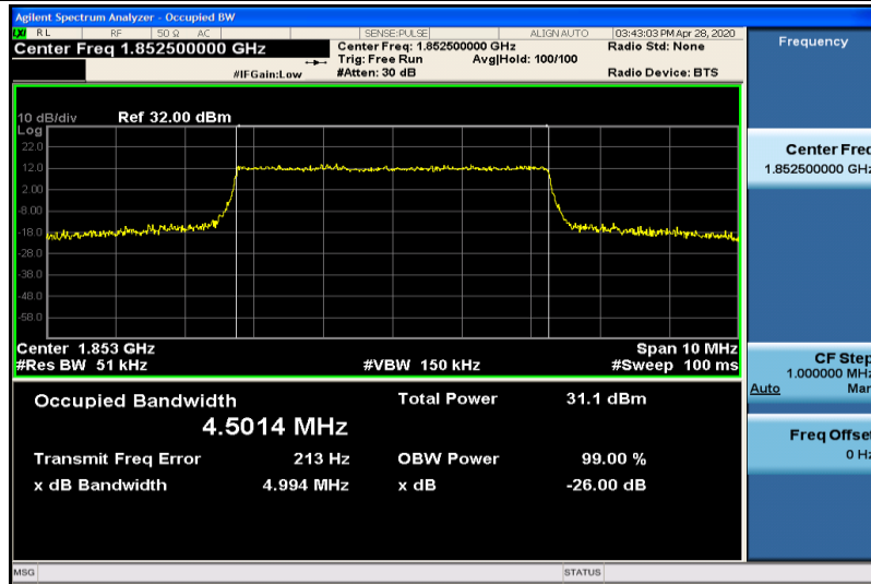
Band2-5MHz-QPSK-18625-25RB#0-4.5014
