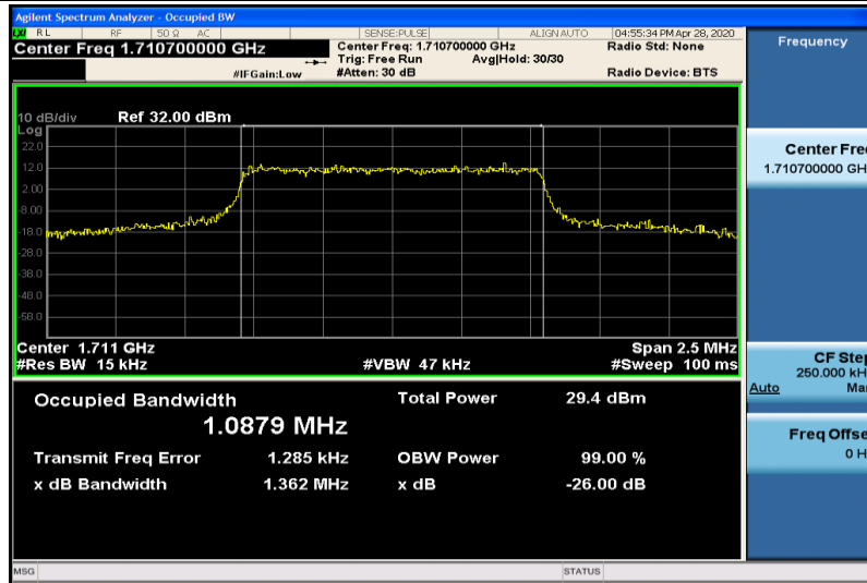
Band4-1.4MHz-16QAM-19957-6RB#0-1.0879
