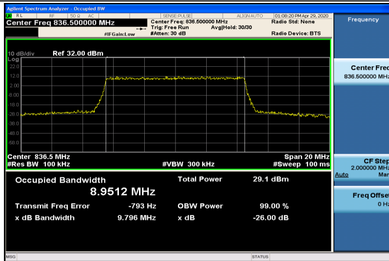
Band5-10MHz-16QAM-20525-50RB#0-8.9512
