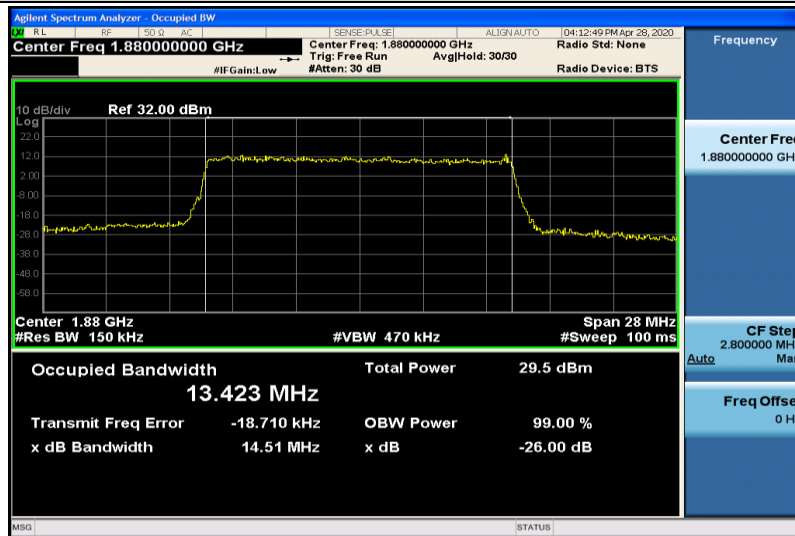
Band2-15MHz-16QAM-18900-75RB#0-13.423
