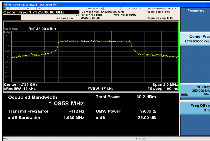
Band4-1.4MHz-QPSK-20175-6RB#0-1.0858
