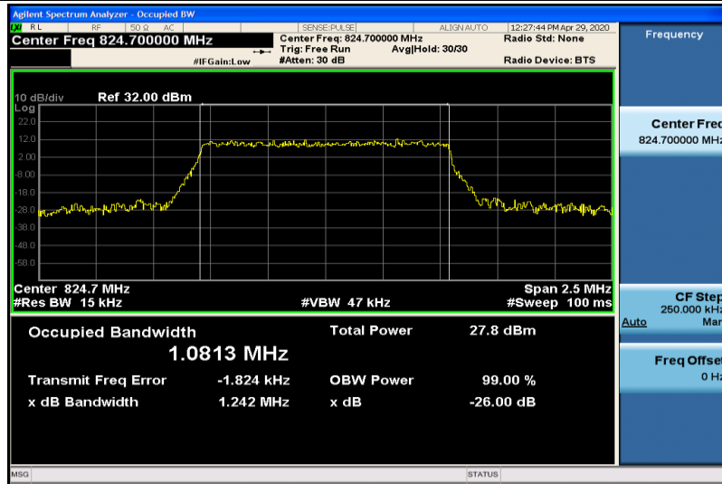
Band5-1.4MHz-16QAM-20407-6RB#0-1.0813
