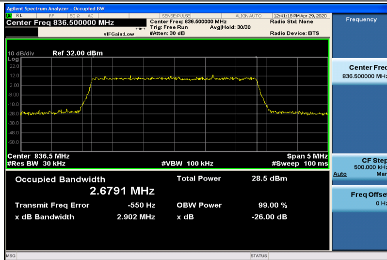
Band5-3MHz-16QAM-20525-15RB#0-2.6791
