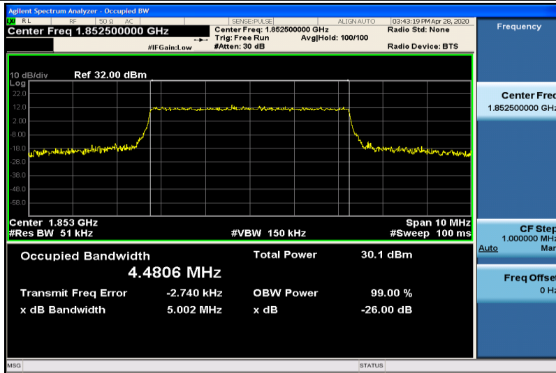
Band2-5MHz-16QAM-18625-25RB#0-4.4806
