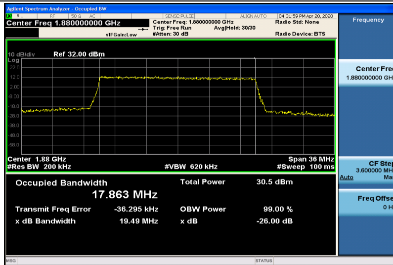
Band2-20MHz-QPSK-18900-100RB#0-17.863
