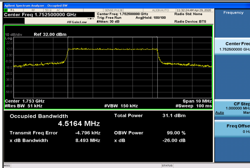
Band4-5MHz-16QAM-20375-25RB#0-4.5164
