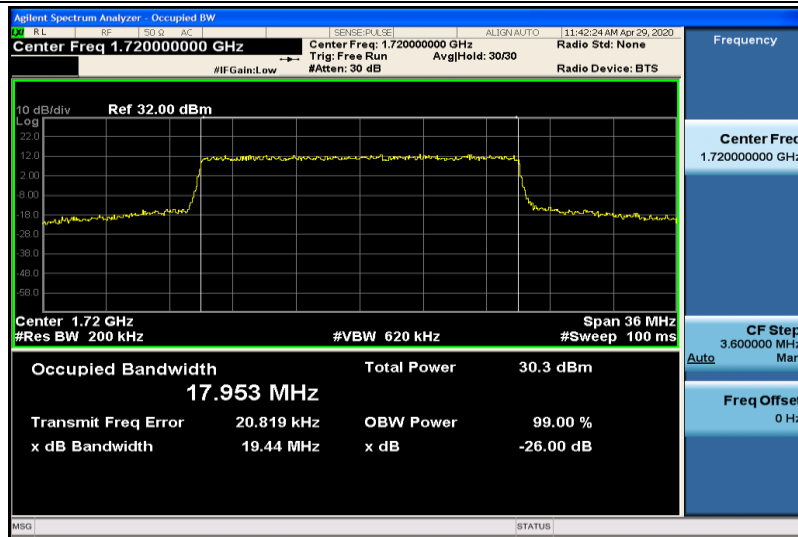
Band4-20MHz-16QAM-20050-100RB#0-17.953
