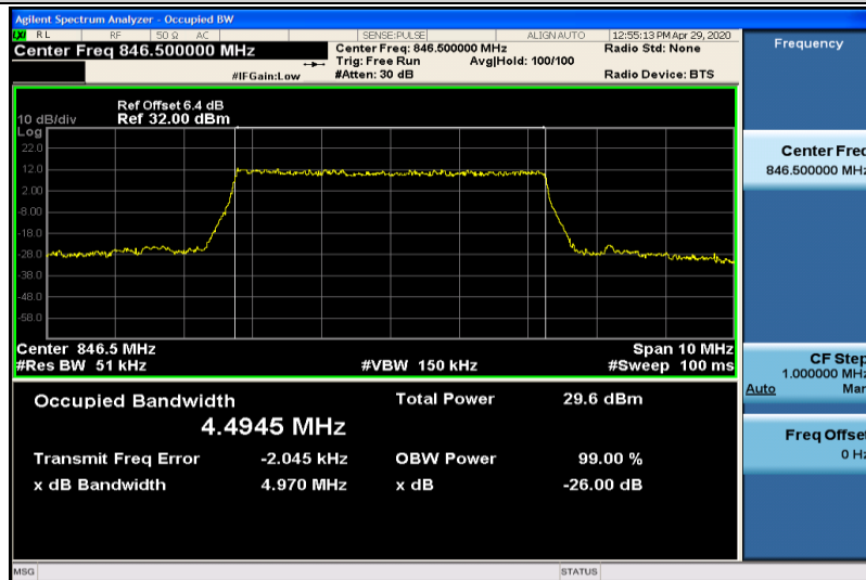
Band5-5MHz-QPSK-20625-25RB#0-4.4945
