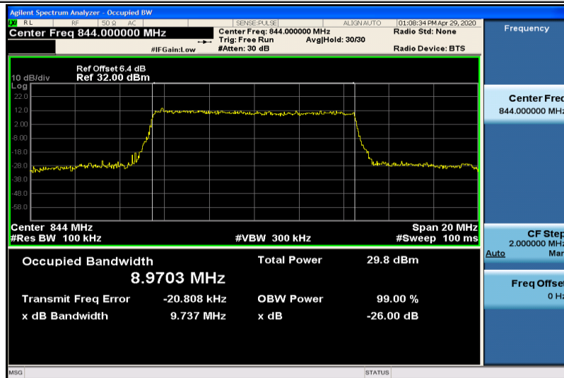
Band5-10MHz-QPSK-20600-50RB#0-8.9703
