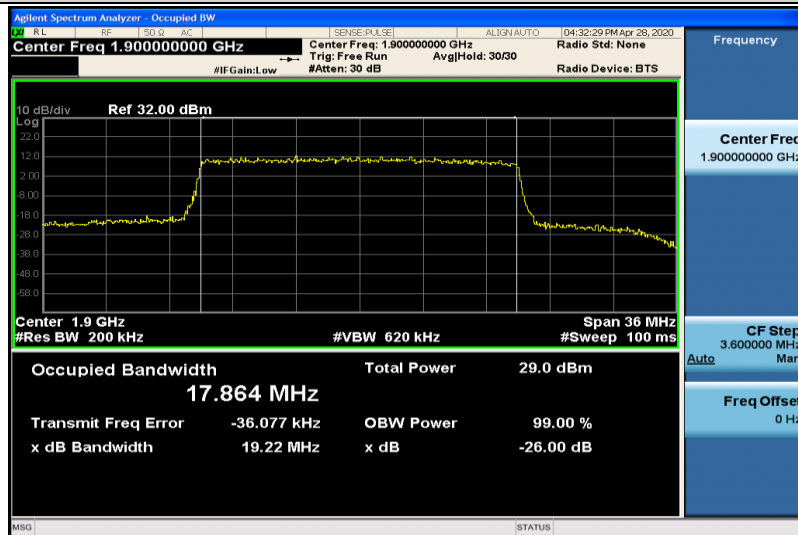
Band2-20MHz-16QAM-19100-100RB#0-17.864
