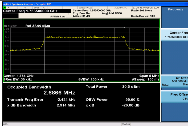
Band4-3MHz-QPSK-20385-15RB#0-2.6866
