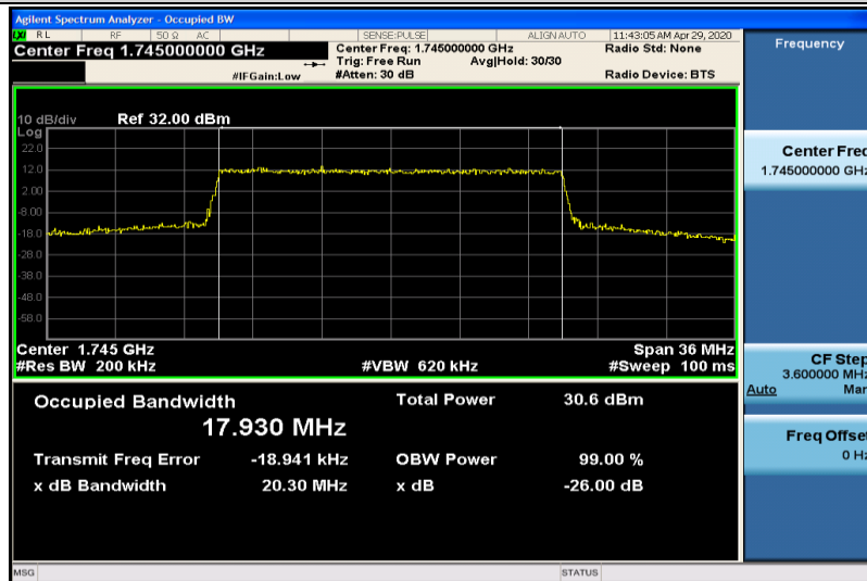
Band4-20MHz-16QAM-20300-100RB#0-17.930
