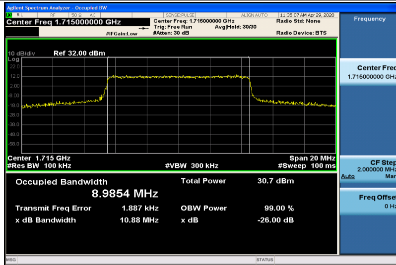
Band4-10MHz-QPSK-20000-50RB#0-8.9854
