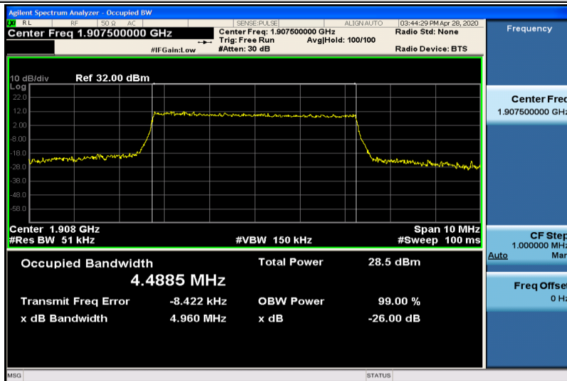
Band2-5MHz-16QAM-19175-25RB#0-4.4885
