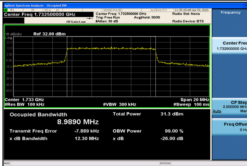
Band4-10MHz-QPSK-20175-50RB#0-8.9890
