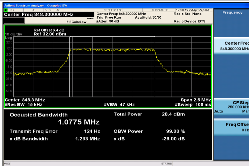
Band5-1.4MHz-QPSK-20643-6RB#0-1.0775
