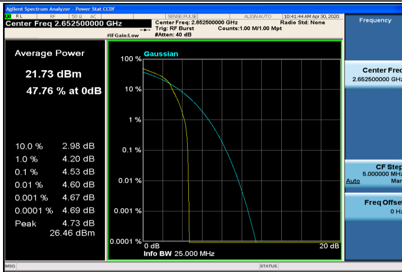
Band41-5MHz-16QAM-41215-1RB#0
