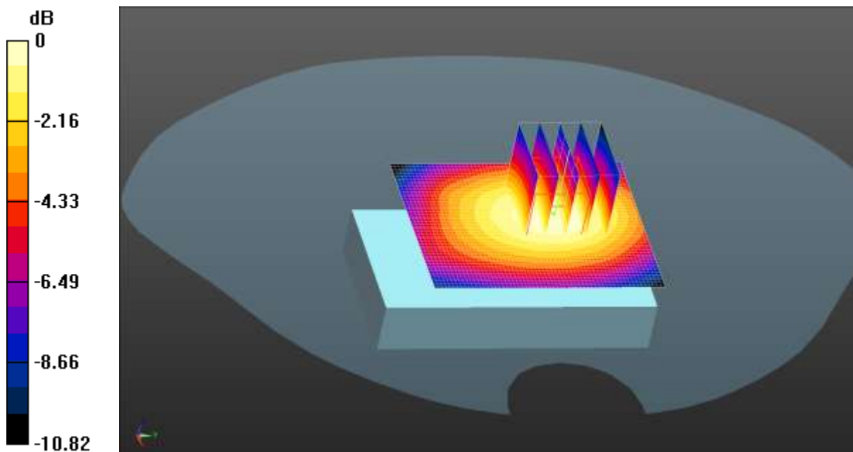
0 dB = 0.994 W/kg = -0.03 dBW/kg
