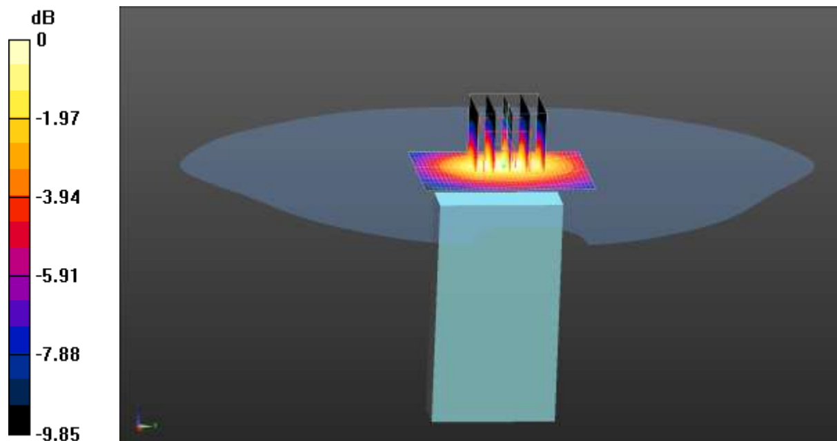
0 dB = 0.420 W/kg = -3.77 dBW/kg
