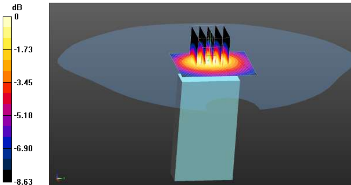
0 dB = 0.454 W/kg = -3.43 dBW/kg
