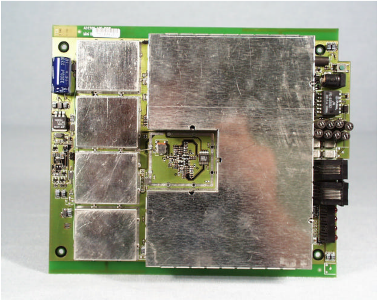
Component Side of the Four Antenna unit (with RF covers installed)
