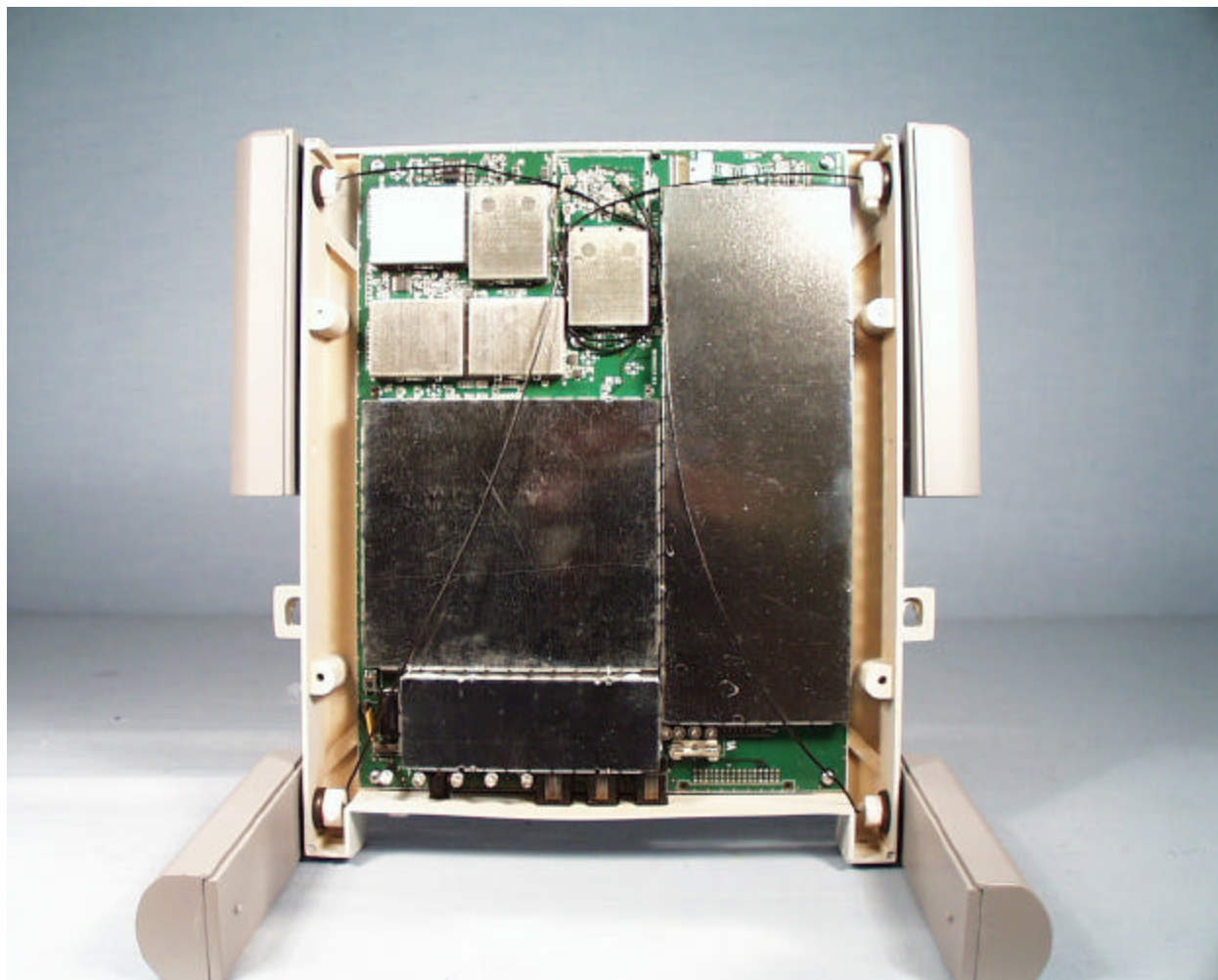
Front inside view of the 530014-759-100
