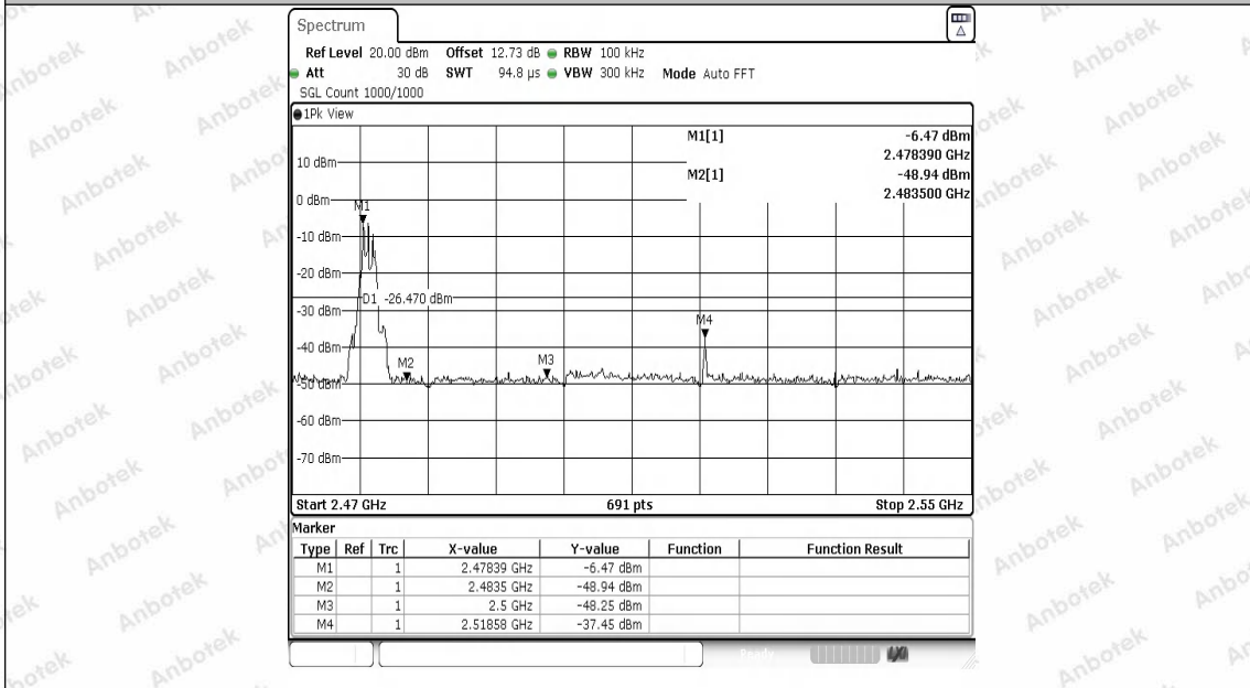
2.4G-Ant1-2479-PASS
