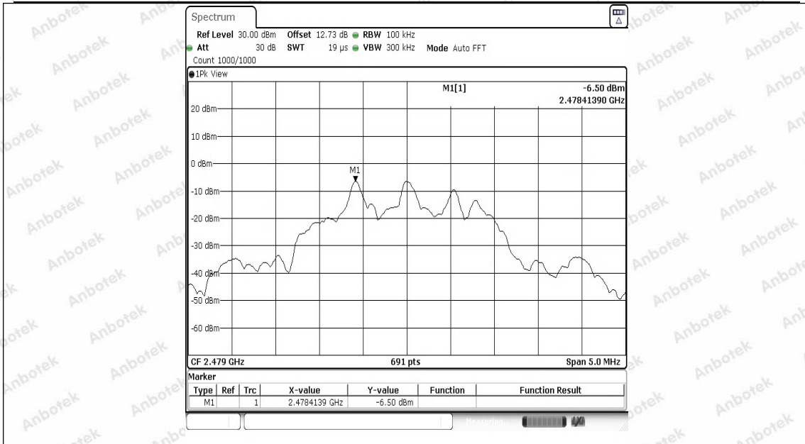
2.4G-Ant1-2479-0~Reference-PASS
