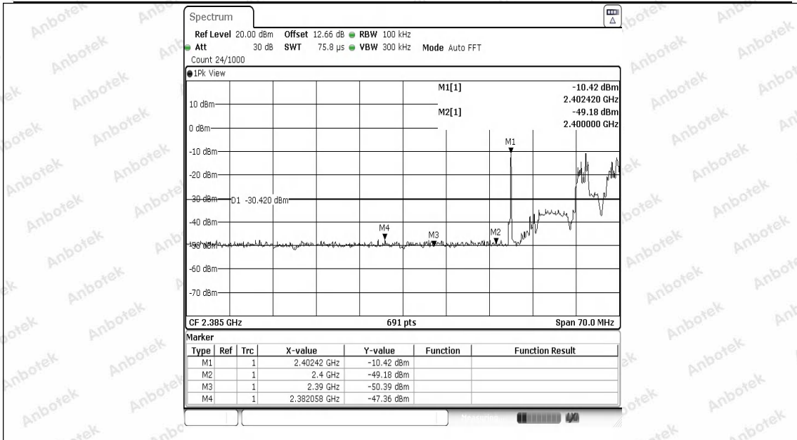
2.4G-Ant1-Hop_2403-PASS
