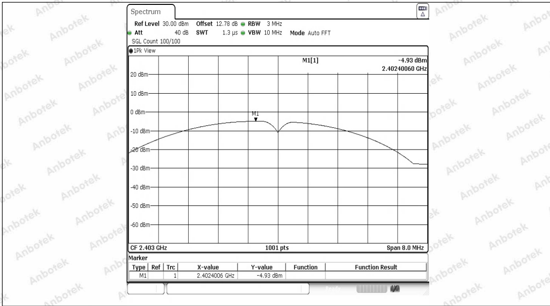
2.4G-Ant1-2403-PASS
