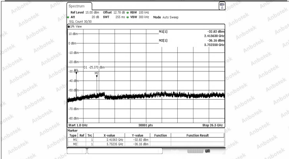
2.4G-Ant1-2403-1000~26500-PASS
