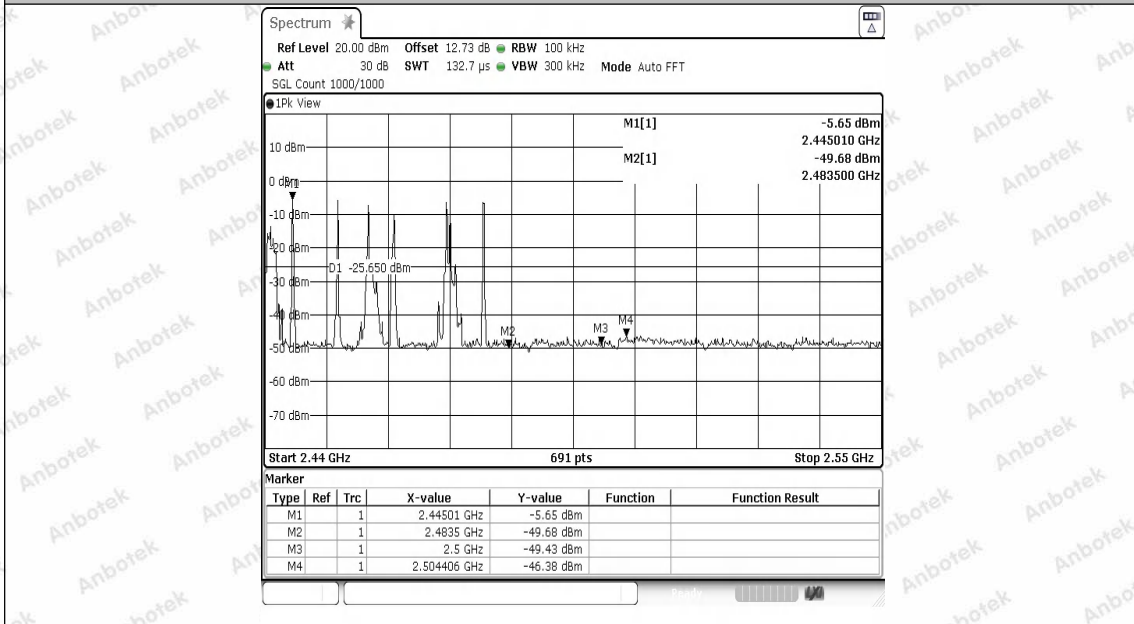
2.4G-Ant1-Hop_2479-PASS
