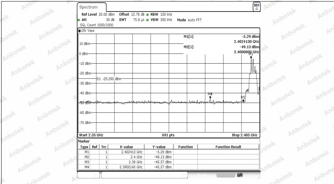
2.4G-Ant1-2403-PASS
