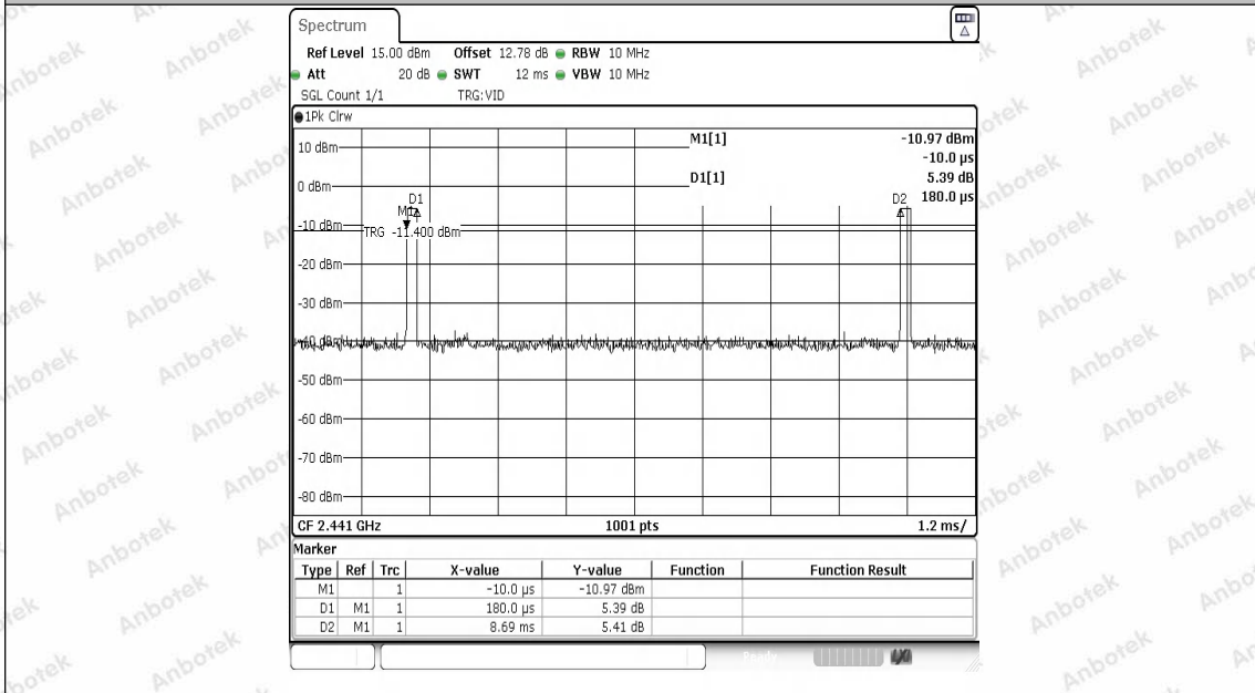
NTNV-2.4G-Ant1-2441
