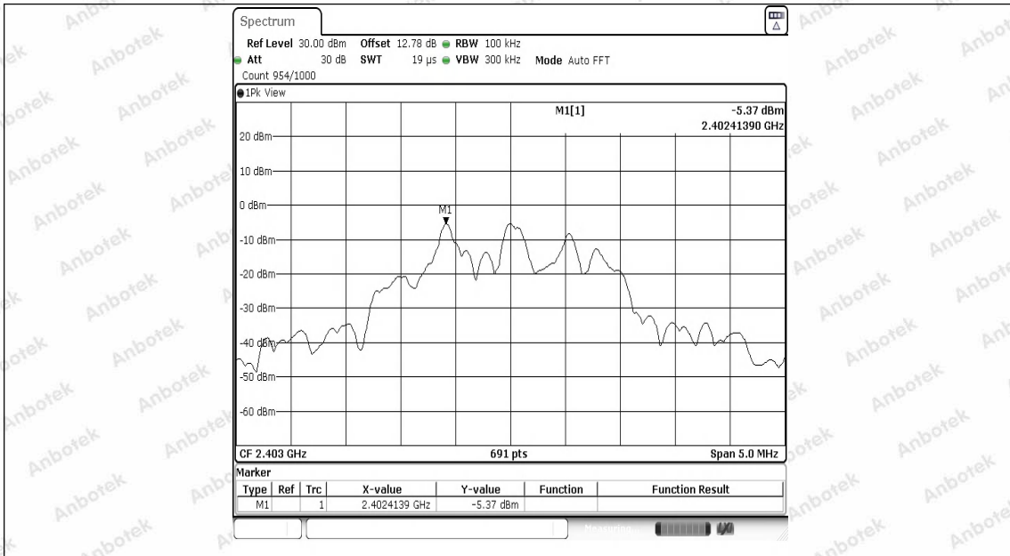
2.4G-Ant1-2403-0~Reference-PASS
