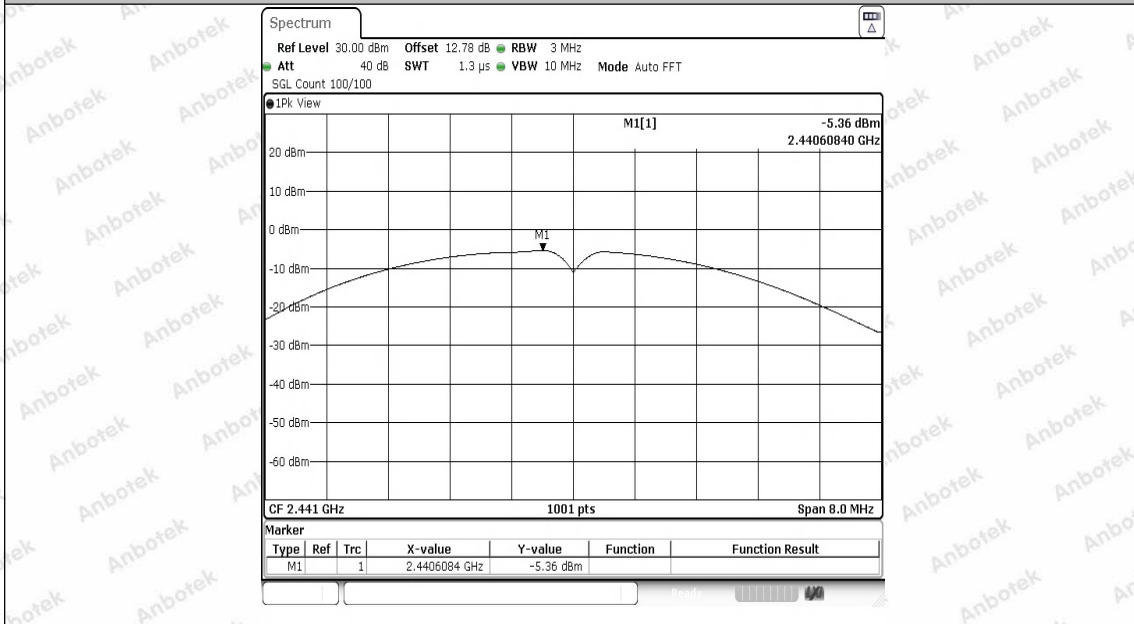
2.4G-Ant1-2441-PASS
