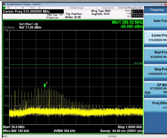
2.4G_Ant1_2440_30~1000
