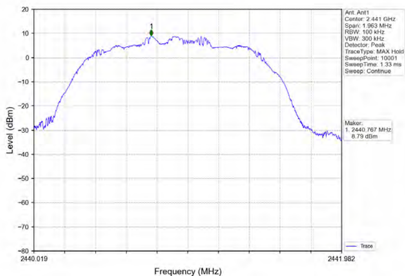
8DPSK_3DH5_MCH_2441MHz_Ant1_NTNV
