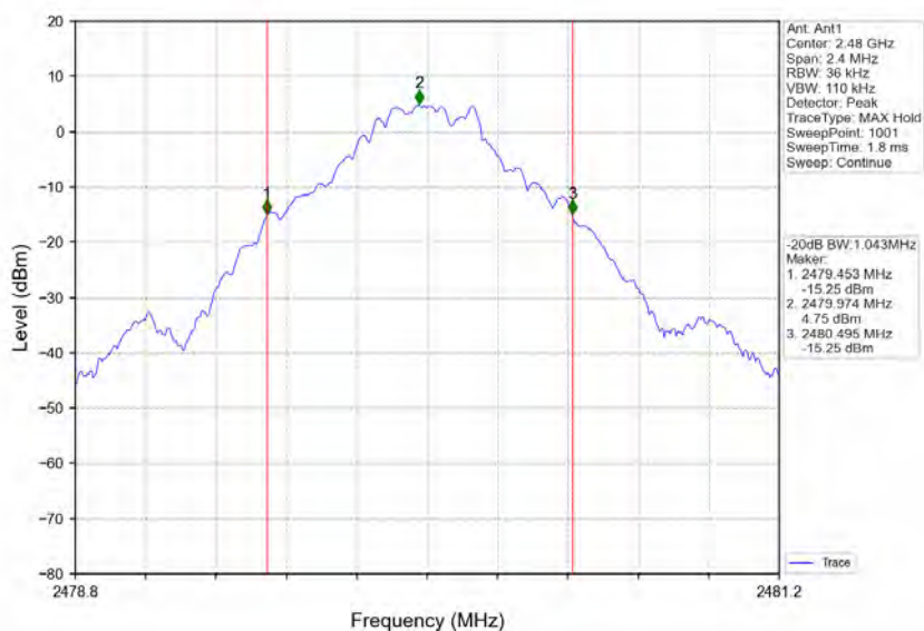
Pi/4DQPSK 2DH5_HCH_2480MHz_Ant1_NTNV
