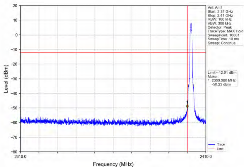
Pi/4DQPSK_2DH5_LCH_2402MHz_Ant1_NTNV
