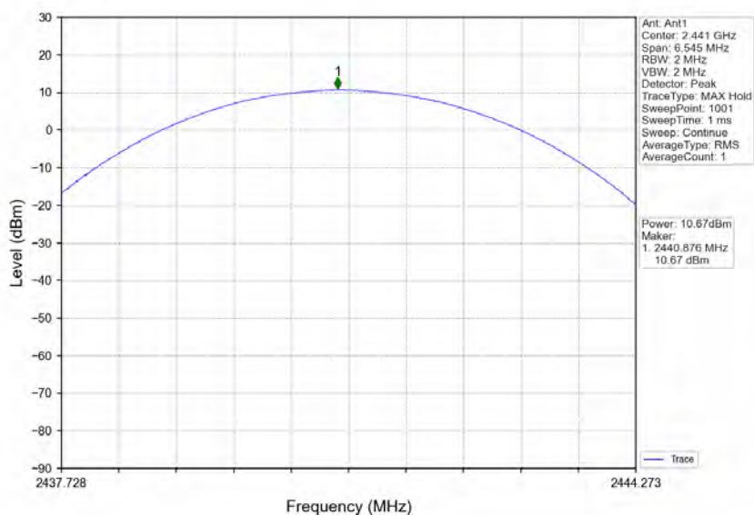
8DPSK 3DH5_MCH_2441MHz_Ant1_NTNV
