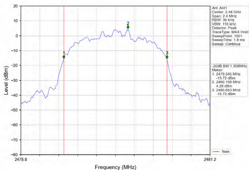
8DPSK_3DH5_HCH_2480MHz_Ant1_NTNV
