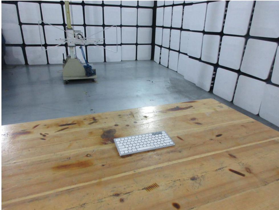
FCC ID: GV3M01502-K Photo of Radiation Emission Test
