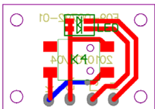
Button PCB TOP
