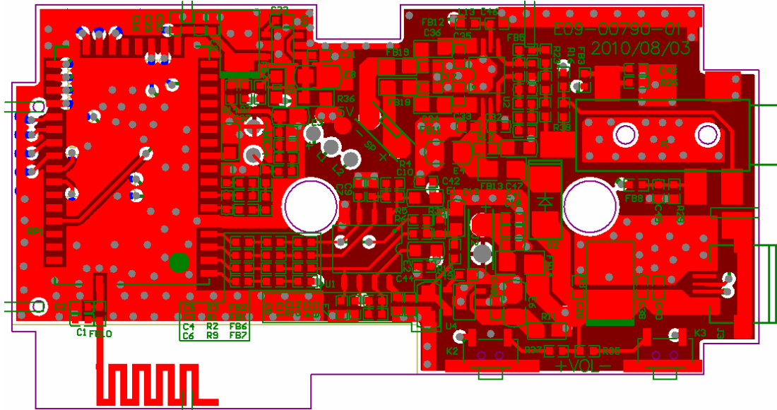
MAIN PCB TOP
