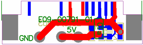
Connector PCB TOP
