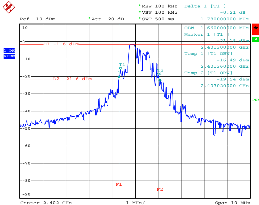
20 dB/99% Bandwidth Plot on 2402 MHz
