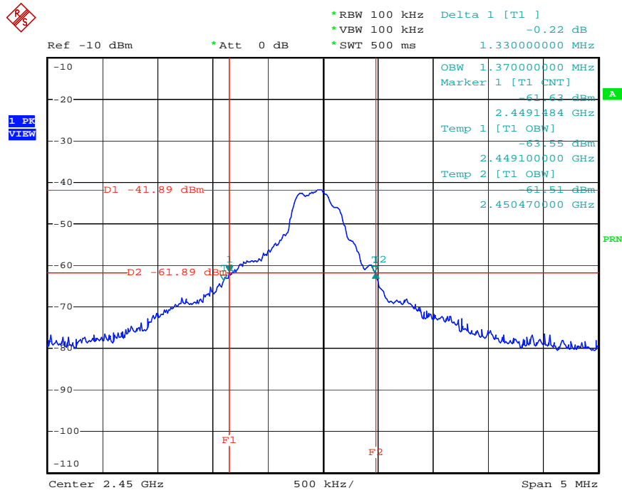
20 dB/99% Bandwidth Plot on 2450 MHz
