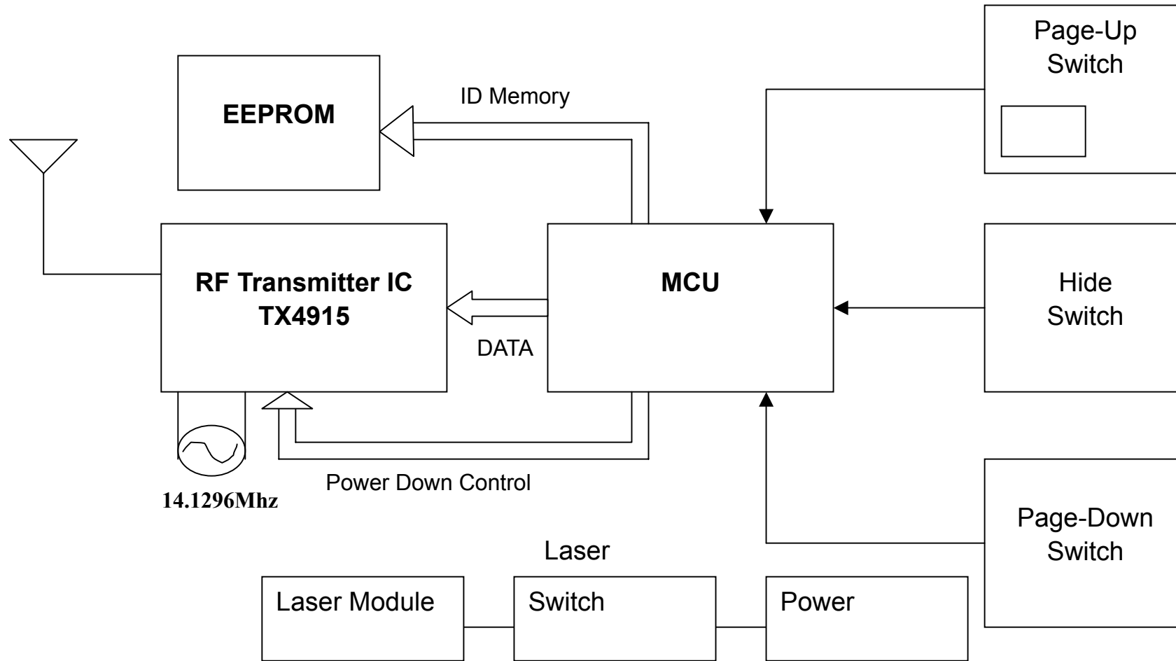
900Mhz Presenter Transmitter System Block
