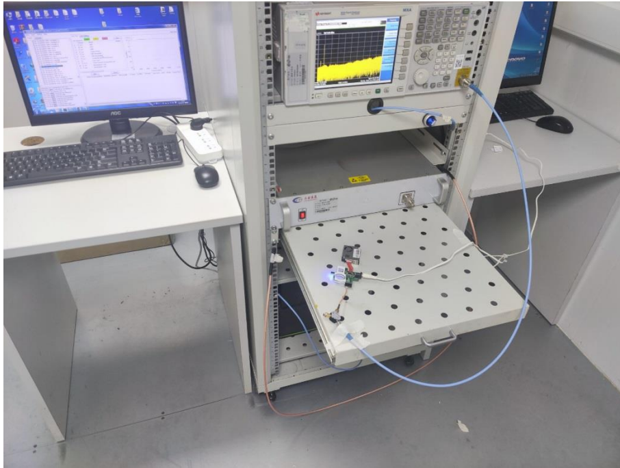
Conducted Test-2.4G
