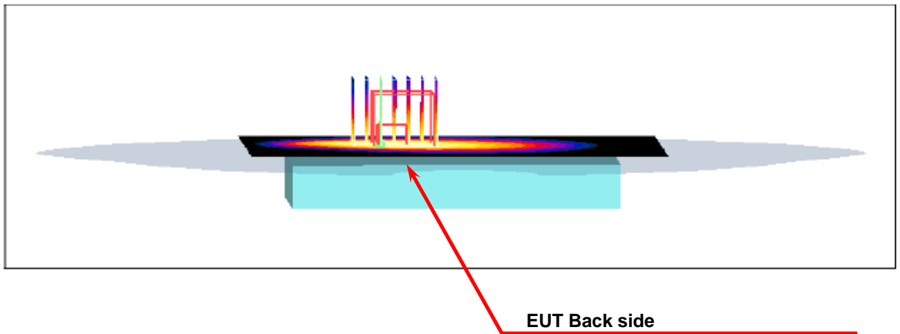
Figure 8. Body SAR Test Setup (Flat Section)
