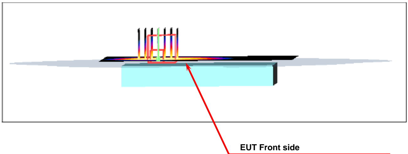
Figure 7. Body SAR Test Setup (Flat Section)
