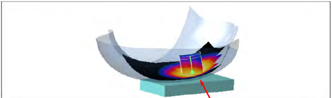
Figure 1. Right Head SAR Test Setup (Cheek)
