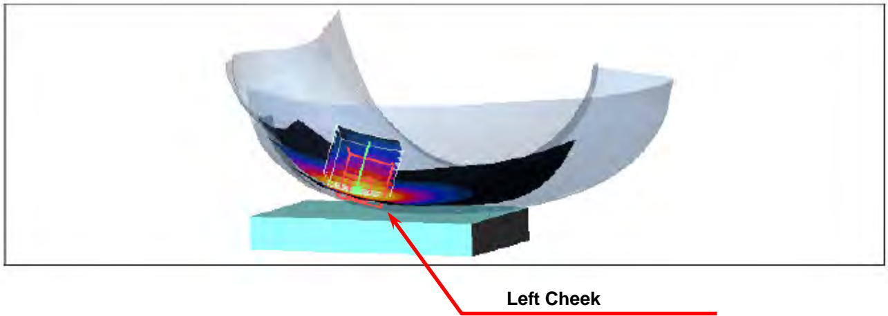
Figure 3. Left Head SAR Test Setup (Cheek)
