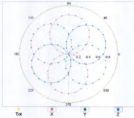
f=600 MHz,TEM
