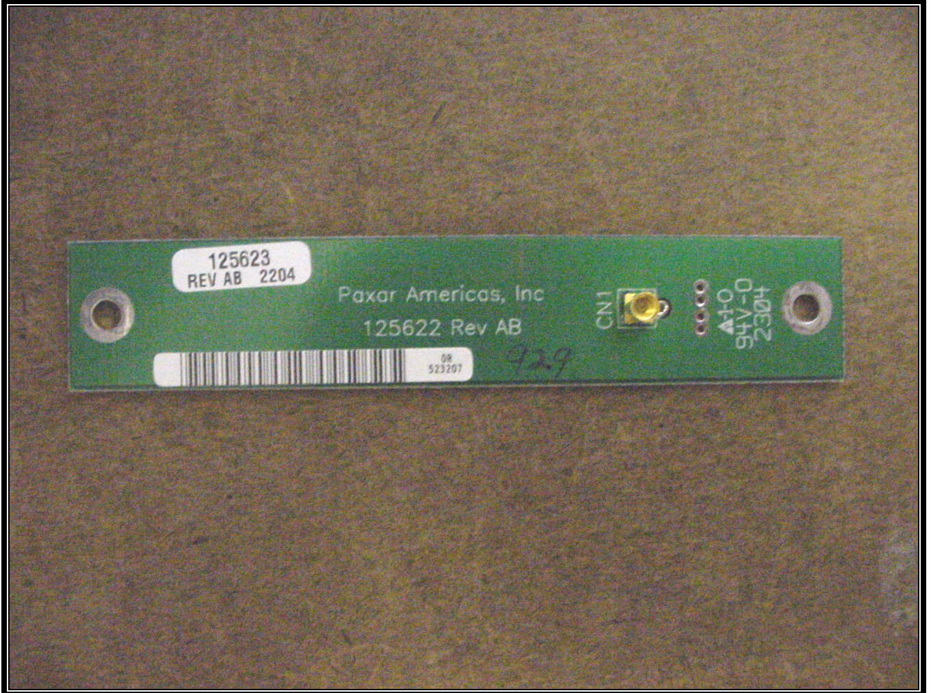
PHOTOGRAPH 11: ANTENNA BACK
