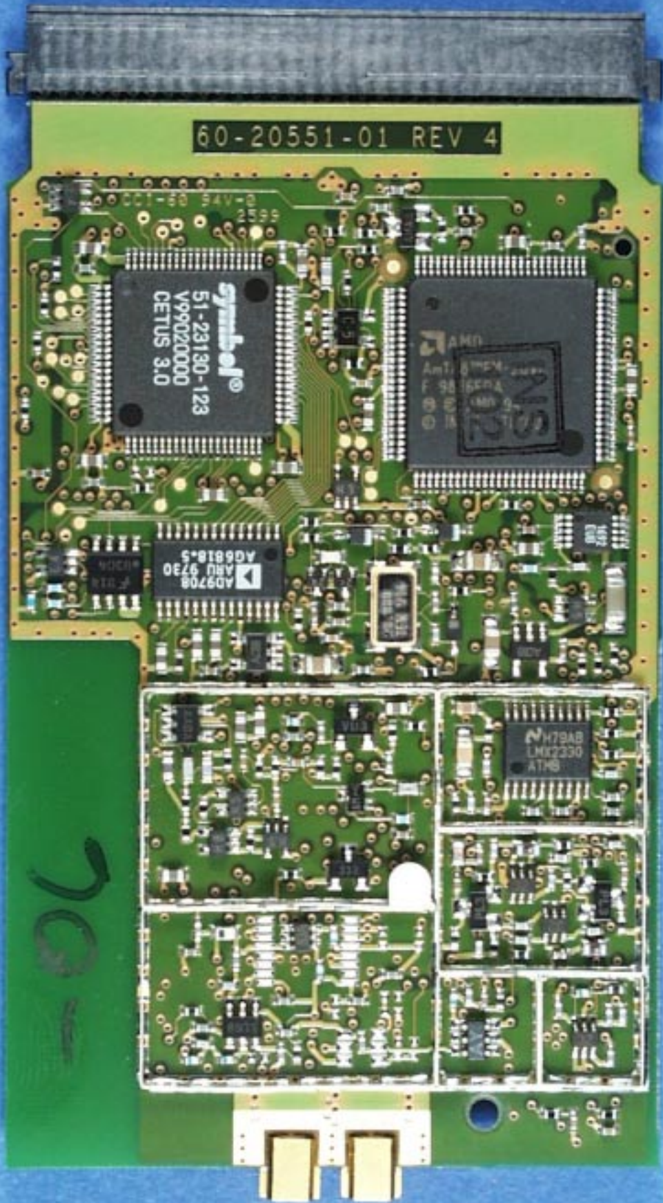
Model LA3021-100 Front View without Shields
