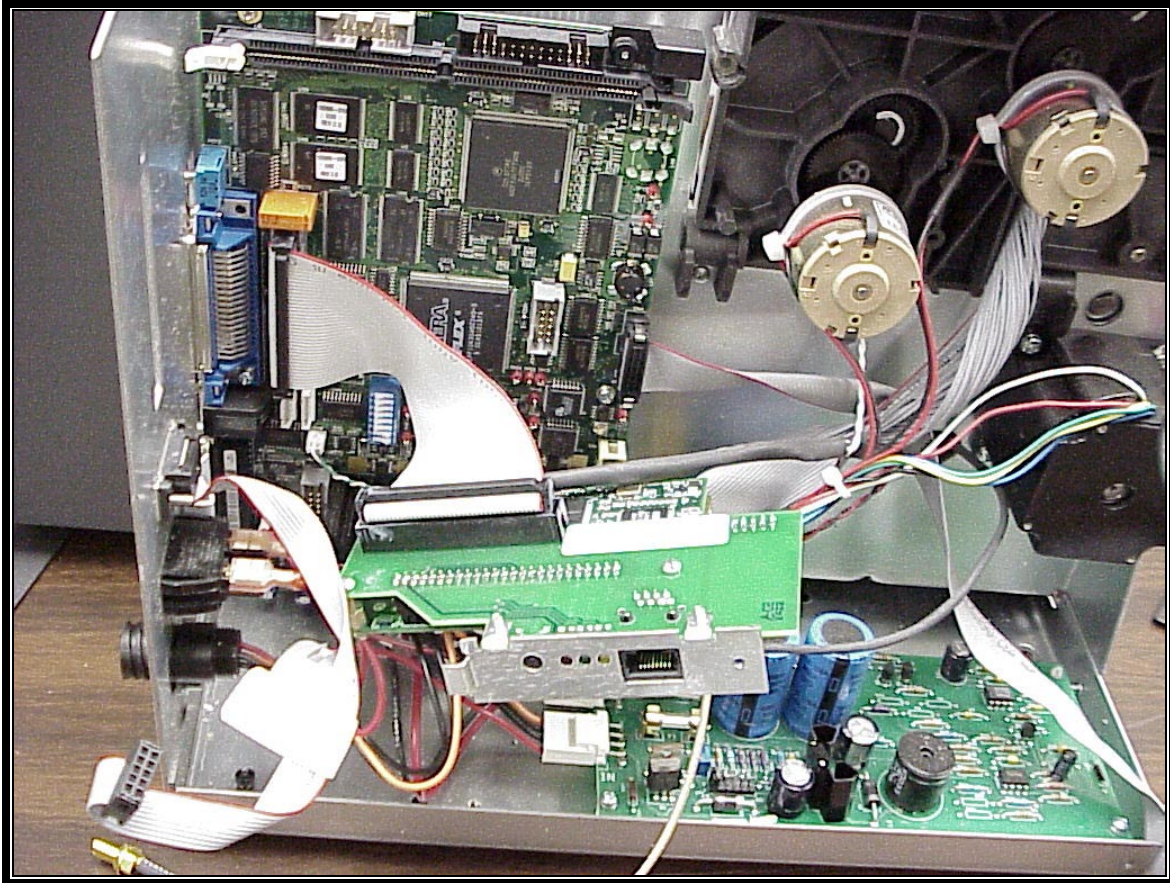
PHOTOGRAPH 29: PRINT SERVER PLUGGED INTO MOUNTED MAIN PCB IN HOST
