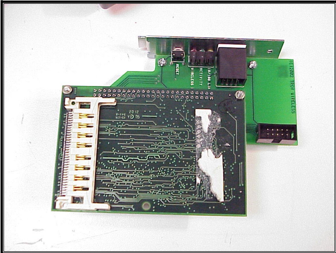
PHOTOGRAPH 25: COMPLETE PRINT SERVER REAR VIEW WITH WLAN CARD REMOVED
