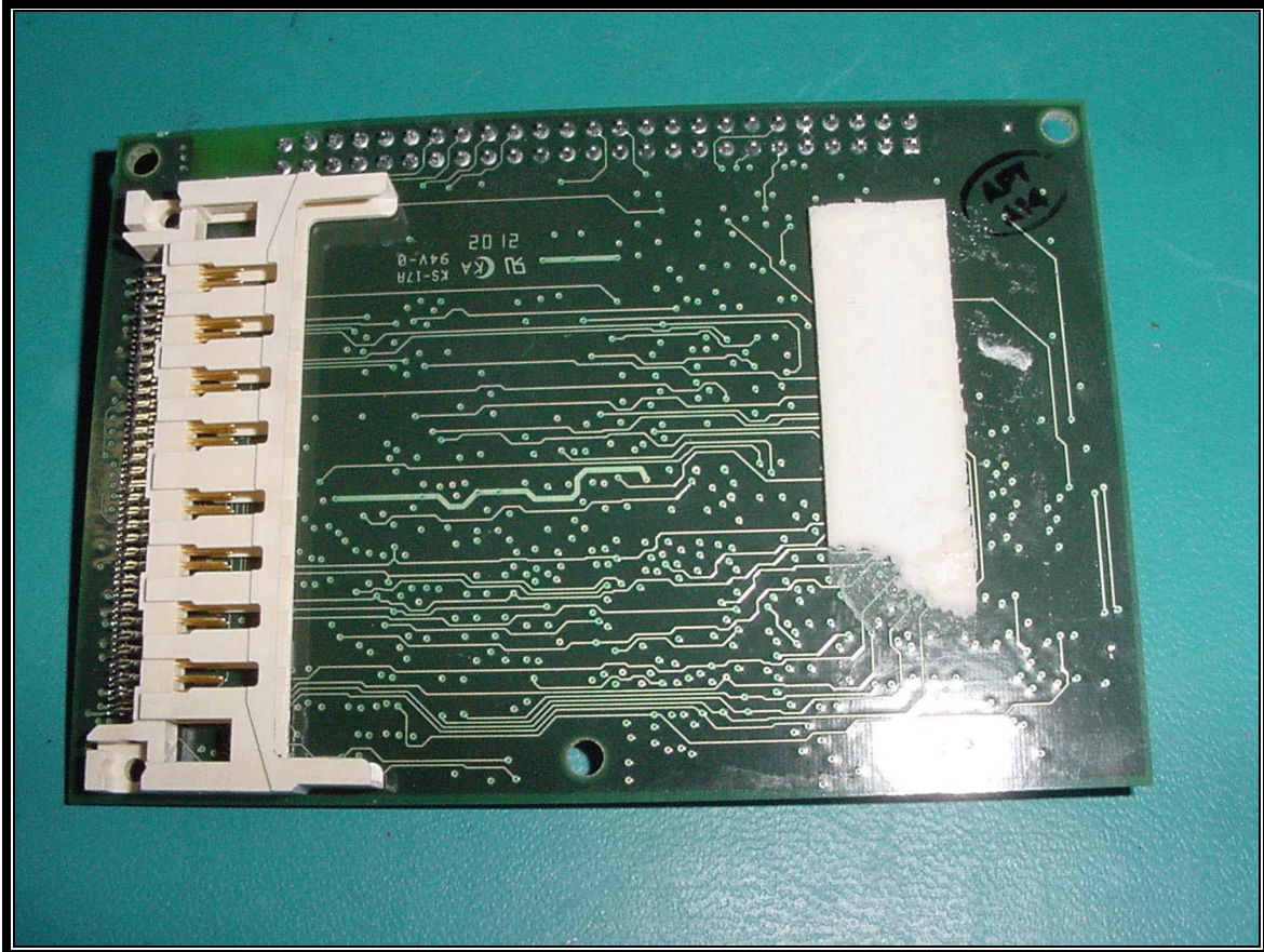
PHOTOGRAPH 24: PRINT SERVER PCB BACK VIEW WITH WLAN PCMCIA CARD AND PCB MOUNTING ADAPTER REMOVED
