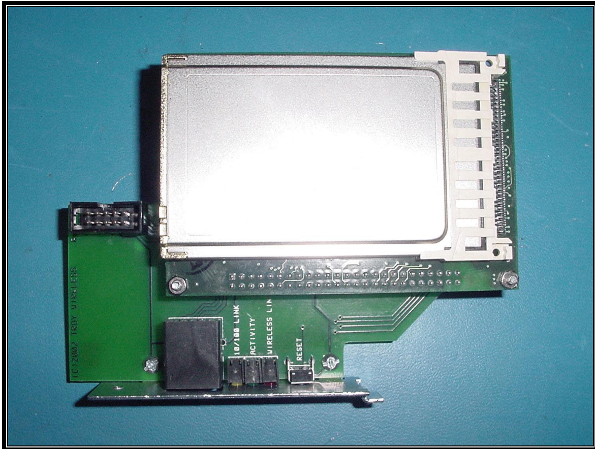
PHOTOGRAPH 16: PRINT SERVER TOP VIEW
