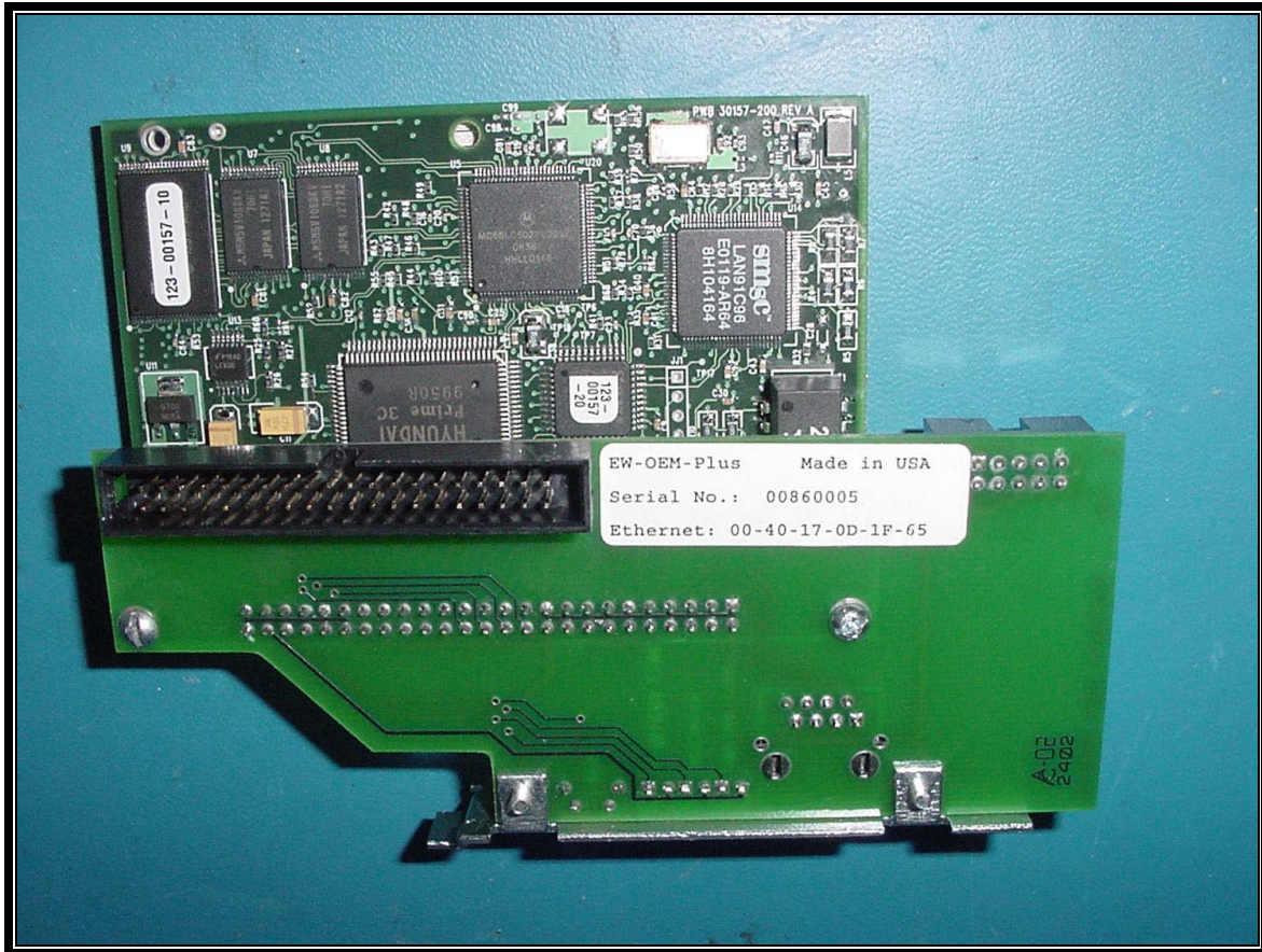
PHOTOGRAPH 17: PRINT SERVER REAR VIEW
