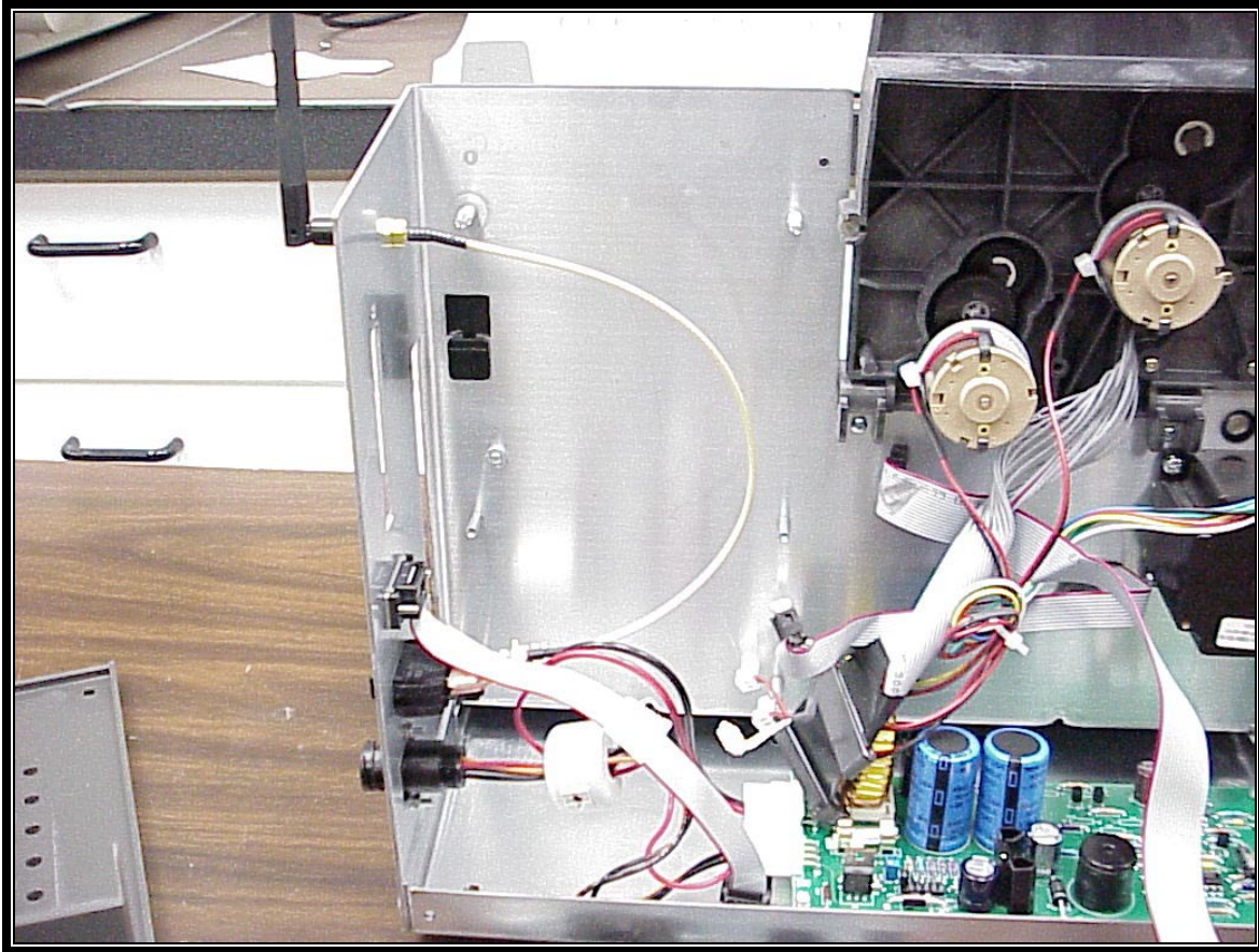
PHOTOGRAPH 9: MAIN PRINTER CONTROL BOARD REMOVED, DC POWER SUPPLY PCB VISIBLE, CABLE TO RIGHT ANGLE ANTENNA
