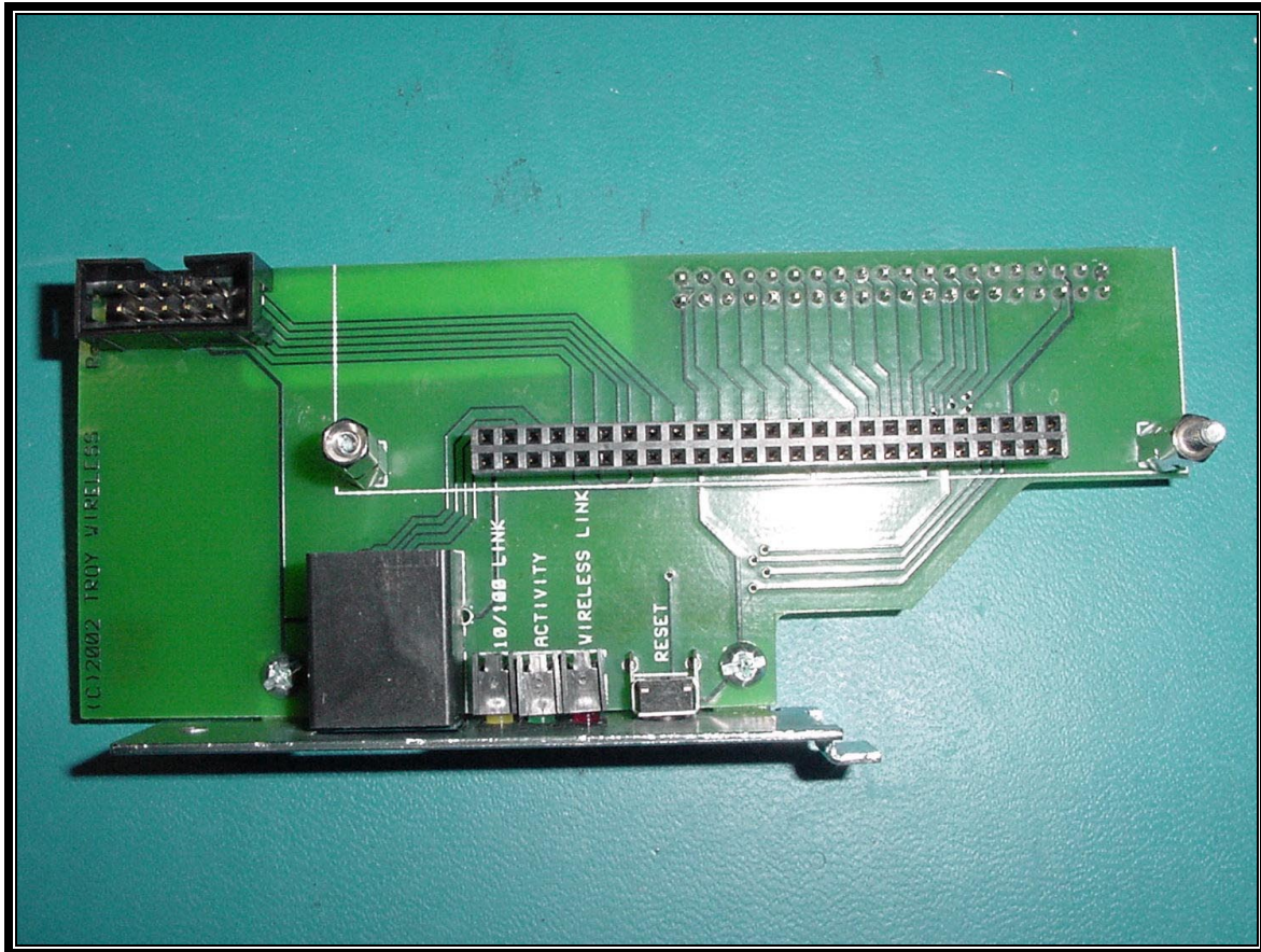
PHOTOGRAPH 18: PRINT SERVER MOUNTING ADAPTER PCB
