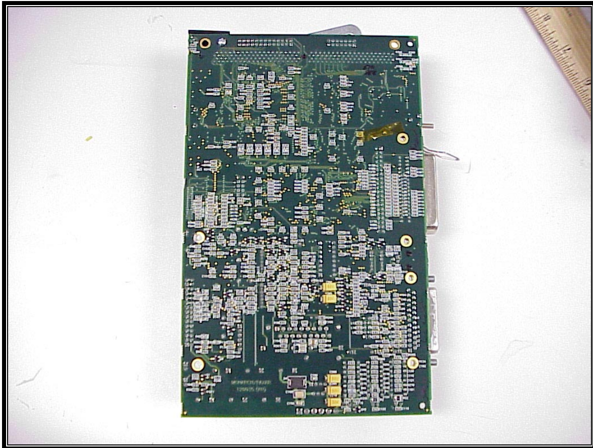
PHOTOGRAPH 15: MAIN PRINTER SYSTEM CONTROL BOARD BACK VIEW
