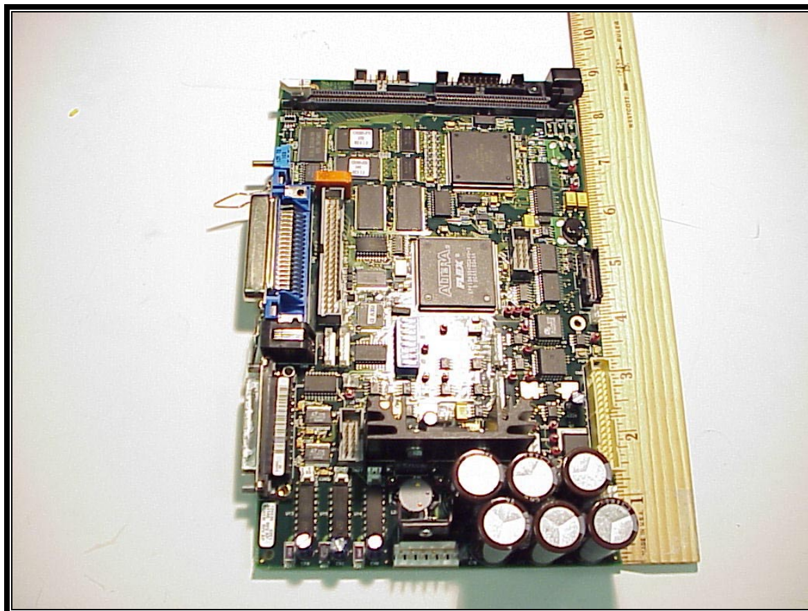
PHOTOGRAPH 14: MAIN PRINTER SYSTEM CONTROL BOARD WITH CONNECTOR WHERE PRINT SERVER PLUGS IN
