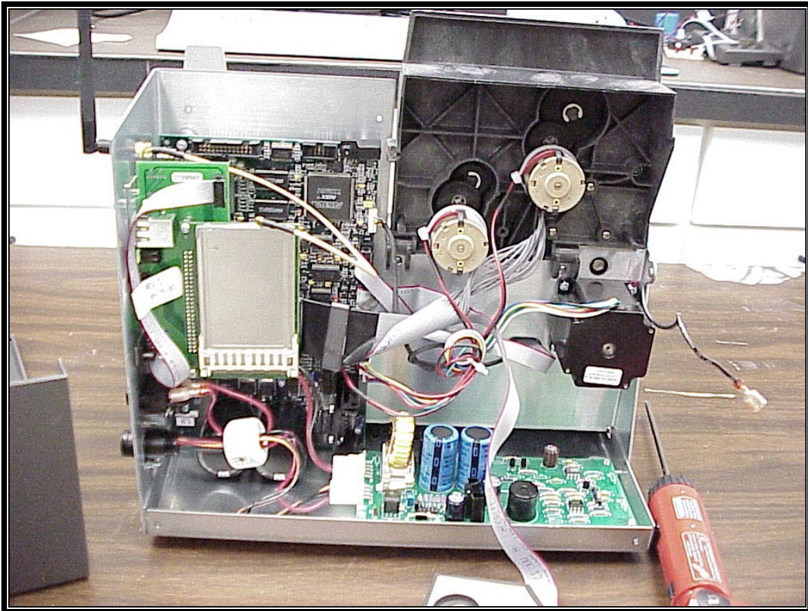
PHOTOGRAPH 13: PRINT SERVER AND WLAN CARD MOUNTED IN PLACE WITH CABLE TO RIGHT ANGLE ANTENNA
