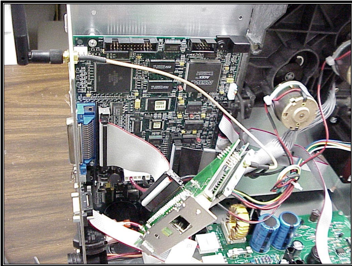
PHOTOGRAPH 12: PRINT SERVER PLUGGED INTO MOUNTED MAIN PCB WITH CABLE TO RIGHT ANGLE ANTENNA
