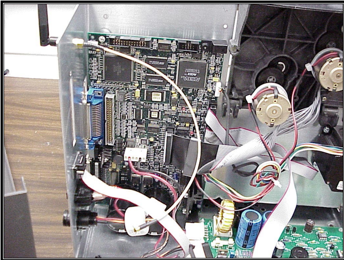
PHOTOGRAPH 10: MOUNTED MAIN PCB WITH PRINT SERVER CONNECTOR
