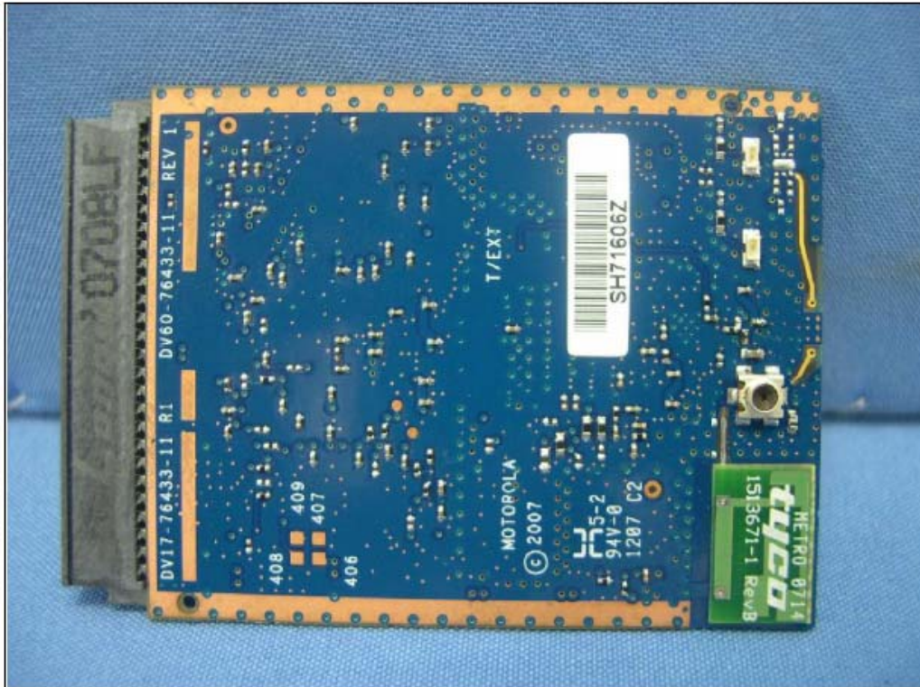
Solder View
